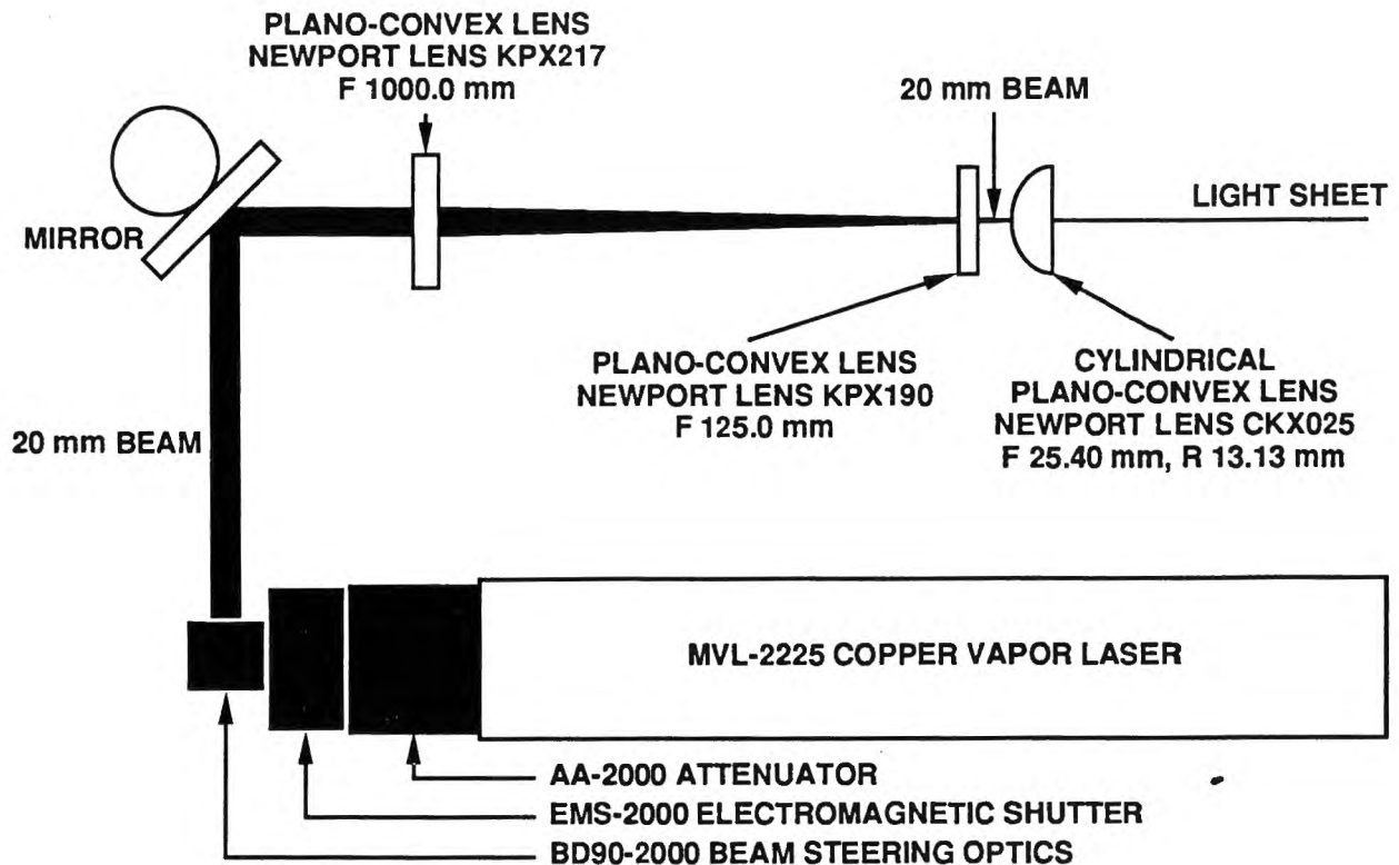
Figure 3. Optical Train
