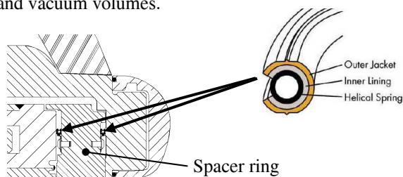
Figure 4. Vacuum spacer and metal seal design
