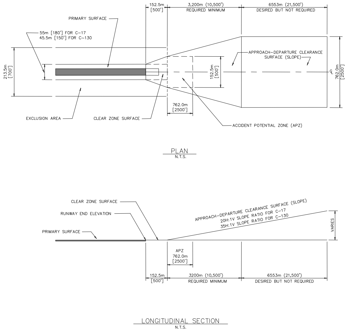
Figure 2-3 Typical Clear Zone and Approach-Departure Clearance Surface
