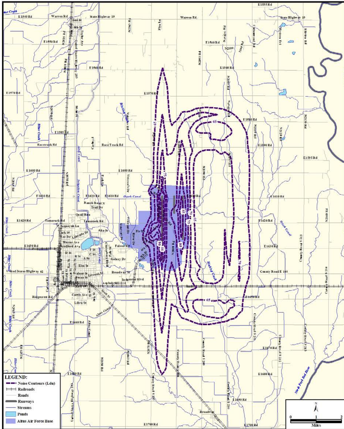
Figure 4-3 Noise Contours, Peak Condition, Alternative Action, Altus Air Force Base
