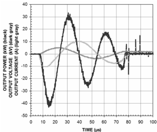
Figure 9. The current (light gray), voltage (dark gray) and power (black) waveforms produced by the FMG across an 18 nF capacitor bank. The pulse-generating coil contained 252 turns.
