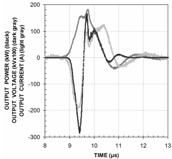
Figure 10. Waveforms of the output high voltage (dark gray), current (gray) and power (black) pulses produced by an FEG connected to a 36 nF capacitor bank.
