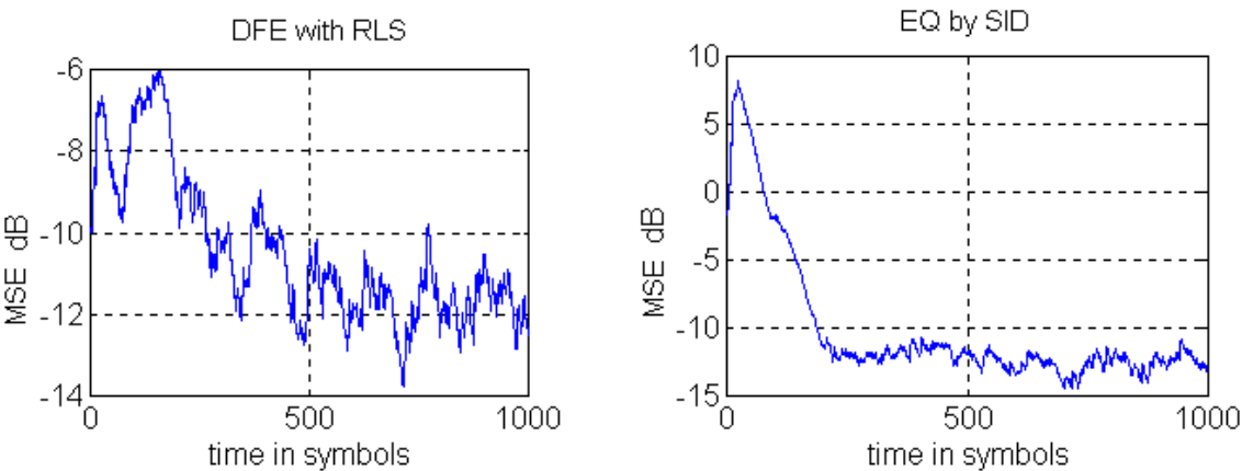
Fig. 2: Performance comparison of SID vs. Decision Feedback Equalizer for an RLS adaptation scheme.
