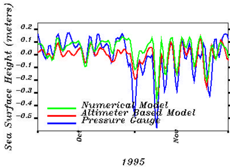
(b) The SSH time series inferred from the pressure gauge and observed from the statistical and numerical models at the same point..
