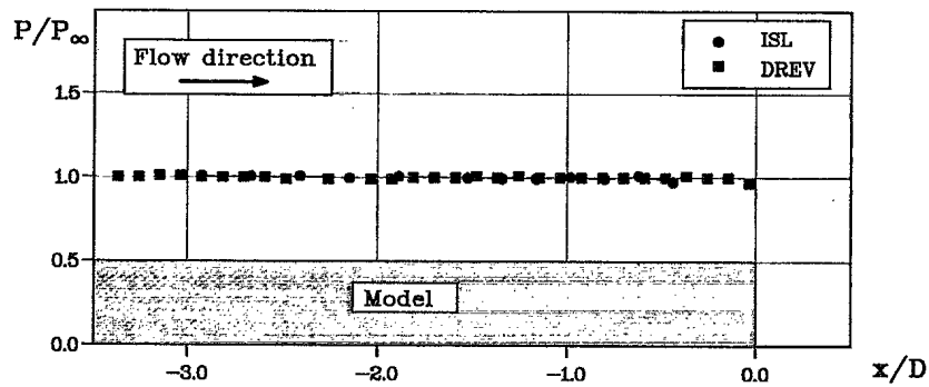
FIGURE 14 - Pressure distributions along the afterbody (up stream sting)
