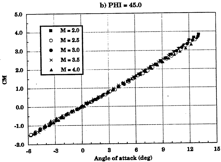
FIGURE 34 - Mach number effects on the pitching moment coefficient (Model B)
