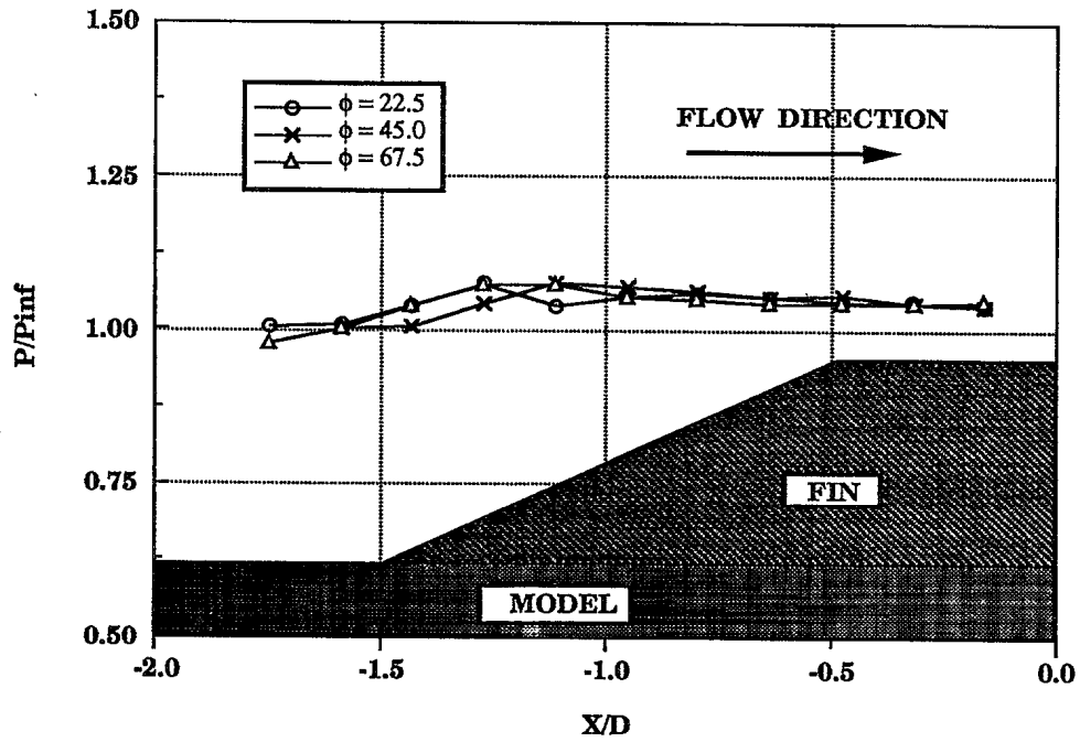
f) DREV results on up stream sting for \alpha = 0^\circ and \phi = 0^\circ
