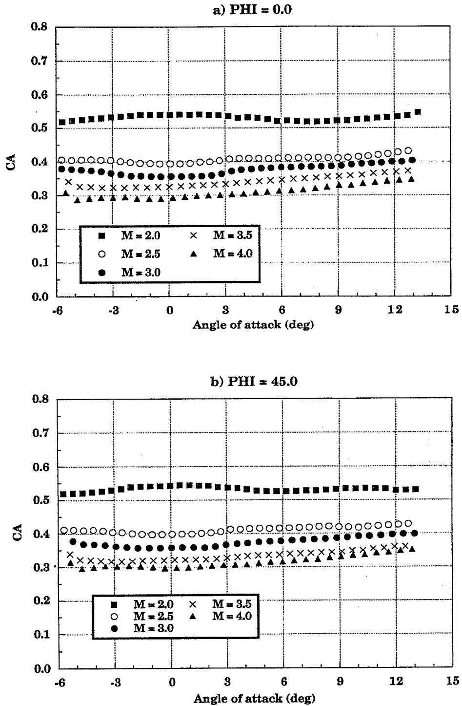
FIGURE 26 - Mach number effects on the axial force coefficient (Model B)
