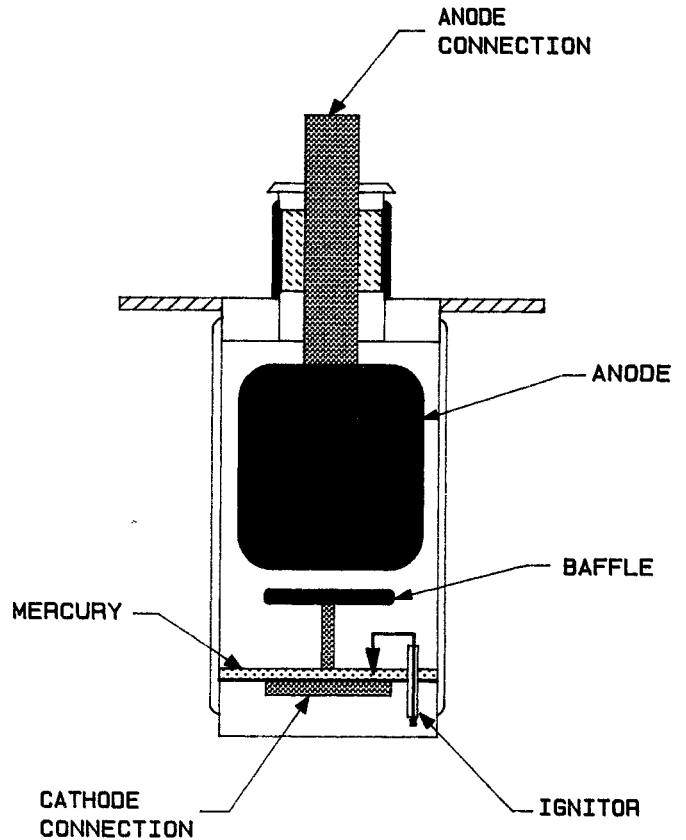
Figure 1. Cross-section of an ignitron.
