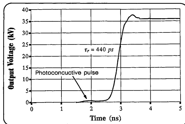
Figure 5: 35 kV pulse generated by avalanche switching of rectangular switch.
