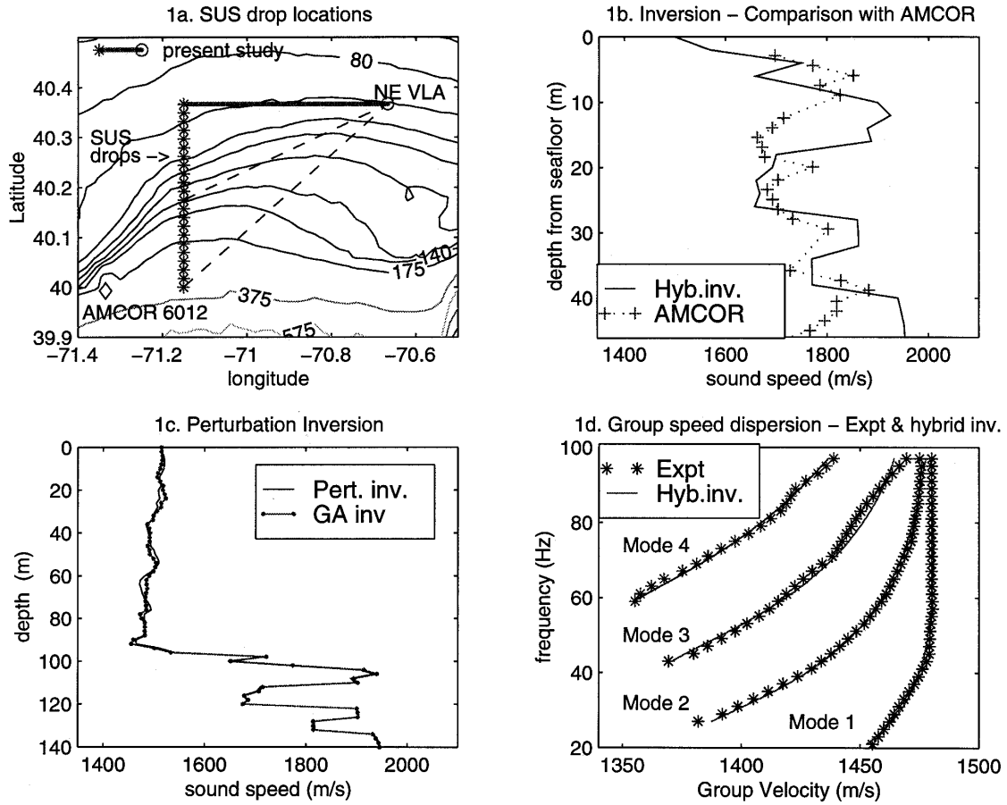
Comparison of inversion results with AMCOR data and Group velocity dispersion. Figure 1a shows the SUS drop locations marked by asterisks and the Northeast Vertical Line Array by a circle. The solid line is propagation path for these inversions. Figure 1b shows the inversion results as a solid line and the Atlantic Margin Coring (AMCOR) site 6012 a plus signs. Figure 1c shows both the water column and sediment inversion, with a solid line for the perturbation method and chain-dots for the Genetic Algorithm inversion. Figure 1d shows the agreement between the measured and the modeled dispersion for modes
