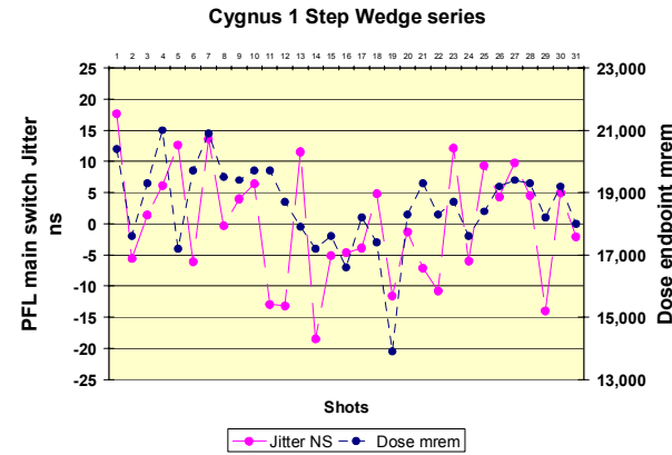
Figure 7. Cygnus 1 – Step Wedge series.
