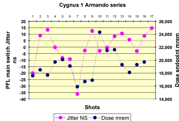
Figure 5. Cygnus 1 – Armando series.
