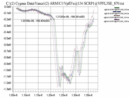
Figure 4. Four Vpfl3 traces showing main PFL switch jitter. From the Cygnus 1 Armando series.
