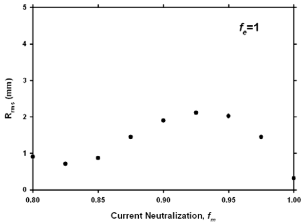
Figure 2. The ballistically-focused diode beam intrinsic spot size at optimally positioned converter as a function of current neutralization for fully space-charge neutralized beam ( f_e=1 ).
