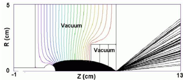
Figure 5. 14-MeV beam focused by anode foil, with additional grids to short out the residual space-charge fields.
