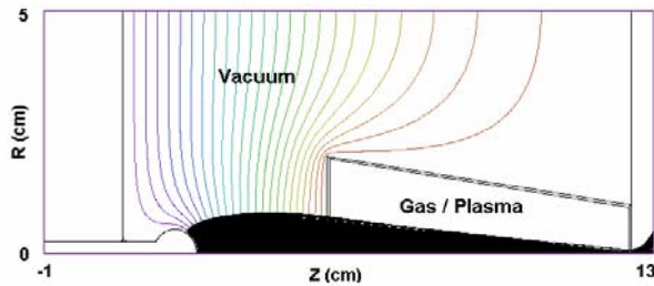
Figure 1. Ideal ballistically-focused diode 14-MeV diode with force-free, ballistic electron trajectories ( f_e=1, f_m=1 ) and optimum gas cell length.
