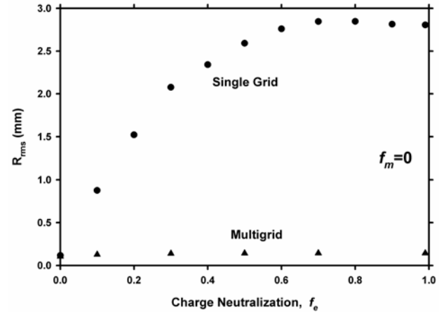
Figure 7. Effect of neutralization by gas desorbed from heated target on the intrinsic spot size of grid focus cells. (Circles) Single grid cell. (Triangles) Multigrid cell. .
