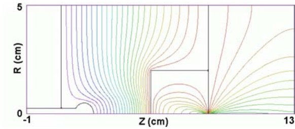
Figure 4. Equipotential contours including space charge for the grid-focus cell shown in Fig. 3.
