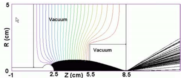
Figure 3. 14-MeV beam focused using only the anode grid. The entire diode volume, including the cell, is in vacuum.
