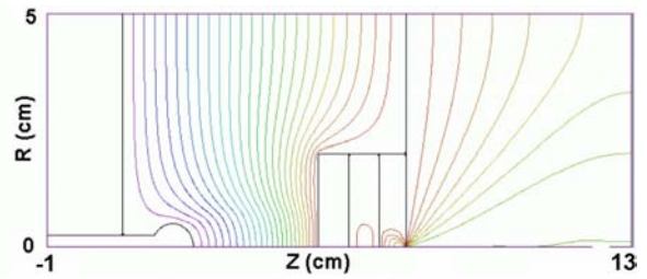
Figure 6. Equipotential contours including space charge for the multi-grid focus cell shown in Fig. 5.
