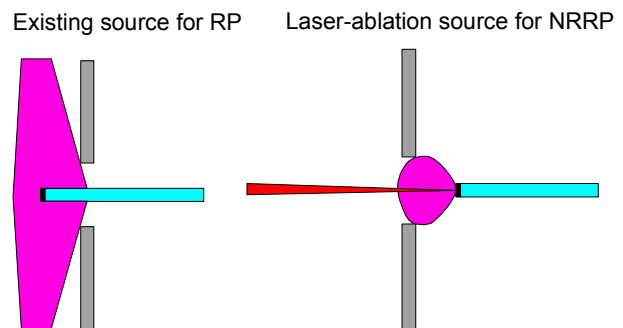
Figure 12. Plasma injection schemes.
