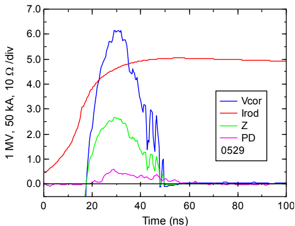
Figure 13. Results from an initial shot with plasma injection
