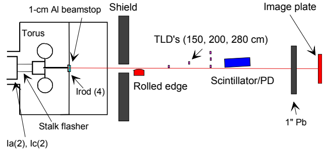
Figure 2. Experimental arrangement.
