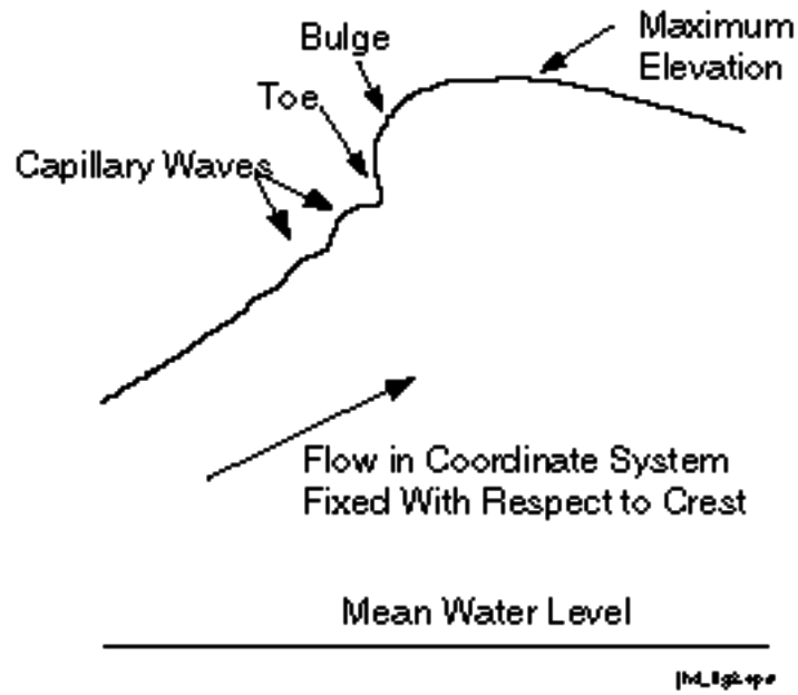
Figure 2. Schematic Showing Nomenclature for Breaking Wave Profiles
