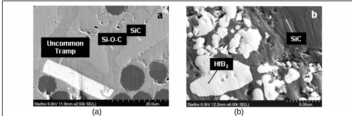
Figure 1.3: A UHTC composite was created by adding a \text{HfB}_2 rich coating on one side of a carbon fiber and a C/SiC rich coating on the other. Both matrices also had an allylhydridopolycarbosilane polymer that acts a binding agent. These FESEM micrographs show the random and non-uniform phase distribution in the UHTC composite, prior to oxidation, for a) the C/SiC rich side and b) the \text{HfB}_2 rich side [11].
