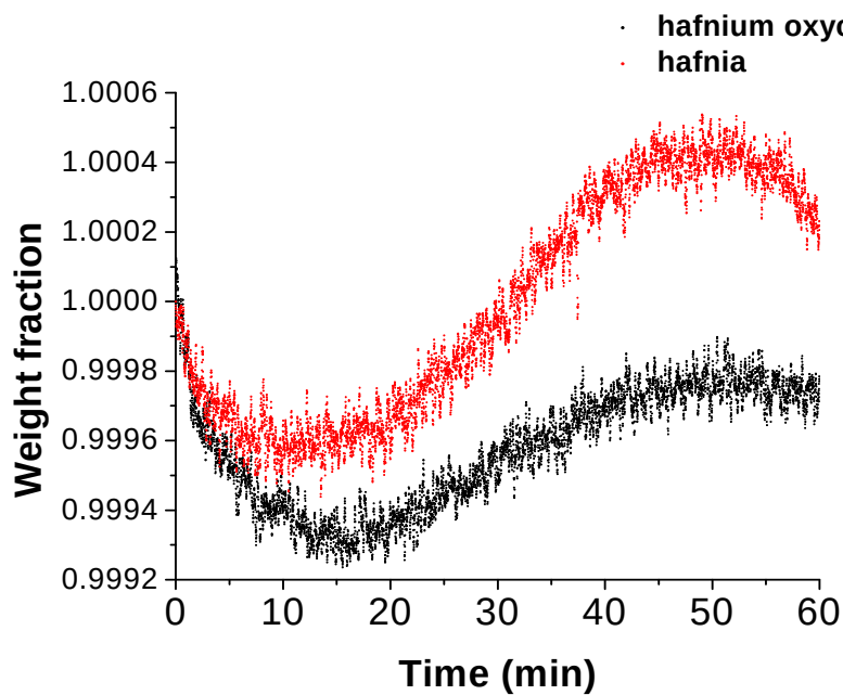
Figure 4.4: The thermogravimetric curves from the oxidation of hafnium and hafnium oxycarbide at a higher temperature of 700 °C.
