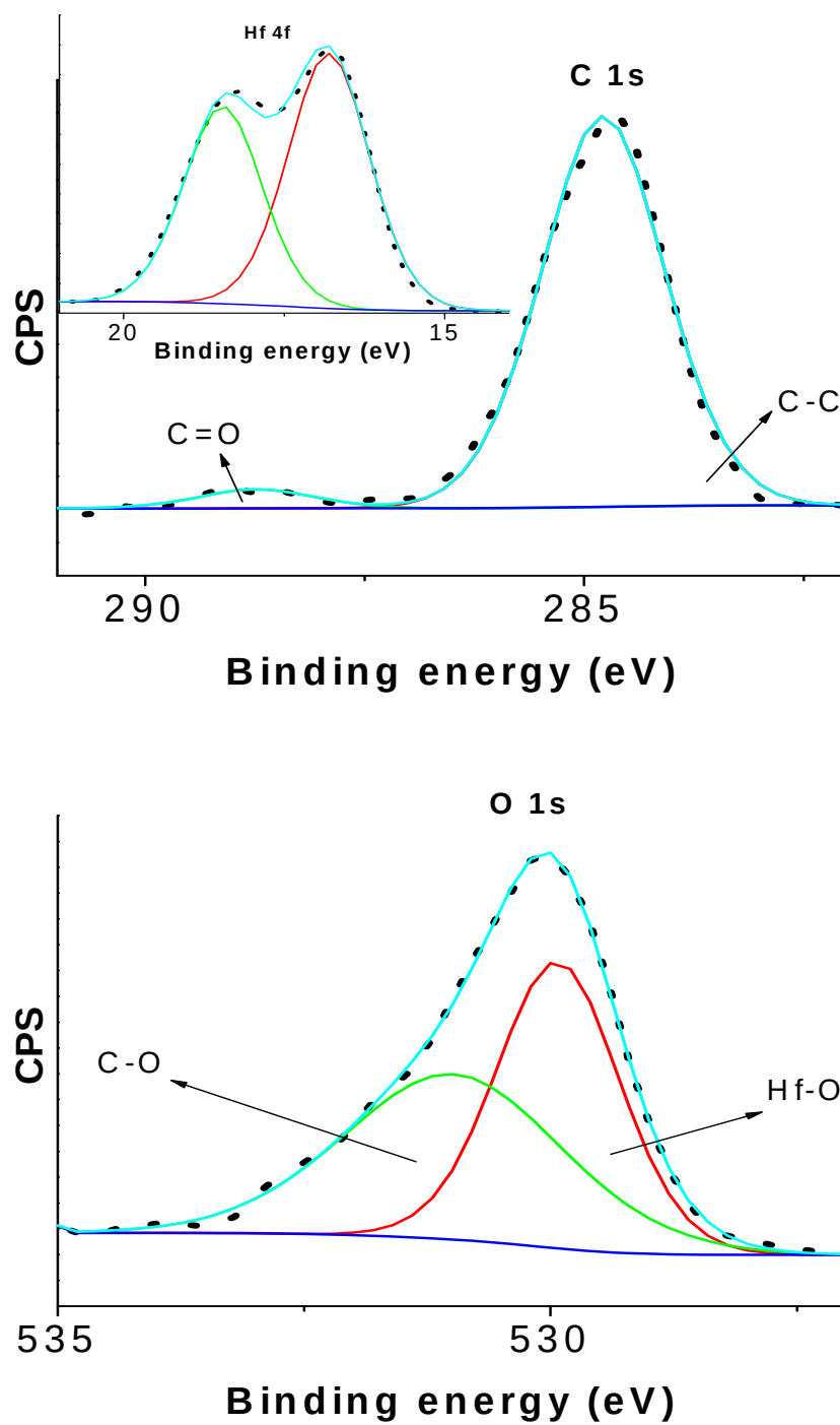
Figure 3.11: Hf 4f (inset), C1s and O1s core shell spectra; counts per second (CPS) versus binding energy, obtained by XPS for film deposited with shadow mask and 5 mTorr Ar.
