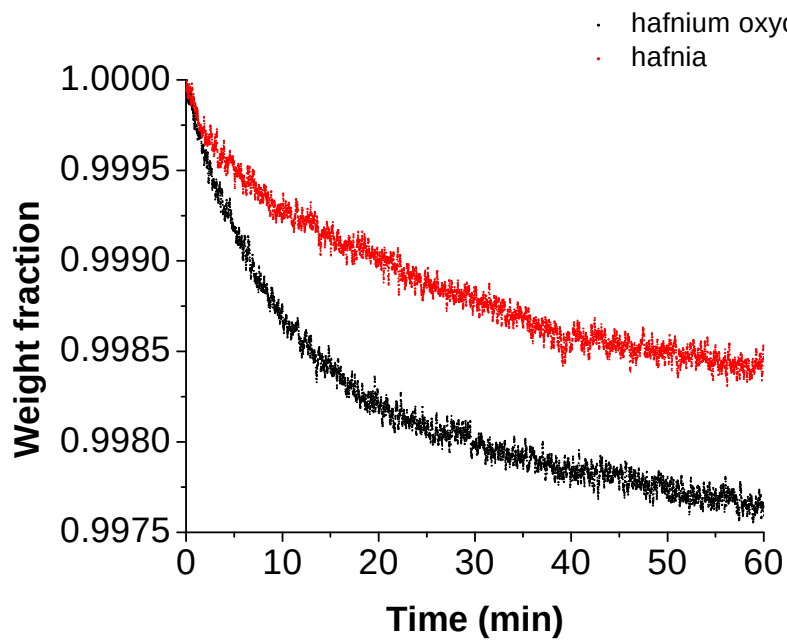
Figure 4.3: The thermogravimetric curves for hafnia and hafnium oxycarbide (28 mTorr) oxidized at 600 °C.
