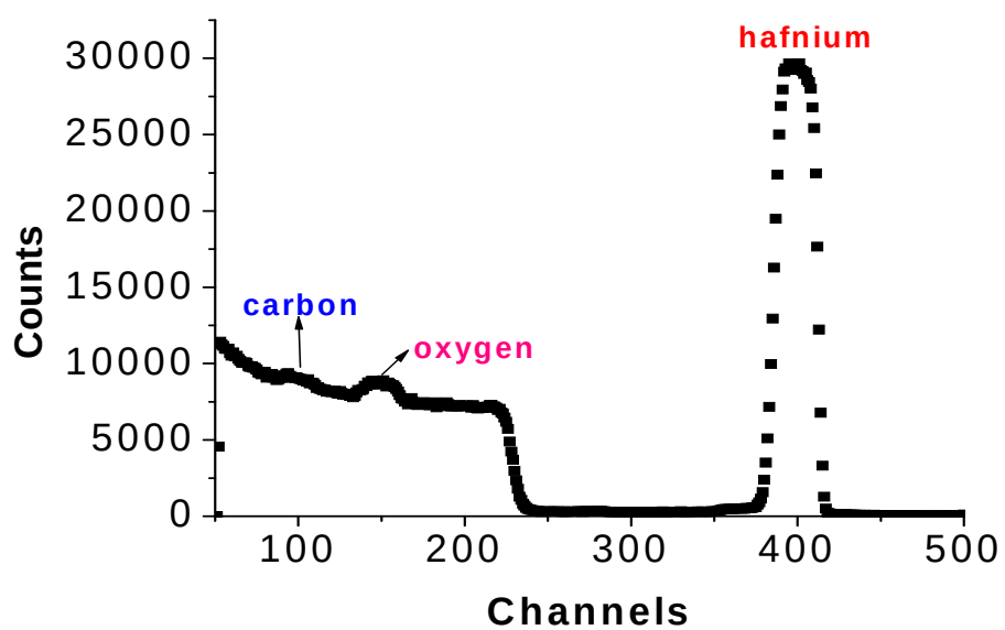
Figure 3.10: RBS spectra for a film deposited with the shadow mask and 20 mTorr Ar from which a ratio of C:Hf=1.5 and O:Hf=2.4 was determined.
