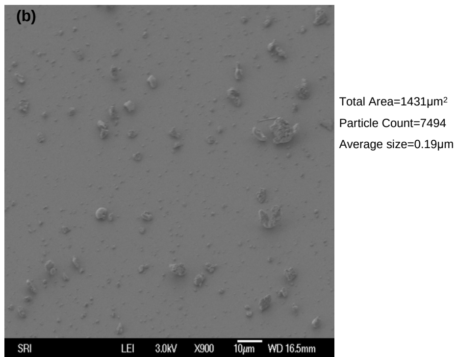
Figure 3.7b: Particle count and SEM image of \text{HfC}_x film deposited with 20 mTorr Ar.
