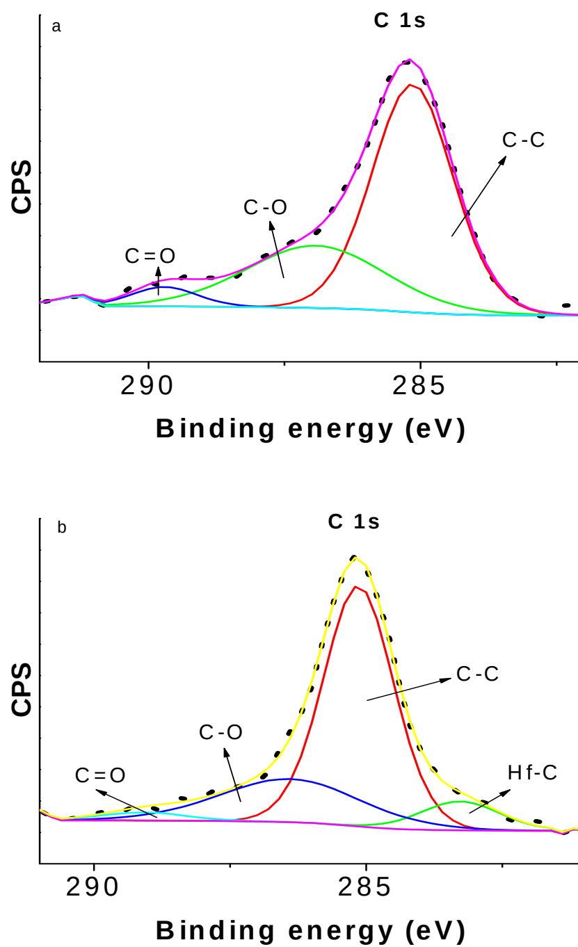
Figure 3.14: Core shell spectra for C1s (a) pre and (b) post sputtering with a 500 V Ar + ion gun.
