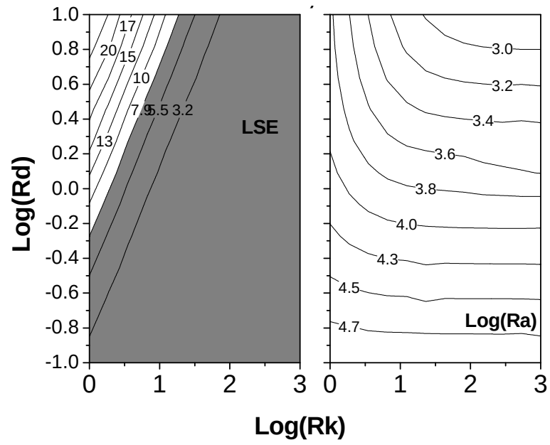
Figure 5.4c: The contour plots for 1150 °C which indicate only a small change from that at T=1050^{\circ}\text{C} in the range of acceptable parameter values.
