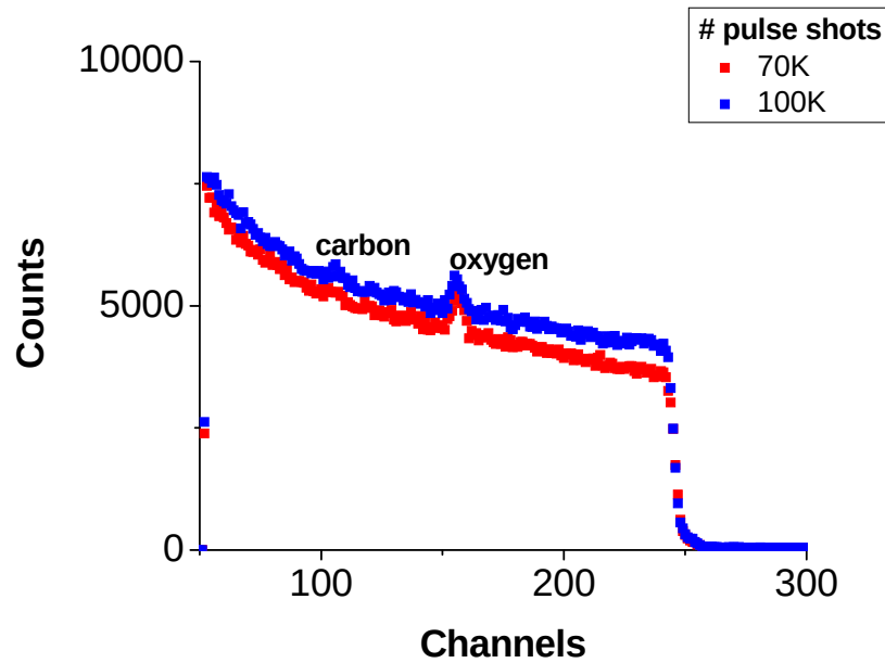
Figure 3.16: RBS spectra for \text{HfC}_x(\text{O}) film deposited with a lower wavelength laser, for a varying number of pulse shots.
