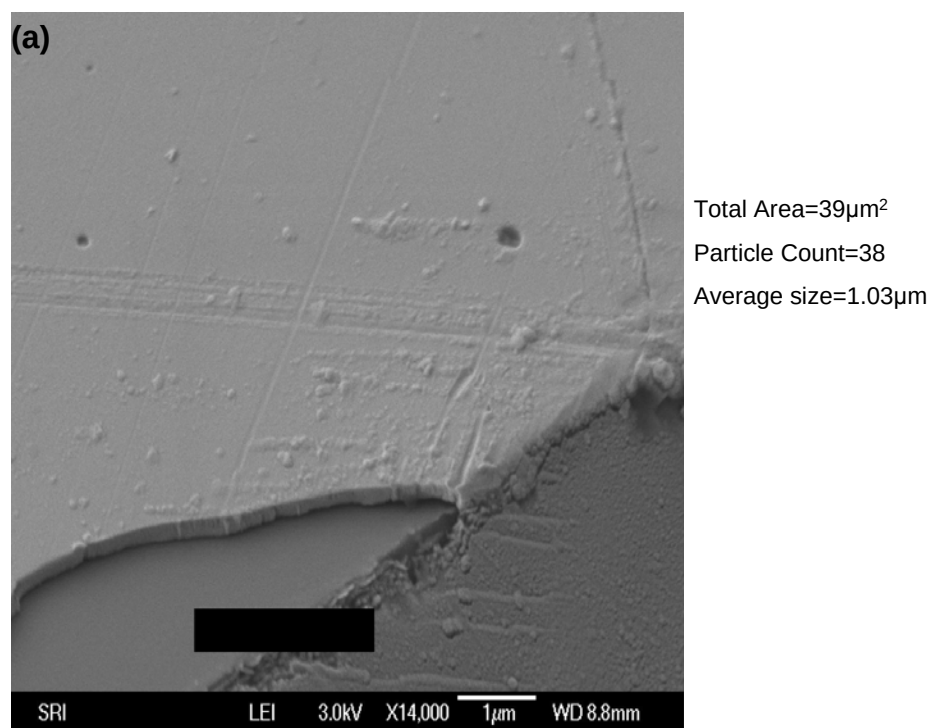
Figure 3.7a: Particle count and SEM image of \text{HfC}_x film deposited with only 5 mTorr Ar.
