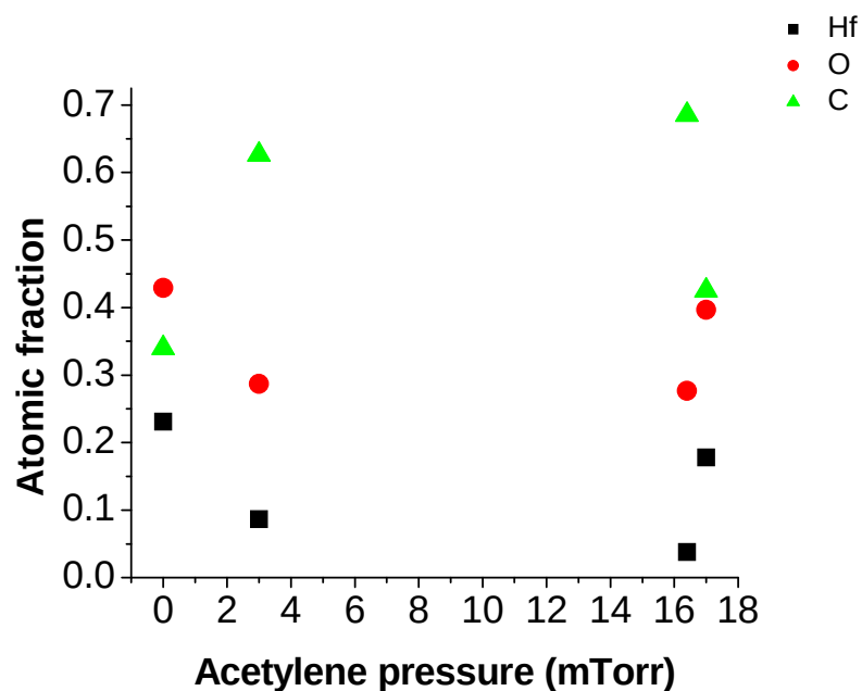
Figure 3.12: Atomic composition variation with pressure increase determined from XPS spectra.
