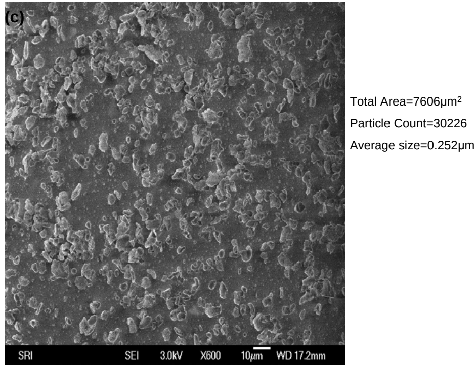
Figure 3.7c: Particle count and SEM image of \text{HfC}_x film deposited with 100 mTorr Ar.
