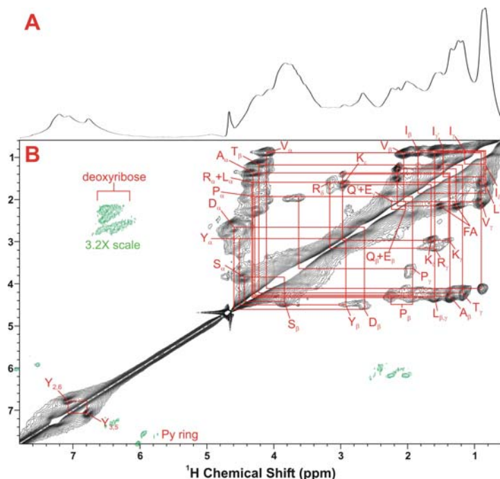
Figure 8. 2-D ^1\text{H} TOCSY spectrum (B) of mobile HS extracted from ^{13}\text{C} -prelabeled PRL60 soil aged in \text{PS}+\text{CaCO}_3 . Also shown is the corresponding 1-D spectrum (A). The red rectangles trace the ^1\text{H} covalent connectivity (expressed as off-diagonal cross-peaks) of various humic substructures (mainly peptidic amino acids). The four sets of green cross-peaks were plotted with 3.2X magnified scale. These data together with the ^1\text{H} - ^{13}\text{C} covalent connectivity obtained from the HSQC spectrum of the same sample allow a reliable assignment of these structures. Py: pyrimidine
