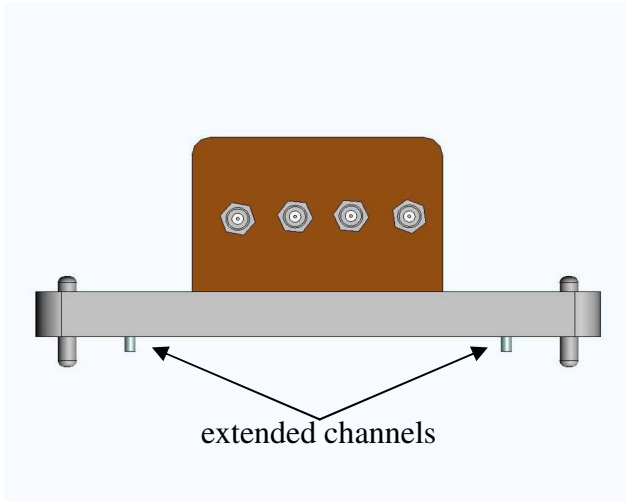
Figure 6. Photodiode framework with extended channels
