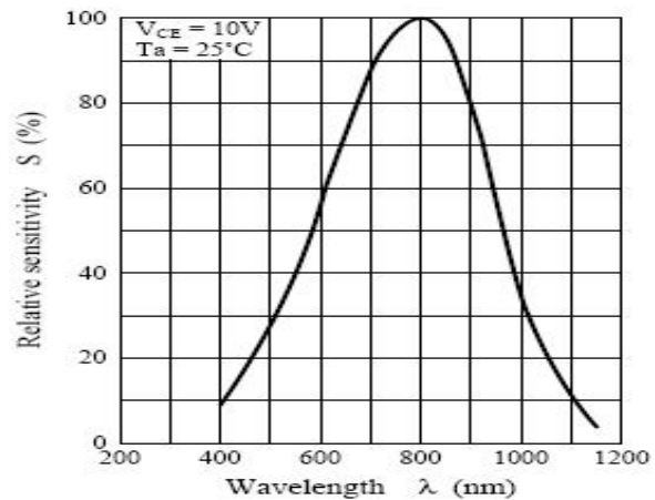
Figure 1. Spectral response of PNZ300 photodiode [3]
