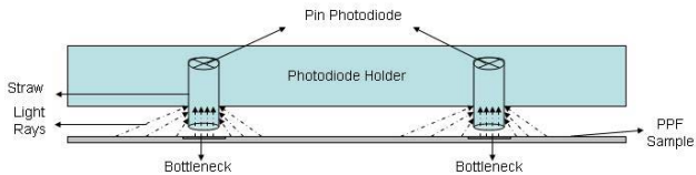
Figure 7. Scenario for light gathering with extended channels
