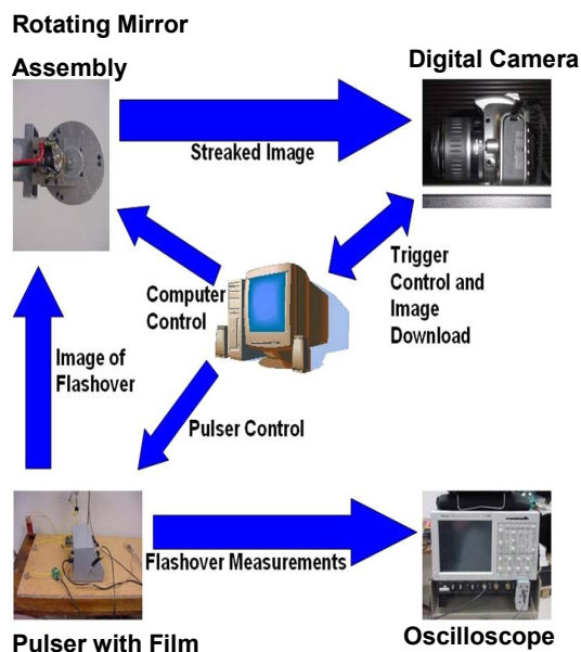
Figure 5. Flow diagram of streak imaging system.
