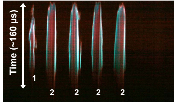
Figure 8. Enhanced streak image of four bottlenecks during aluminum metallization flash
