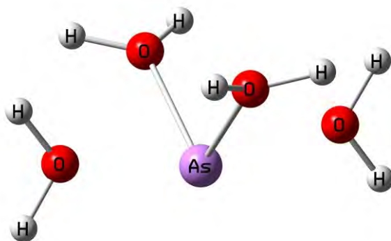
Figure 7c. \text{As}^{+3} 4(\text{H}_2\text{O})
