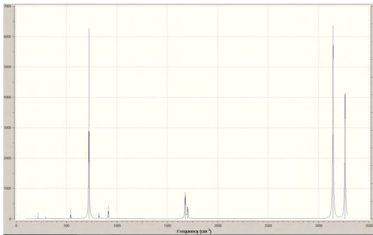
Figure 8a. \text{As}^{+3} 2(\text{H}_2\text{O})
