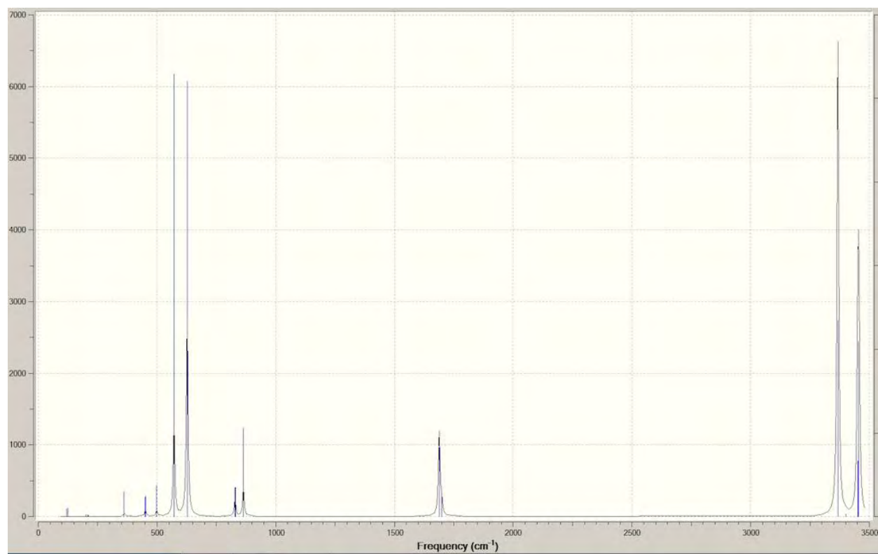
Figure 8b. \text{As}^{+3} 3(\text{H}_2\text{O})
