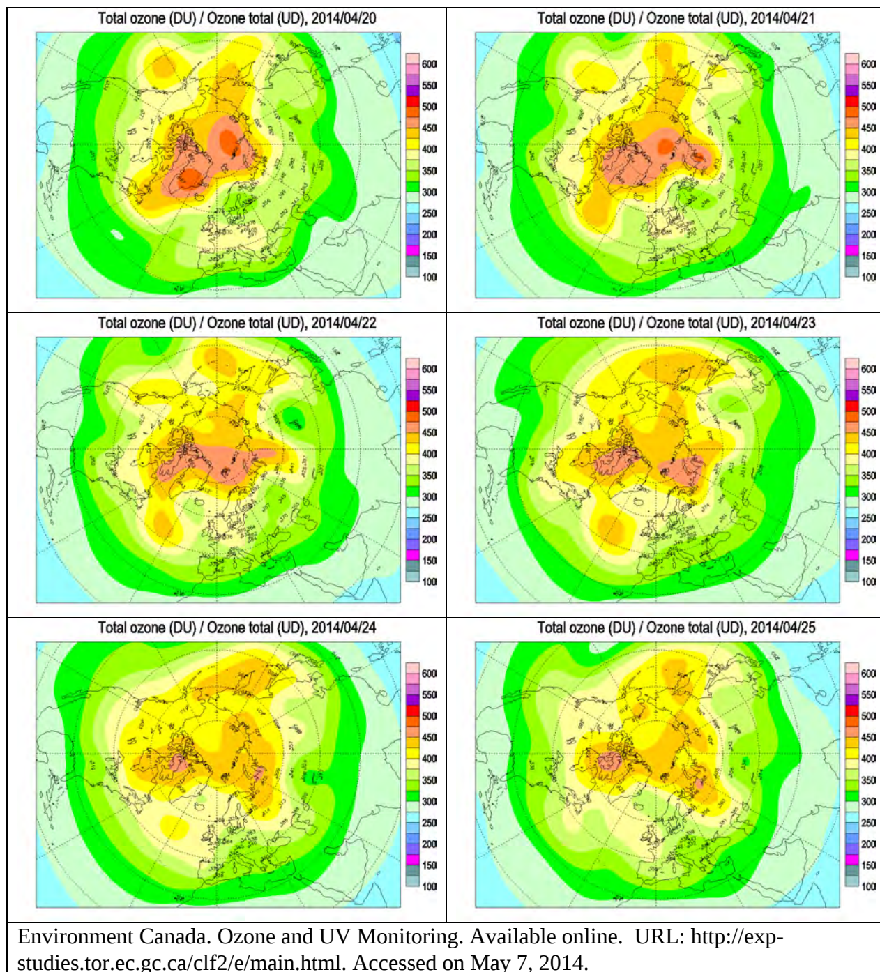
Figure J- 1. Northern Hemisphere Ozone Map from 14-25 April 2014.
