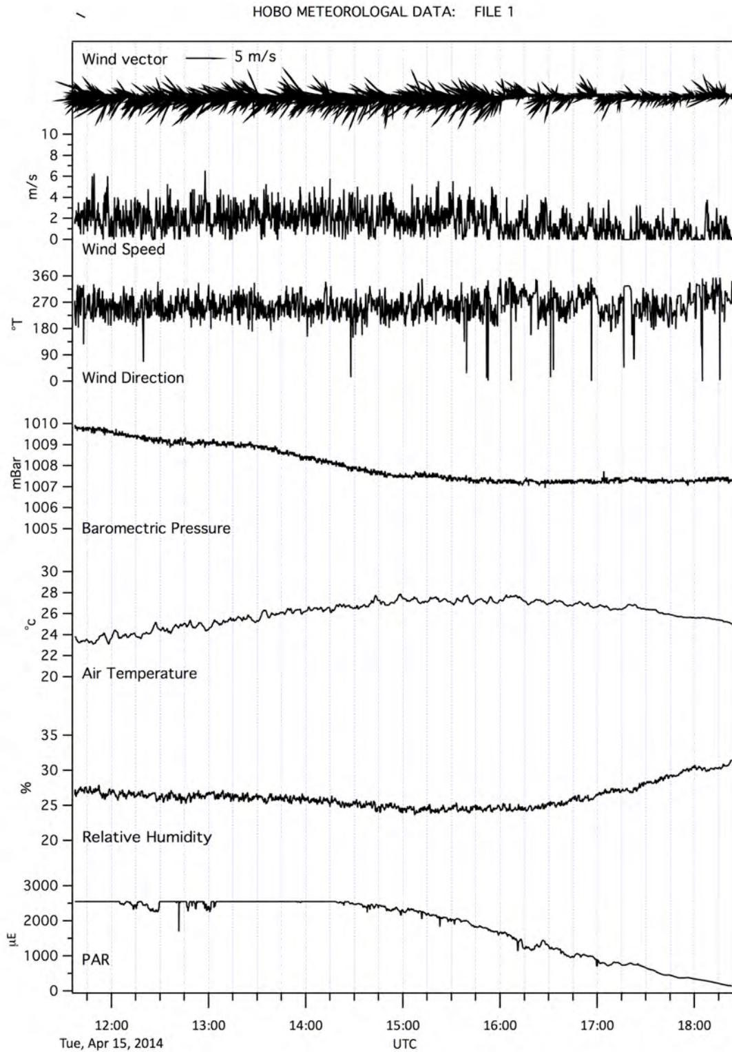
Figure I- 3. HOBO Meteorological Data File 1.
