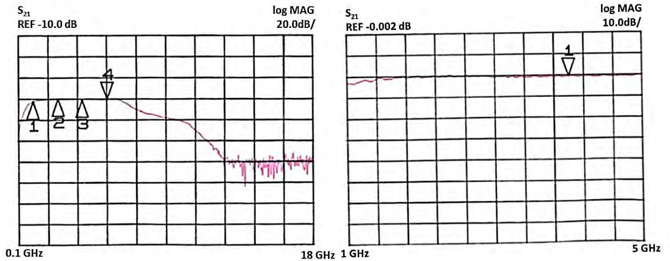
Figure 3 – Bandwidth of Miteq's fiber-optical delay line. Left: 0.1 GHz to 18 GHz, Right: 1 GHz to 5 GHz.
