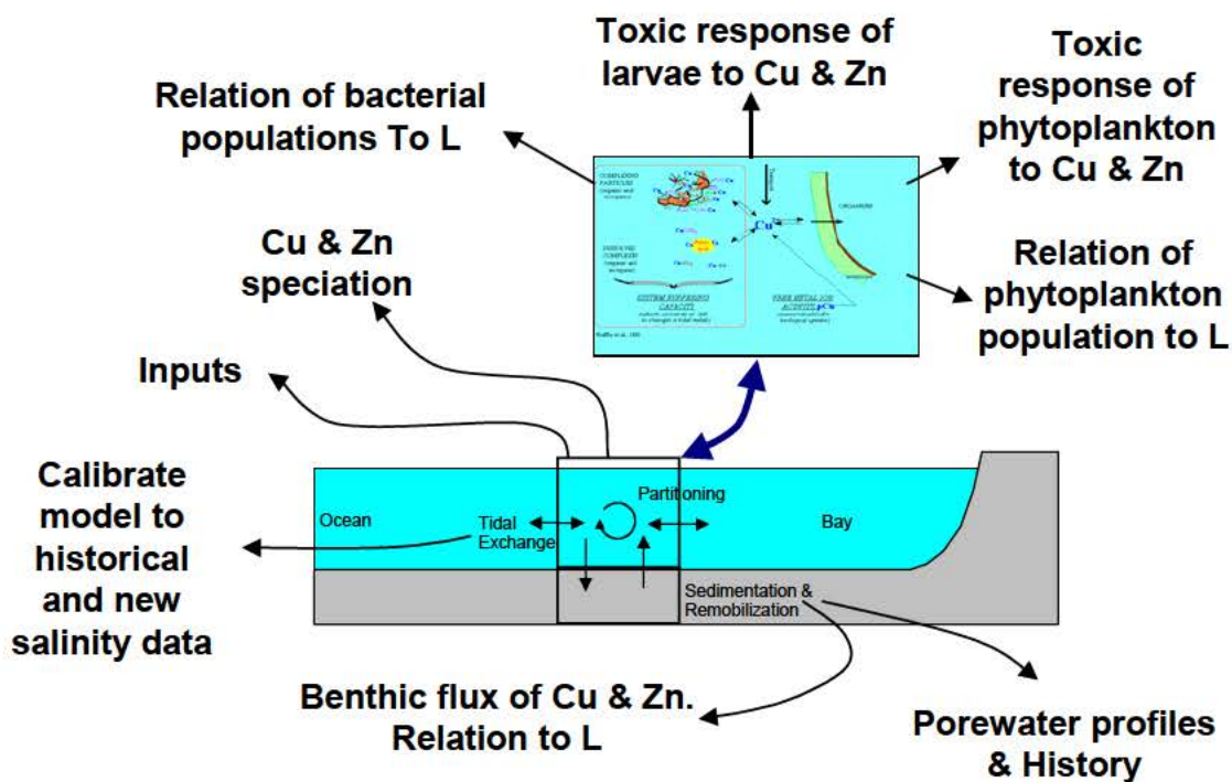
Figure 2. Diagram of the components of the multidisciplinary effort. The top box represents the Free Ion Model (Figure 3) and the chemical characteristics measured in this effort. Similarly, the bottom box represents the physical parameters measured in each of the boxes of the one-dimensional model.
