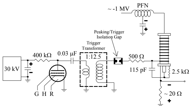
Figure 3. Schematic diagram of the triggering system for the ETDL cascade switch.
