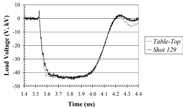
Figure 4. PFN voltage waveforms from the final tabletop test (in V) and from Test Shot 129 (in kV).
