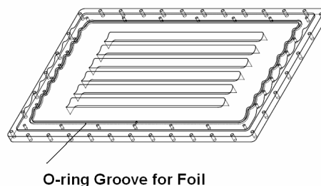
Figure 5. Perspective rendering of hibachi test fixture.
