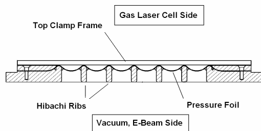
Figure 3. Side view of scalloped hibachi test fixture.
