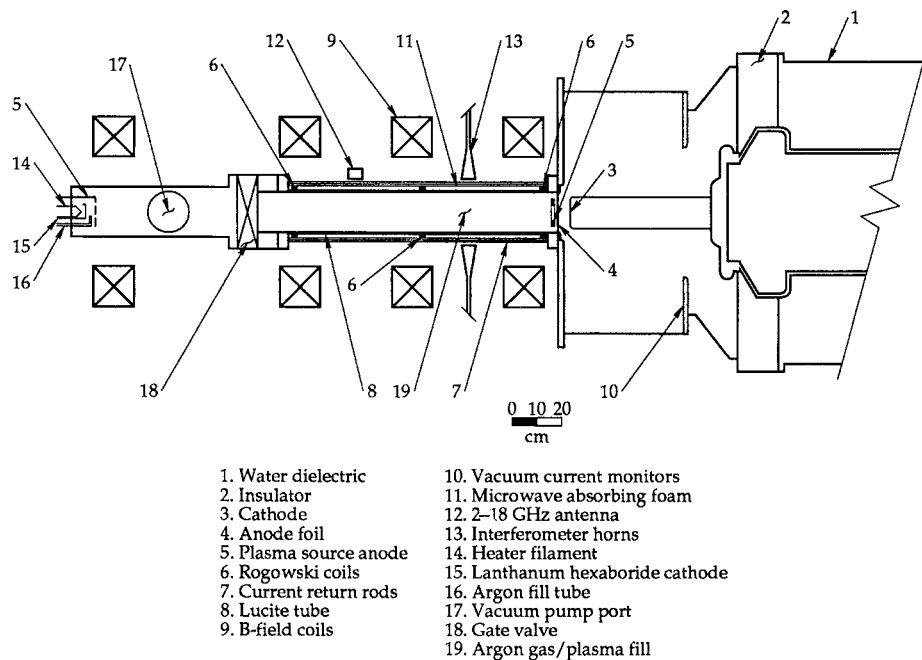
Figure 1—Experimental apparatus.
