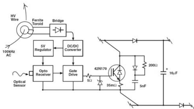
The IGBTs are triggered independently by fiber optic signals received through an optical interface on each stage. We selected the IXYS model IXBT42N170 for the Marx stage switch because it is a good compromise between operating voltage, pulsed current, and commutation speed [11]. We chose the IXYS model DSDI60 fast-recovery diode for the charging elements and a self-healing film capacitor from Aerovox for energy storage.
