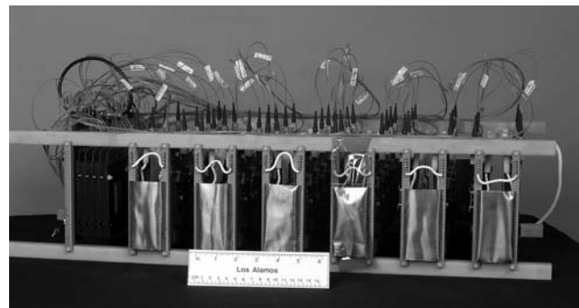
Two views of the assembled modulator are shown in Figures 6 and 7. The assembled modulator weighs 11 kg, and measures 76.2 cm x 30.5 cm x 17.8 cm.
