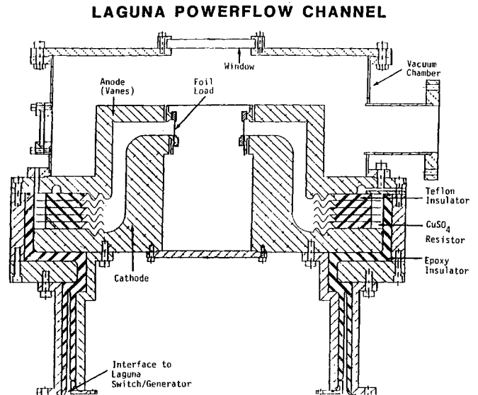
Figure 1. Powerflow Channel.
