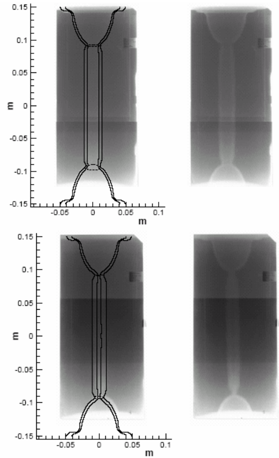
Fig 3: Comparison of 2d-MHD calculation of liner inner and outer boundary with radiographs at 21 \mu s (top) and 22 \mu s (bottom) after start of implosion discharge.
