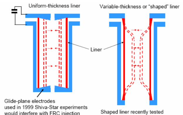
Fig 1: Imploding liner – electrode contacts: sliding shown on left, deformable on right.
