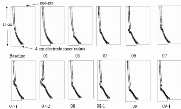
Fig.4: Contour plots of 2D-MHD simulations of liners with various thickness vs axial position profiles. Plots show half (15 cm) of 30 cm tall, 5 cm initial outer radius, Al liner position and shape at 21 \mu s after start of 1300 \mu f, 80 KV, 544 nanoHenry initial inductance Shiva Star discharge with standard safety fuse. Initial liner thickness is 1.1 mm at mid-gap (15 cm above lower electrode).
