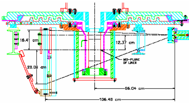
Fig. 2: Experiment setup and geometry. 30 cm tall, 10 cm diameter Al liner and concentric outer conductor are in center. Radiography pulser tube shown on right, just below vacuum current feed. Armored film pack shown on left. Ray traces indicate radiographic coverage. There were two pulsers and film packs, with lines of sight 60 degrees apart.
