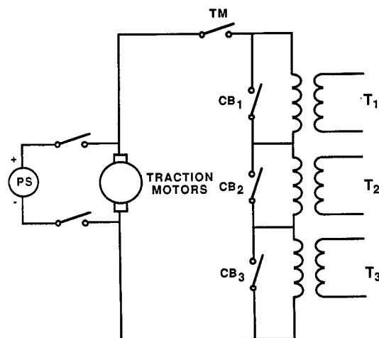
Fig. 1. Simplified LTS circuit diagram.
