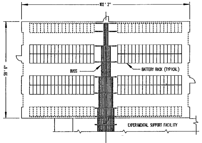
Figure 4. Battery Power Supply Facility Floor Plan.
