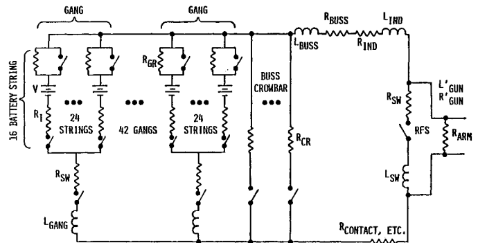
Figure 2. Battery Power Supply Schematic.
