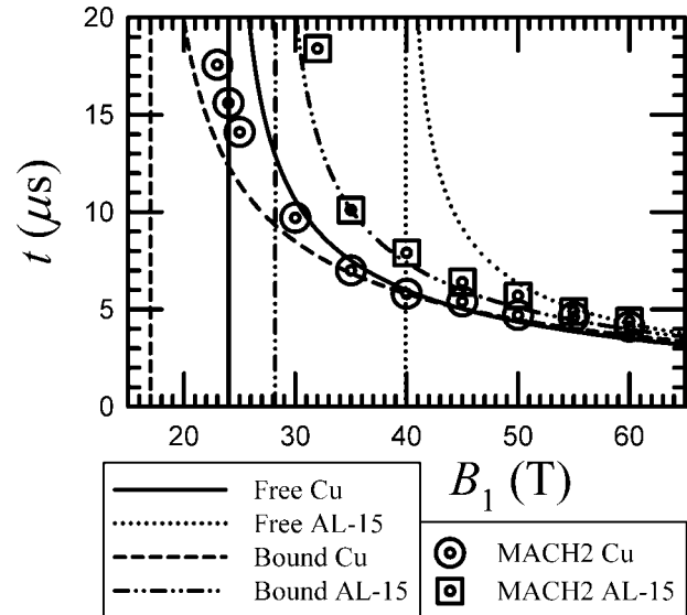
Figure 3. The time it takes a 0.318 cm radius wire in a solenoid with at 10% intertwining gap to spread 10% vs. internal magnetic field. AL-15 and Cu wires using the three theoretical models presented are compared. The vertical lines represent the analytic critical values for B_1 where no deformation occurs.
