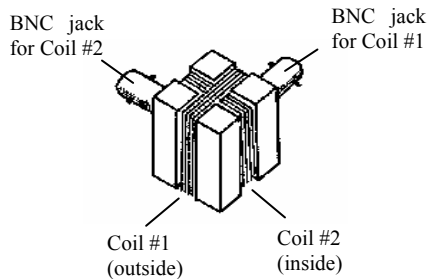
Figure 3. Design of the dual-coil probes.
