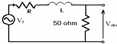
Figure 3. Equivalent circuit of the measurement system.
