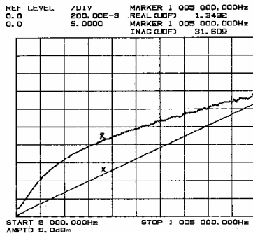
Figure 2. Resistance (upper trace, at 0.2 ohm/div.) and inductive reactance (lower trace, at 5 ohms/div.) change of the inner coil of a dB/dt probe with frequency.
