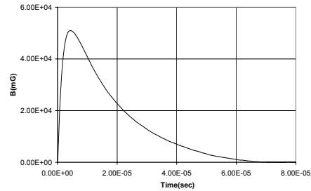
Figure 7. Filtered and calibrated dB/dt probe output; B vs. time function.
