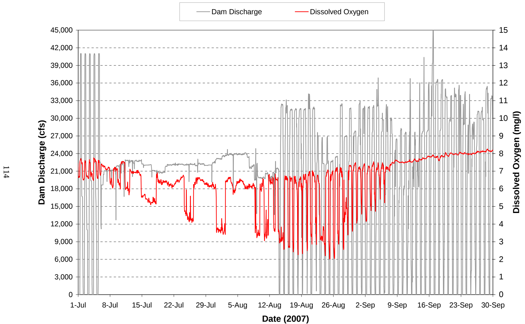
Plate 60. Hourly discharge and dissolved oxygen concentrations monitored at the Fort Randall powerplant during the period July through September 2007.
