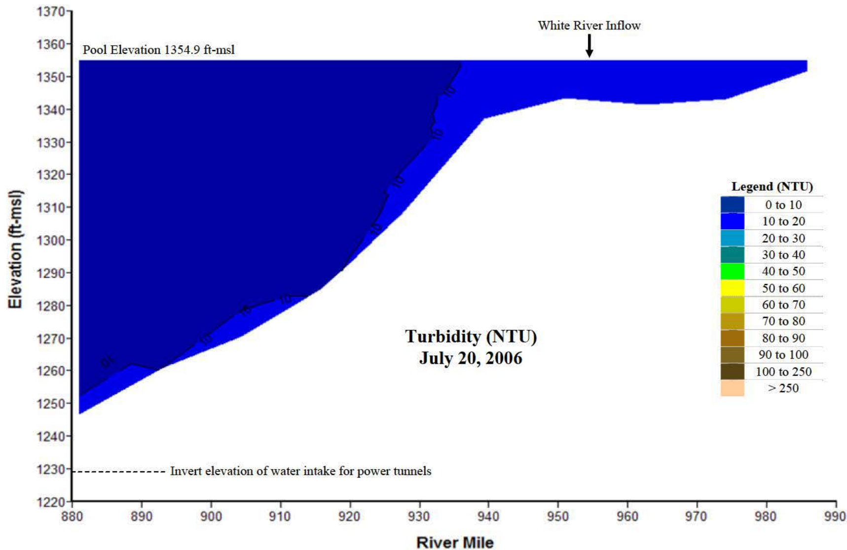
Plate 26. Longitudinal turbidity (NTU) contour plot of Fort Randall Reservoir based on depth-profile turbidity levels measured along the submerged old Missouri River channel at River Miles 880, 892, 911, 924, 940, 955, 968, and 987 on July 20, 2006.
