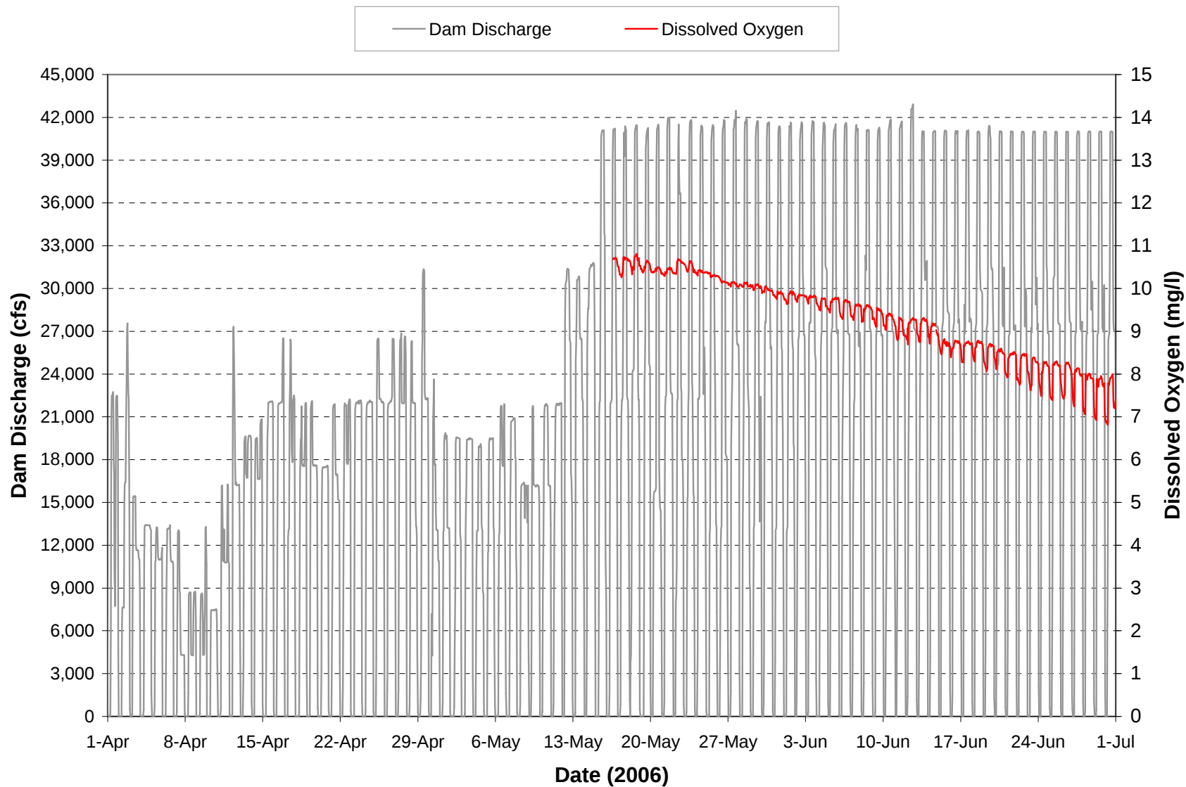
Plate 55. Hourly discharge and dissolved oxygen concentrations monitored at the Fort Randall powerplant during the period April through June 2006. (Note: Gaps in dissolved oxygen plot are periods when the monitoring equipment was not operational.)
