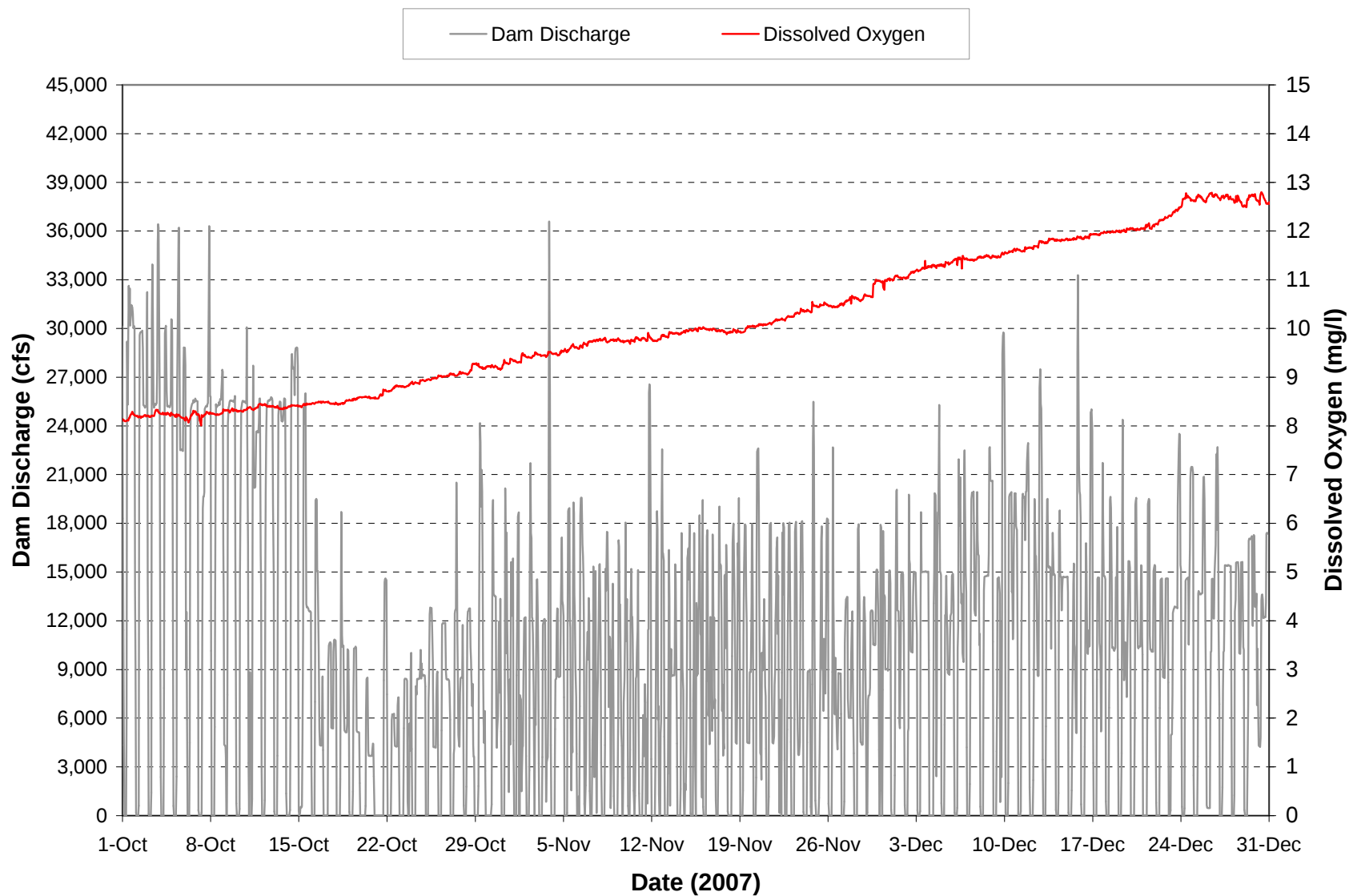
Plate 61. Hourly discharge and dissolved oxygen concentrations monitored at the Fort Randall powerplant during the period October through December 2007.
