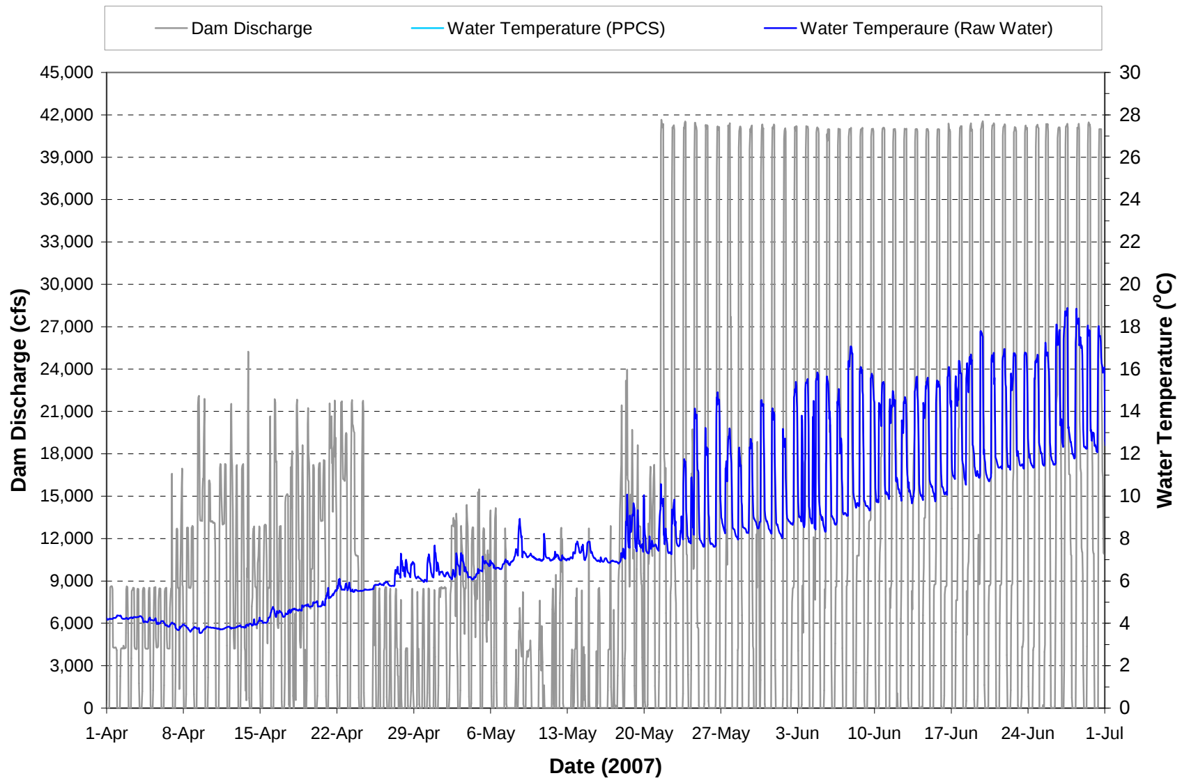
Plate 47. Hourly discharge and water temperature monitored at the Fort Randall powerplant during the period April through June 2007. (Note: Gaps in temperature plot are periods when the monitoring equipment was not operational.)
