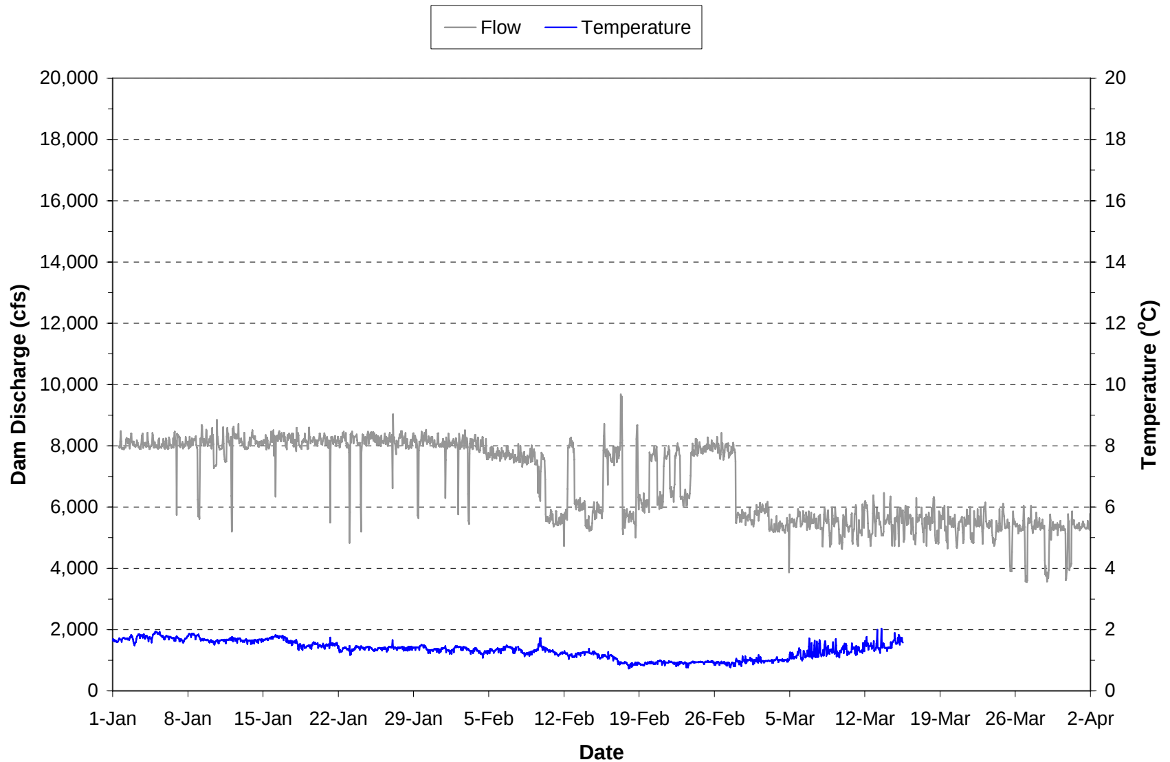
Plate 59. Hourly discharge and water temperature monitored in the “raw water supply line” at the Fort Peck powerhouse during the period January through March 2006. (Note: Gaps in temperature plot are periods when the monitoring equipment was not operational.)
