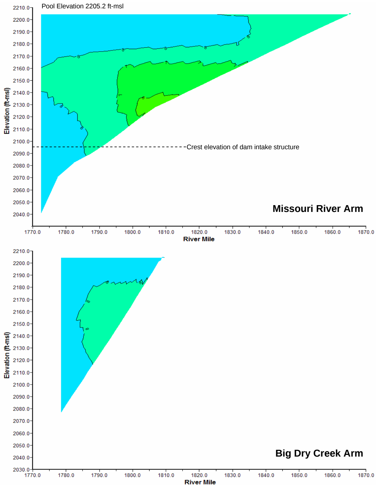
Plate 22. Longitudinal dissolved oxygen contour plot of Fort Peck Reservoir based on depth-profile dissolved oxygen concentrations monitored at sites L1, L2, L3, L4, L5, L6, and NF1 on July 26, 2006.
