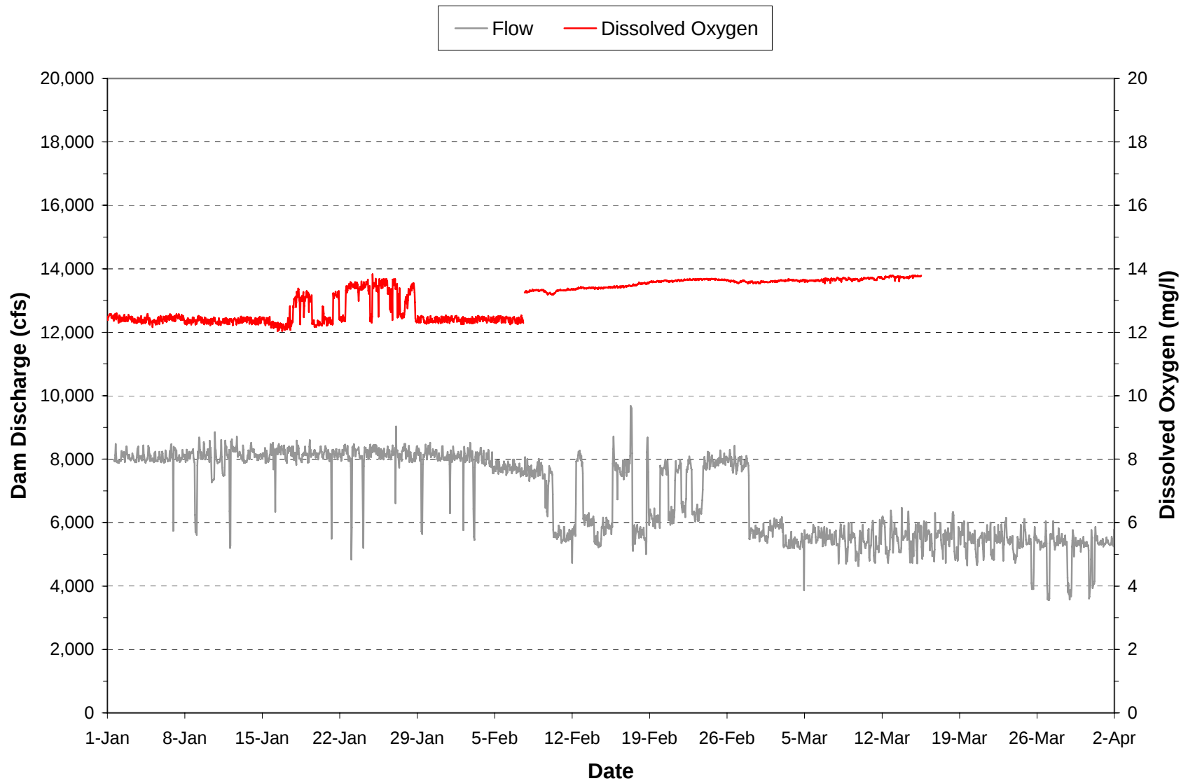
Plate 71. Hourly discharge and dissolved oxygen concentrations monitored in the “raw water supply line” at the Fort Peck powerhouse during the period January through March 2006. (Note: Gaps in dissolved oxygen plot are periods when the monitoring equipment was not operational.)
