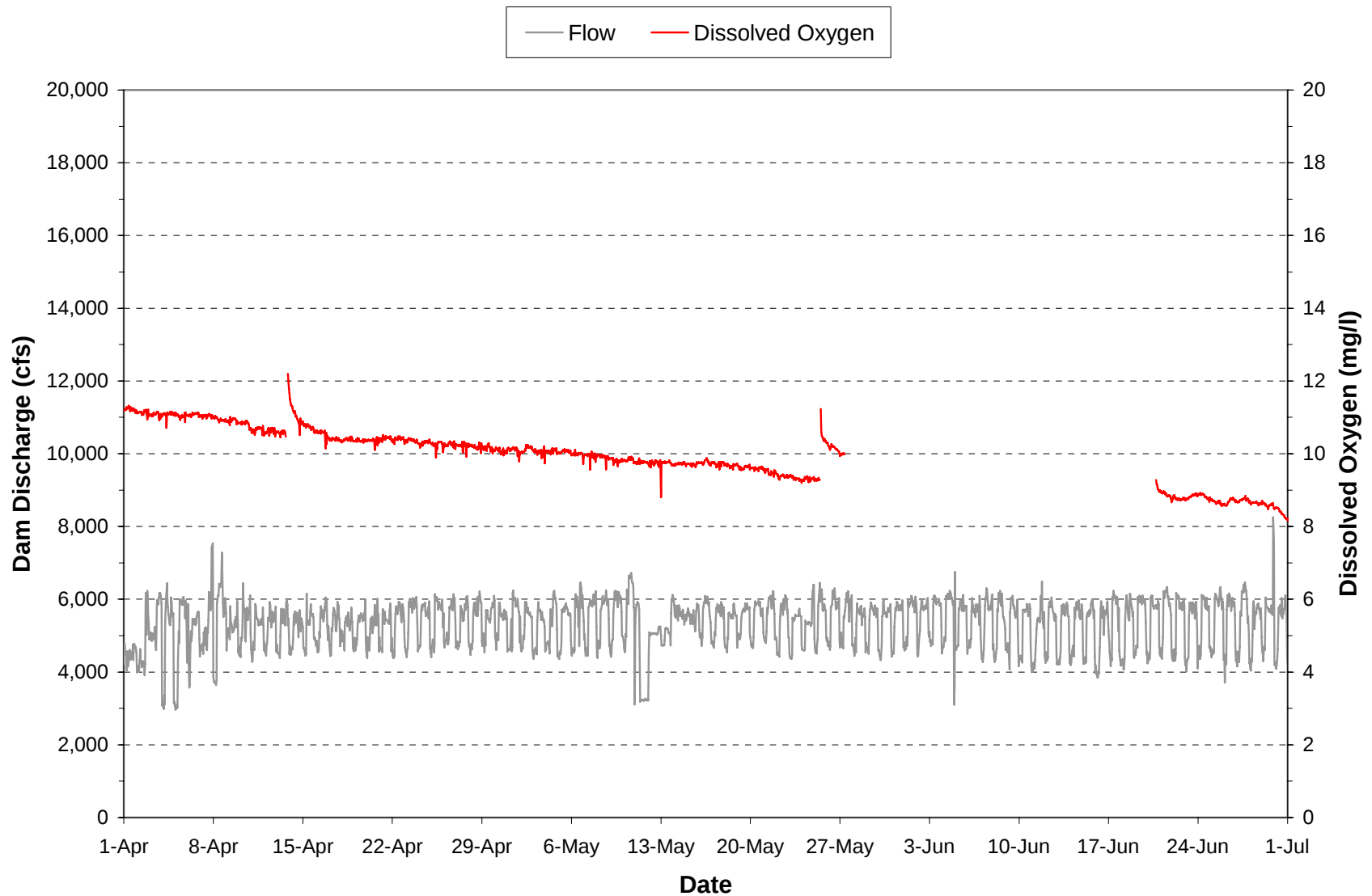
Plate 68. Hourly discharge and dissolved oxygen concentrations monitored in the “raw water supply line” at the Fort Peck powerhouse during the period April through June 2005. (Note: Gaps in dissolved oxygen plot are periods when the monitoring equipment was not operational.)
