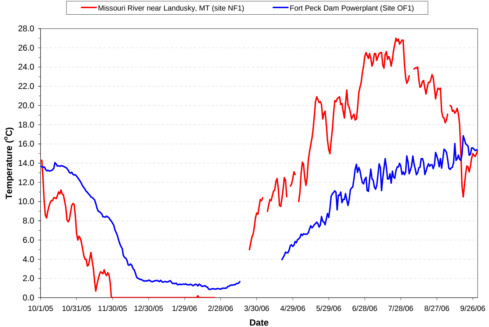
Figure 7.2. Mean daily water temperatures monitored at the Fort Peck powerplant and the Missouri near Landusky, Montana from October 2005 through September 2006. (Note: Gaps in temperature plots are periods when monitoring equipment was not operational.)
