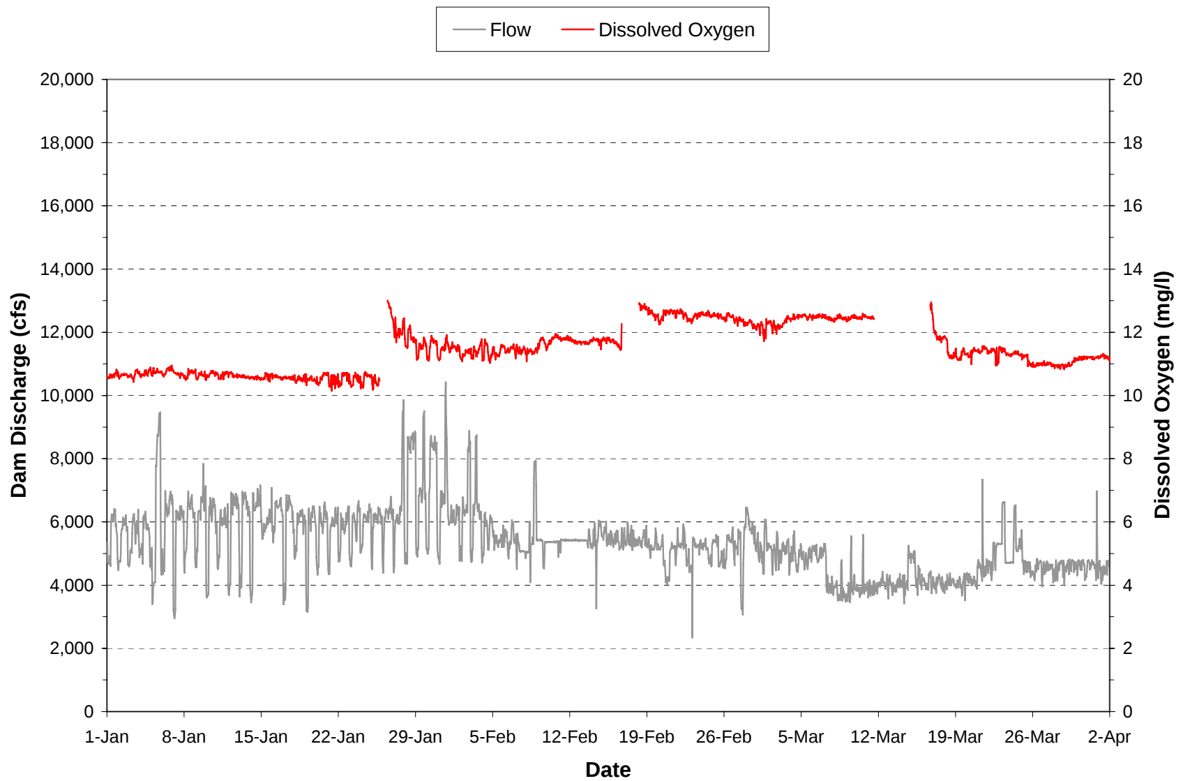
Plate 67. Hourly discharge and dissolved oxygen concentrations monitored in the “raw water supply line” at the Fort Peck powerhouse during the period January through March 2005. (Note: Gaps in dissolved oxygen plot are periods when the monitoring equipment was not operational.)
