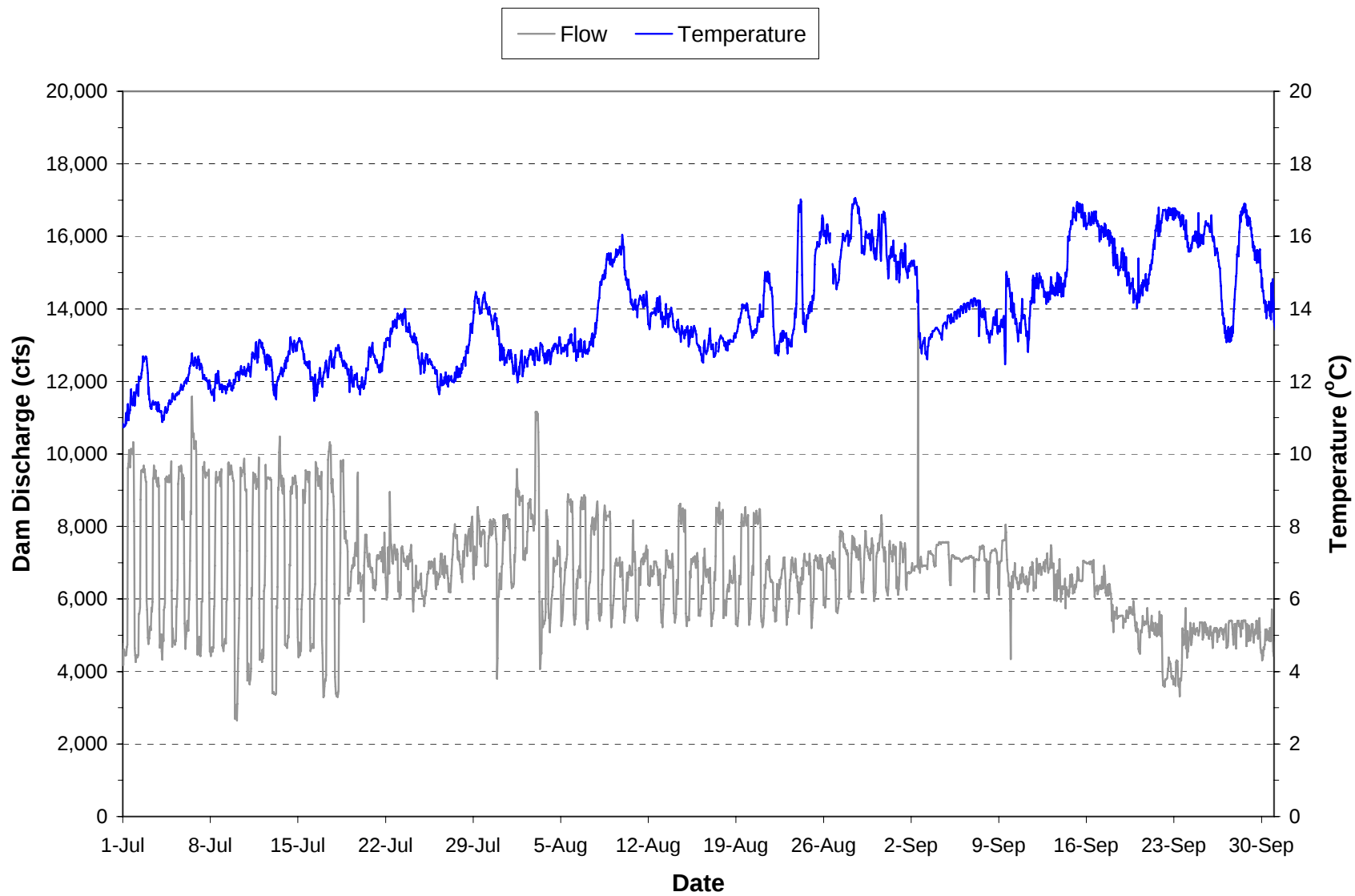
Plate 53. Hourly discharge and water temperature monitored in the “raw water supply line” at the Fort Peck powerhouse during the period July through September 2004.
