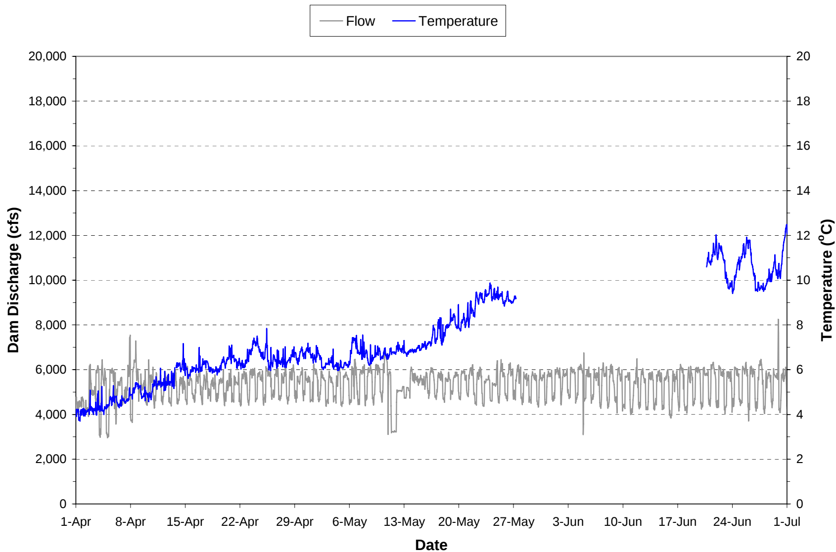
Plate 56. Hourly discharge and water temperature monitored in the “raw water supply line” at the Fort Peck powerhouse during the period April through June 2005. (Note: Gaps in temperature plot are periods when the monitoring equipment was not operational.)
