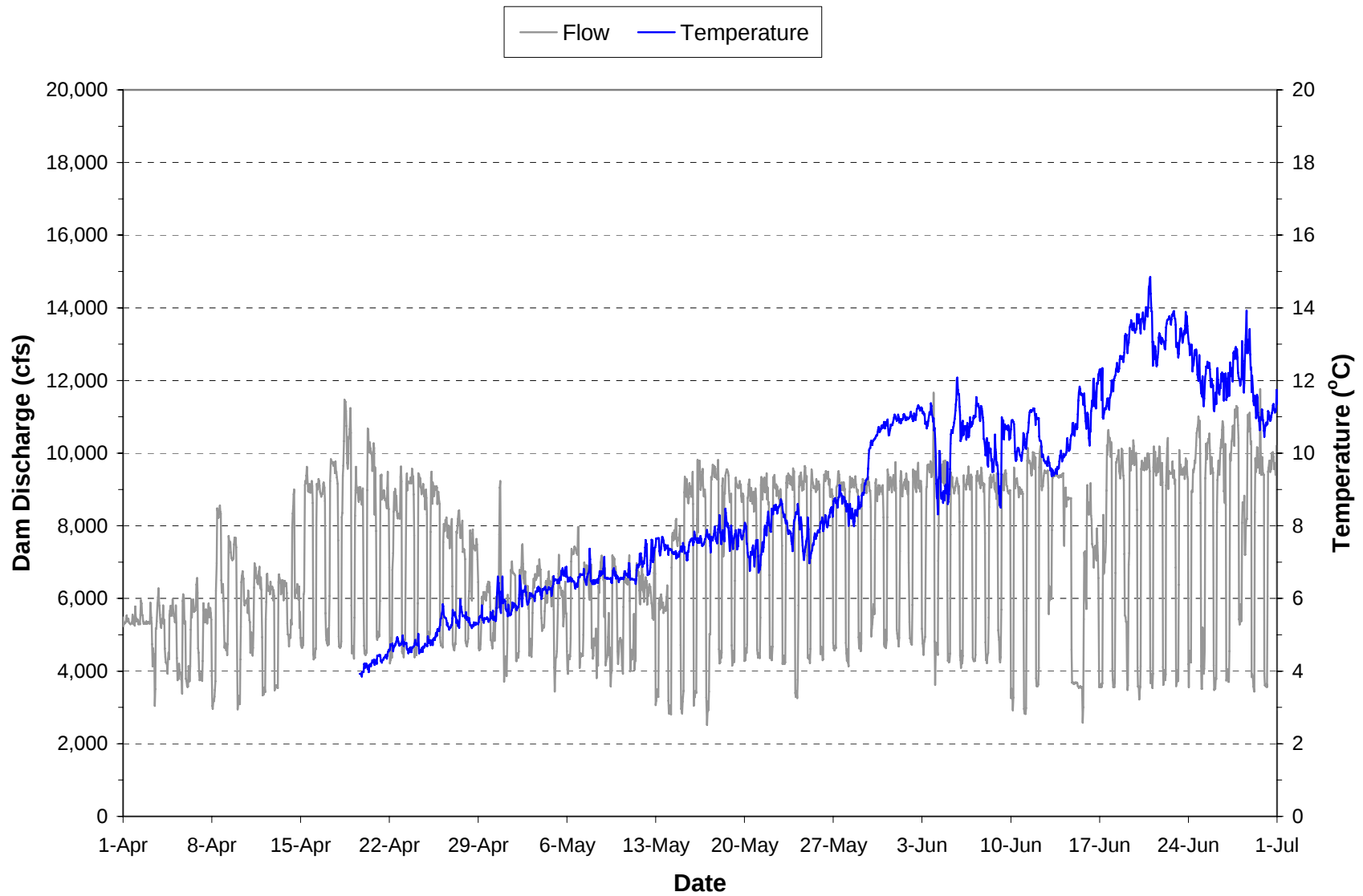
Plate 60. Hourly discharge and water temperature monitored in the “raw water supply line” at the Fort Peck powerhouse during the period April through June 2006. (Note: Gaps in temperature plot are periods when the monitoring equipment was not operational.)
