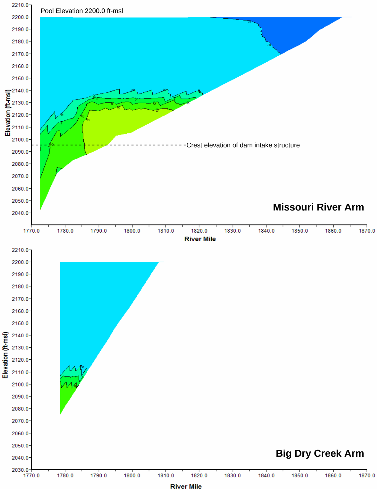
Plate 16. Longitudinal dissolved oxygen contour plot of Fort Peck Reservoir based on depth-profile dissolved oxygen concentrations monitored at sites L1, L2, L3, L5, L6, and NF1 on September 22, 2004.
