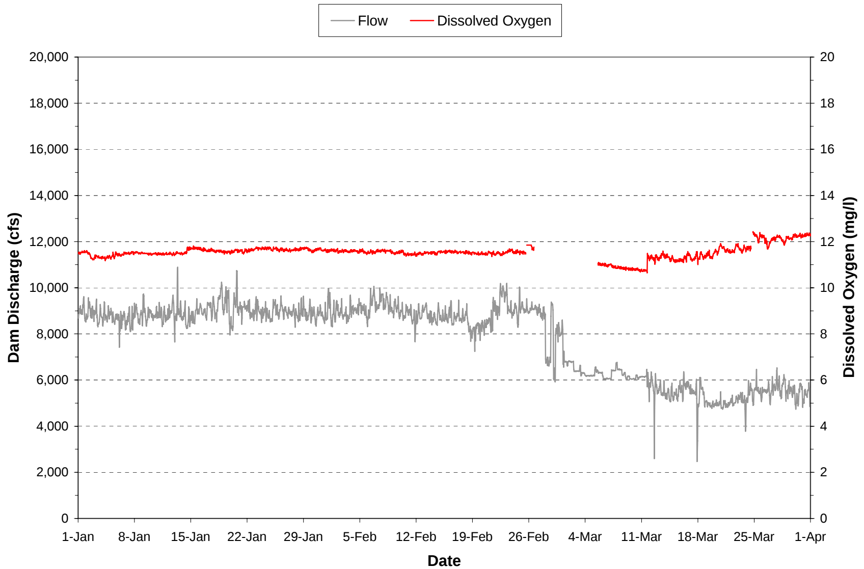
Plate 63. Hourly discharge and dissolved oxygen concentrations monitored in the “raw water supply line” at the Fort Peck powerhouse during the period January through March 2004. (Note: Gaps in dissolved oxygen plot are periods when the monitoring equipment was not operational.)
