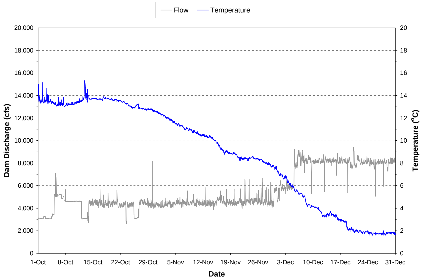
Plate 58. Hourly discharge and water temperature monitored in the “raw water supply line” at the Fort Peck powerhouse during the period October through December 2005.
