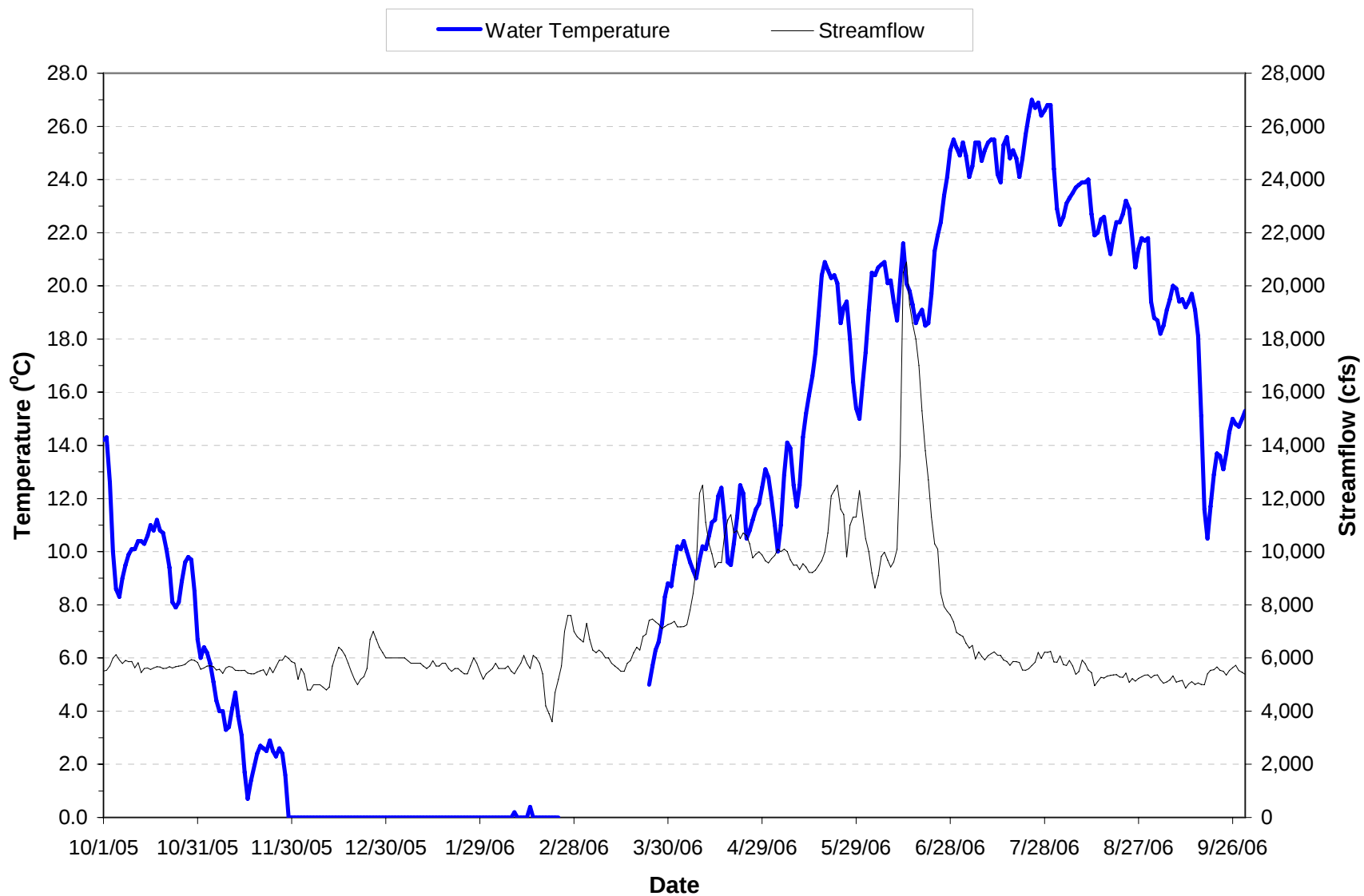
Figure 6.2. Mean daily water temperature and streamflow of the Missouri River at inflow site NF1 for water year 2006 (i.e., October 2005 through September 2006). Means based on hourly measurements recorded at USGS gaging station 06115200. (Gaps in plot indicate missing data).
