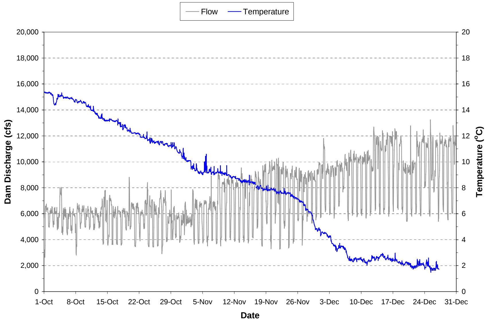
Plate 62. Hourly discharge and water temperature monitored in the “raw water supply line” at the Fort Peck powerhouse during the period October through December 2006. (Note: Gaps in temperature plot are periods when the monitoring equipment was not operational.)
