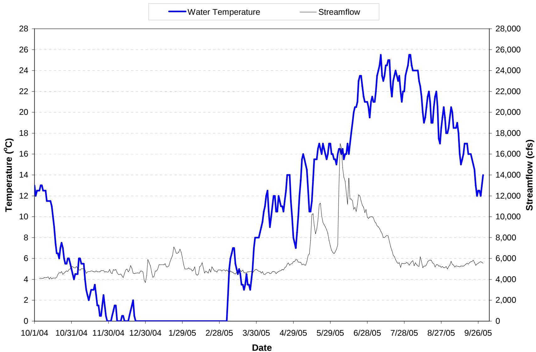
Figure 6.1. Mean daily water temperature and streamflow of the Missouri River at inflow site NF1 for water year 2005 (i.e., October 2004 through September 2005). Means based on hourly measurements recorded at USGS gaging station 06115200.
