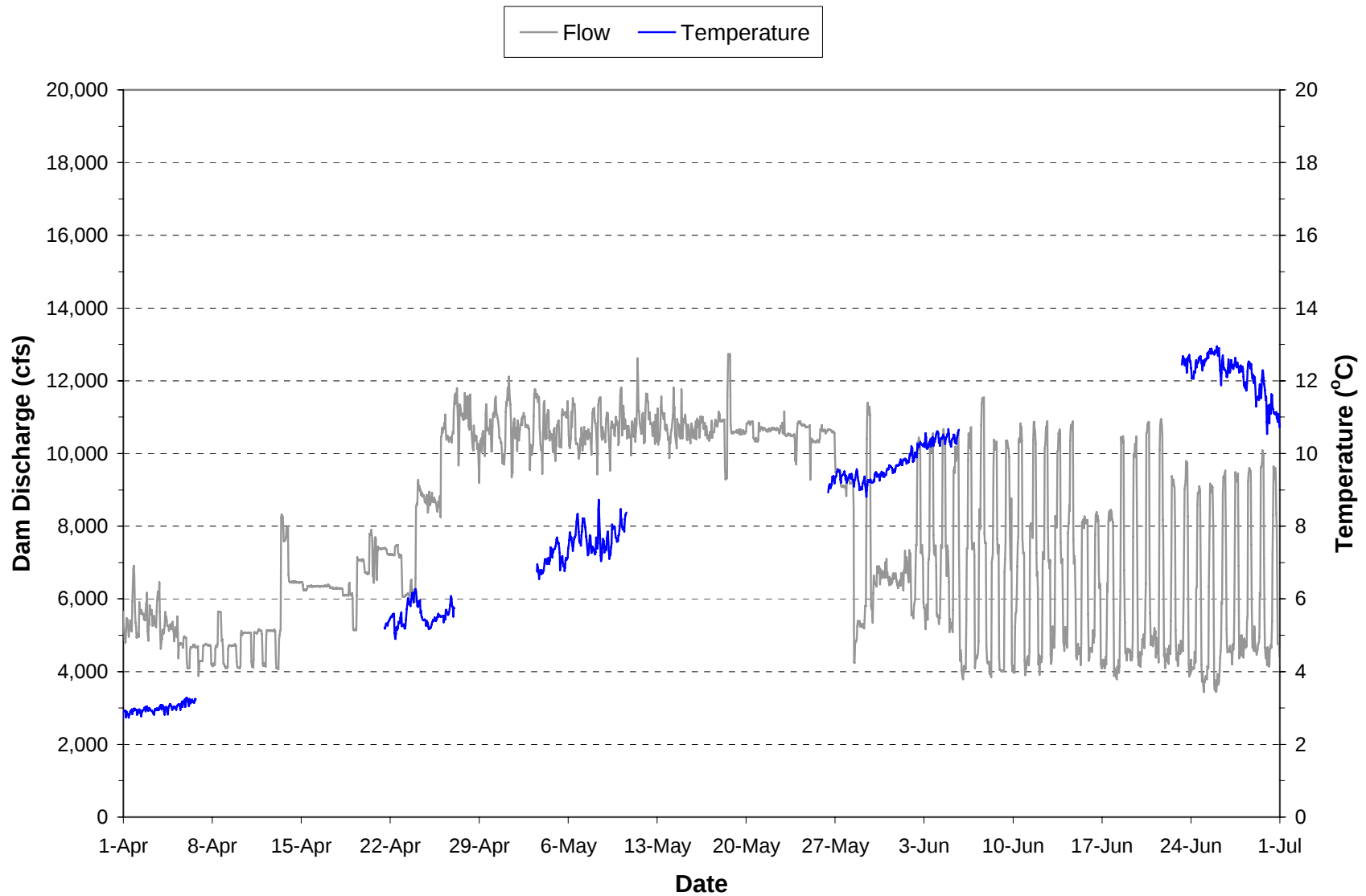
Plate 52. Hourly discharge and water temperature monitored in the “raw water supply line” at the Fort Peck powerhouse during the period April through June 2004. (Note: Gaps in temperature plot are periods when the monitoring equipment was not operational.)
