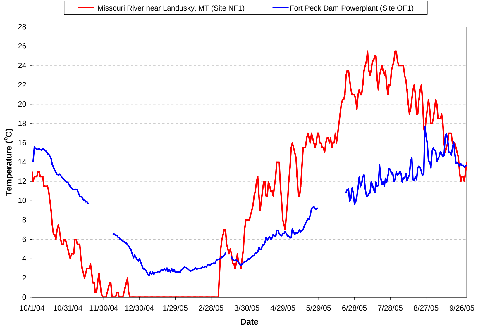
Figure 7.1. Mean daily water temperatures monitored at the Fort Peck powerplant and the Missouri near Landusky, Montana from October 2004 through September 2005. (Note: Gaps in temperature plots are periods when monitoring equipment was not operational.)
