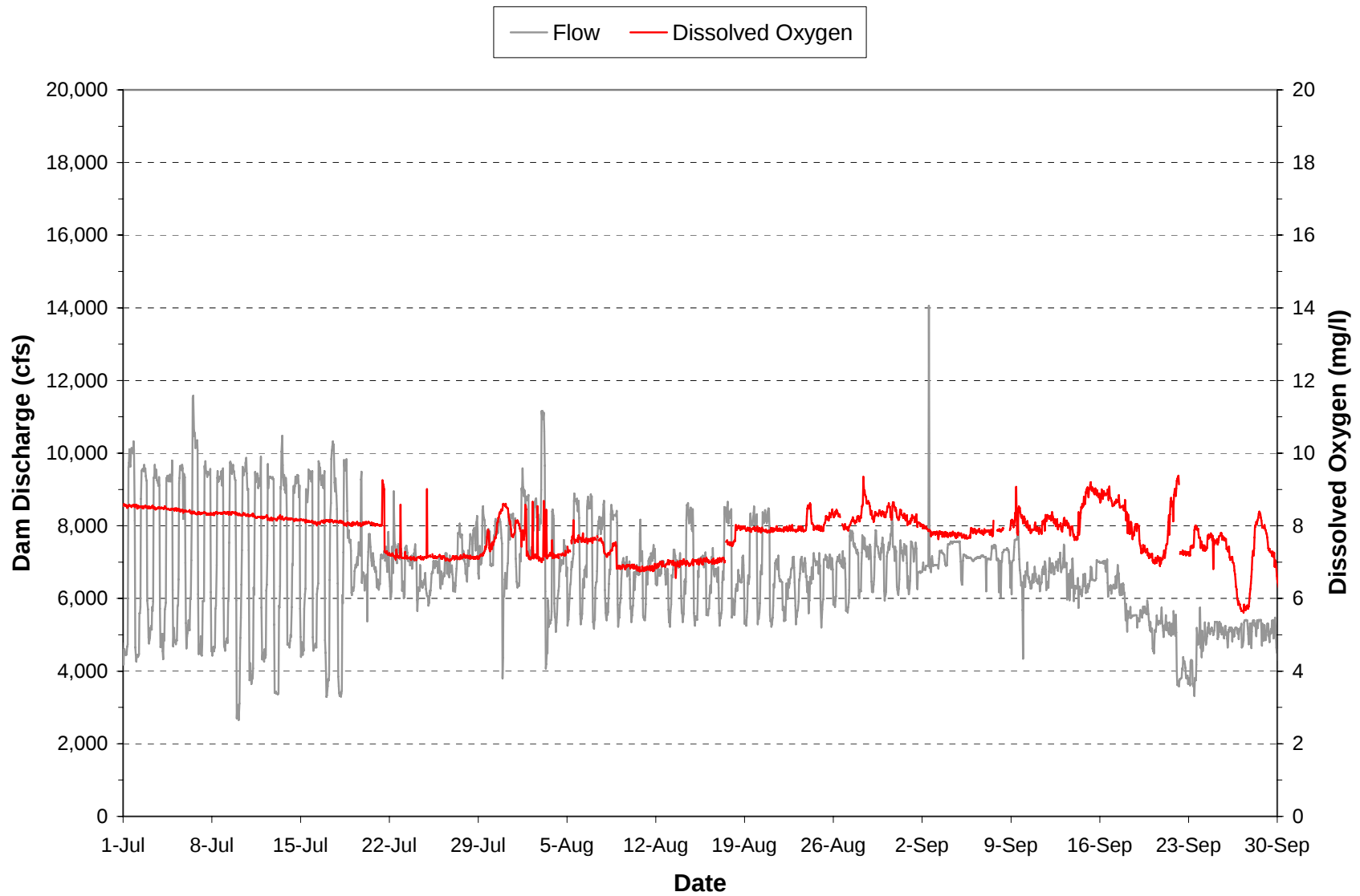
Plate 65. Hourly discharge and dissolved oxygen concentrations monitored in the “raw water supply line” at the Fort Peck powerhouse during the period July through September 2004. (Note: Gaps in dissolved oxygen plot are periods when the monitoring equipment was not operational.)
