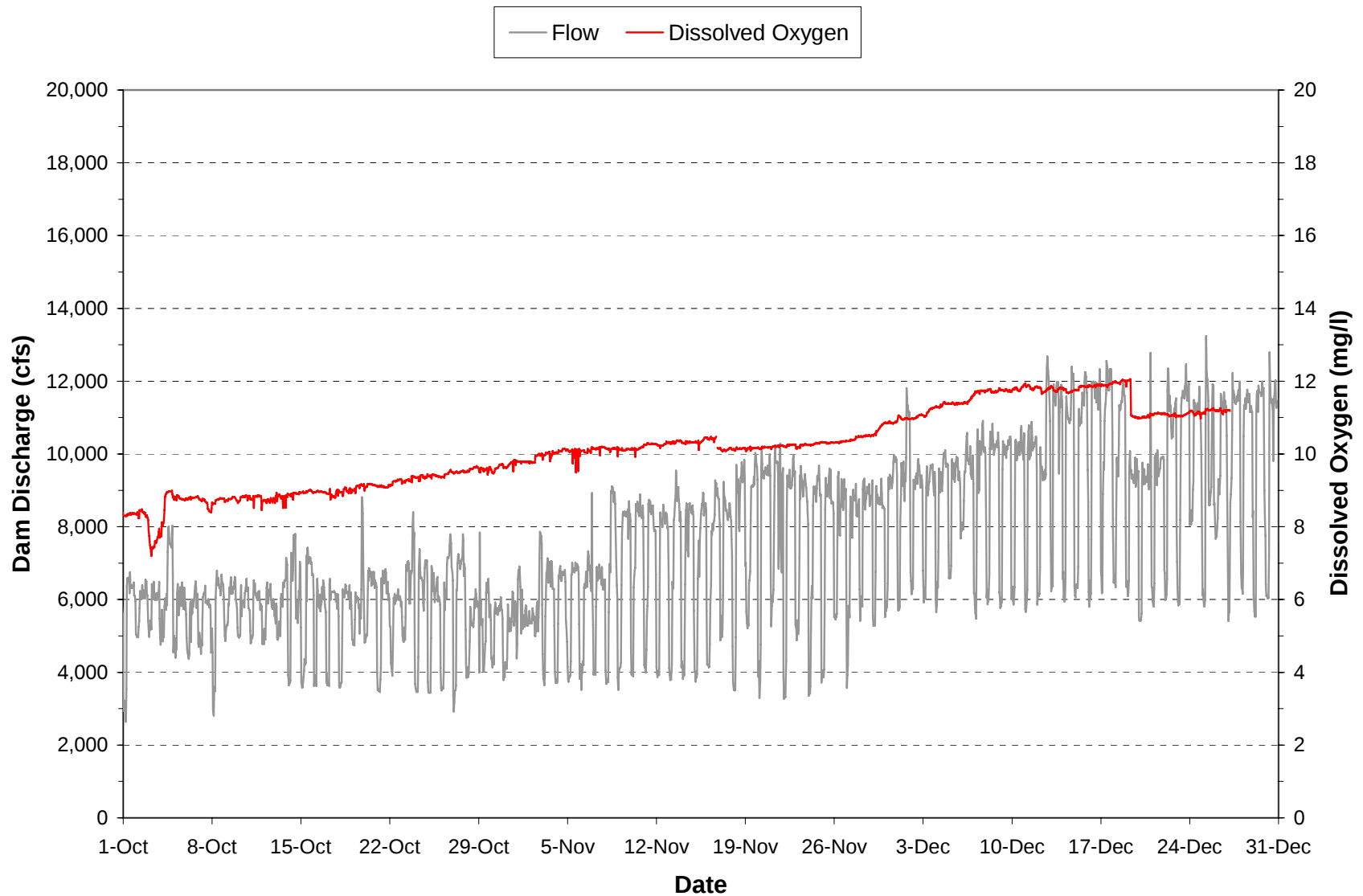
Plate 74. Hourly discharge and dissolved oxygen concentrations monitored in the “raw water supply line” at the Fort Peck powerhouse during the period October through December 2006. (Note: Gaps in dissolved oxygen plot are periods when the monitoring equipment was not operational.)
