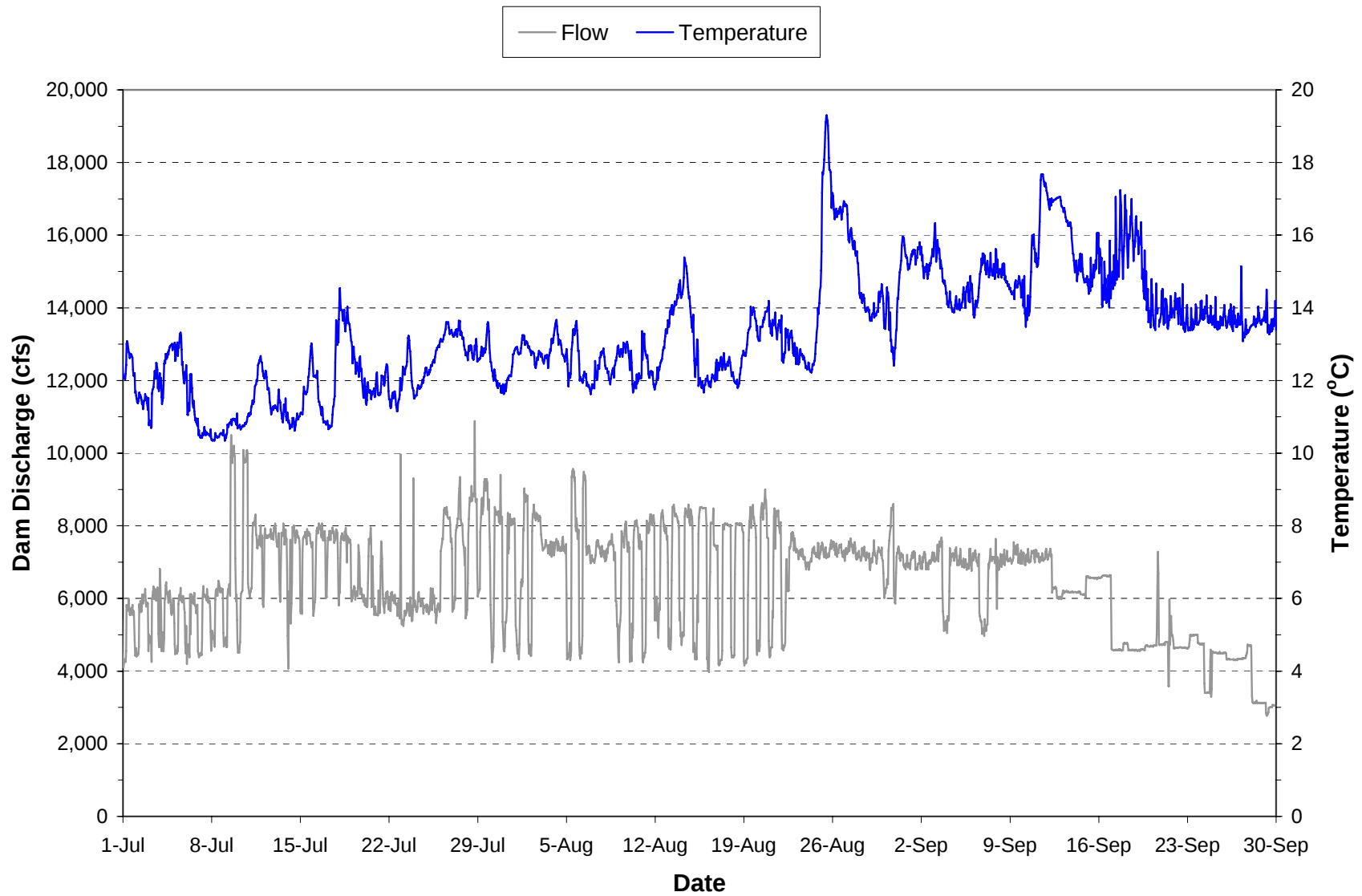
Plate 57. Hourly discharge and water temperature monitored in the “raw water supply line” at the Fort Peck powerhouse during the period July through September 2005.
