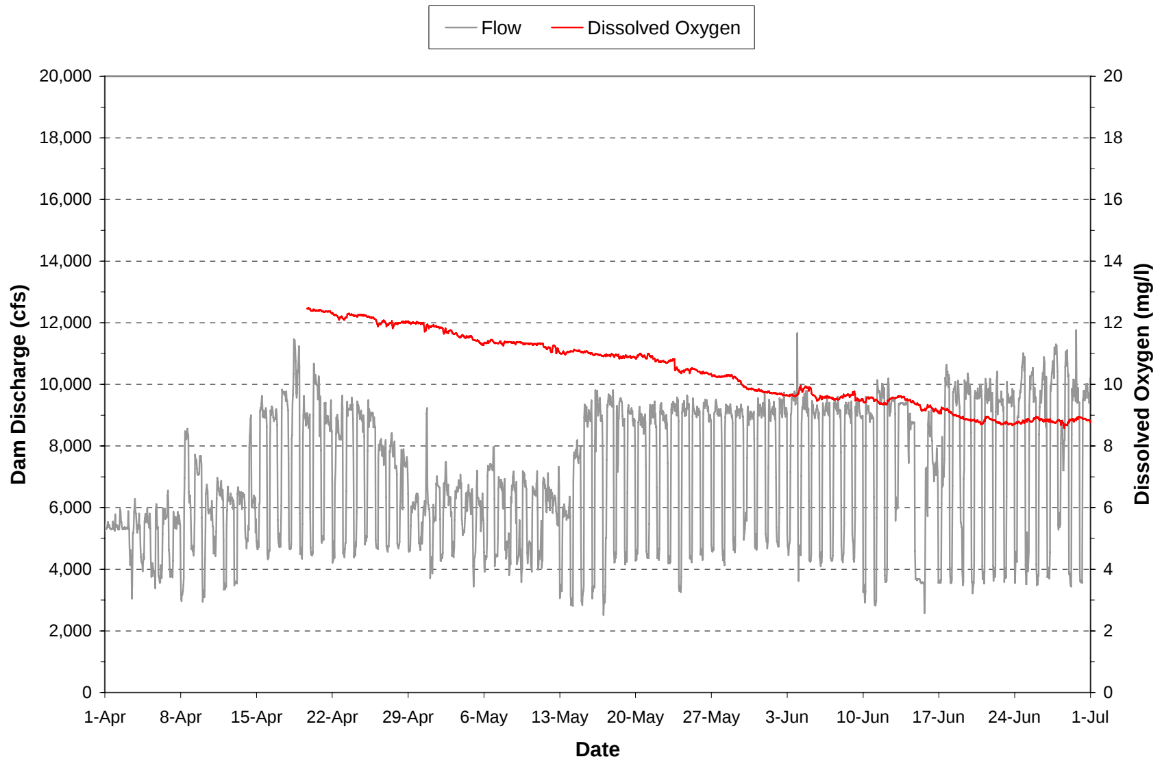
Plate 72. Hourly discharge and dissolved oxygen concentrations monitored in the “raw water supply line” at the Fort Peck powerhouse during the period April through June 2006. (Note: Gaps in dissolved oxygen plot are periods when the monitoring equipment was not operational.)
