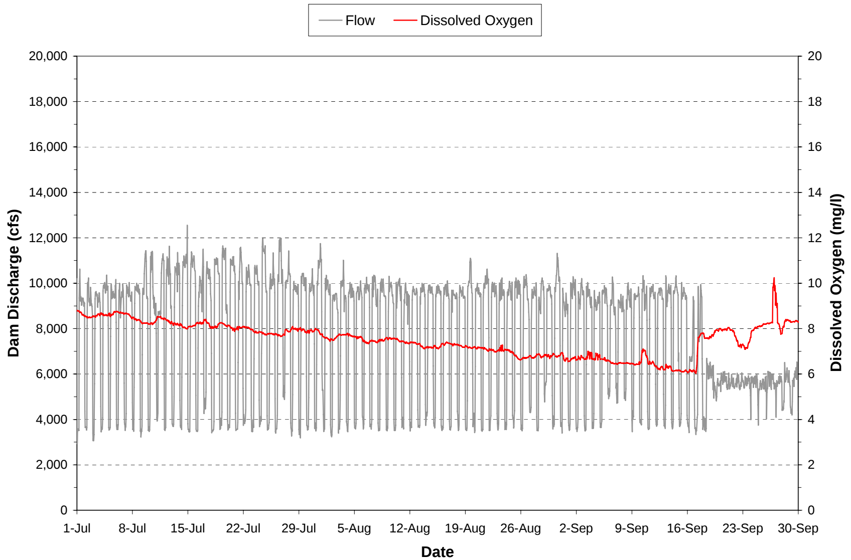
Plate 73. Hourly discharge and dissolved oxygen concentrations monitored in the “raw water supply line” at the Fort Peck powerhouse during the period July through September 2006.
