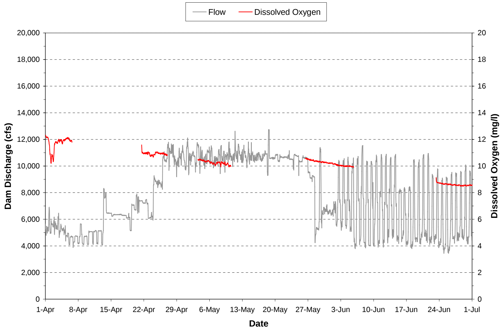
Plate 64. Hourly discharge and dissolved oxygen concentrations monitored in the “raw water supply line” at the Fort Peck powerhouse during the period April through June 2004. (Note: Gaps in dissolved oxygen plot are periods when the monitoring equipment was not operational.)
