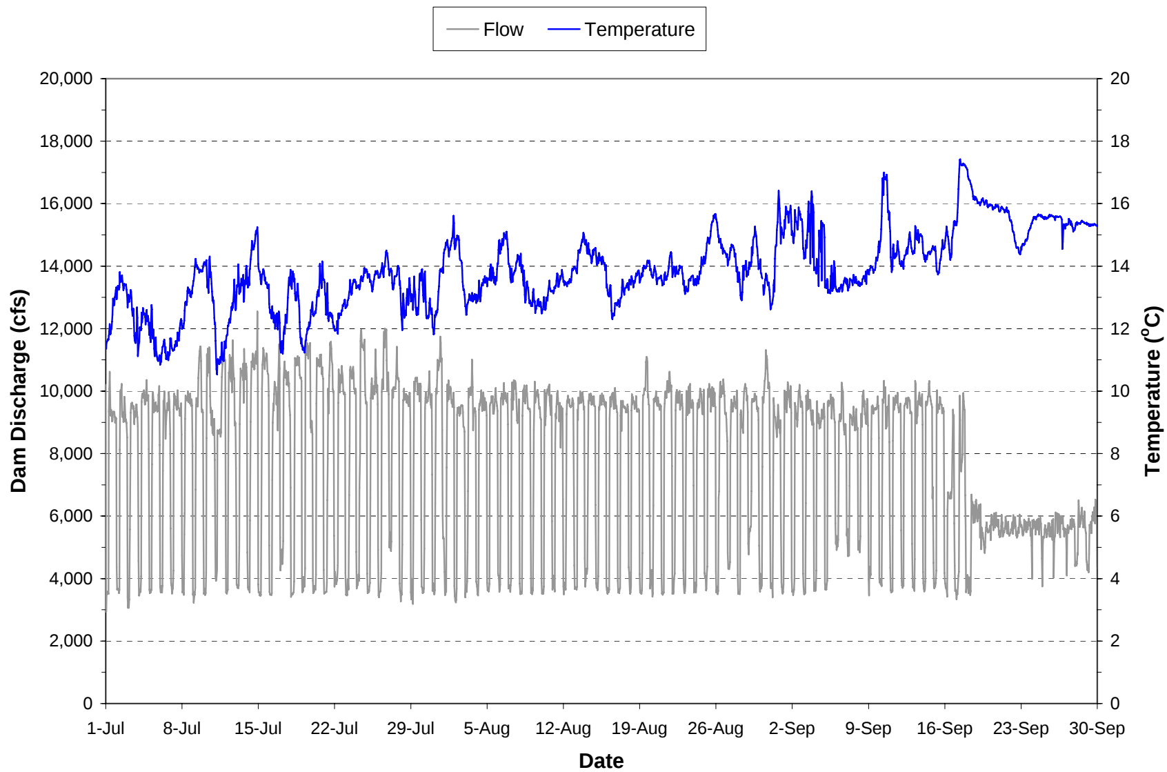
Plate 61. Hourly discharge and water temperature monitored in the “raw water supply line” at the Fort Peck powerhouse during the period July through September 2006.
