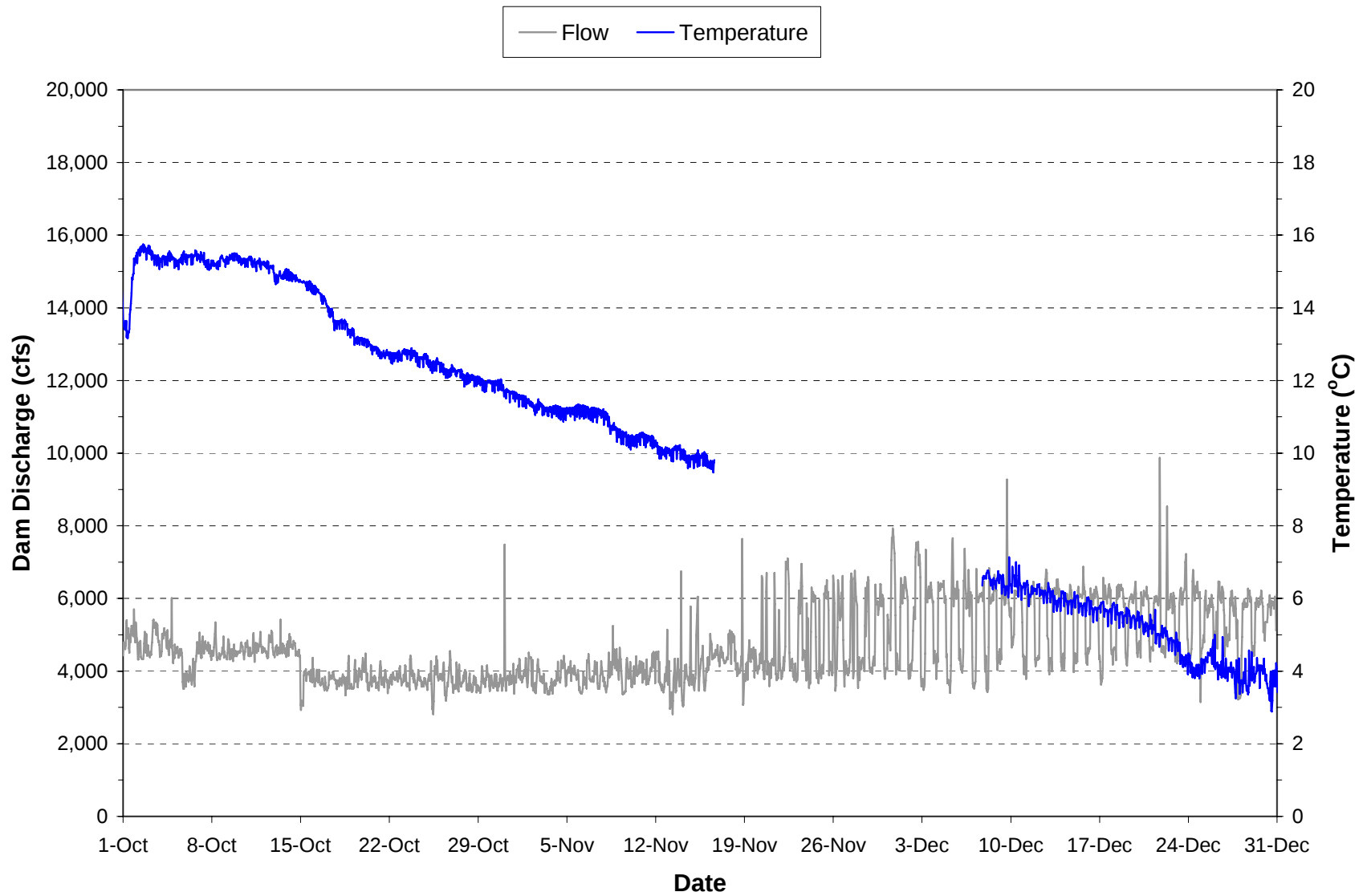
Plate 54. Hourly discharge and water temperature monitored in the “raw water supply line” at the Fort Peck powerhouse during the period October through December 2004. (Note: Gaps in temperature plot are periods when the monitoring equipment was not operational.)
