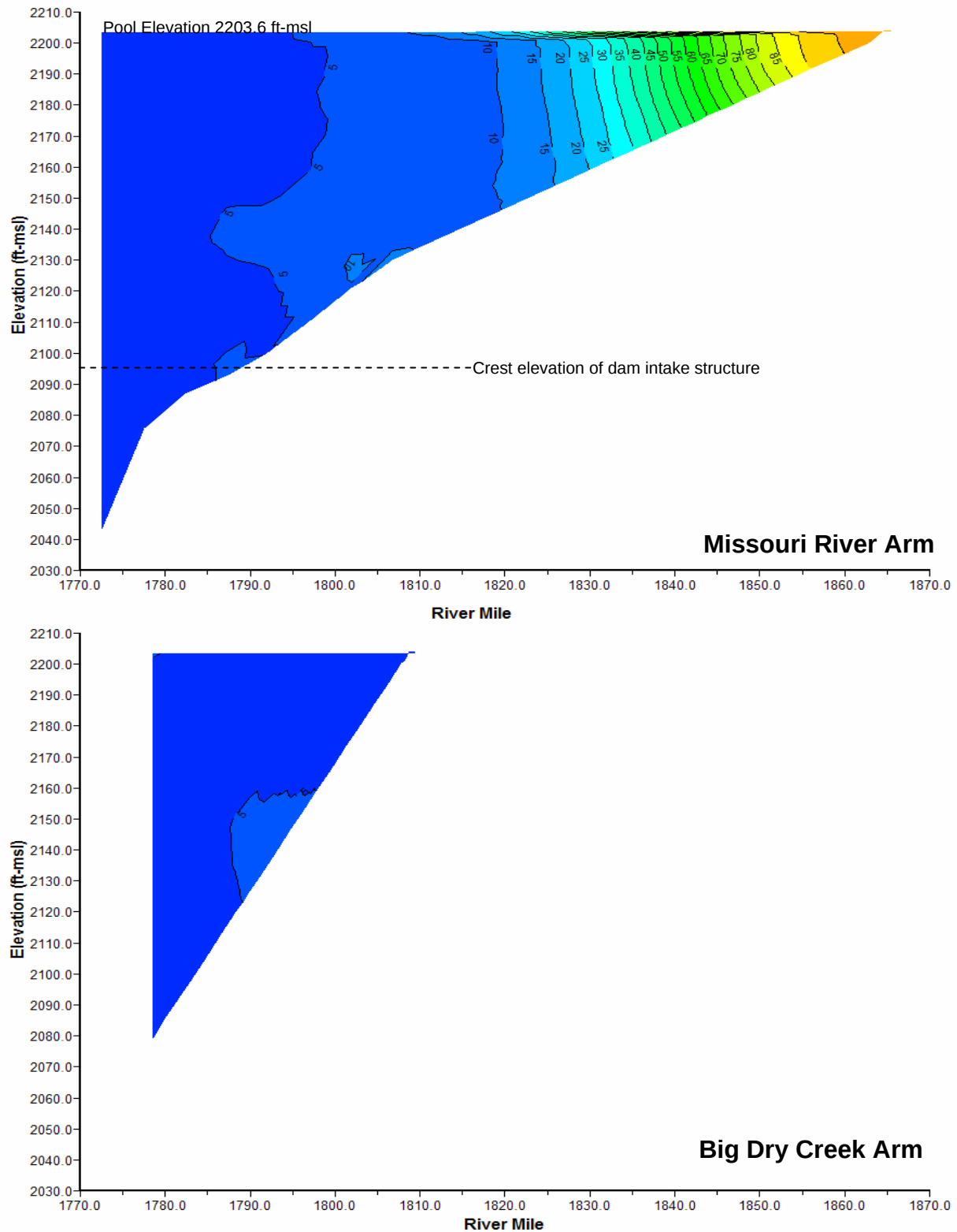
Plate 25. Longitudinal turbidity contour plot of Fort Peck Reservoir based on depth-profile turbidity levels monitored at sites L1, L2, L3,L4, L5, L6, and NF1 on June 23, 2004.
