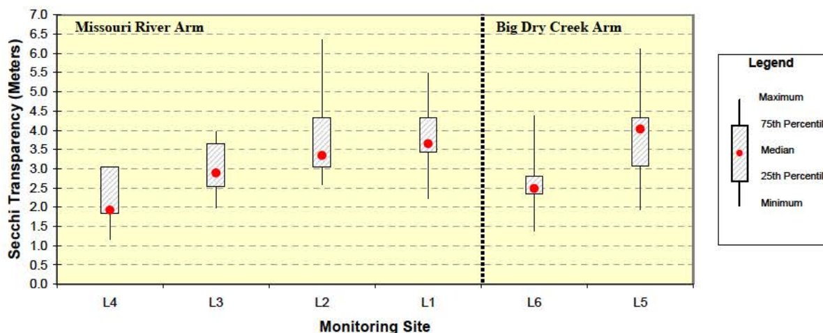
Figure 5.1. Box plot of Secchi transparencies measured at sites L1 through L6 during the period 2004 through 2006. (Note: monitoring sites are oriented on the x-axis in an upstream to downstream direction for both arms of the reservoir.)
