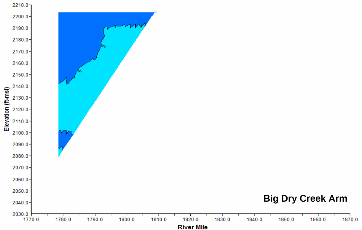
Plate 13. Longitudinal dissolved oxygen contour plot of Fort Peck Reservoir based on depth-profile dissolved oxygen concentrations monitored at sites L1, L2, L3, L4, L5, L6, and NF1 on June 23, 2004.
