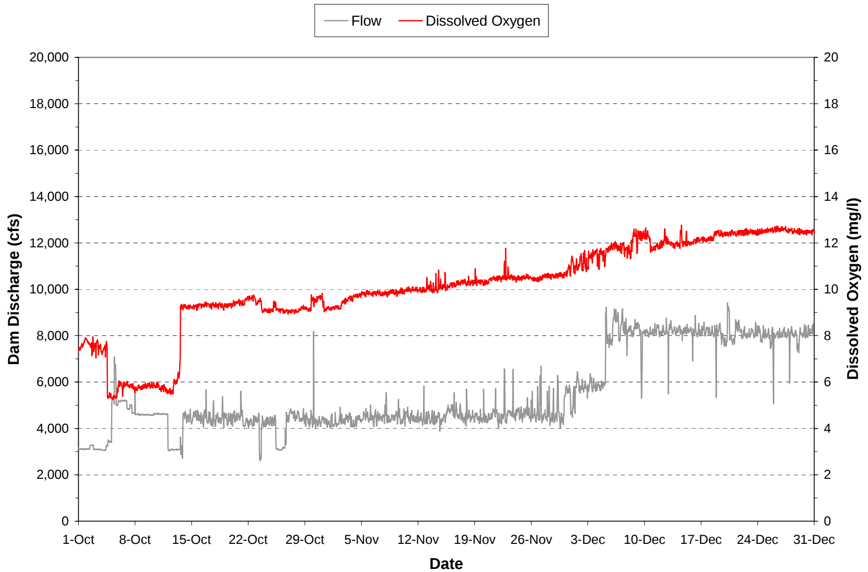
Plate 70. Hourly discharge and dissolved oxygen concentrations monitored in the “raw water supply line” at the Fort Peck powerhouse during the period October through December 2005.
