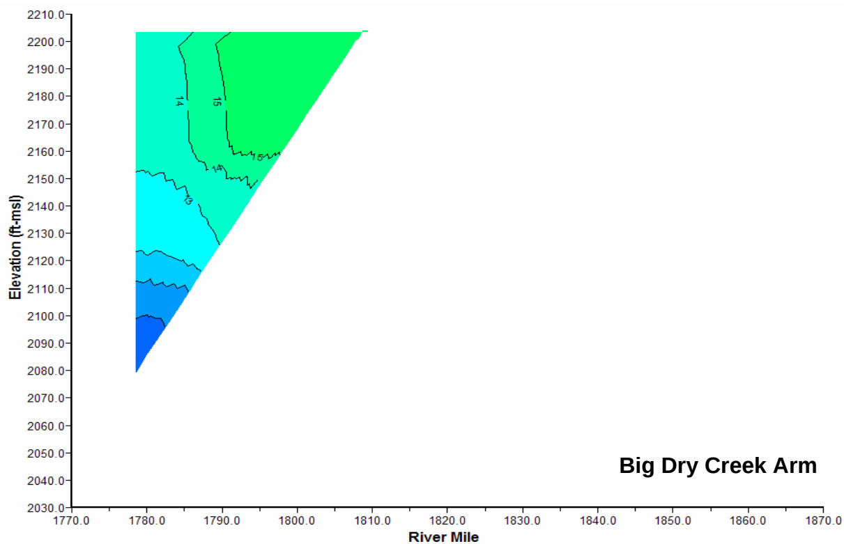
Plate 1. Longitudinal water temperature contour plot of Fort Peck Reservoir based on depth-profile water temperatures monitored at sites L1, L2, L3, L4, L5, L6, and NF1 on June 23, 2004.
