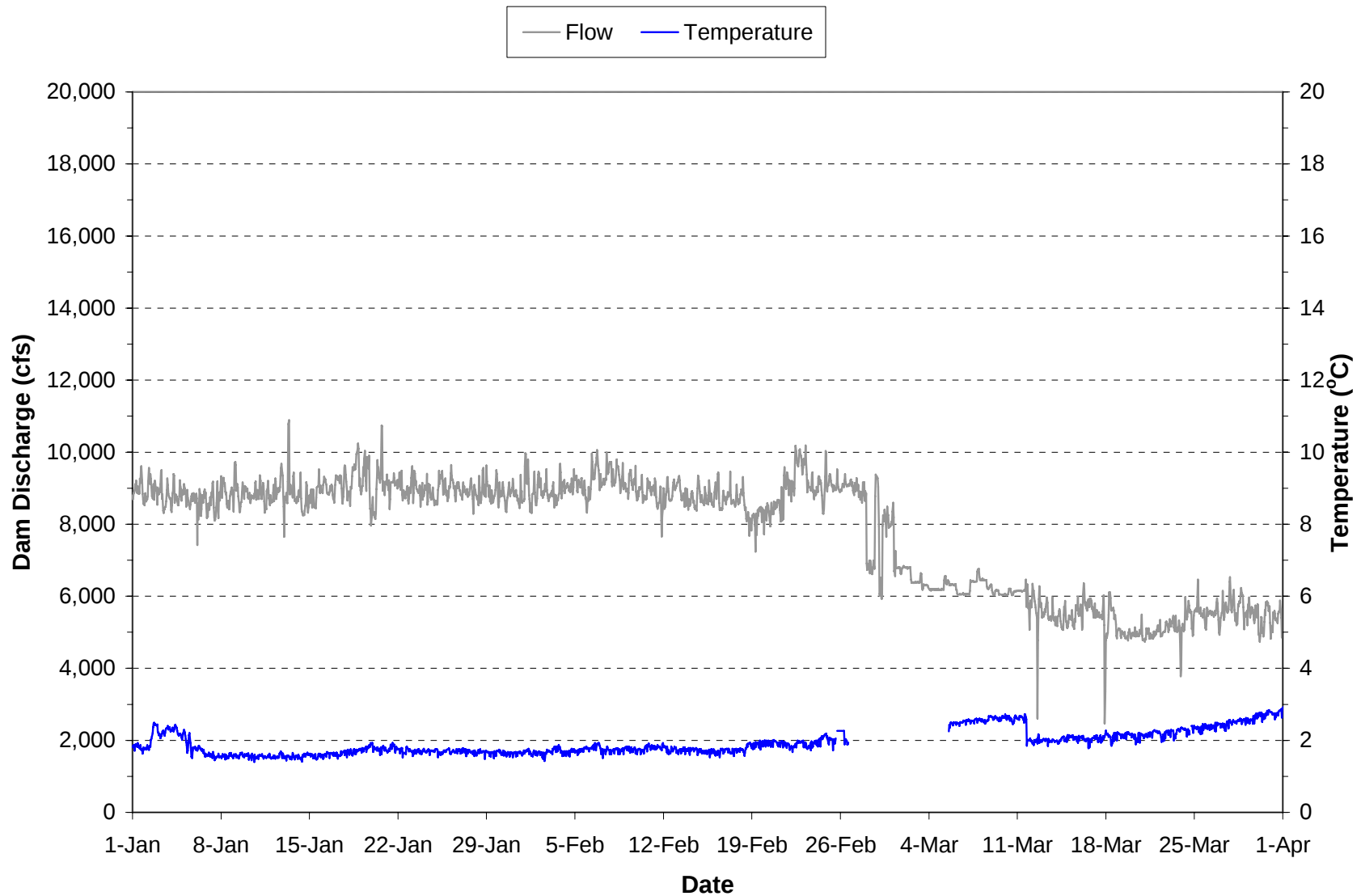
Plate 51. Hourly discharge and water temperature monitored in the “raw water supply line” at the Fort Peck powerhouse during the period January through March 2004. (Note: Gaps in temperature plot are periods when the monitoring equipment was not operational.)
