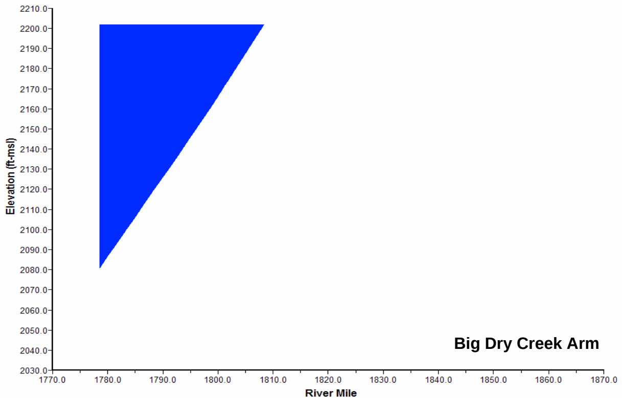
Plate 36. Longitudinal turbidity contour plot of Fort Peck Reservoir based on depth-profile turbidity levels monitored at sites L1, L2, L3, L4, L5, L6, and NF1 on October 5, 2006.
