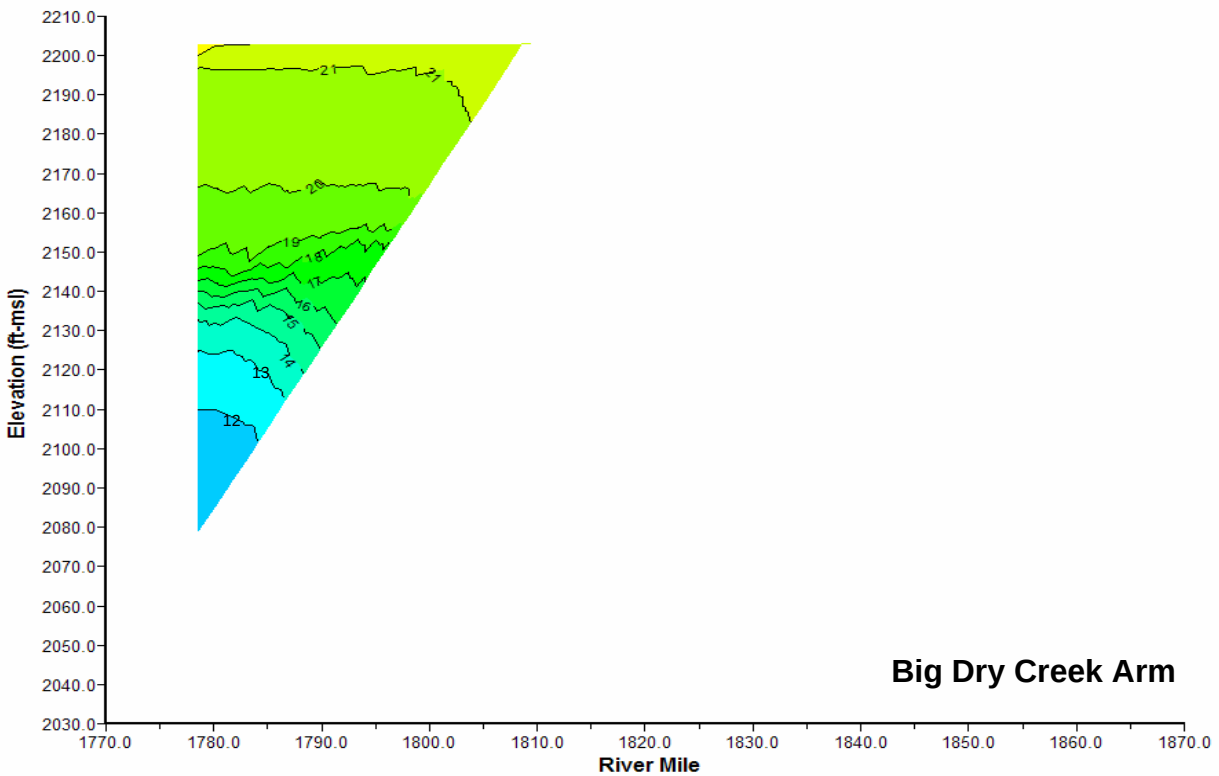
Plate 7. Longitudinal water temperature contour plot of Fort Peck Reservoir based on depth-profile water temperatures monitored at sites L1, L2, L3, L4, L5, L6, and NF1 on August 22, 2005.
