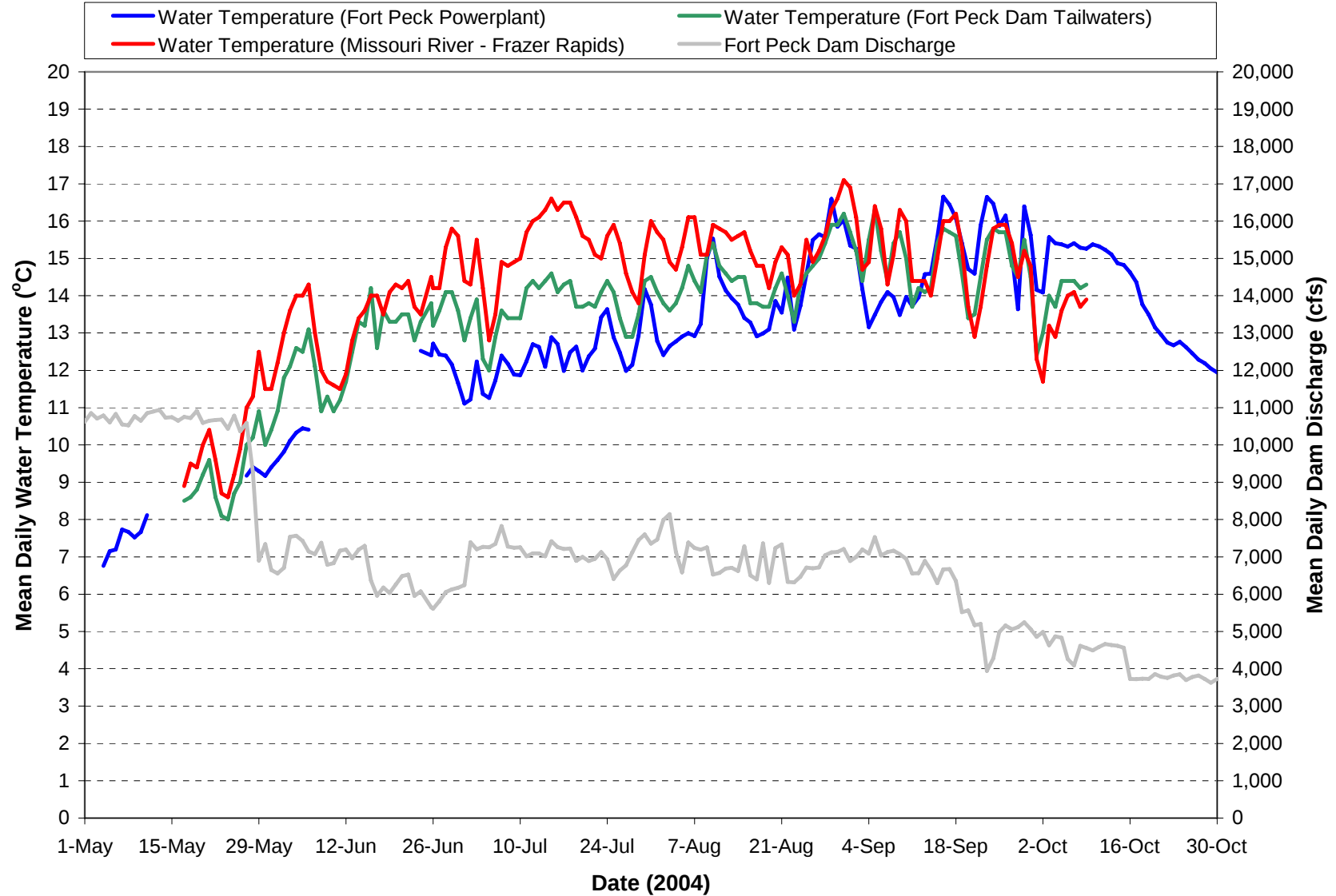
Figure 7.3. Mean daily water temperatures monitored at the Fort Peck powerplant, Missouri River tailwaters, and Missouri River Frazer Rapids and the mean daily discharge of Fort Peck Dam from May through October during 2004.
