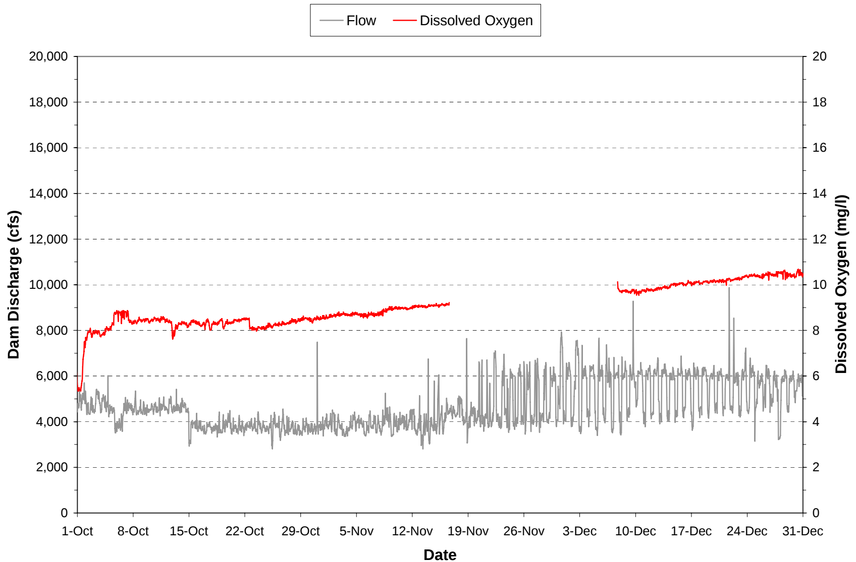
Plate 66. Hourly discharge and dissolved oxygen concentrations monitored in the “raw water supply line” at the Fort Peck powerhouse during the period October through December 2004. (Note: Gaps in dissolved oxygen plot are periods when the monitoring equipment was not operational.)
