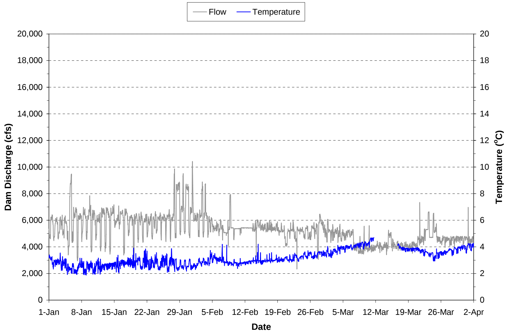
Plate 55. Hourly discharge and water temperature monitored in the “raw water supply line” at the Fort Peck powerhouse during the period January through March 2005. (Note: Gaps in temperature plot are periods when the monitoring equipment was not operational.)
