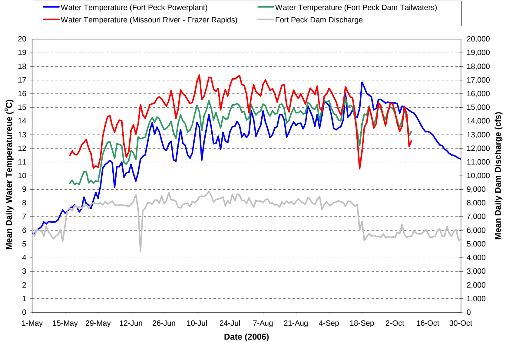
Figure 7.5. Mean daily water temperatures monitored at the Fort Peck powerplant, Missouri River tailwaters, and Missouri River Frazer Rapids and the mean daily discharge of Fort Peck Dam from May through October during 2006.
