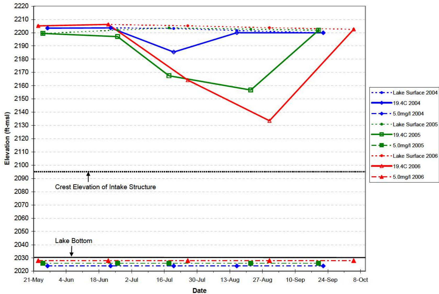
Figure 5.2. Elevation of reservoir surface and 19.4°C water temperature and 5 mg/l dissolved oxygen concentration isopleths by year for station L1.
