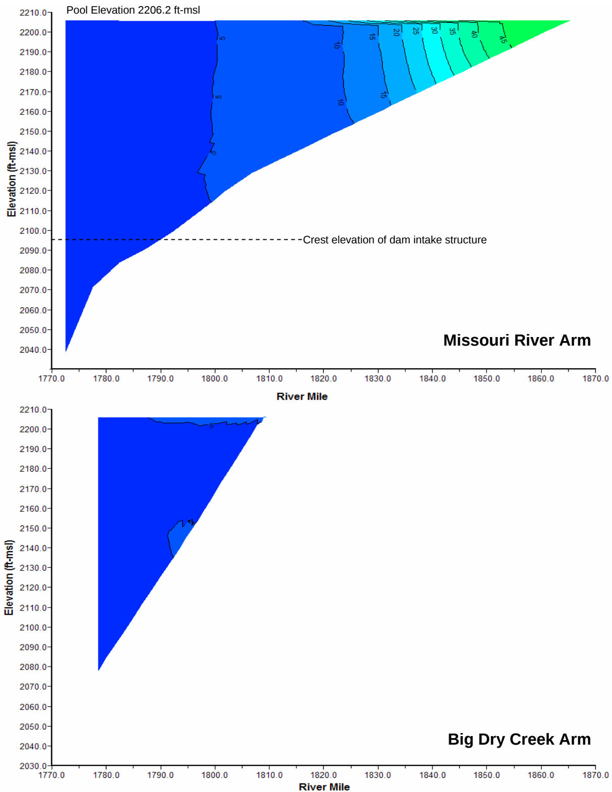
Plate 33. Longitudinal turbidity contour plot of Fort Peck Reservoir based on depth-profile turbidity levels monitored at sites L1, L2, L3, L4, L5, L6, and NF1 on June 22, 2006.
