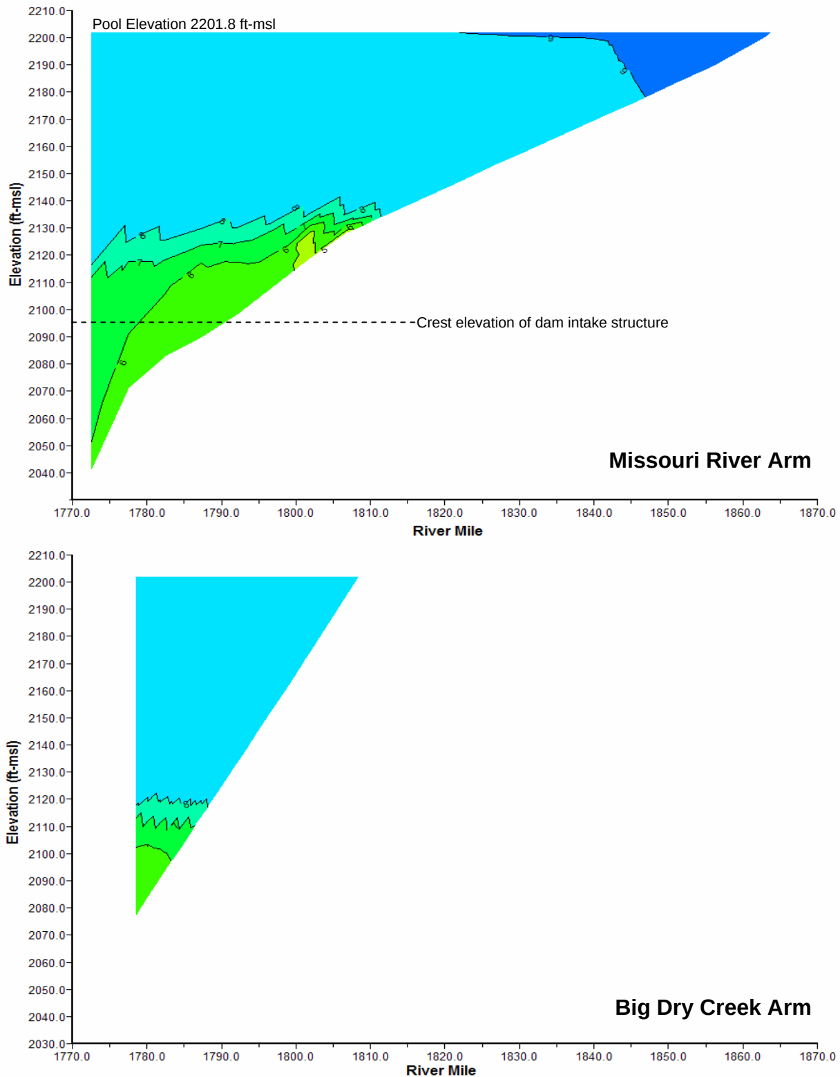
Plate 20. Longitudinal dissolved oxygen contour plot of Fort Peck Reservoir based on depth-profile dissolved oxygen concentrations monitored at sites L1, L2, L3, L4, L5, L6, and NF1 on September 20, 2005.
