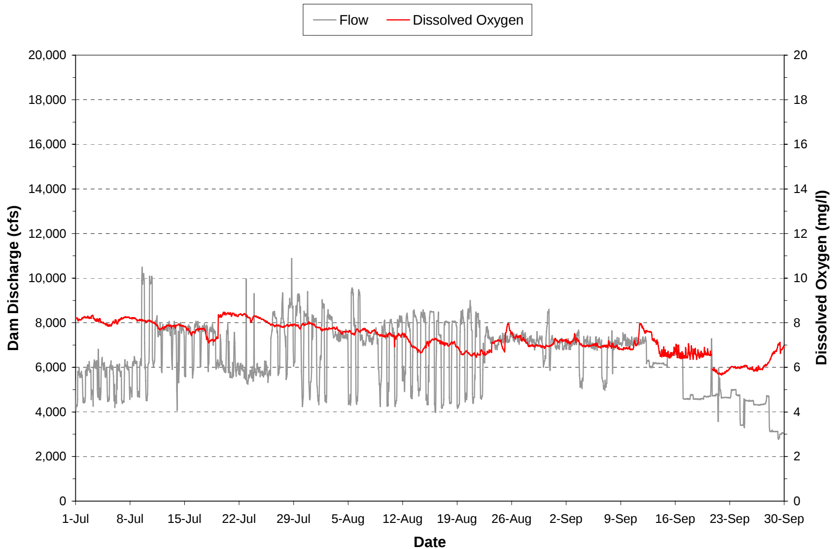
Plate 69. Hourly discharge and dissolved oxygen concentrations monitored in the “raw water supply line” at the Fort Peck powerhouse during the period July through September 2005. (Note: Gaps in dissolved oxygen plot are periods when the monitoring equipment was not operational.)
