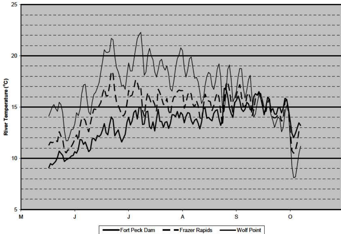
Figure 10. 2005 USGS measured temperature increases in the Missouri River from Fort Peck Dam to Wolf Point.
