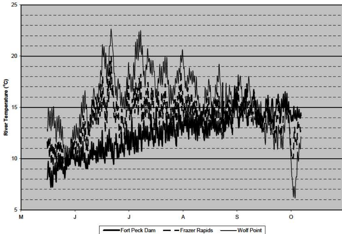
Figure 11. 2005 simulated temperature increases in the Missouri River from Fort Peck Dam to Wolf Point.
