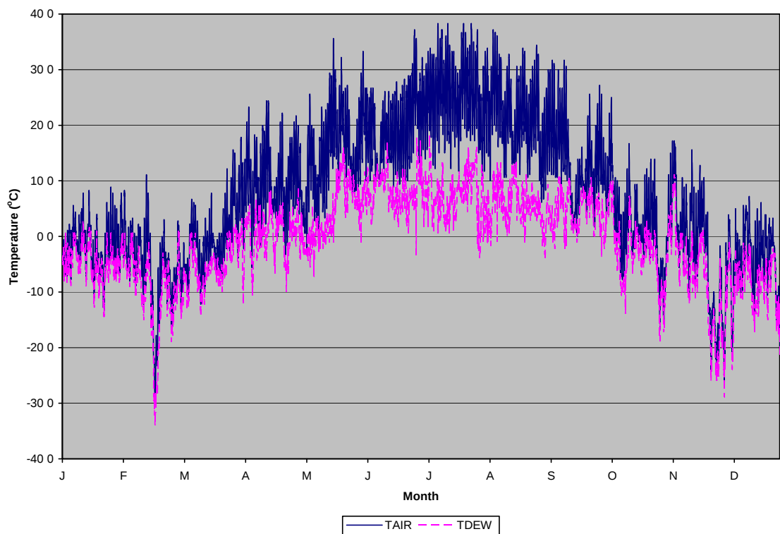
Plate 5. 2006 Glasgow International Airport (KGGW) hourly air and dew point temperature.
