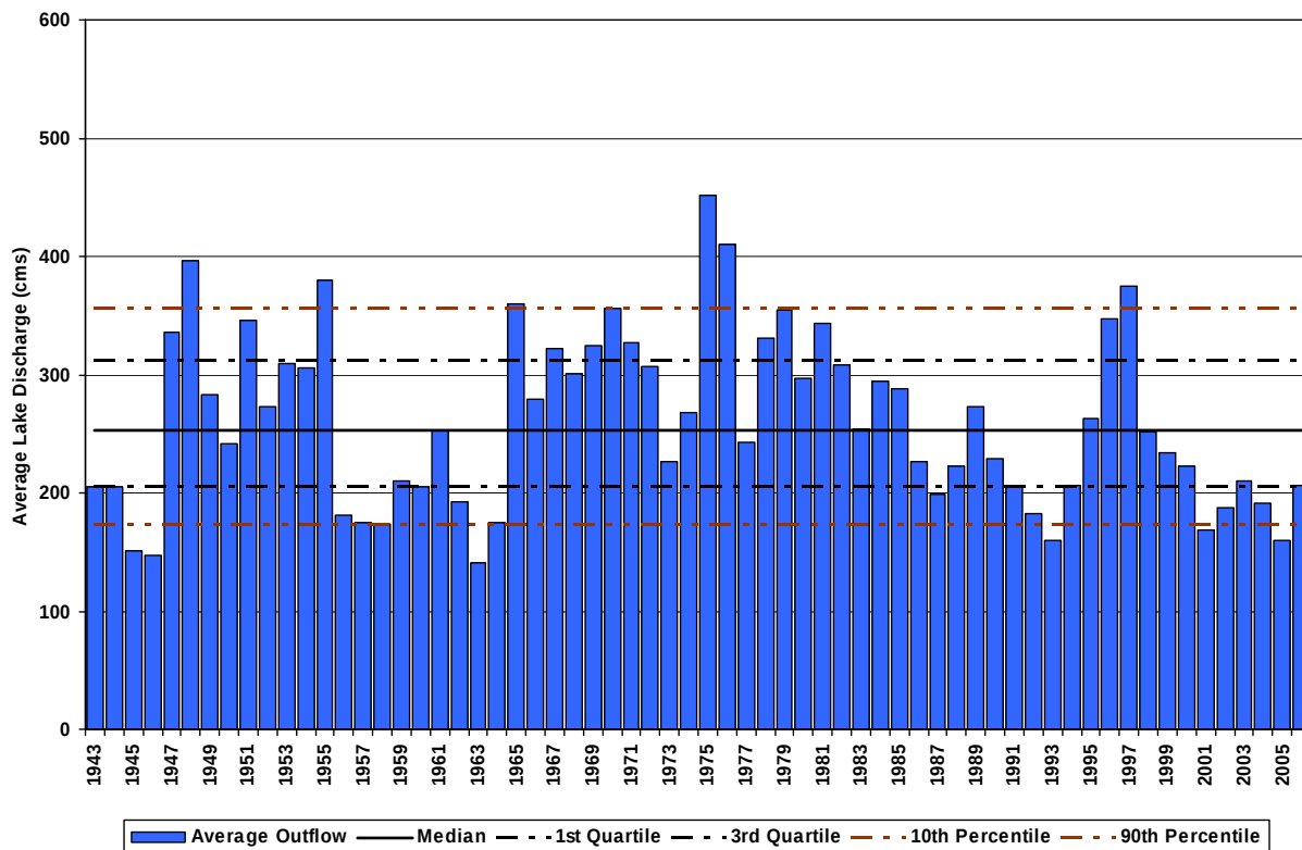
Plate 47. Fort Peck Lake average annual lake outflow and statistics.
