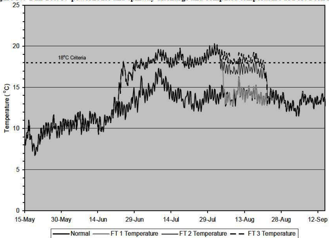
Figure 38. Comparison of Full Test simulated river temperatures at Frazer Rapids, MT.
