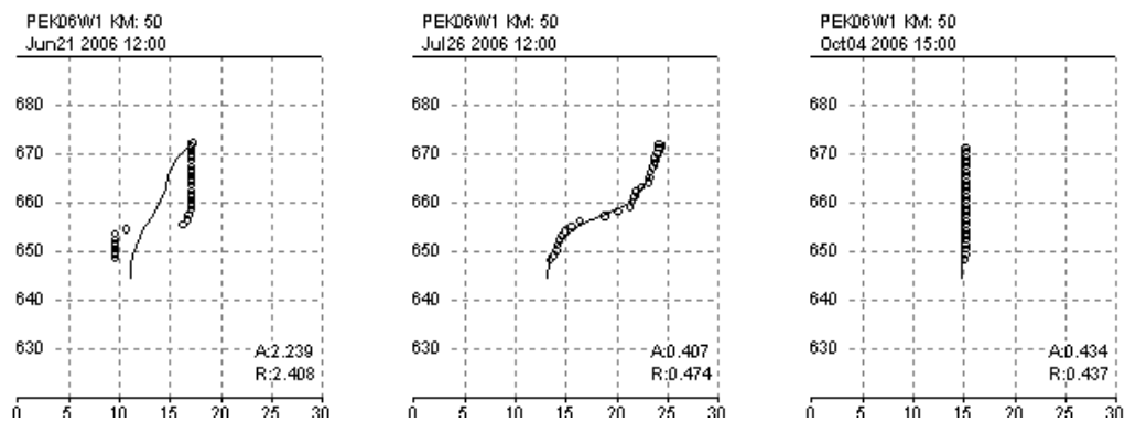
Figure 9-8. 2006 temperature calibration at L4.
