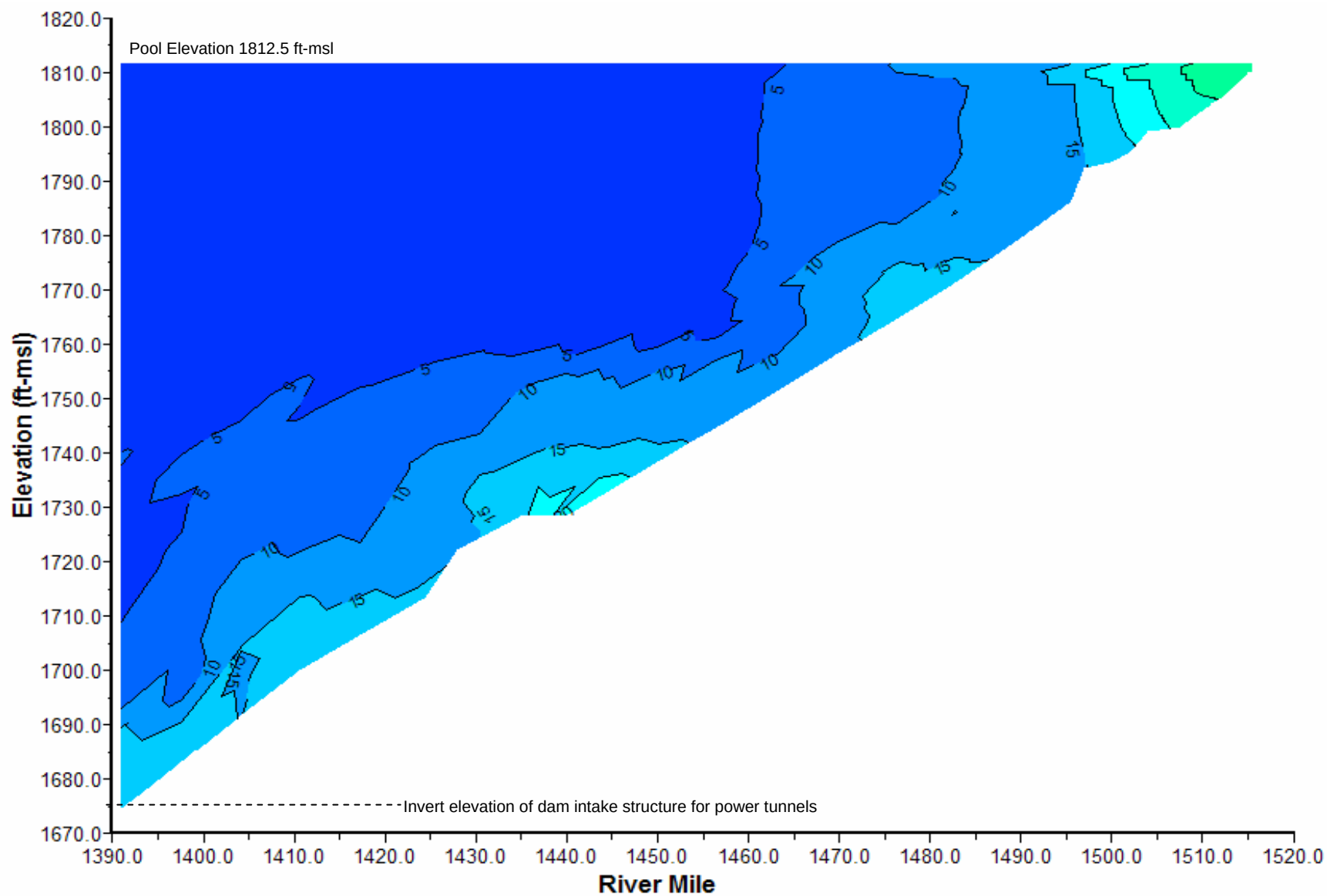
Plate 74. Longitudinal turbidity (NTU) contour plot of Garrison Reservoir based on depth-profile turbidity levels monitored at sites GARLK1390A, GARLK1412DW, GARLK1445DW, GARLK1481DW, and GARNFMORRR1 on August 29, 2006.
