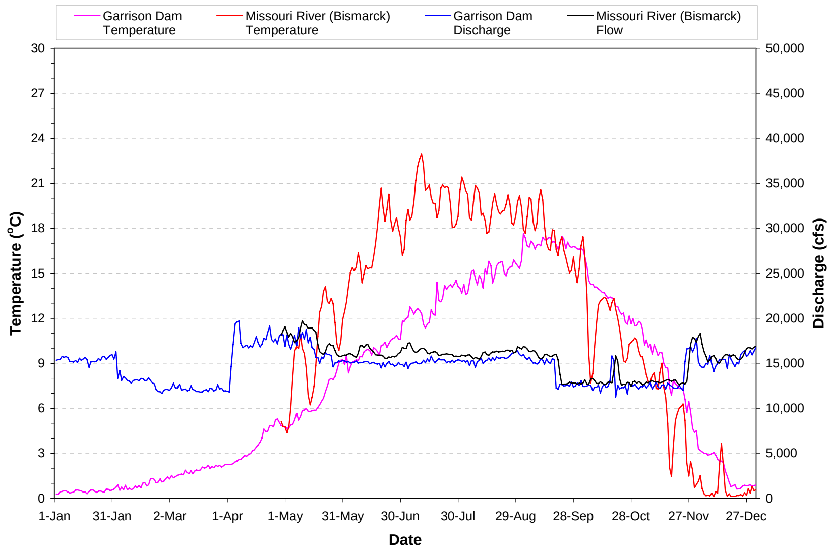
Plate 107. Mean daily water temperature and discharge for the Garrison Dam discharge and Missouri River at Bismarck, North Dakota for 2005. (Daily means based on hourly measurements.)
