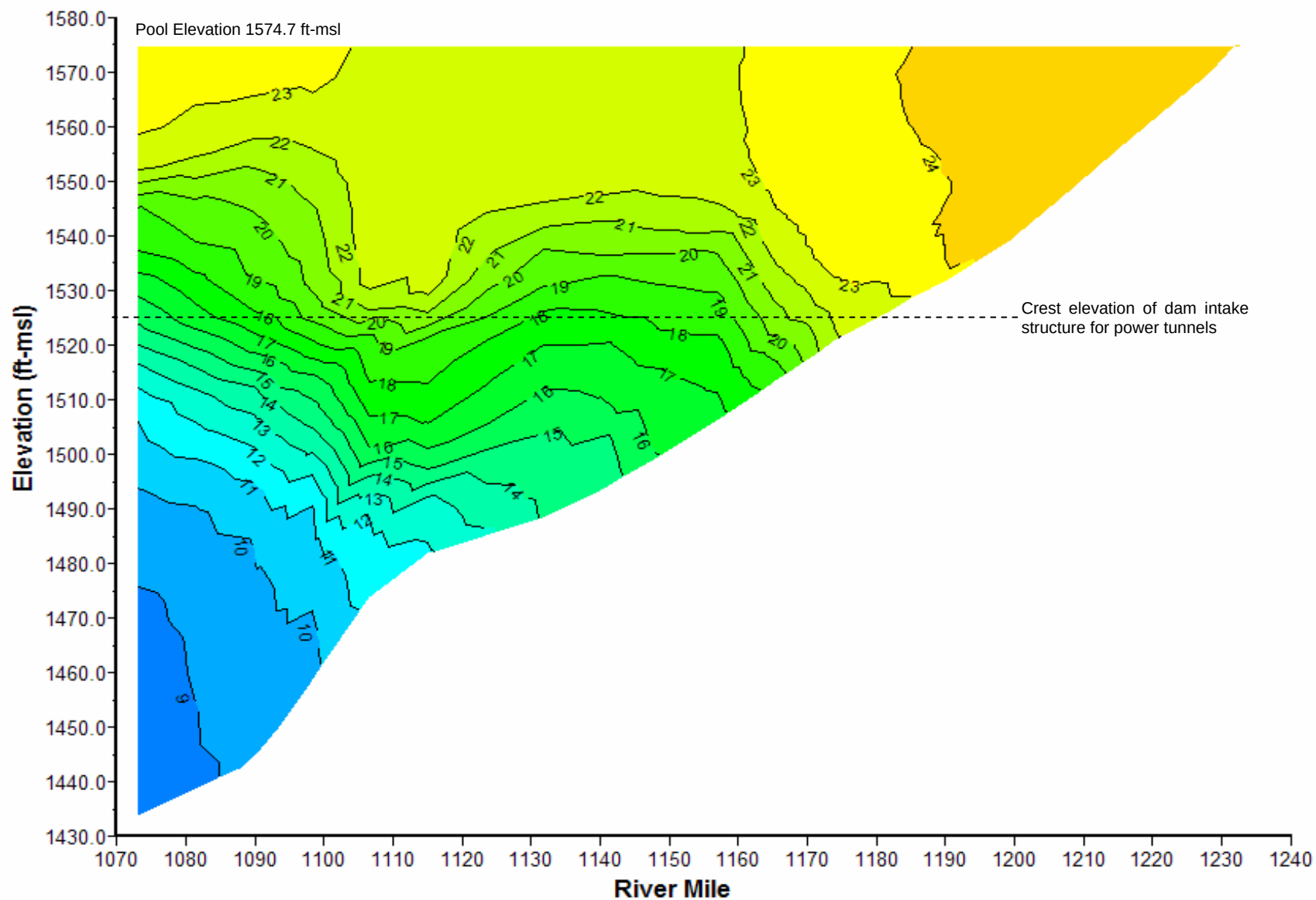
Plate 119. Longitudinal temperature (°C) contour plot of Oahe Reservoir based on depth-profile water temperatures measured at sites OAHRLK1073A, OAHLK1090DW, OAHLK1110DW, OAHLK1135DW, OAHLK1153DW, OAHLK1176DW, OAHLK1196DW and OAHNFMORR1 on July 19, 2006.
