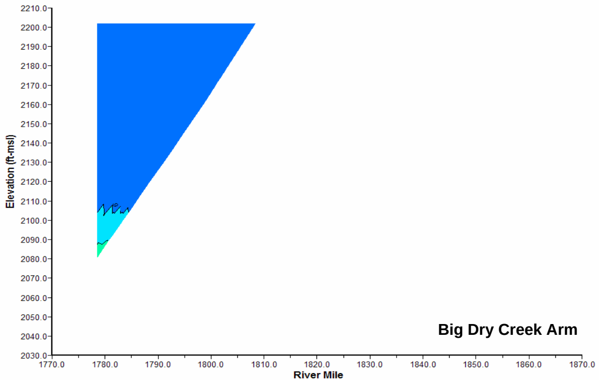
Plate 15. Longitudinal dissolved oxygen (mg/l) contour plot of Fort Peck Reservoir based on depth-profile dissolved oxygen concentrations monitored at sites FTPLK1772A, FTPLK1778DW, FTPLK1789DW, FTPLK1805DW, FTPLKBDCA01, FTPLKBDCA02, and FTPNFMORR1 on October 5, 2006.
