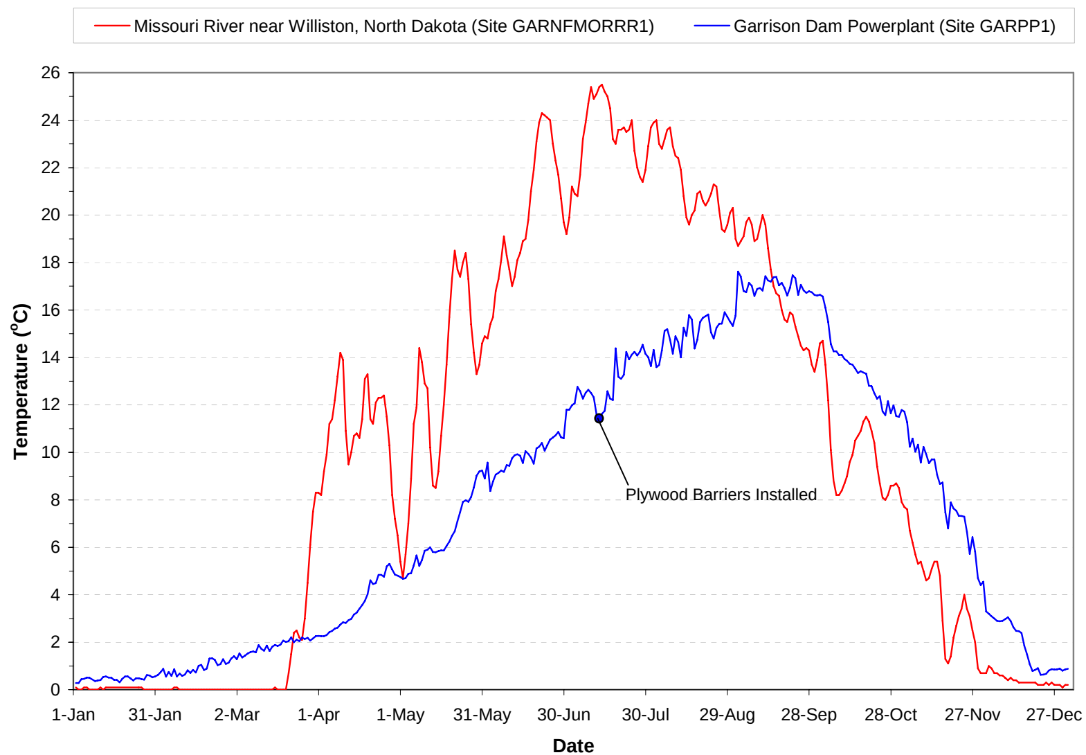
Plate 105. Mean daily water temperatures monitored at the Garrison Powerplant (i.e., site GARPP1) and the Missouri River near Williston, North Dakota (i.e., site GARNFMORRR1) during 2005.
