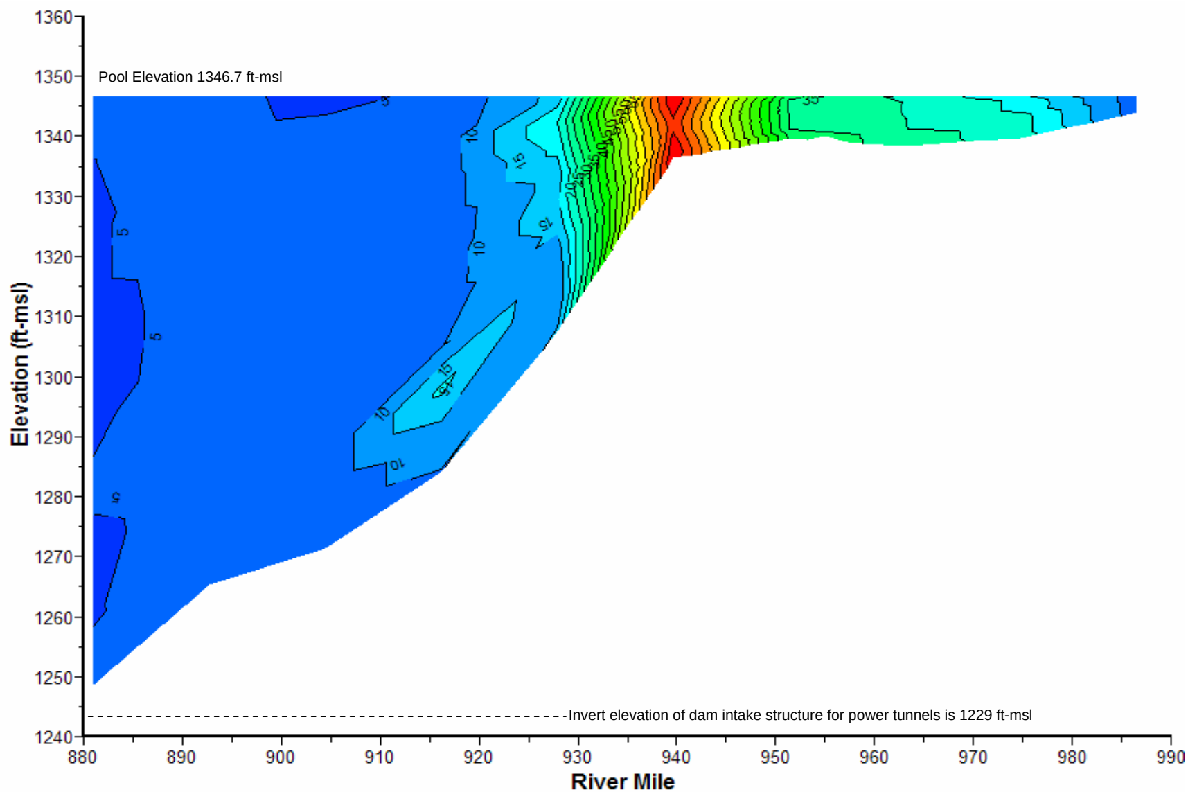
Plate 201. Longitudinal turbidity (NTU) contour plot of Fort Randall Reservoir based on depth-profile dissolved oxygen concentrations measured at sites FTRLK0880A, FTRLK0892DW, FTRLK0911DW, FTRLK0924DW, FTRLK0940DW, FTRLK0955DW, FTRLK0968DW, and BBDPP1 on September 21, 2006.
