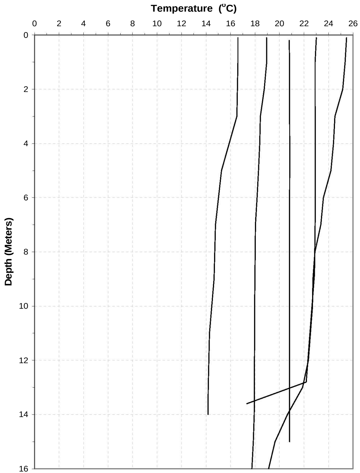
Plate 272. Temperature depth profiles for Lake Audubon generated from data collected at the near-dam, deepwater ambient monitoring site during the months of June, July, and August during 2002 and 2006.
