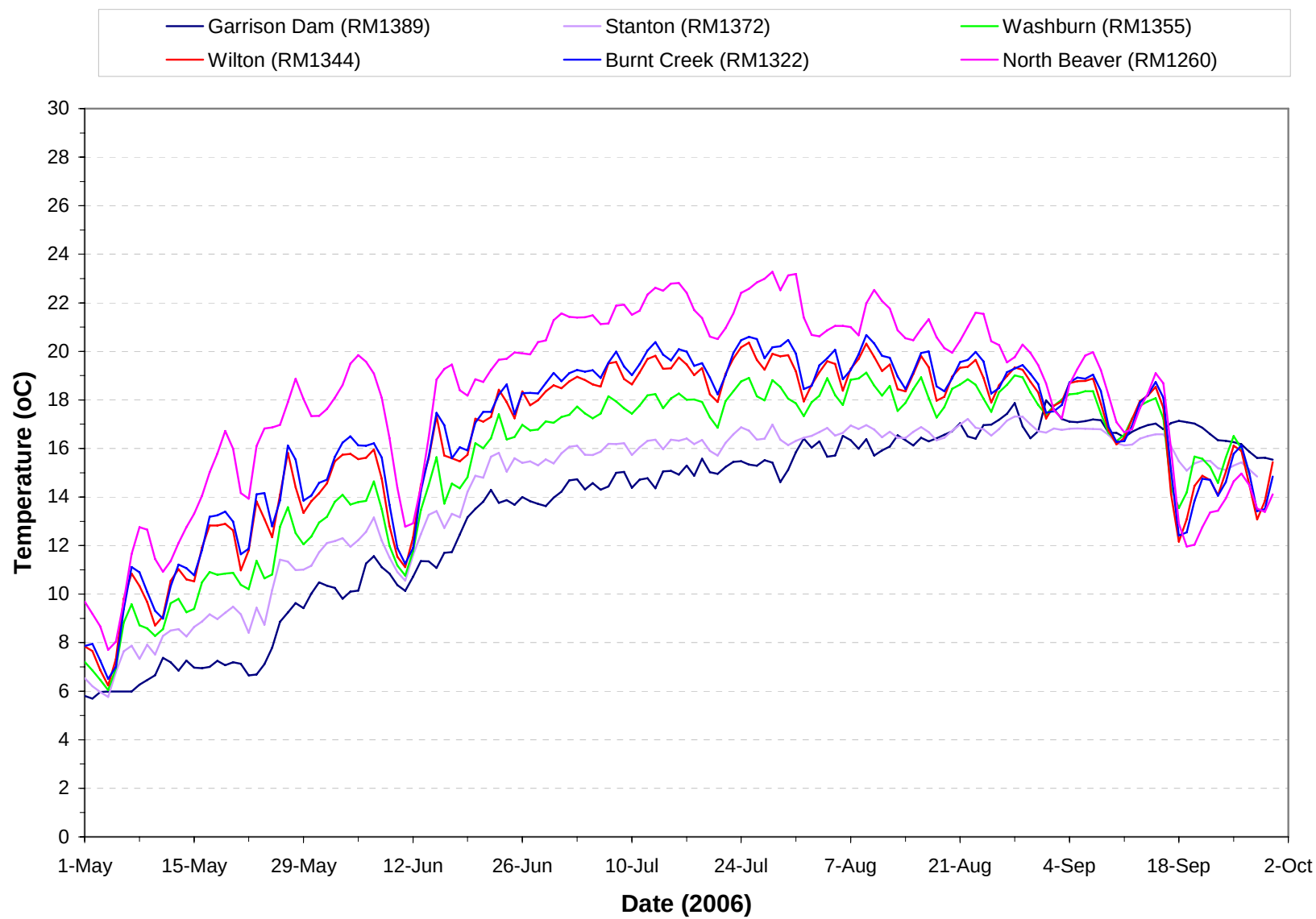
Plate 110. Mean daily water temperatures monitored in the Missouri River from Garrison Dam to Beaver Bay for the period May through September 2006.
