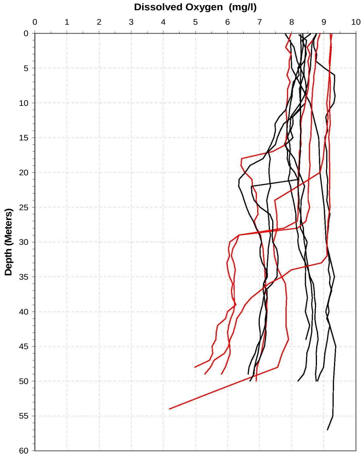
Plate 16. Dissolved oxygen depth profiles for Fort Peck Reservoir compiled from data collected at the near-dam, deepwater ambient monitoring site (i.e., FTPLK1772A) during the months of July, August, and September over the 5-year period of 2002 to 2006. (Note: Red profile plots were measured in the month of September.)
