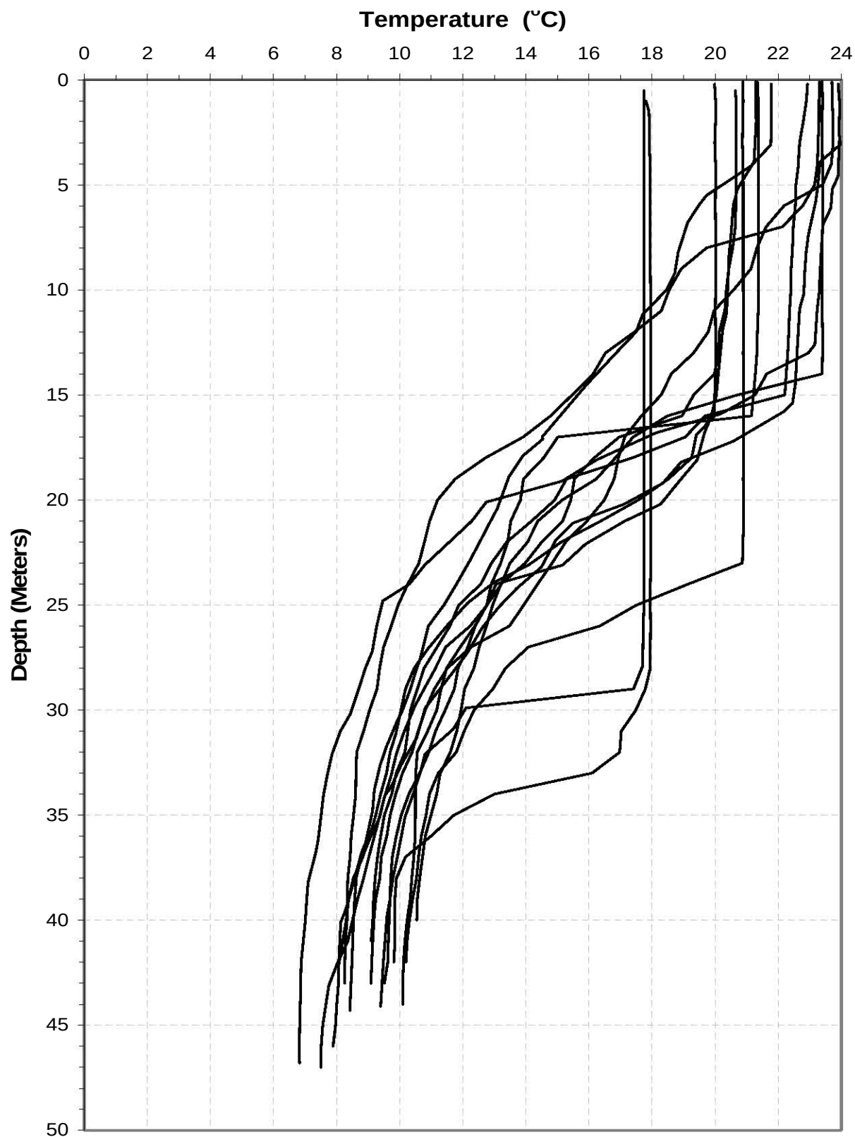
Plate 122. Temperature depth profiles for Oahe Reservoir generated from data collected at the near-dam, deepwater ambient monitoring site (i.e., OAHLK1073A) during the months of July, August, and September over the 5-year period of 2002 to 2006.
