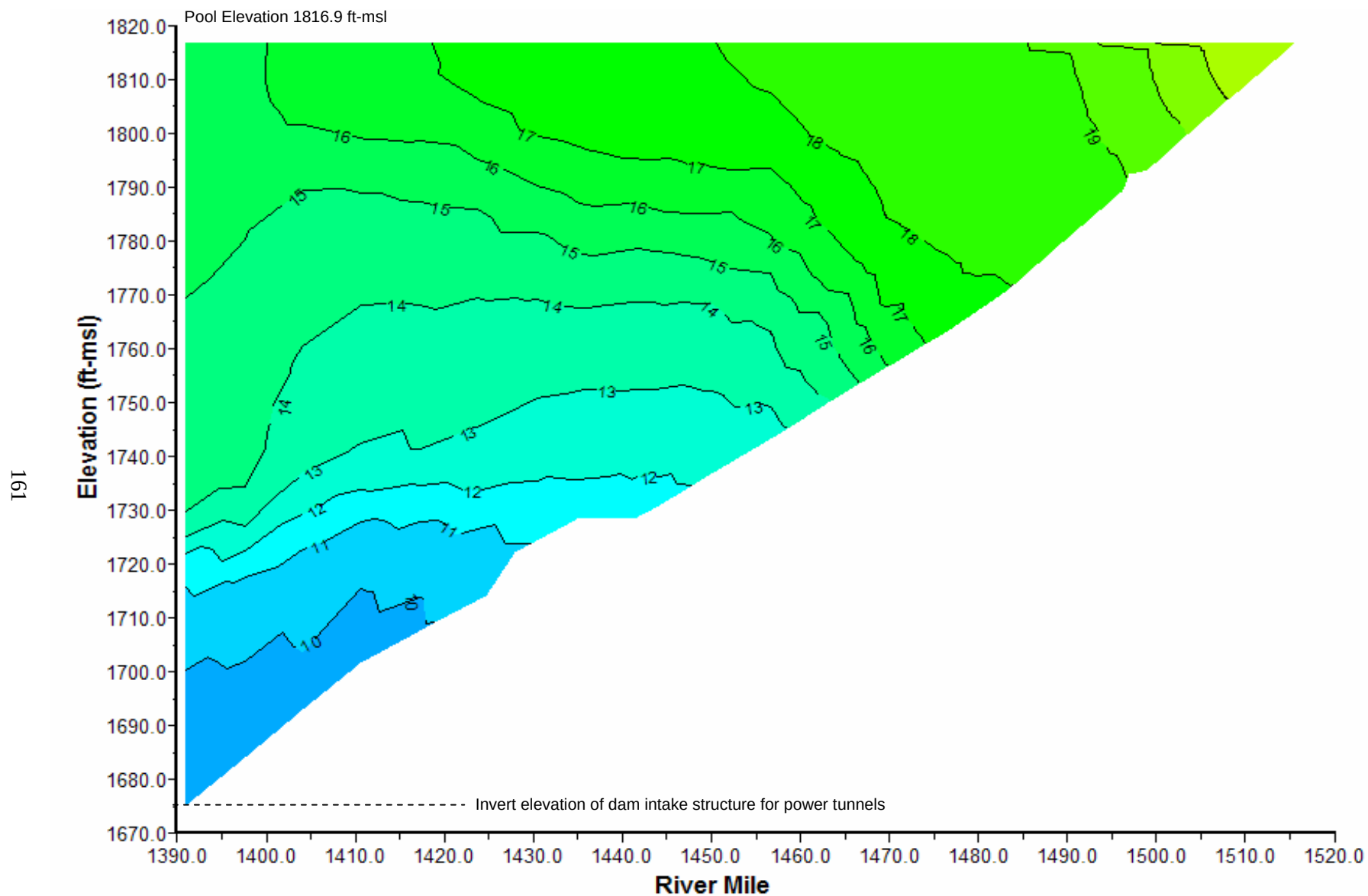
Plate 58. Longitudinal water temperature (°C) contour plot of Garrison Reservoir based on depth-profile water temperatures measured at sites GARLK1390A, GARLK1412DW, GARLK1445DW, GARLK1481DW, and GARNFMORRR1 on June 20, 2006.
