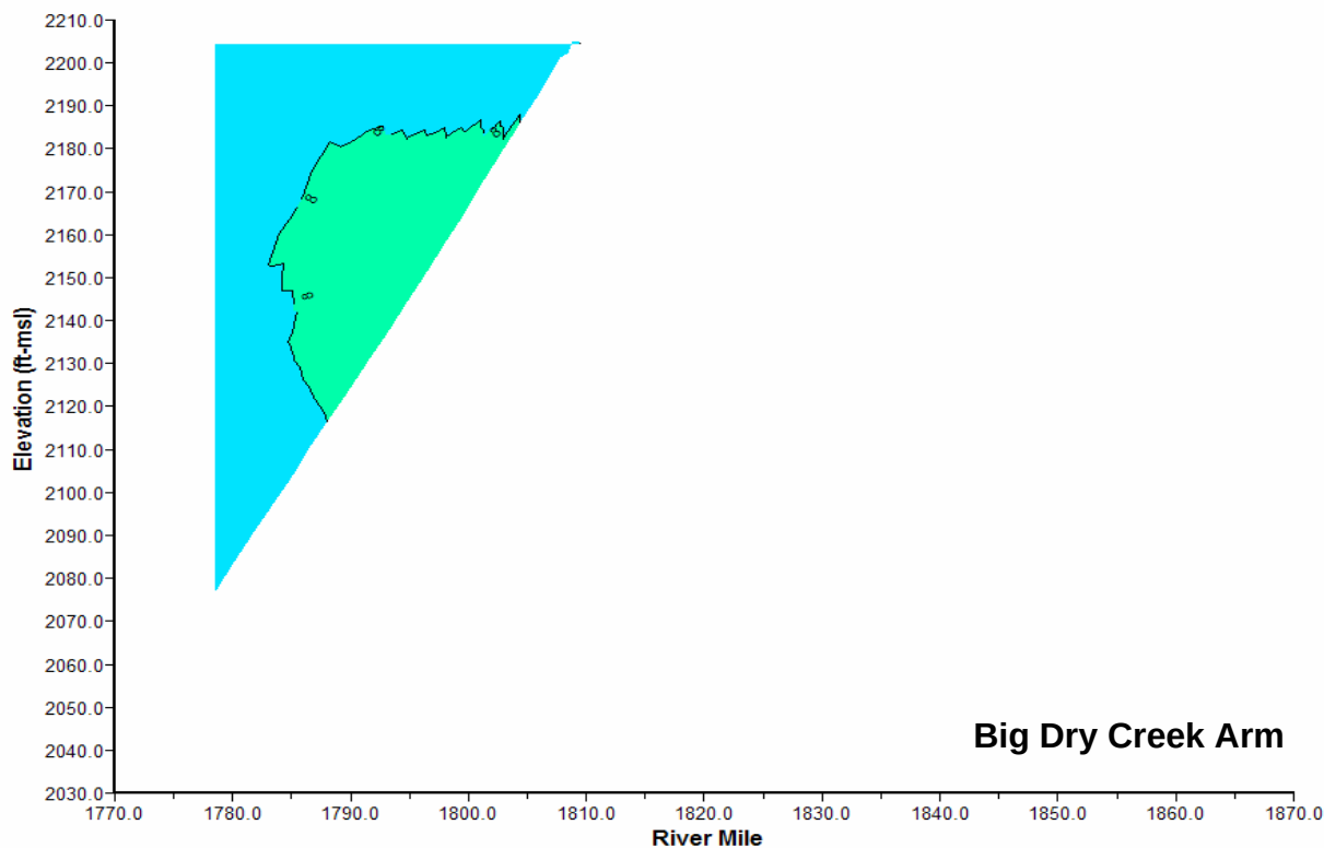
Plate 13. Longitudinal dissolved oxygen (mg/l) contour plot of Fort Peck Reservoir based on depth-profile dissolved oxygen concentrations monitored at sites FTPLK1772A, FTPLK1778DW, FTPLK1789DW, FTPLK1805DW, FTPLKBDCA01, FTPLKBDCA02, and FTPNFMORR1 on July 26, 2006.
