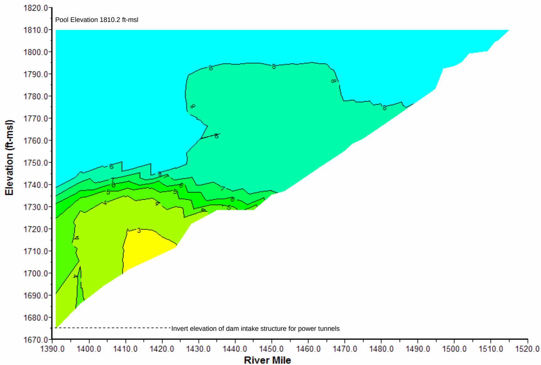
Plate 68. Longitudinal dissolved oxygen (mg/l) contour plot of Garrison Reservoir based on depth-profile dissolved oxygen concentrations measured at sites GARLK1390A, GARLK1412DW, GARLK1445DW, GARLK1481DW, and GARNFMORRR1 on September 13, 2006.
