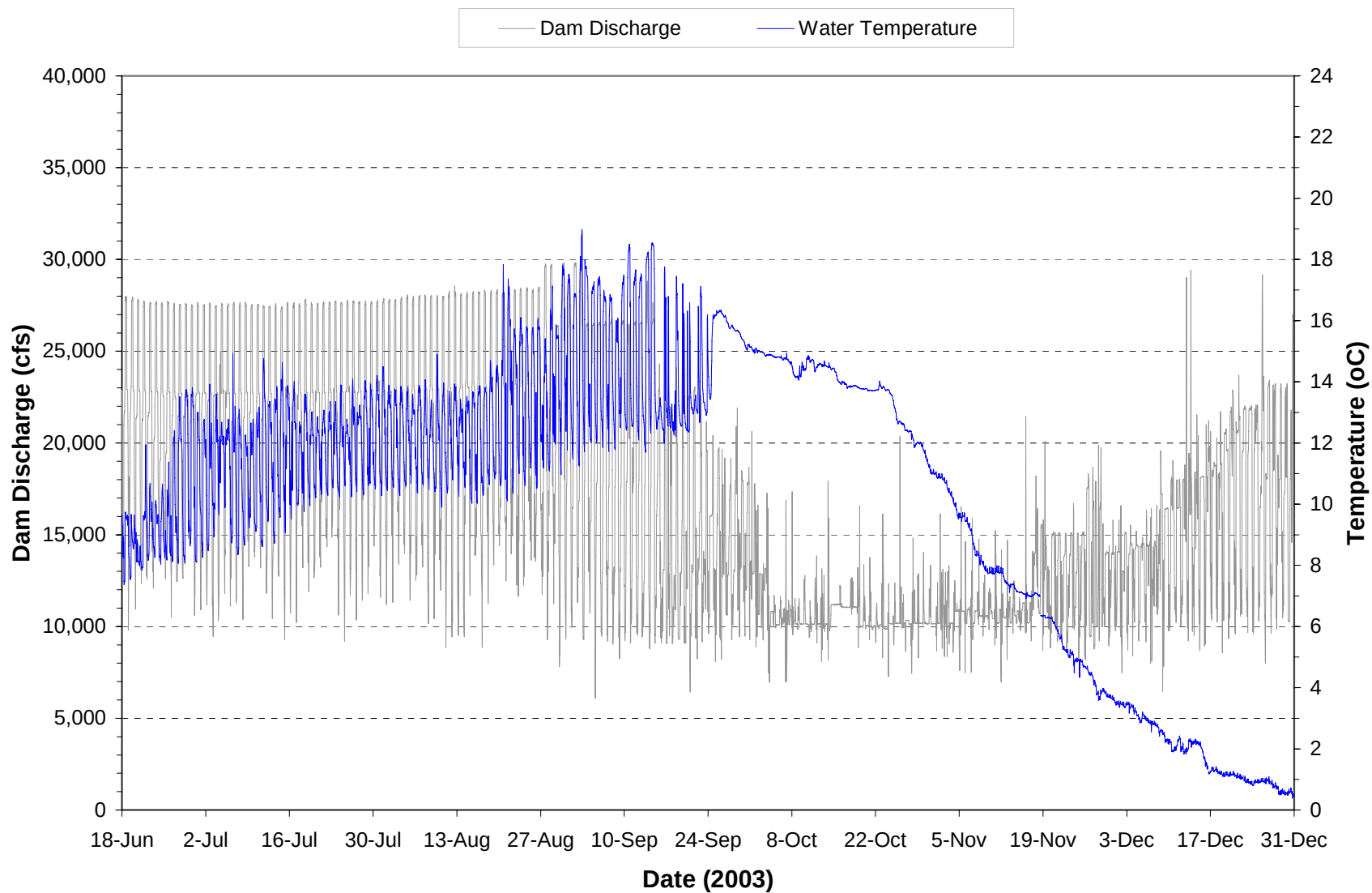
Plate 89. Hourly discharge and water temperature monitored at the Garrison powerplant on water discharged through the dam during the period June through December 2003.
