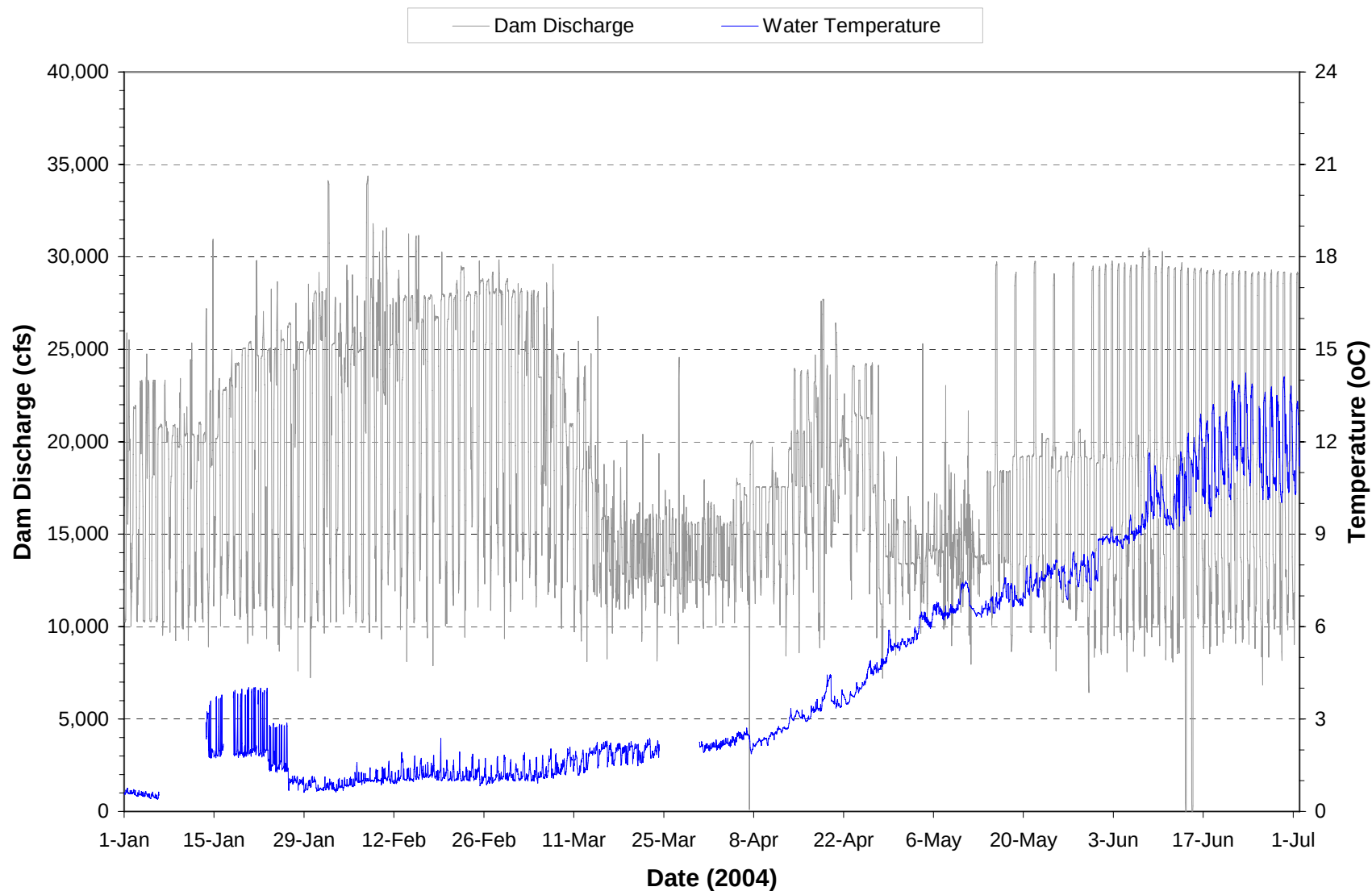
Plate 90. Hourly discharge and water temperature monitored at the Garrison powerplant on water discharged through the dam during the period January through June 2004. (Note: Gaps in temperature plot represents periods when monitoring equipment was not operational.)
