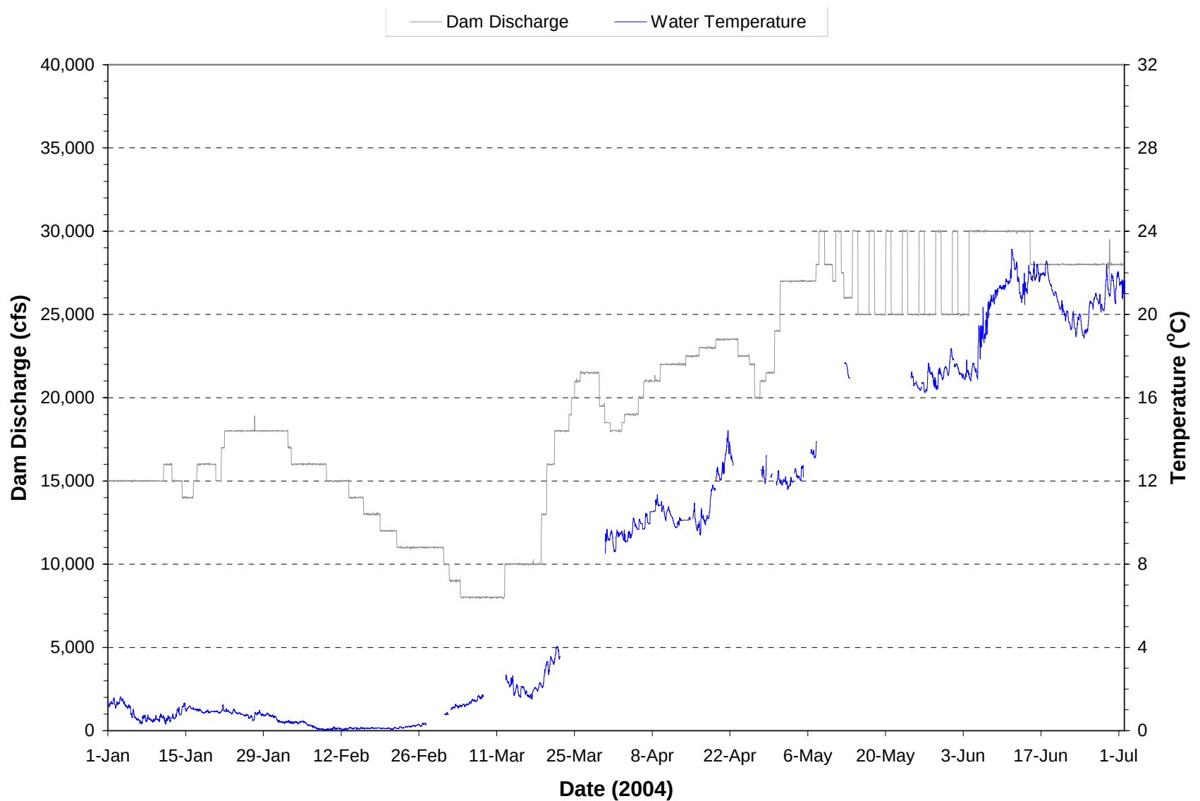
Plate 243. Hourly discharge and water temperature monitored at the Gavins Point powerplant on water discharged through the dam during the period January through June 2004. (Note: Gaps in temperature plot represents periods when monitoring equipment was not operational.)
