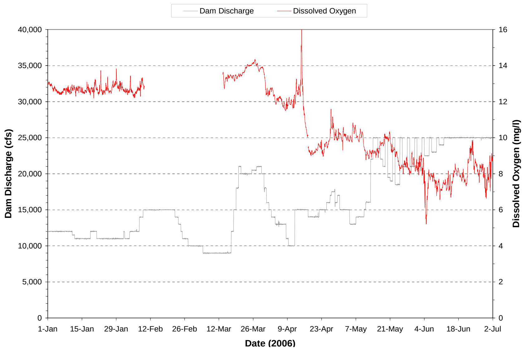
Plate 253. Hourly discharge and dissolved oxygen monitored at the Gavins Point powerplant on water discharged through the dam during the period January through June 2006. (Note: Gaps in temperature plot represents periods when monitoring equipment was not operational.)
