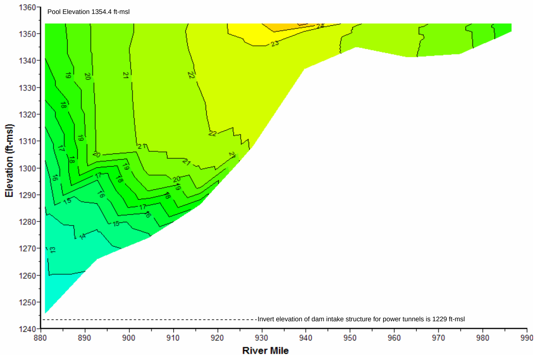
Plate 188. Longitudinal water temperature (°C) contour plot of Fort Randall Reservoir based on depth-profile water temperatures measured at sites FTRLK0880A, FTRLK0892DW, FTRLK0911DW, FTRLK0924DW, FTRLK0940DW, FTRLK0955DW, FTRLK0968DW, and BBDPP1 on June 15, 2006.
