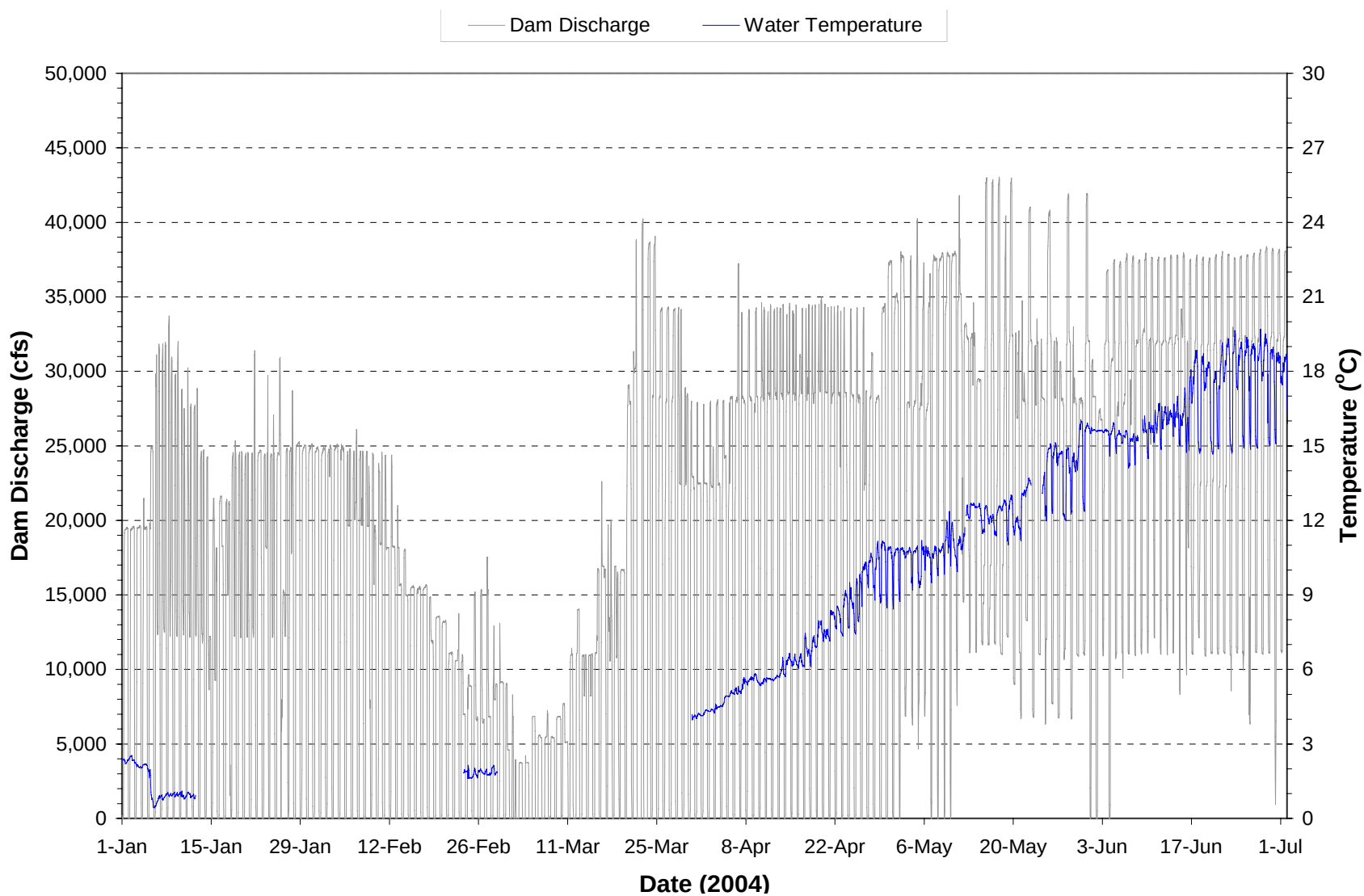
Plate 212. Hourly discharge and water temperature monitored at the Fort Randall powerplant on water discharged through the dam during the period January through June 2004. (Note: Gaps in temperature plot represents periods when monitoring equipment was not operational.)
