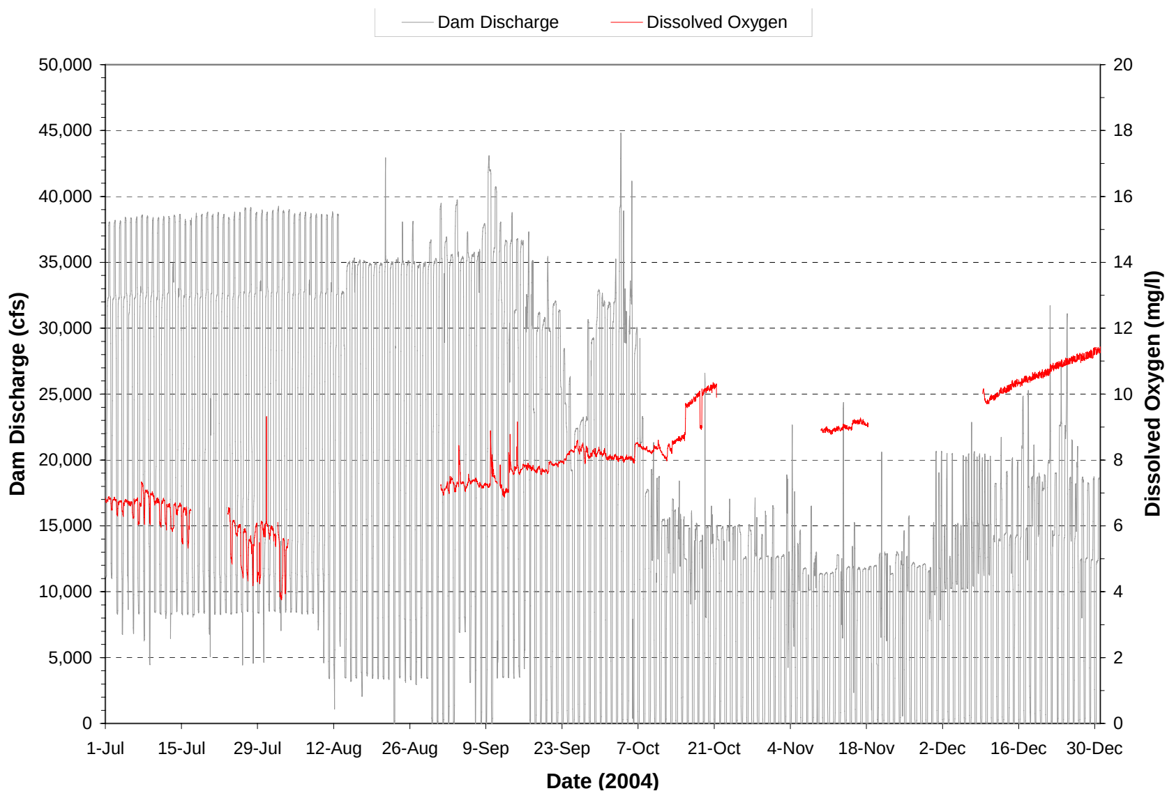
Plate 219. Hourly discharge and dissolved oxygen concentrations monitored at the Fort Randall powerplant on water discharged through the dam during the period July through December 2004. (Note: Gaps in dissolved oxygen plot represents periods when monitoring equipment was not operational.)
