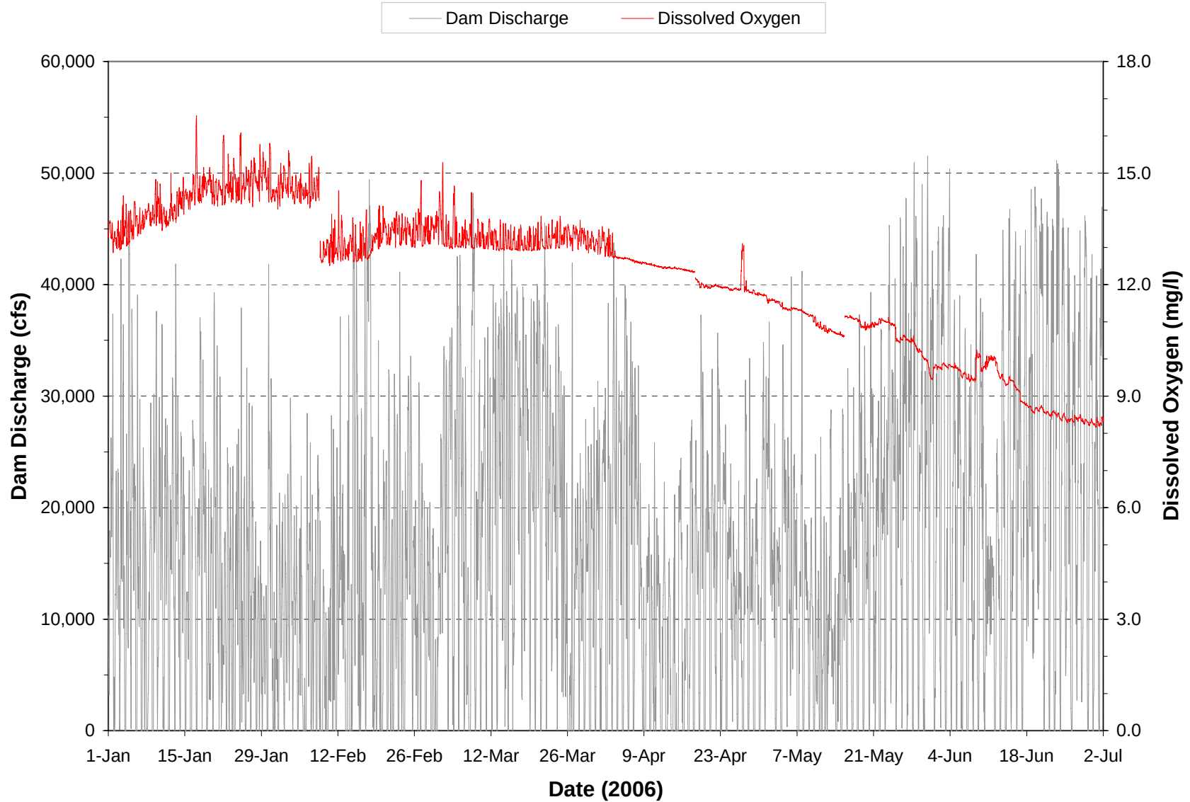
Plate 153. Hourly discharge and dissolved oxygen monitored at the Oahe powerplant on water discharged through the dam during the period January through June 2006. (Note: Gaps in dissolved oxygen plot represents periods when monitoring equipment was not operational.)
