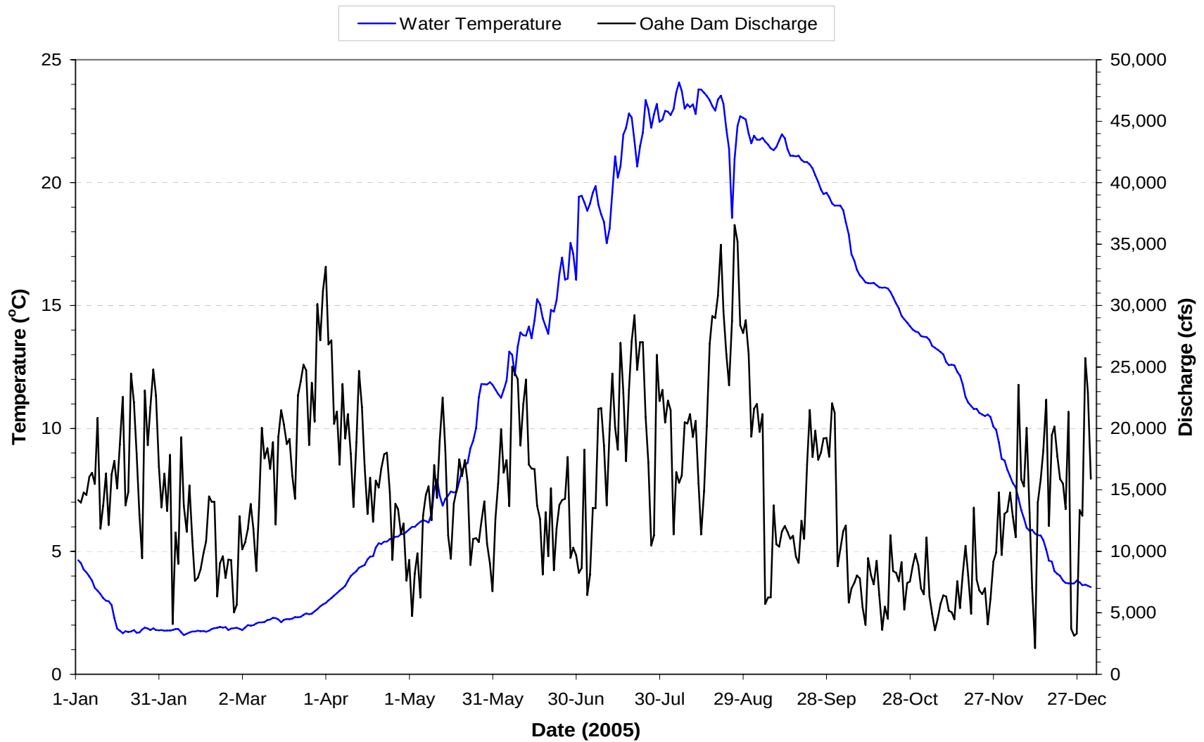
Plate 164. Mean daily water temperature and discharge of the Missouri River at Oahe Dam (i.e., site OAHPP1) for 2005. Mean daily temperatures and discharges based on hourly measurements recorded on discharge through Oahe Dam.
