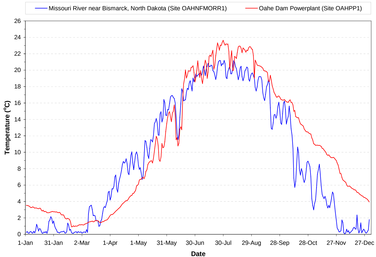
Plate 156. Mean daily water temperatures monitored at the Oahe Powerplant (i.e., site OAHPP1) and the Missouri River near Bismarck, North Dakota (i.e., site OAHNFMORR1) during 2006. (Note: Gaps in temperature plots are periods when monitoring equipment was not operational.)
