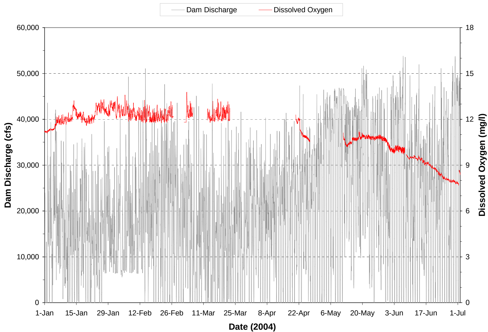
Plate 149. Hourly discharge and dissolved oxygen monitored at the Oahe powerplant on water discharged through the dam during the period January through June 2004. (Note: Gaps in dissolved oxygen plot represents periods when monitoring equipment was not operational.)
