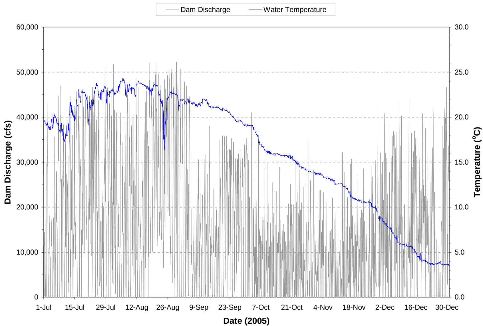
Plate 146. Hourly discharge and water temperature monitored at the Oahe powerplant on water discharged through the dam during the period July through December 2005.
