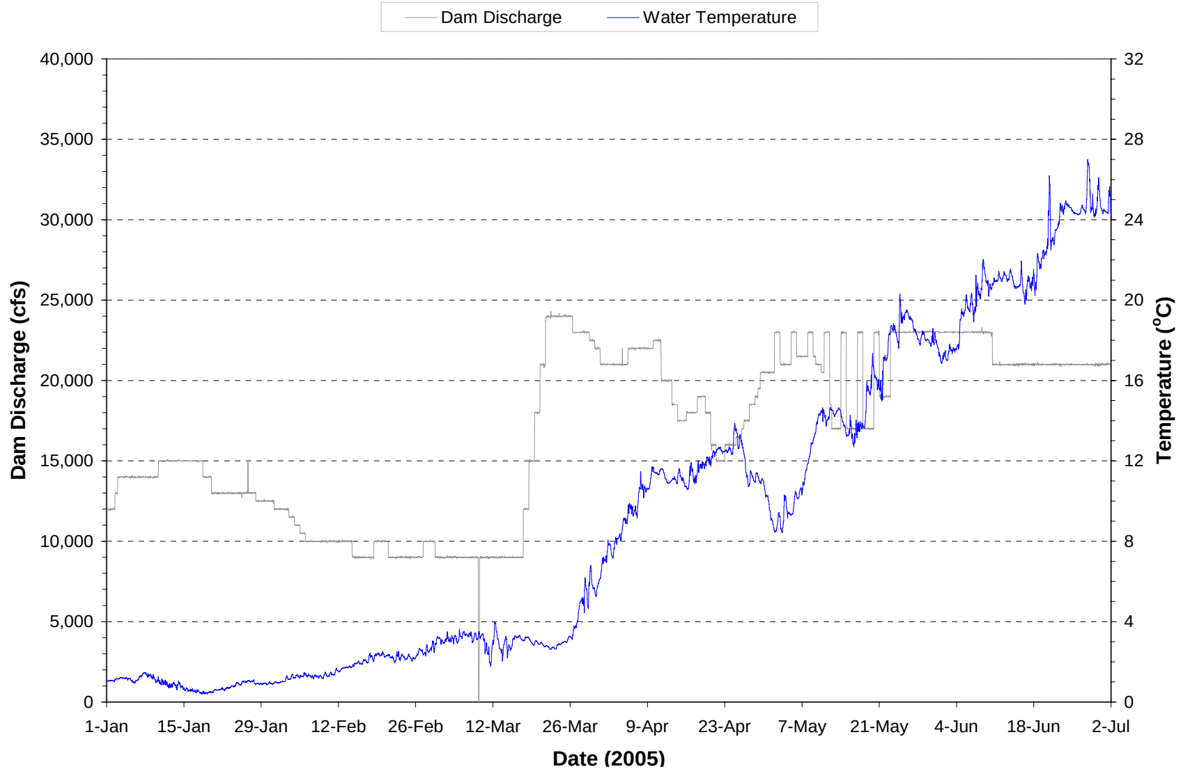
Plate 245. Hourly discharge and water temperature monitored at the Gavins Point powerplant on water discharged through the dam during the period January through June 2005. (Note: Gaps in temperature plot represents periods when monitoring equipment was not operational.)
