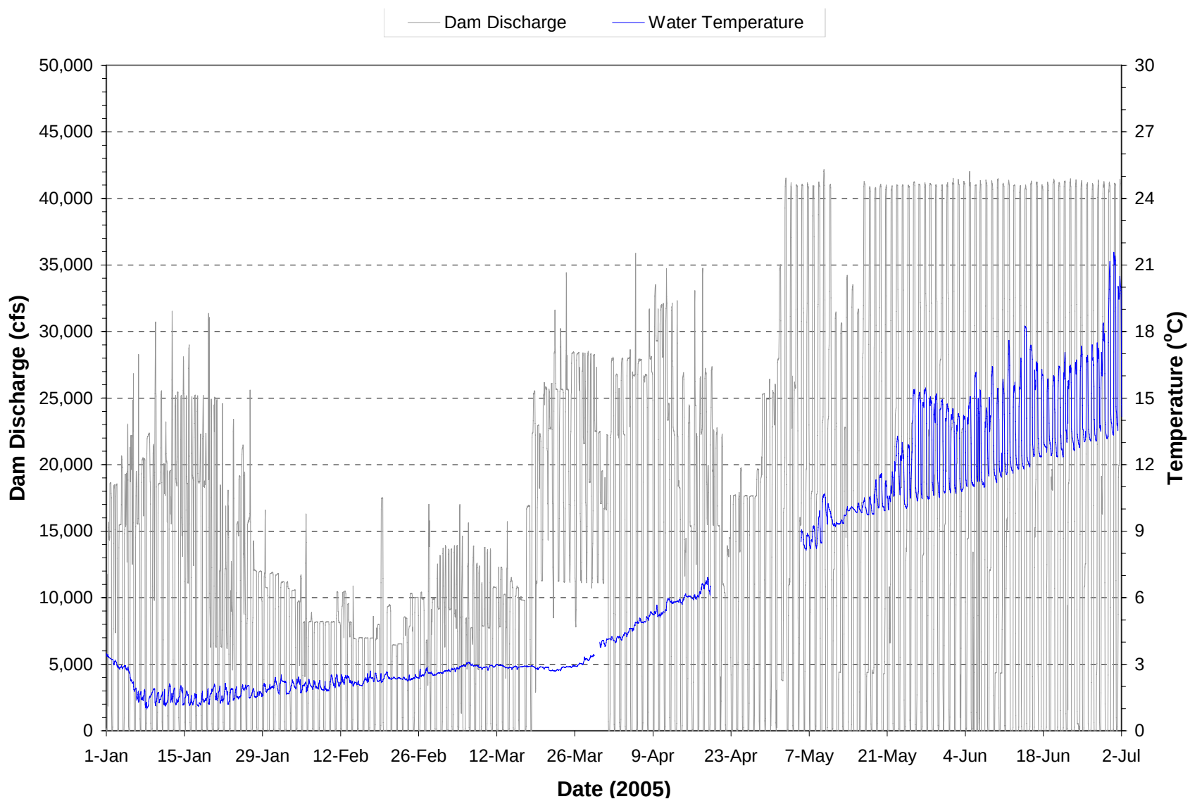
Plate 214. Hourly discharge and water temperature monitored at the Fort Randall powerplant on water discharged through the dam during the period January through June 2005. (Note: Gaps in temperature plot represents periods when monitoring equipment was not operational.)
