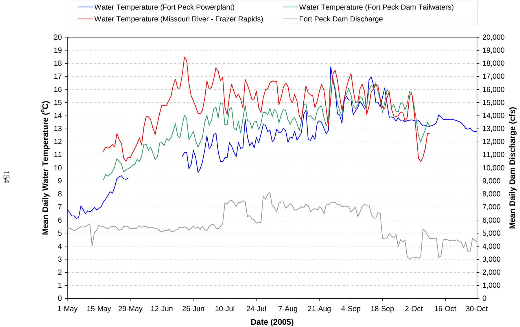
Plate 47. Mean daily water temperature monitored at the Fort Peck powerplant, Missouri River tailwaters, and Missouri River Frazer Rapids and the mean daily discharge of Fort Peck Dam from May through October during 2005.
