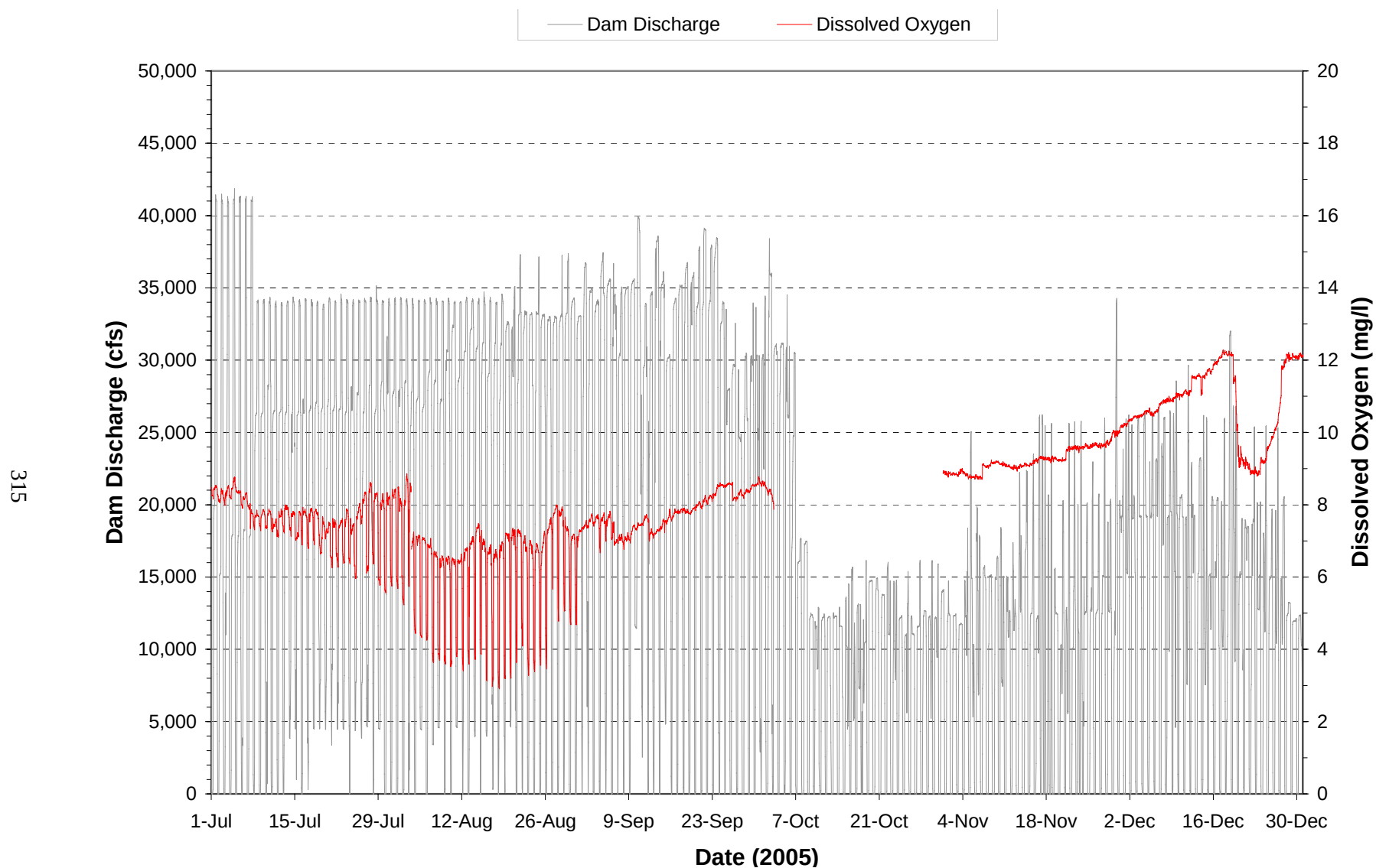
Plate 221. Hourly discharge and dissolved oxygen concentrations monitored at the Fort Randall powerplant on water discharged through the dam during the period July through December 2005. (Note: Gaps in dissolved oxygen plot represents periods when monitoring equipment was not operational.)
