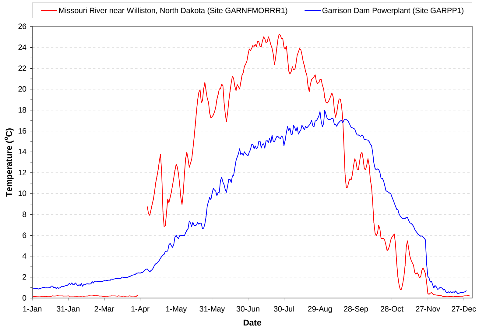
Plate 106. Mean daily water temperatures monitored at the Garrison Powerplant (i.e., site GARPP1) and the Missouri River near Williston, North Dakota (i.e., site GARNFMORRR1) during 2006. (Note: Gaps in temperature plots are periods when monitoring equipment was not operational.)
