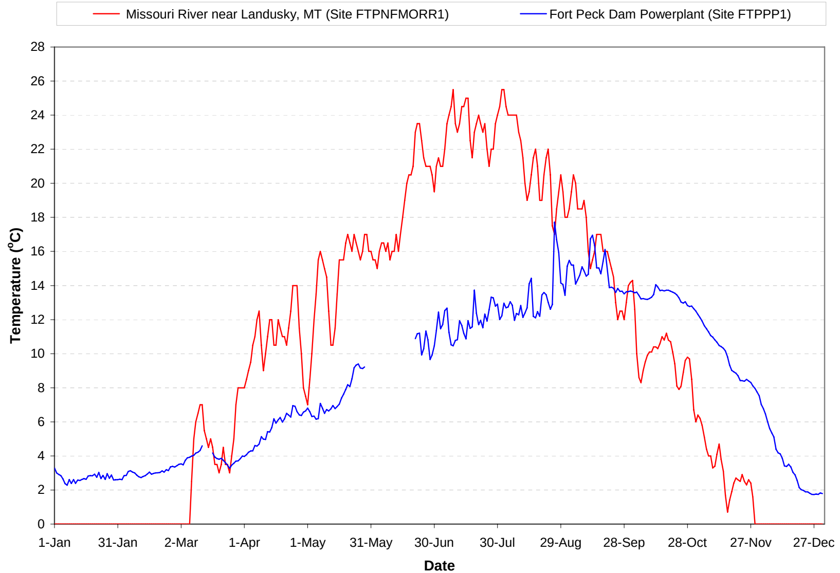
Plate 44. Mean daily water temperatures monitored at the Fort Peck Powerplant (i.e., site FTPPP1) and the Missouri River near Landusky, Montana (i.e., site FTPNFMORR1) during 2005. (Note: Gaps in temperature plots are periods when monitoring equipment was not operational.)
