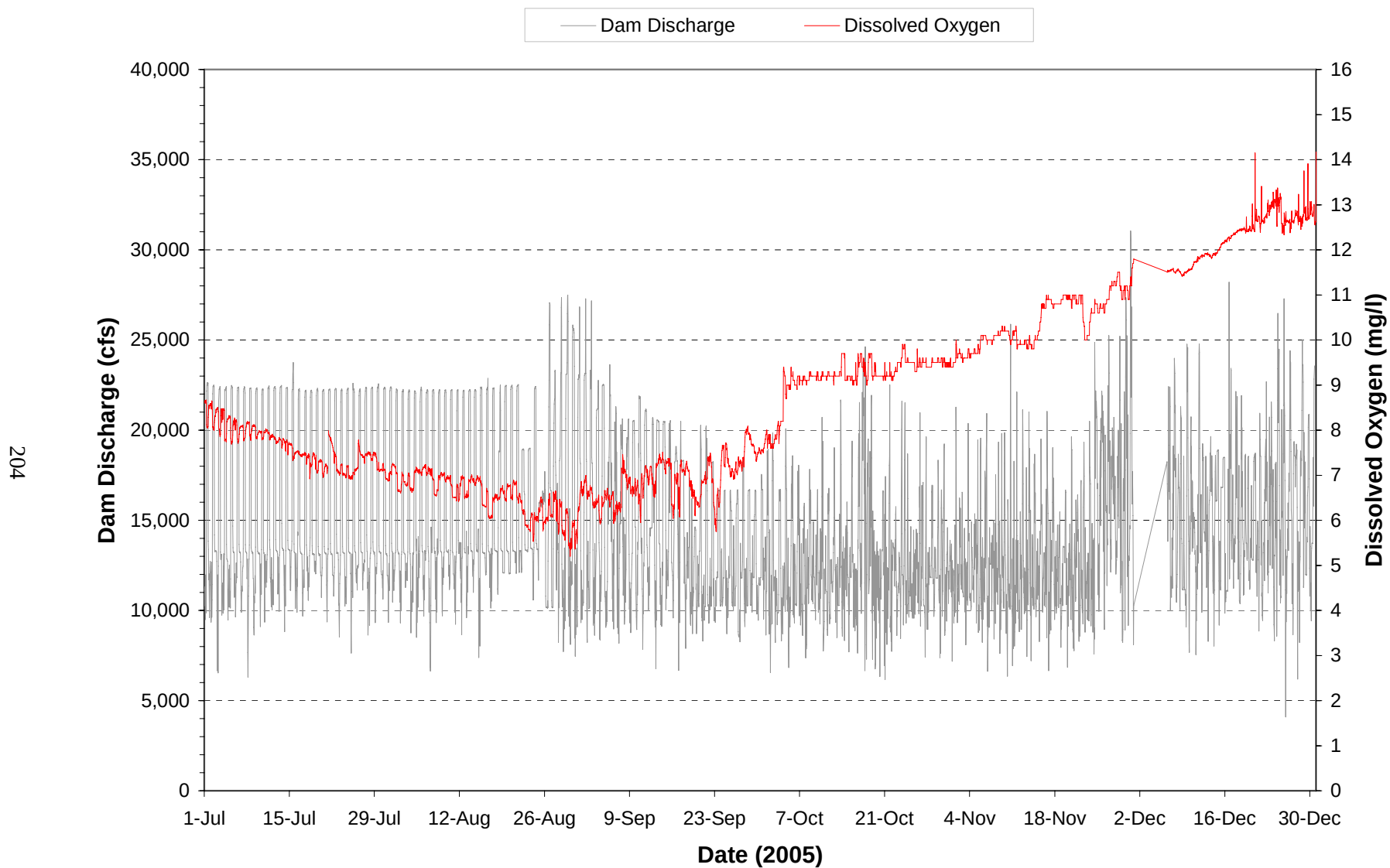
Plate 101. Hourly discharge and dissolved oxygen monitored at the Garrison powerplant on water discharged through the dam during the period July through December 2005.
