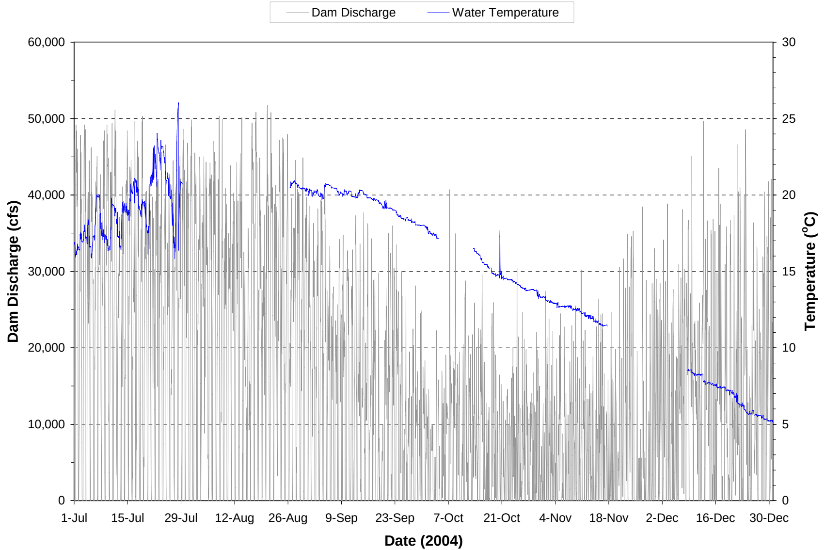
Plate 144. Hourly discharge and water temperature monitored at the Oahe powerplant on water discharged through the dam during the period July through December 2004. (Note: Gaps in temperature plot represents periods when monitoring equipment was not operational.)
