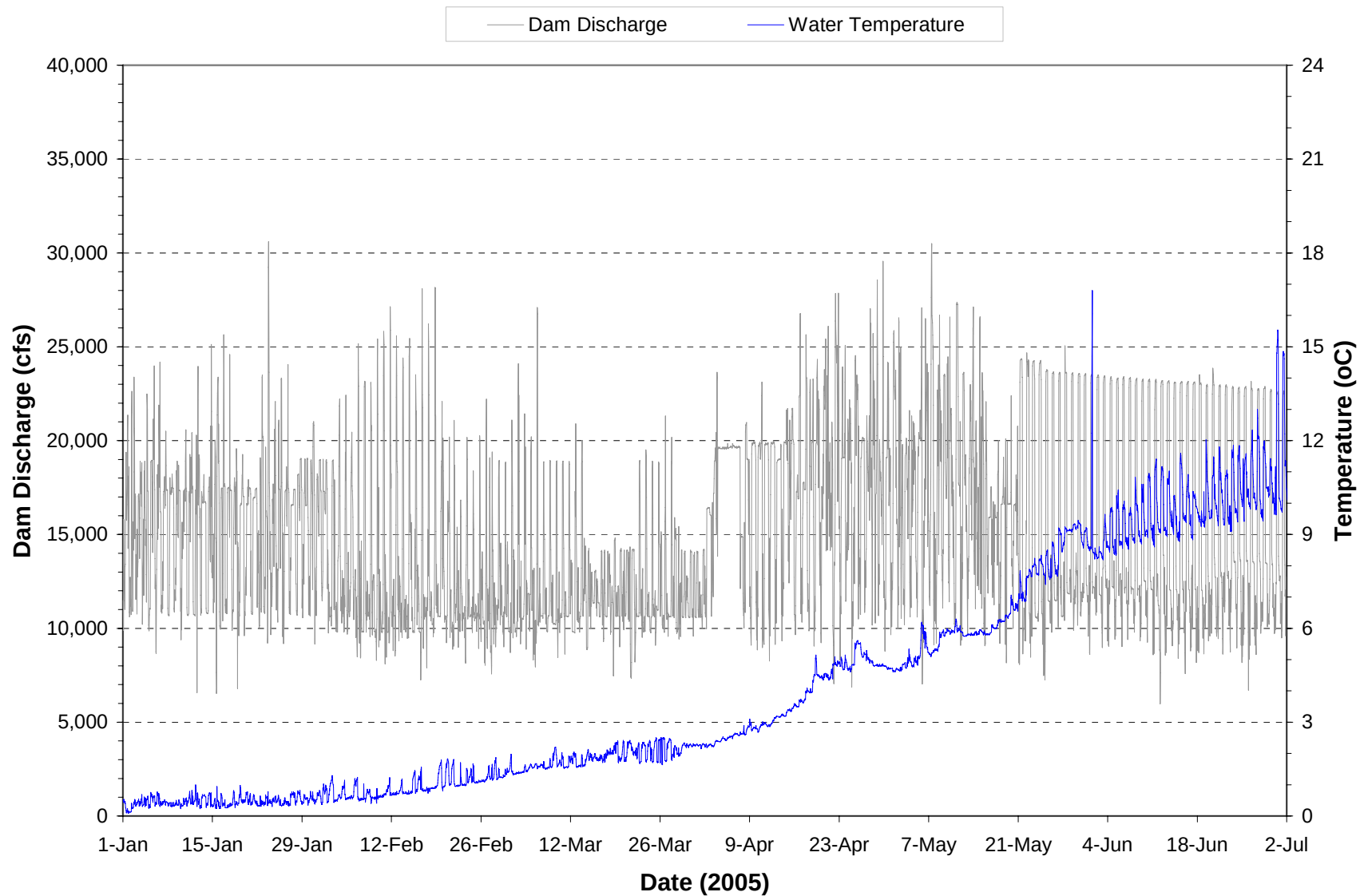
Plate 92. Hourly discharge and water temperature monitored at the Garrison powerplant on water discharged through the dam during the period January through June 2005.
