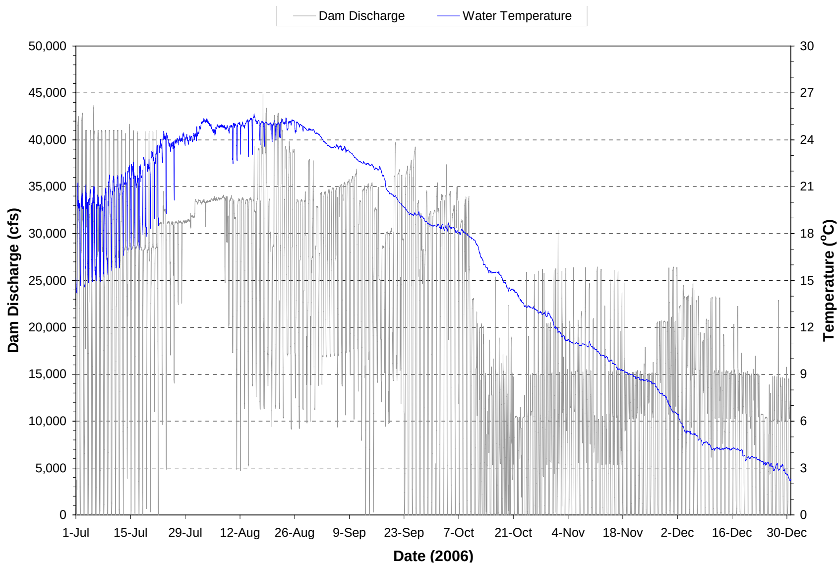
Plate 217. Hourly discharge and water temperature monitored at the Fort Randall powerplant on water discharged through the dam during the period July through December 2006.
