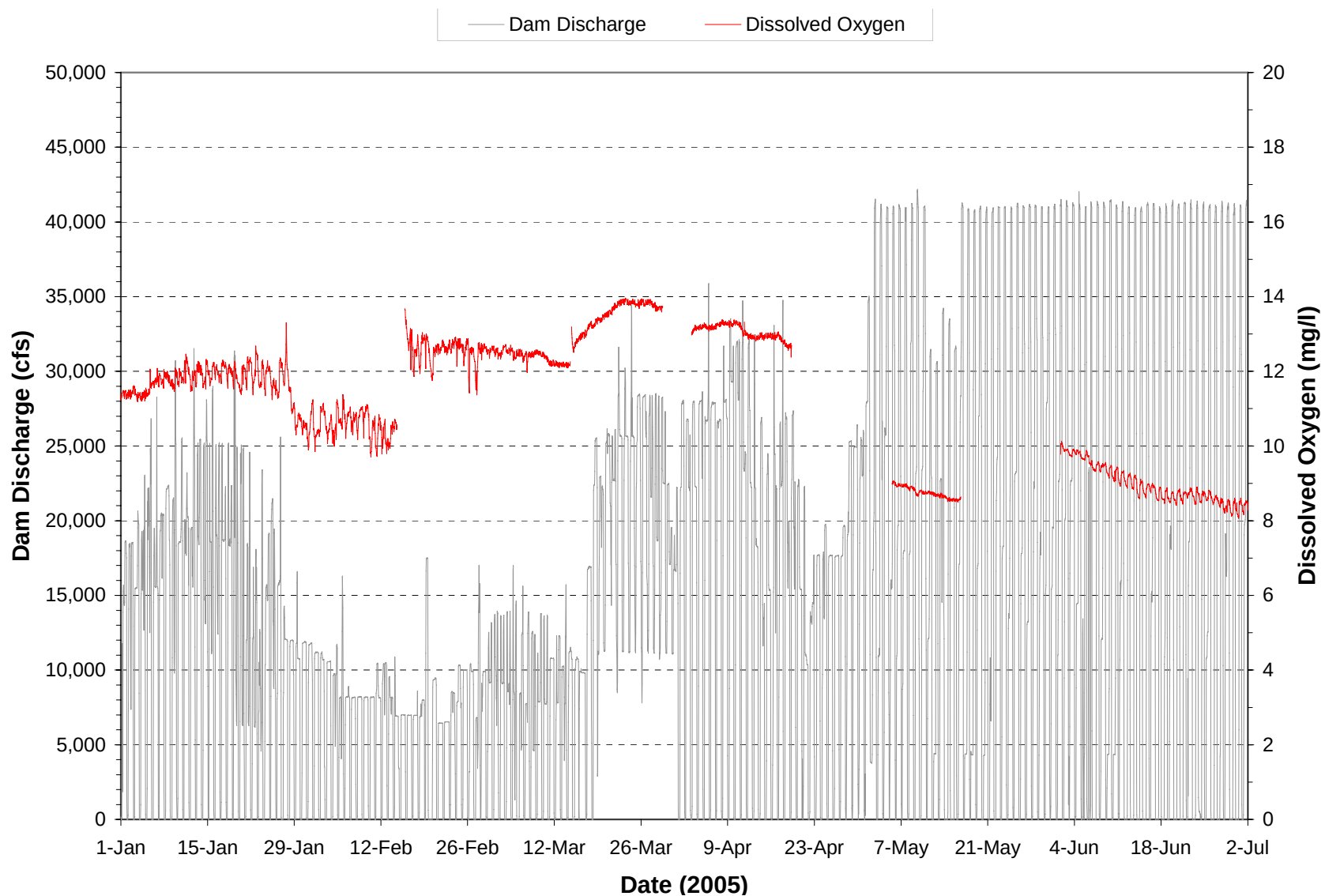
Plate 220. Hourly discharge and dissolved oxygen concentrations monitored at the Fort Randall powerplant on water discharged through the dam during the period January through June 2005. (Note: Gaps in dissolved oxygen plot represents periods when monitoring equipment was not operational.)
