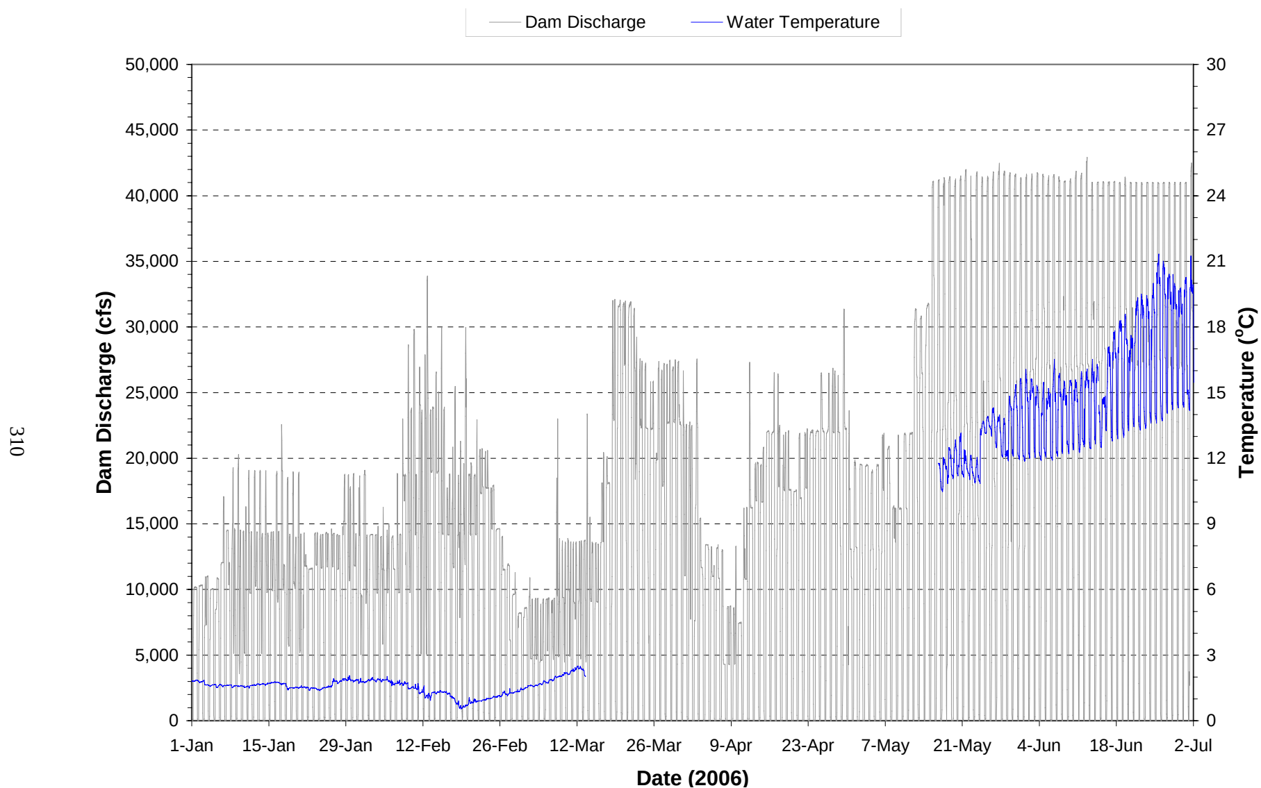
Plate 216. Hourly discharge and water temperature monitored at the Fort Randall powerplant on water discharged through the dam during the period January through June 2006. (Note: Gaps in temperature plot represents periods when monitoring equipment was not operational.)
