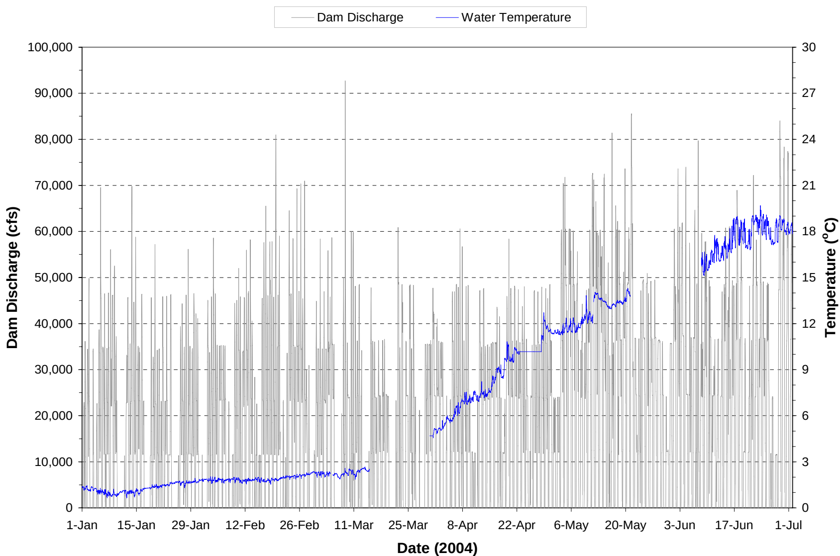
Plate 167. Hourly discharge and water temperature monitored at the Big Bend powerplant on water discharged through the dam during the period January through June 2004. (Note: Gaps in temperature plot represents periods when monitoring equipment was not operational.)
