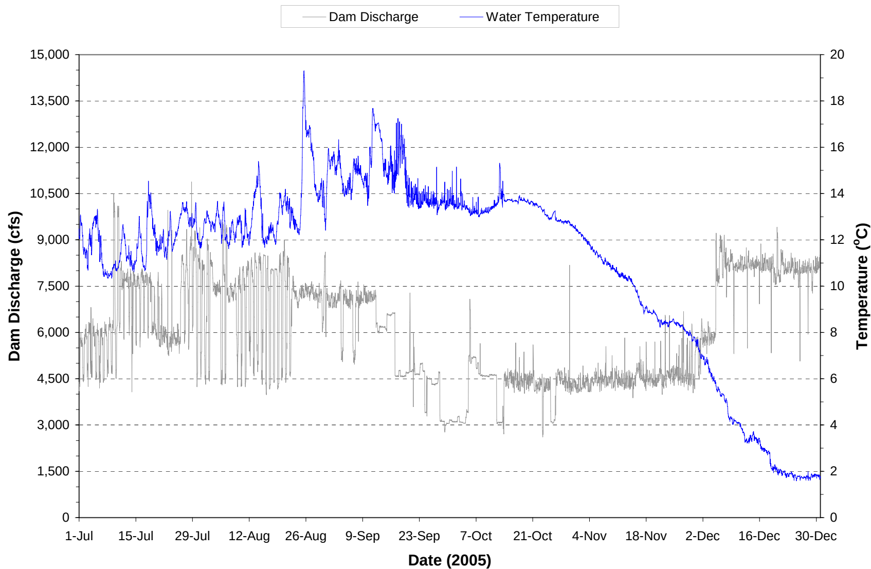
Plate 35. Hourly discharge and water temperature monitored at the Fort Peck powerplant on water discharged through the dam during the period July through December 2005.
