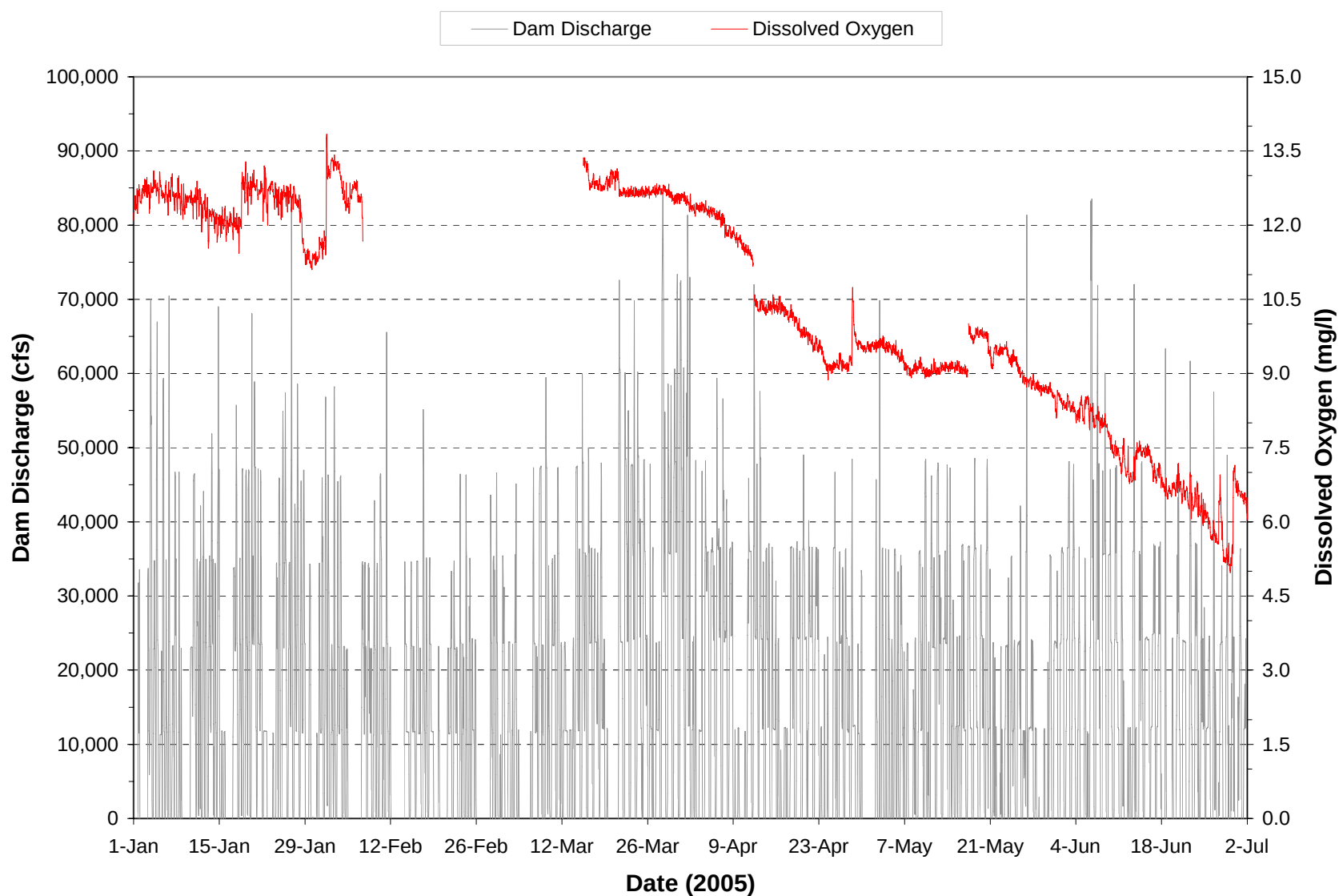
Plate 175. Hourly discharge and dissolved oxygen concentrations monitored at the Big Bend powerplant on water discharged through the dam during the period January through June 2005. (Note: Gaps in dissolved oxygen plot represents periods when monitoring equipment was not operational.)
