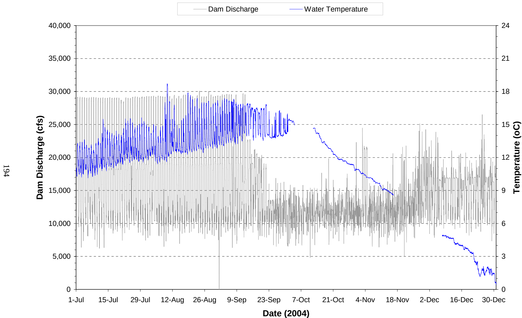
Plate 91. Hourly discharge and water temperature monitored at the Garrison powerplant on water discharged through the dam during the period July through December 2004. (Note: Gaps in temperature plot represents periods when monitoring equipment was not operational.)
