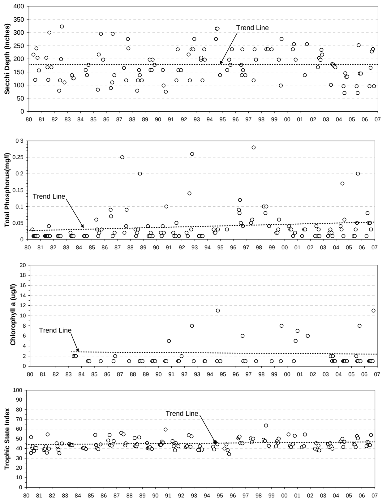
Plate 138. Historic trends for Secchi depth, total phosphorus, chlorophyll a , and Trophic State Index (TSI) monitored in Oahe Reservoir at the near-dam, ambient site (i.e., site OAHLK1073A) over the 27-year period of 1980 to 2006.
