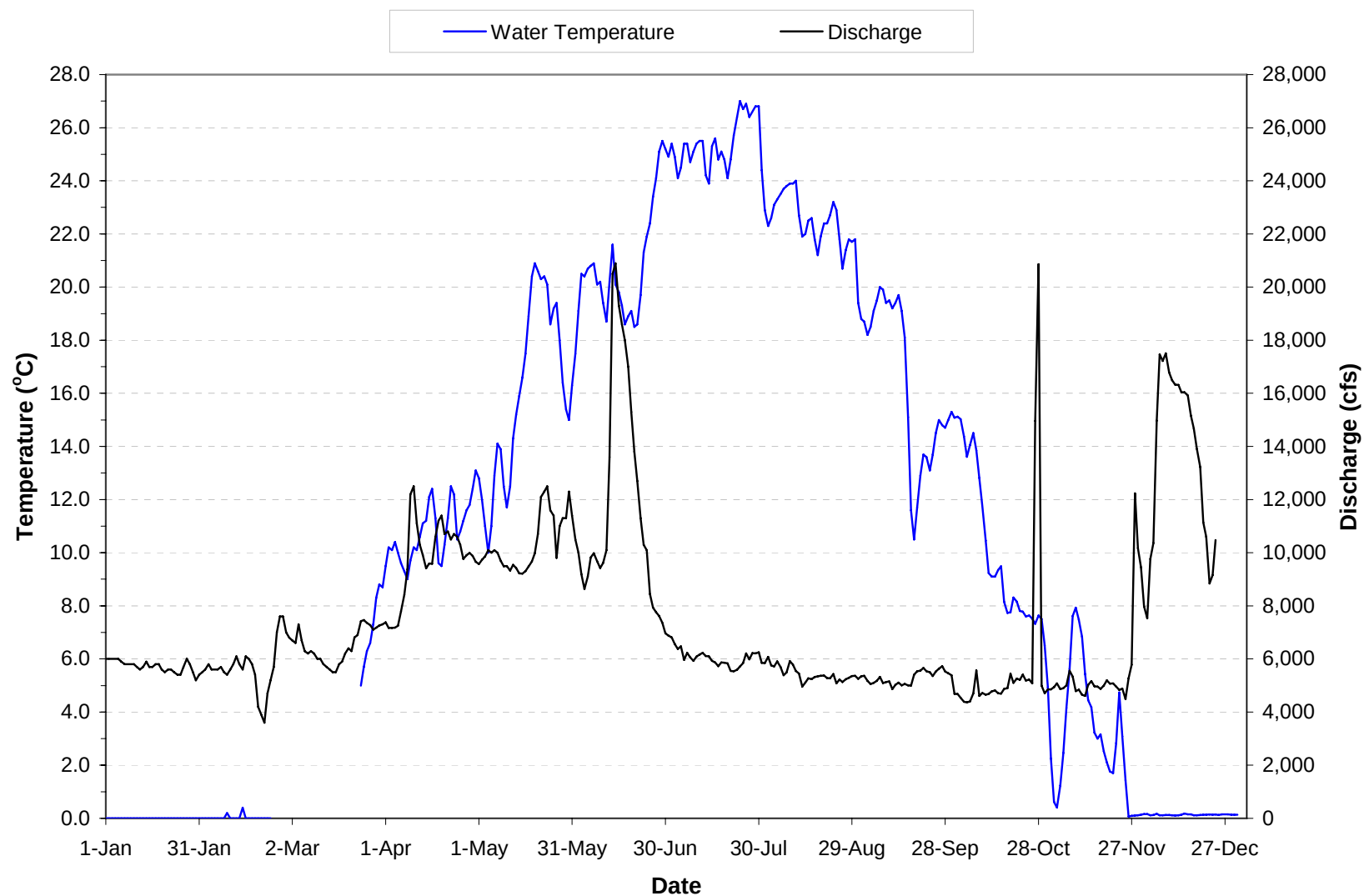
Plate 30. Mean daily water temperature and discharge of the Missouri River near Landusky, Montana (i.e., site FTPNFMORR1) for 2006. Means based on hourly measurements recorded at USGS gaging station 06115200. (Note: data are provisional.)
