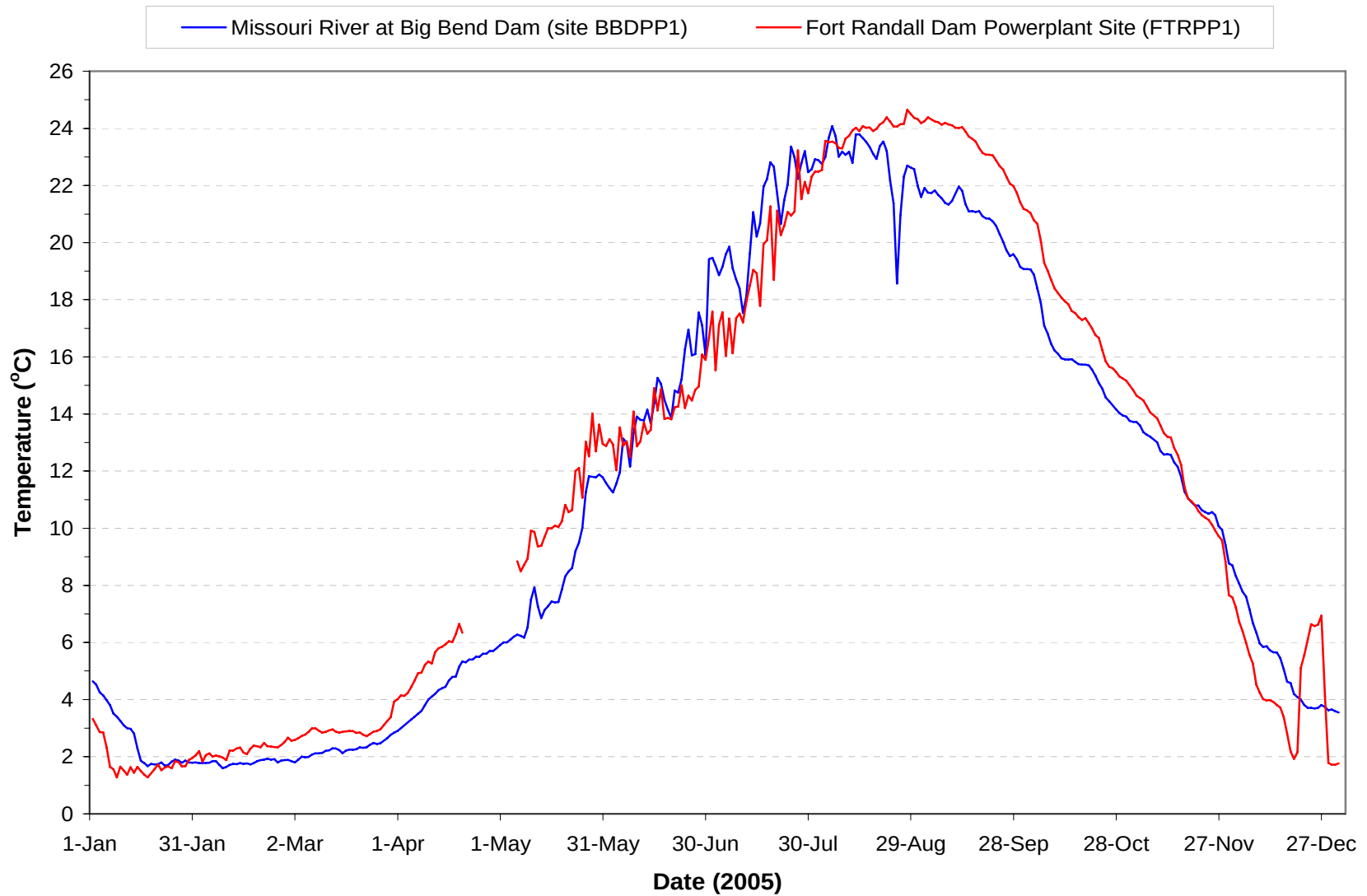
Plate 224. Mean daily water temperatures monitored at the Fort Randall Powerplant (i.e., site FTRPP1) and the Missouri River at Big Bend Dam (i.e., site BBDPP1) during 2005. (Note: Gaps in temperature plots are periods when monitoring equipment was not operational.)
