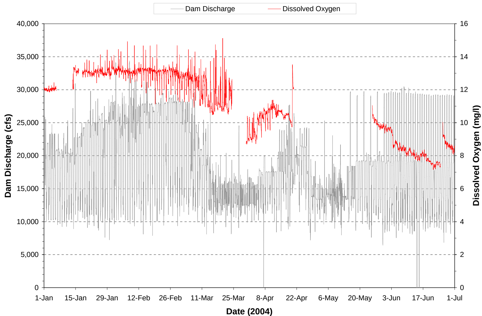
Plate 98. Hourly discharge and dissolved oxygen monitored at the Garrison powerplant on water discharged through the dam during the period January through June 2004. (Note: Gaps in dissolved plot represents periods when monitoring equipment was not operational.)
