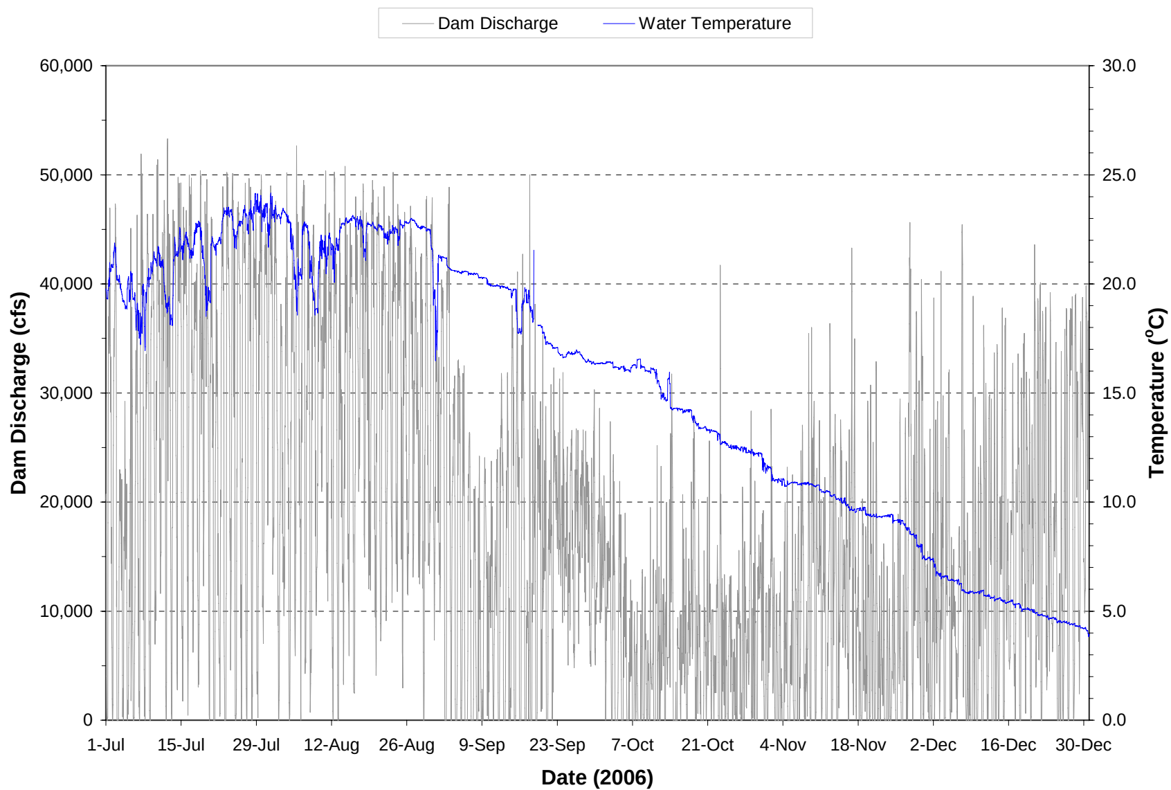
Plate 148. Hourly discharge and water temperature monitored at the Oahe powerplant on water discharged through the dam during the period July through December 2006.
