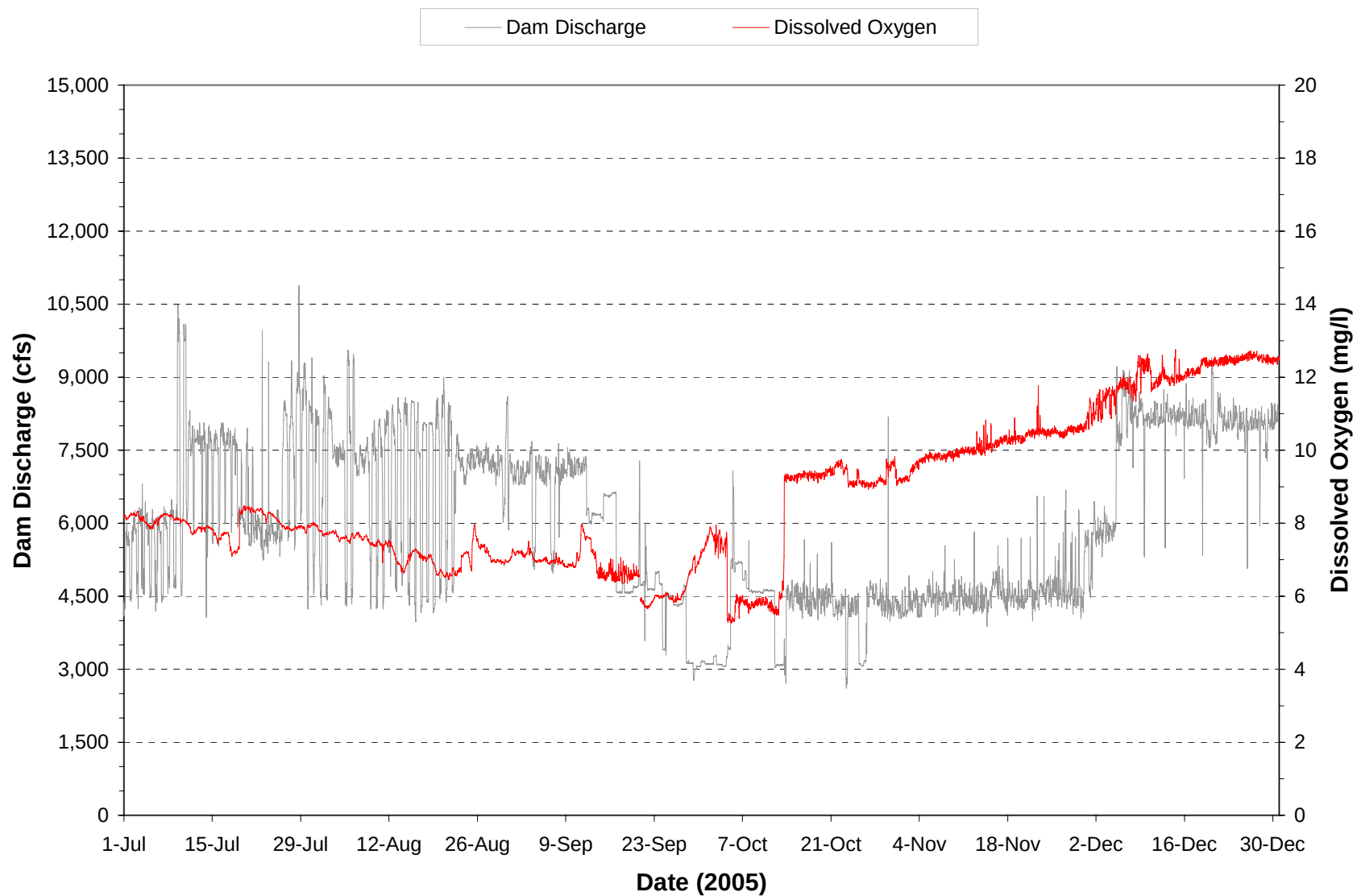
Plate 41. Hourly discharge and dissolved oxygen monitored at the Fort Peck powerplant on water discharged through the dam during the period July through December 2005.
