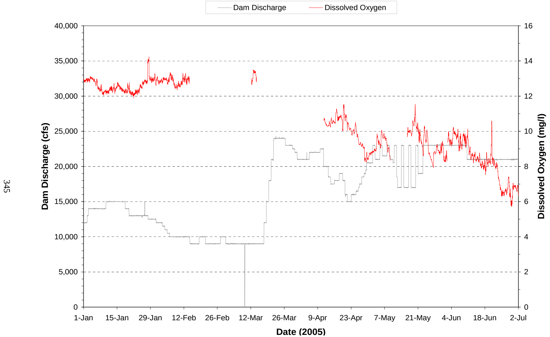
Plate 251. Hourly discharge and dissolved oxygen monitored at the Gavins Point powerplant on water discharged through the dam during the period January through June 2005. (Note: Gaps in temperature plot represents periods when monitoring equipment was not operational.)
