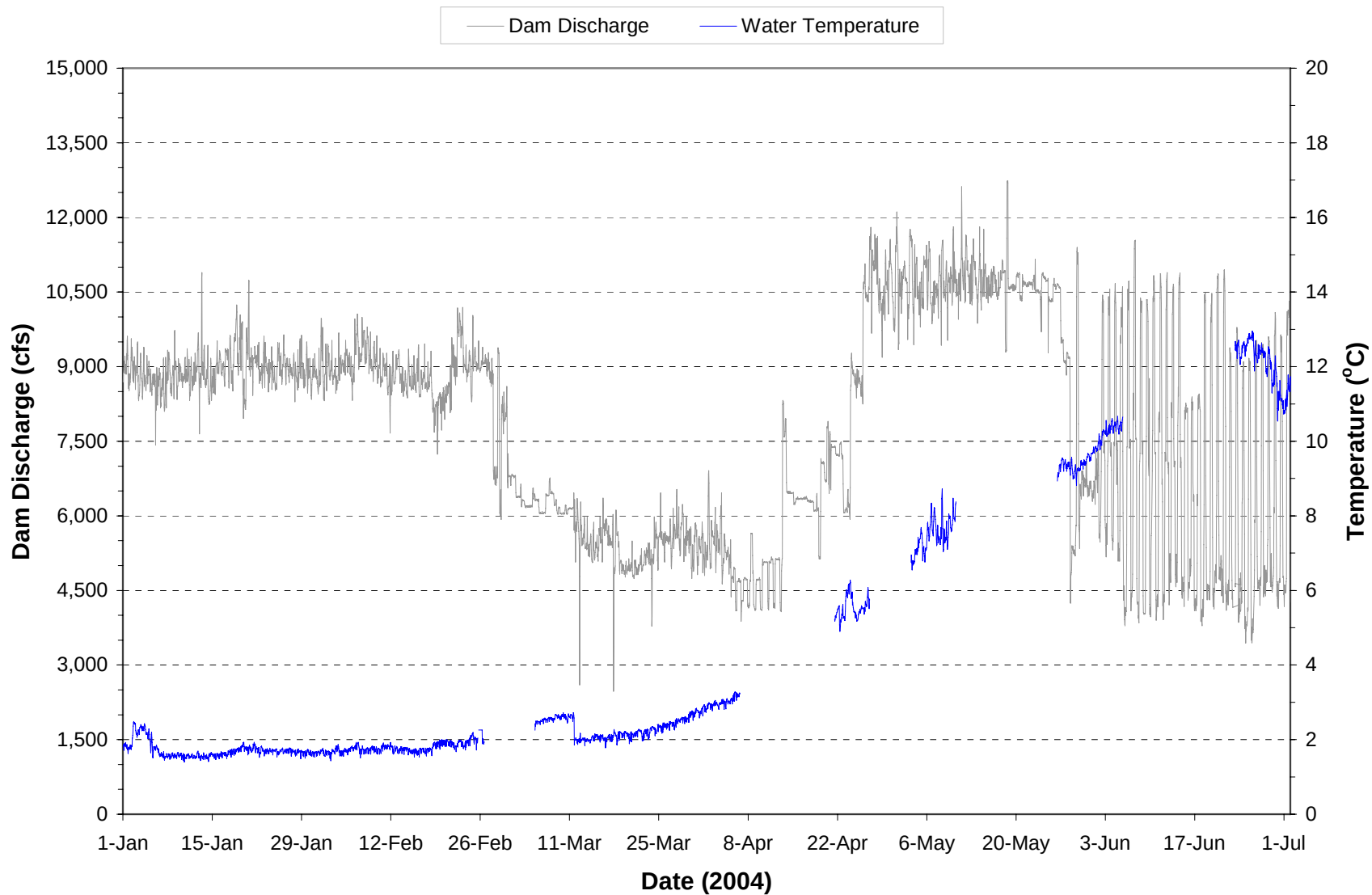
Plate 32. Hourly discharge and water temperature monitored at the Fort Peck powerplant on water discharged through the dam during the period January through June 2004. (Note: Gaps in temperature plot represents periods when monitoring equipment was not operational.)
