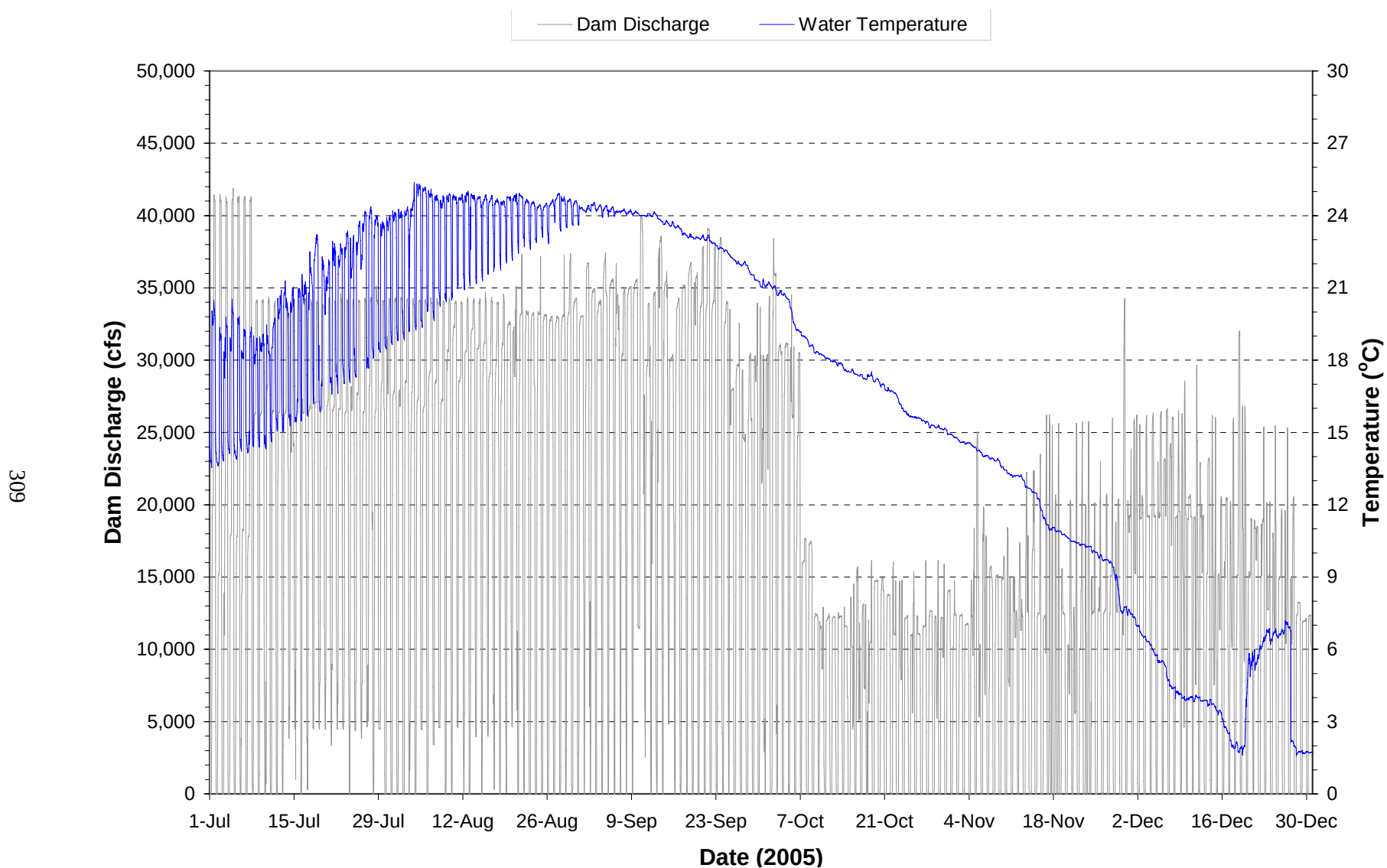
Plate 215. Hourly discharge and water temperature monitored at the Fort Randall powerplant on water discharged through the dam during the period July through December 2005.
