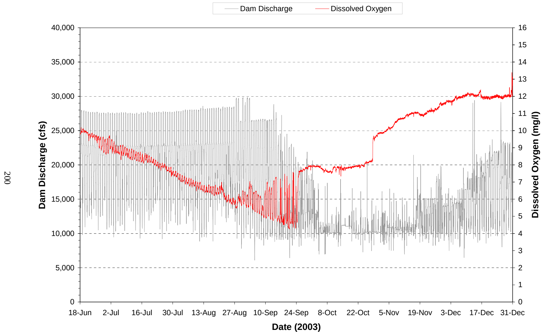
Plate 97. Hourly discharge and dissolved oxygen monitored at the Garrison powerplant on water discharged through the dam during the period June through December 2003.
