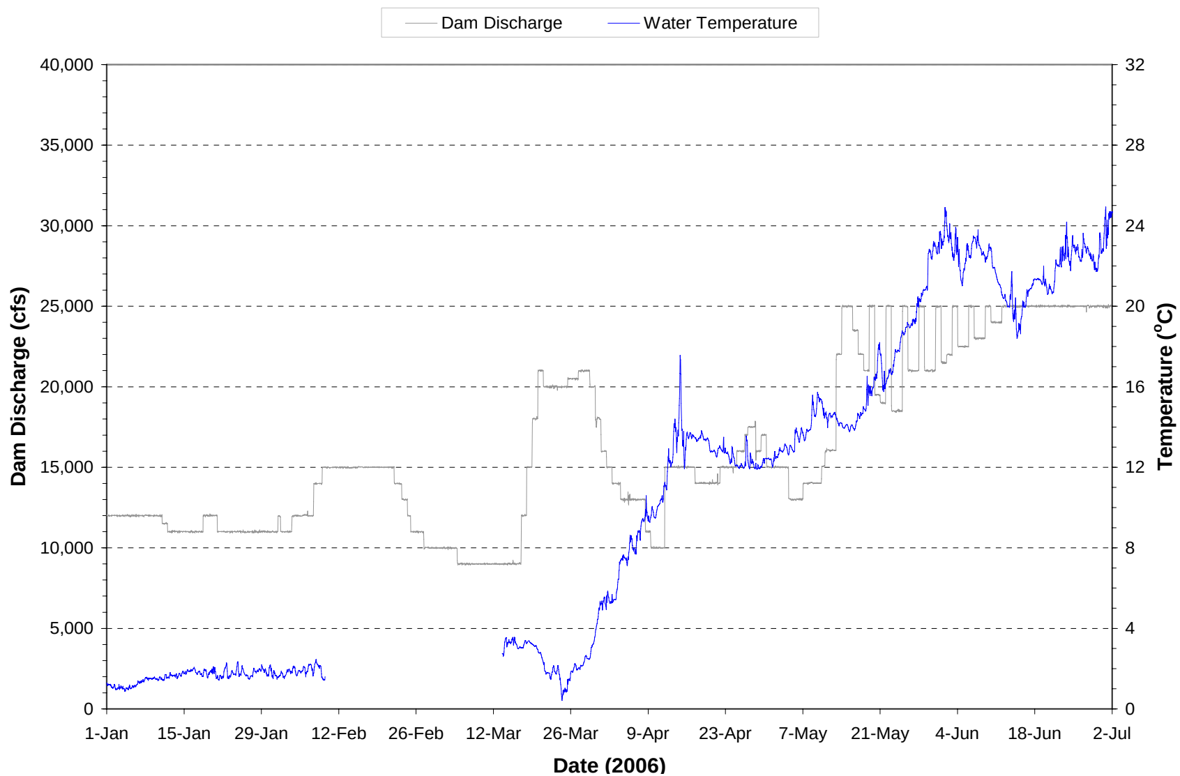
Plate 247. Hourly discharge and water temperature monitored at the Gavins Point powerplant on water discharged through the dam during the period January through June 2006. (Note: Gaps in temperature plot represents periods when monitoring equipment was not operational.)
