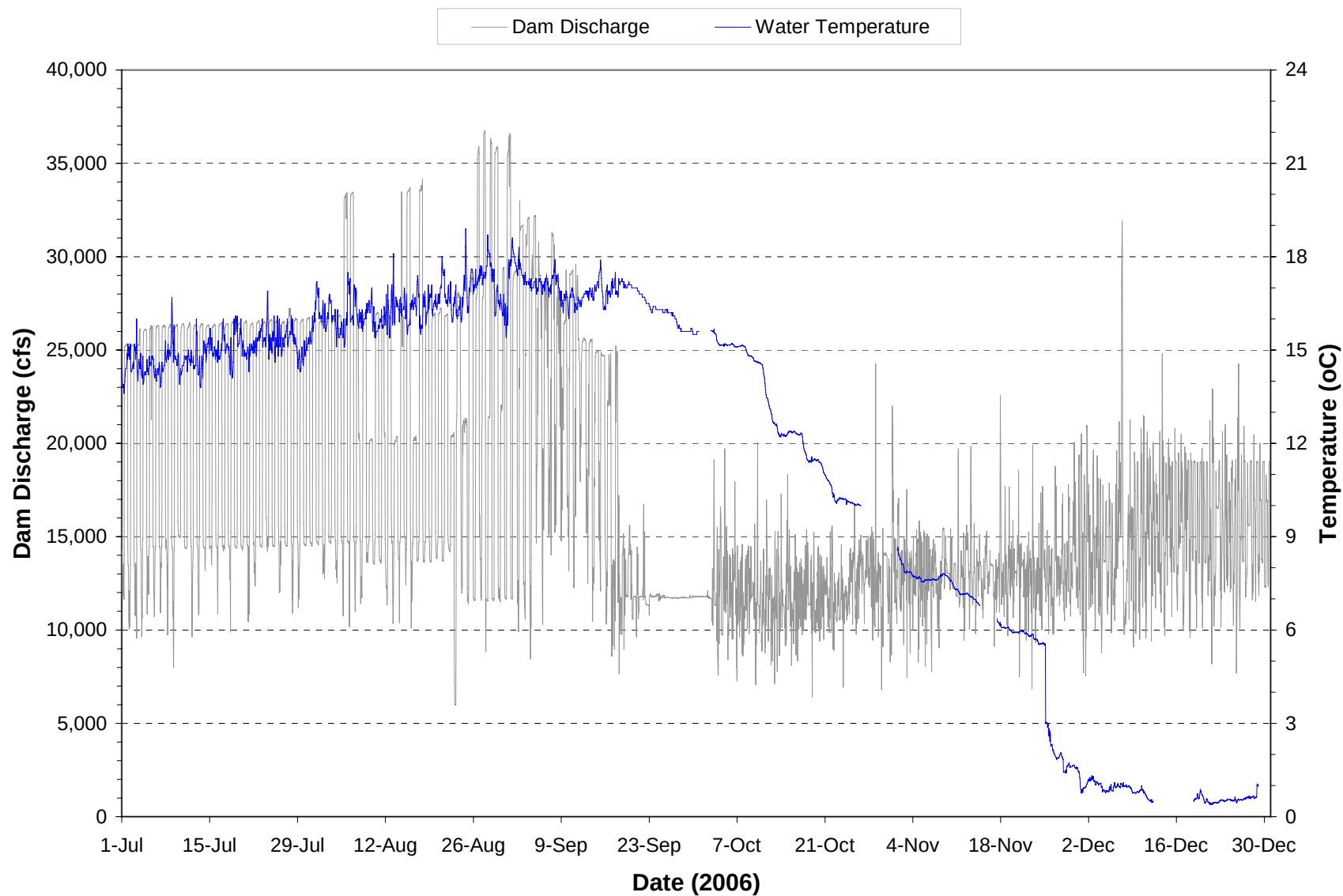
Plate 95. Hourly discharge and water temperature monitored at the Garrison powerplant on water discharged through the dam during the period July through December 2006. (Note: Gaps in temperature plot represents periods when monitoring equipment was not operational.)
