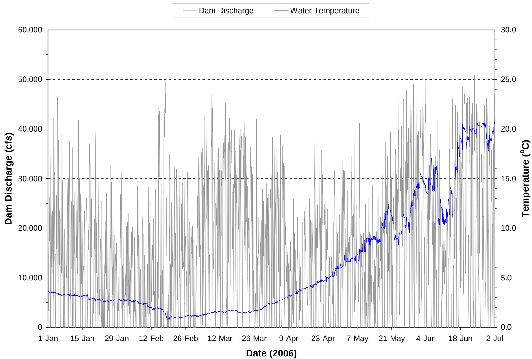
Plate 147. Hourly discharge and water temperature monitored at the Oahe powerplant on water discharged through the dam during the period January through June 2006.
