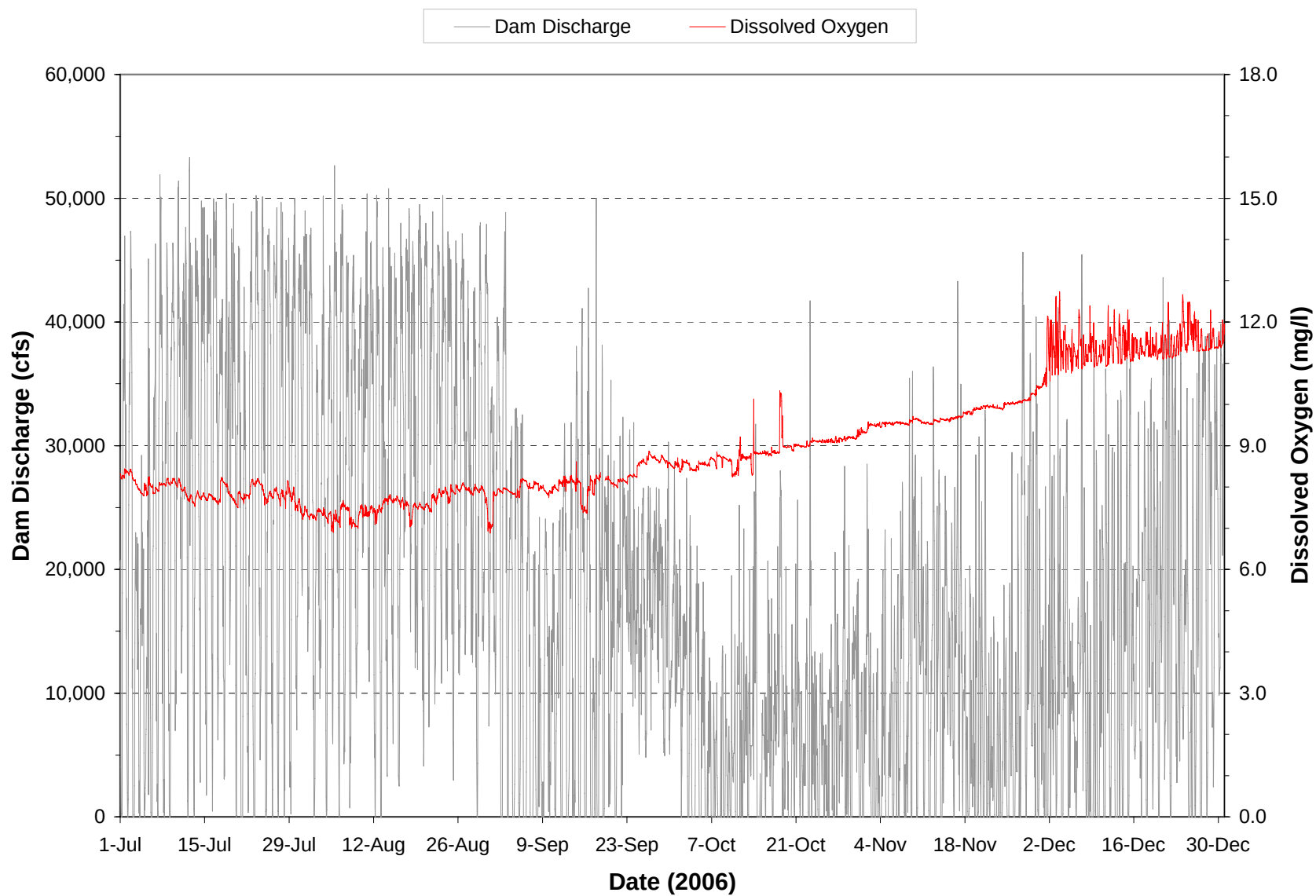
Plate 154. Hourly discharge and dissolved oxygen monitored at the Oahe Powerplant on water discharged through the dam during the period July through December 2006. (Note: Gaps in dissolved oxygen plot represents periods when monitoring equipment was not operational.)
