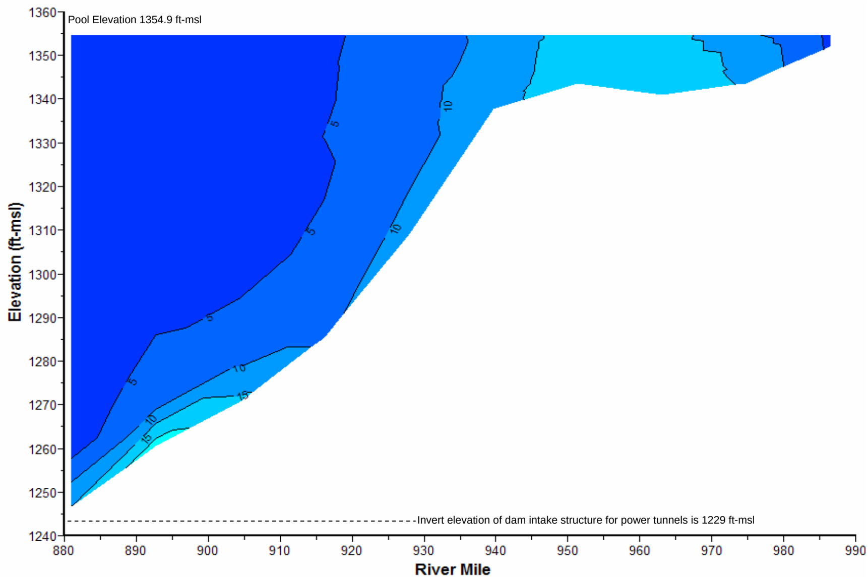
Plate 199. Longitudinal turbidity (NTU) contour plot of Fort Randall Reservoir based on depth-profile dissolved oxygen concentrations measured at sites FTRLK0880A, FTRLK0892DW, FTRLK0911DW, FTRLK0924DW, FTRLK0940DW, FTRLK0955DW, FTRLK0968DW, and BBDPP1 on July 20, 2006.
