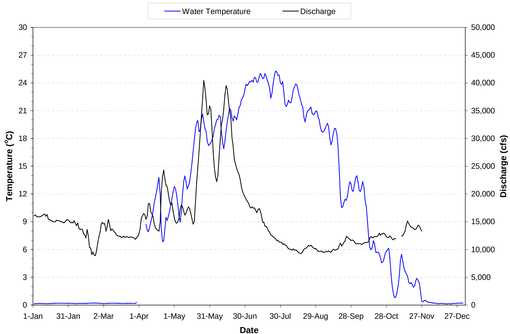
Plate 86. Mean daily water temperature and discharge of the Missouri River near Williston, North Dakota (i.e., site GARNFMORRR1) for 2006. Mean temperatures based on hourly measurements recorded on the Missouri River near Williston, North Dakota (USGS gaging station 06330000). Mean daily discharge estimated by adding mean daily discharge recorded for the Missouri River near Culbertson, Montana (USGS gaging station 06185500) and the mean daily discharge recorded for the Yellowstone River near Sidney, Montana (USGS gaging station 06329500).
