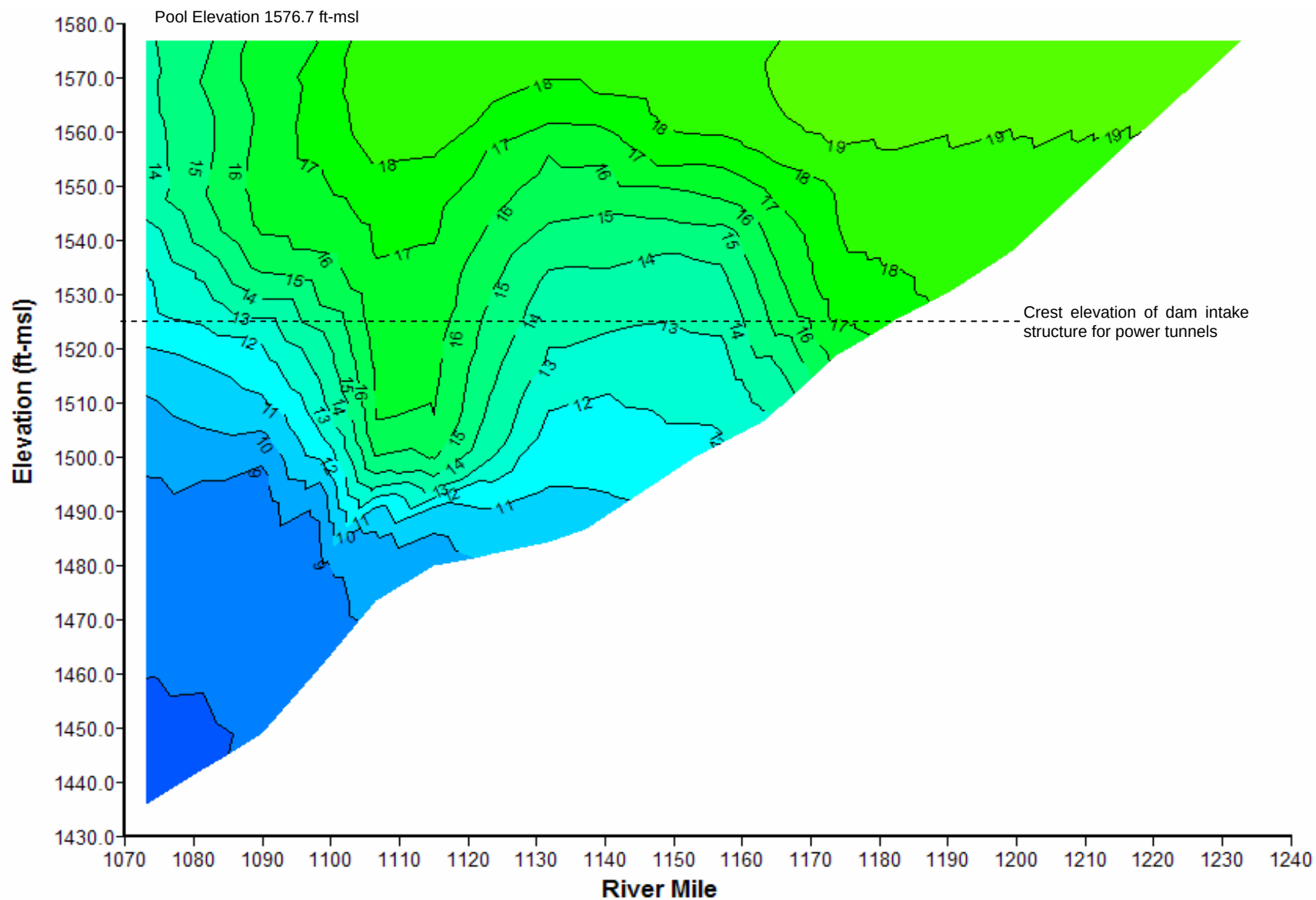
Plate 118. Longitudinal temperature ( ^{\circ}\text{C} ) contour plot of Oahe Reservoir based on depth-profile water temperatures measured at sites OAHRLK1073A, OAHLK1090DW, OAHLK1110DW, OAHLK1135DW, OAHLK1153DW, OAHLK1176DW, OAHLK1196DW and OAHNFMORR1 on June 14, 2006.
