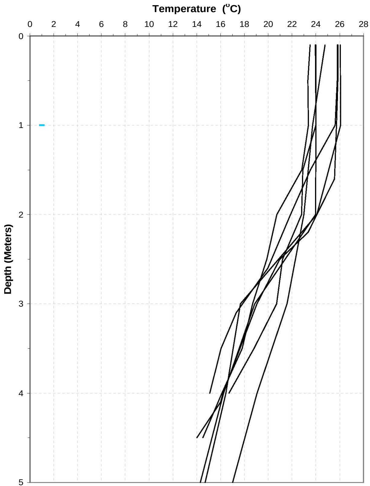
Plate 276. Temperature depth profiles for Lake Yankton generated from data collected at the deepwater ambient monitoring site during the months of June, July, August, and September during 2002 and 2006.
