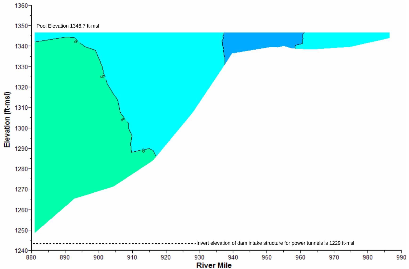
Plate 196. Longitudinal dissolved oxygen (mg/l) contour plot of Fort Randall Reservoir based on depth-profile dissolved oxygen concentrations measured at sites FTRLK0880A, FTRLK0892DW, FTRLK0911DW, FTRLK0924DW, FTRLK0940DW, FTRLK0955DW, FTRLK0968DW, and BBDPP1 on September 21, 2006.
