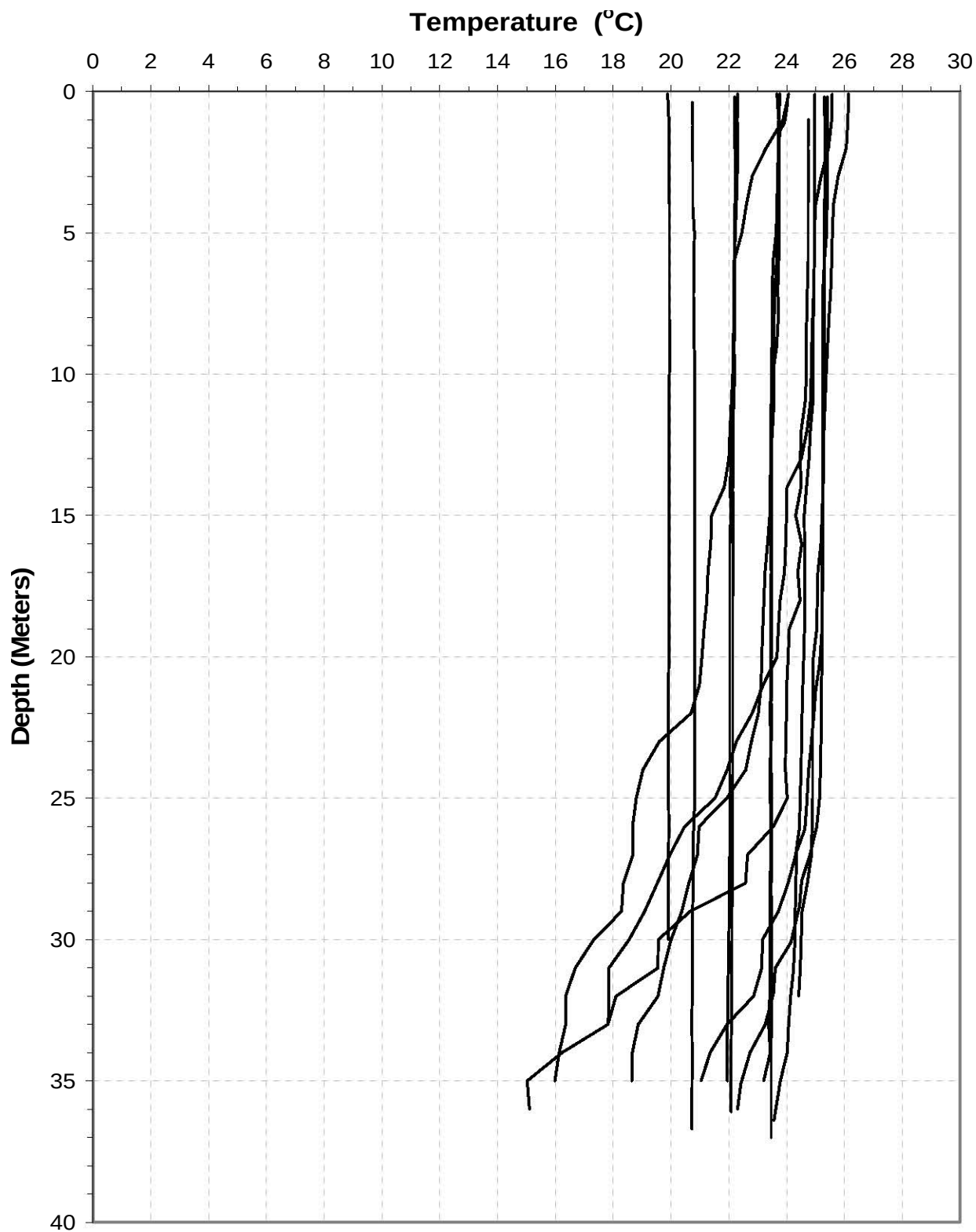
Plate 192. Temperature depth profiles for Fort Randall Reservoir generated from data collected at the near-dam, deepwater ambient monitoring site (i.e., site FTRLK0880A) during the months of July, August, and September over the 5-year period of 2002 to 2006.
