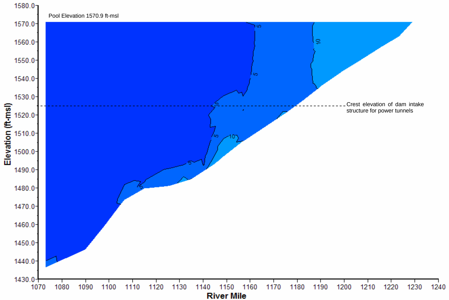
Plate 130. Longitudinal turbidity (NTU) contour plot of Oahe Reservoir based on depth-profile turbidity levels measured at sites OAHRLK1073A, OAHLK1090DW, OAHLK1110DW, OAHLK1135DW, OAHLK1153DW, OAHLK1176DW, OAHLK1196DW and OAHNFMORR1 on August 23, 2006.
