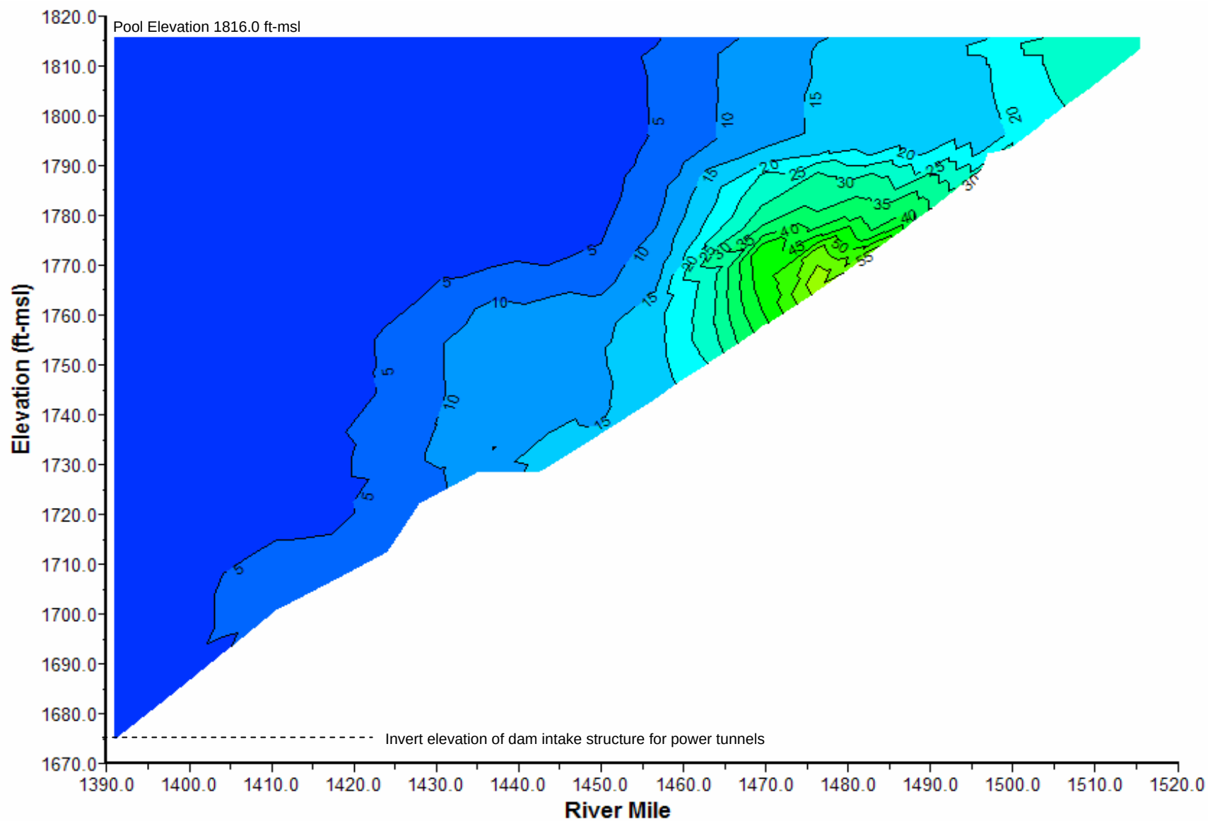
Plate 73. Longitudinal turbidity (NTU) contour plot of Garrison Reservoir based on depth-profile turbidity levels monitored at sites GARLK1390A, GARLK1412DW, GARLK1445DW, GARLK1481DW, and GARNFMORRR1 on July 25, 2006.
