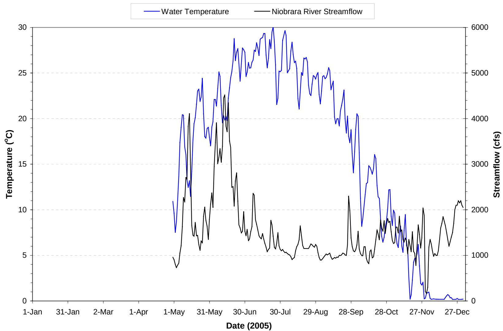
Plate 238. Mean daily water temperature and streamflow of the Niobrara River near Verdel, Nebraska (i.e., site USGS 06465500) for 2005. Mean daily temperatures and streamflows based on hourly measurements recorded at the USGS gaging station.
