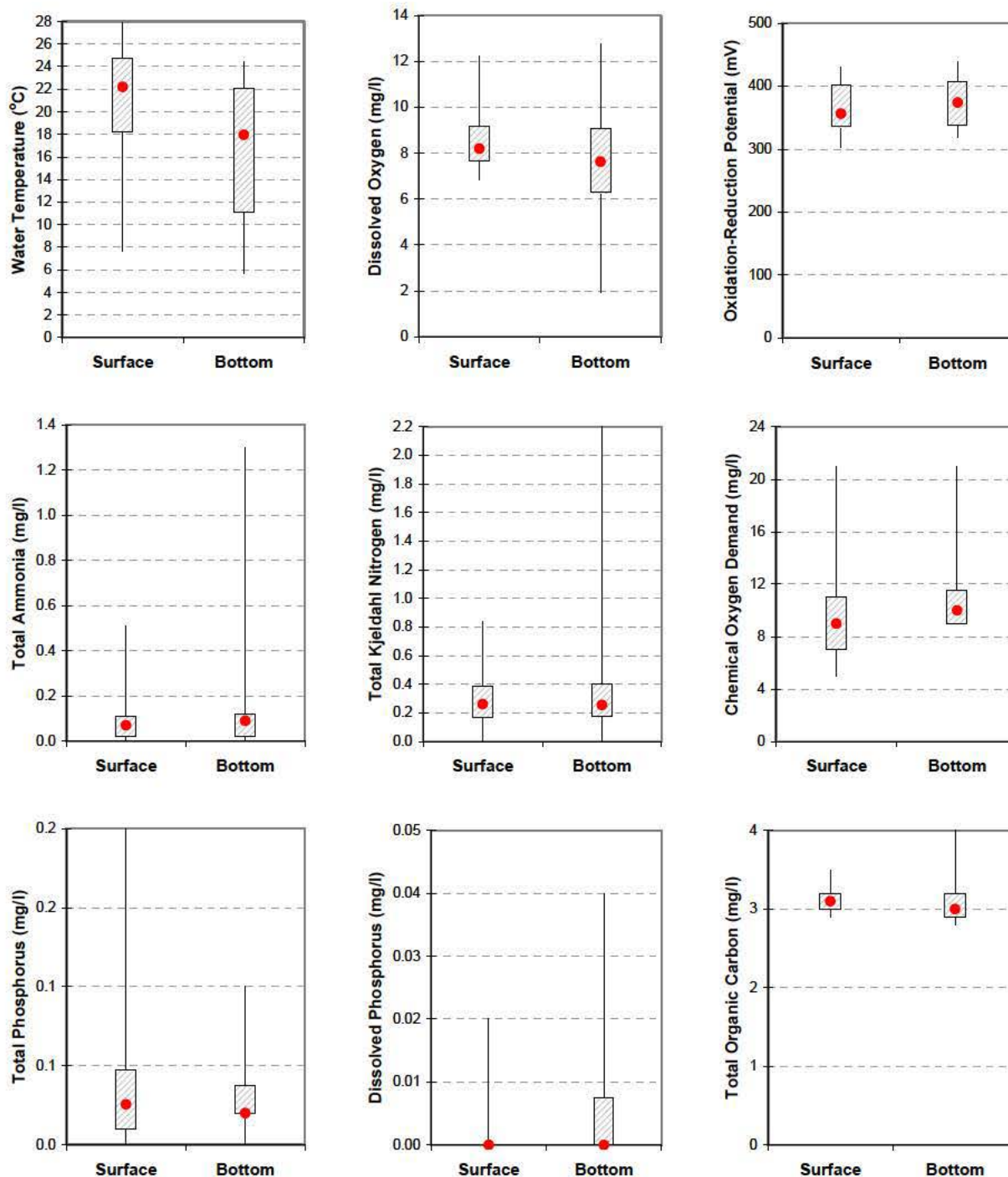
Plate 202. Box plots comparing surface and bottom water temperature, dissolved oxygen, oxidation-reduction potential, total Kjeldahl nitrogen, total ammonia nitrogen, chemical oxygen demand, total phosphorus, dissolved phosphorus, and total organic carbon measured in Fort Randall Reservoir at site FTRLK0880A during the summer months of 2002 through 2006. (Box plots display minimum, 25 th percentile, 75 th percentile, and maximum. Median value is indicated by the red dot. Non-overlapping interquartile ranges of the adjacent box plots indicate a significant difference between surface and bottom measurements.)
