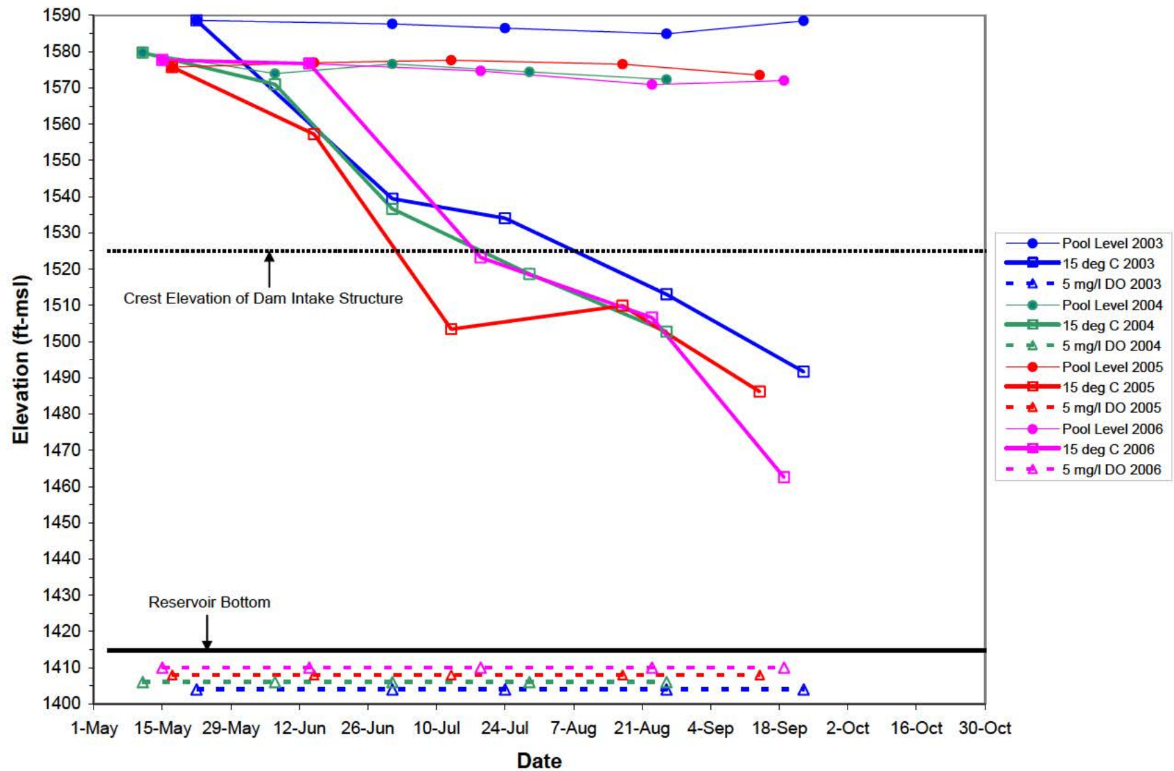
Plate 262. Elevation of the 15°C water temperature and 5 mg/l dissolved oxygen concentration isopleths for Oahe Reservoir based on water quality conditions monitored at a near-dam, deepwater location during 2003 through 2006. (Also shown are the reservoir pool elevation and the lower elevation of water withdrawal from the reservoir for power production.)
