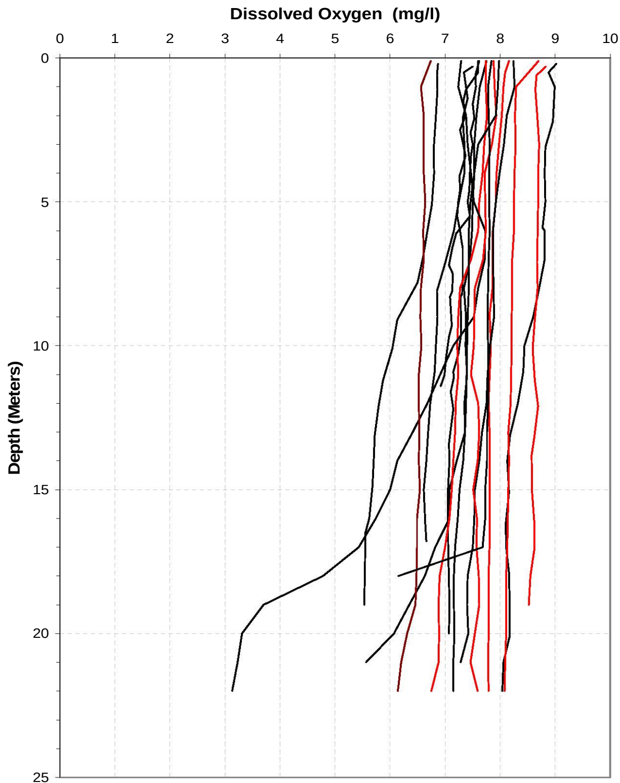
Plate 159. Dissolved oxygen depth profiles for Big Bend Reservoir generated from data collected at the near-dam, deepwater ambient monitoring site during the months of July, August, and September over the 5-year period of 2002 to 2006. (Note: Red profile plots were measured in the month of September.)
