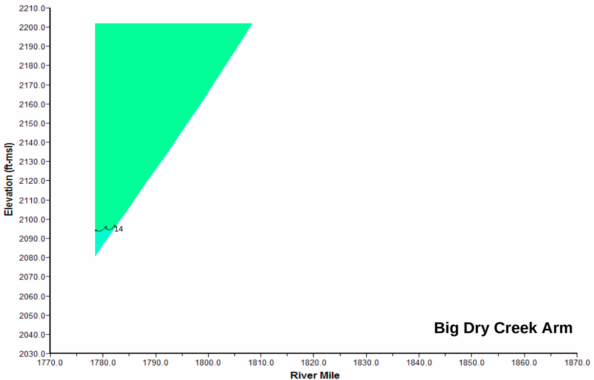
Plate 10. Longitudinal water temperature ( ^{\circ}\text{C} ) contour plot of Fort Peck Reservoir based on depth-profile water temperatures measured at sites FTPLK1772A, FTPLK1778DW, FTPLK1789DW, FTPLK1805DW, FTPLKBDCA01, FTPLKBDCA02, and FTPNFMORR1 on October 5, 2006.
