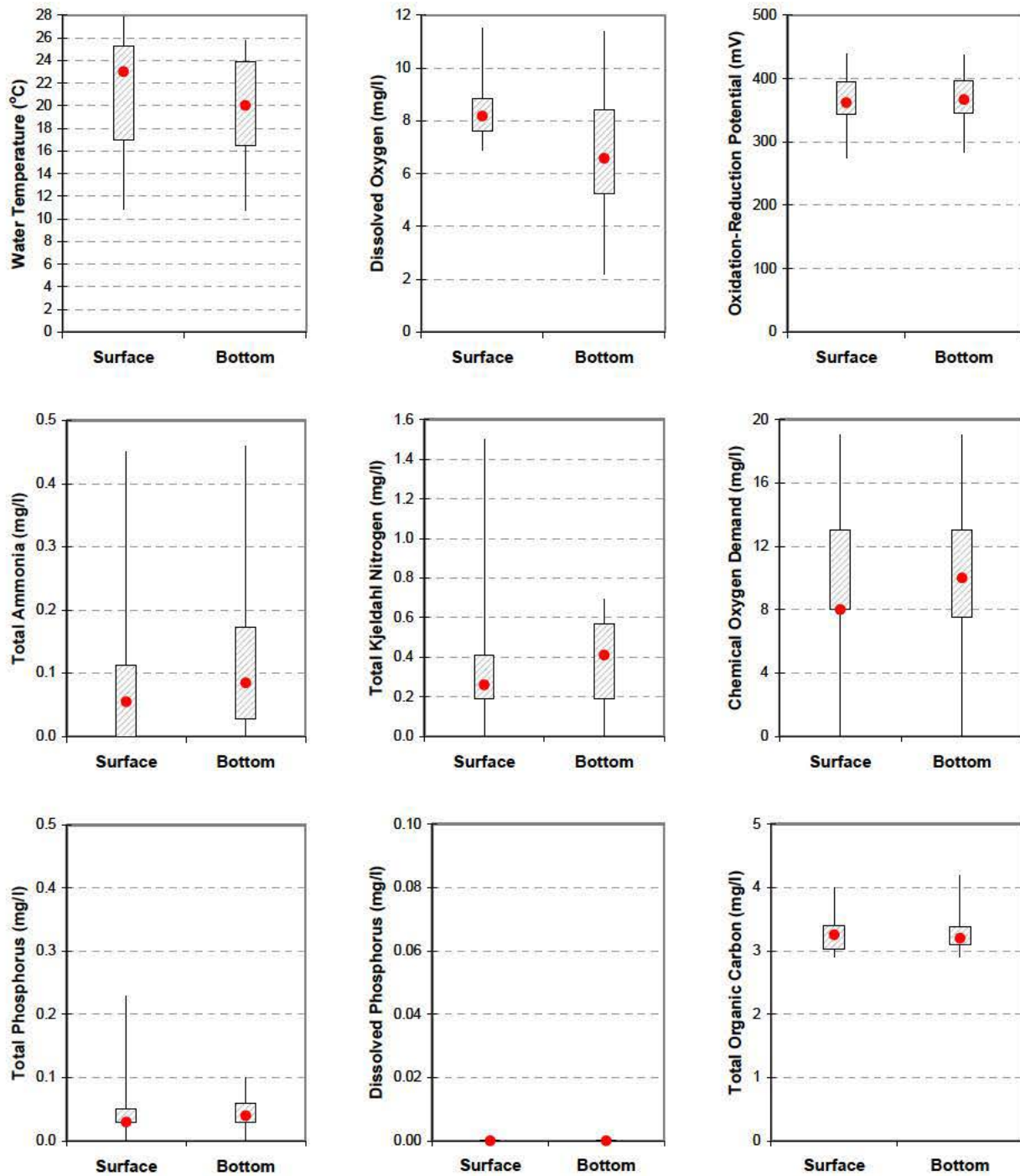
Plate 231. Box plots comparing surface and bottom water temperature, dissolved oxygen, oxidation-reduction potential, total Kjeldahl nitrogen, total ammonia nitrogen, chemical oxygen demand, total phosphorus, dissolved phosphorus, and total organic carbon measured in Gavins Point Reservoir at site GPTLK0811A during the summer months of 2002 through 2006. (Box plots display minimum, 25 th percentile, 75 th percentile, and maximum. Median value is indicated by the red dot. Non-overlapping interquartile ranges of the adjacent box plots indicate a significant difference between surface and bottom measurements.)
