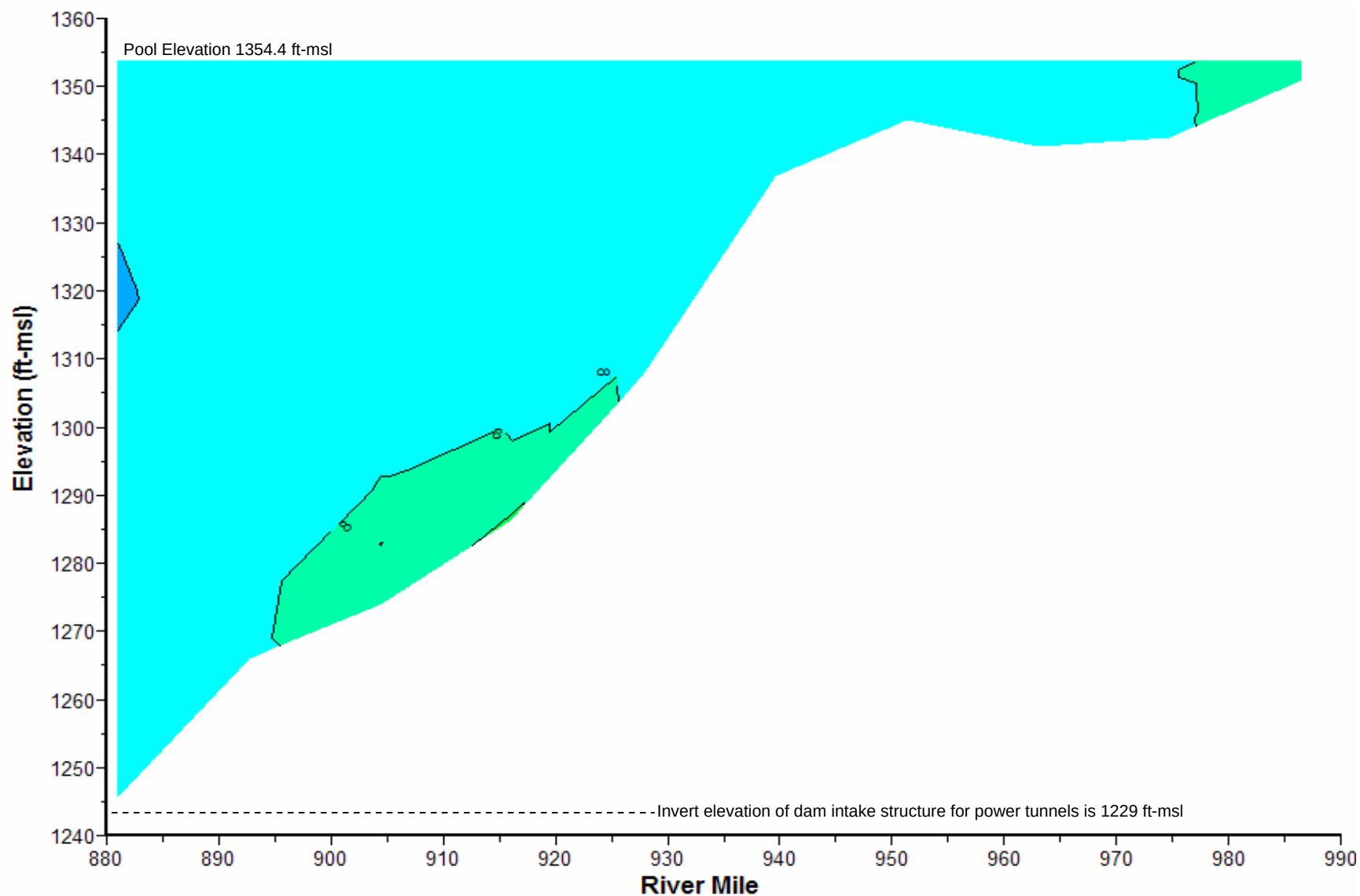
Plate 193. Longitudinal dissolved oxygen (mg/l) contour plot of Fort Randall Reservoir based on depth-profile dissolved oxygen concentrations measured at sites FTRLK0880A, FTRLK0892DW, FTRLK0911DW, FTRLK0924DW, FTRLK0940DW, FTRLK0955DW, FTRLK0968DW, and BBDPP1 on June 15, 2006.
