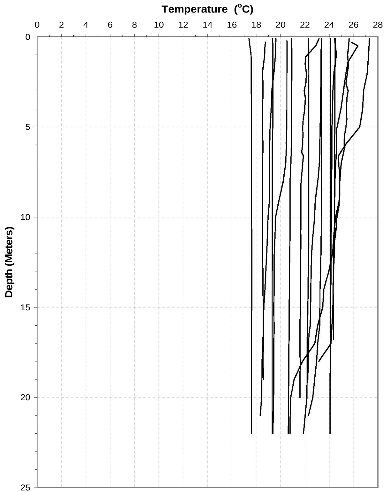
Plate 158. Temperature depth profiles for Big Bend Reservoir generated from data collected at the near-dam, deepwater ambient monitoring site during the months of July, August, and September over the 5-year period of 2002 to 2006.
