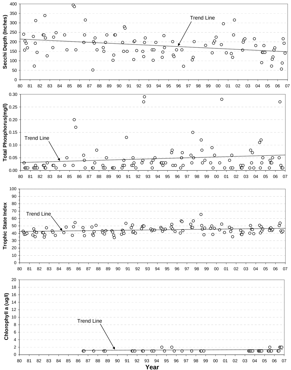
Plate 27. Historic trends for Secchi depth, total phosphorus, chlorophyll a , and Trophic State Index (TSI) monitored in Fort Peck Reservoir at the near-dam, ambient site (i.e., site FTPLK1772A) over the 27-year period of 1980 to 2006.
