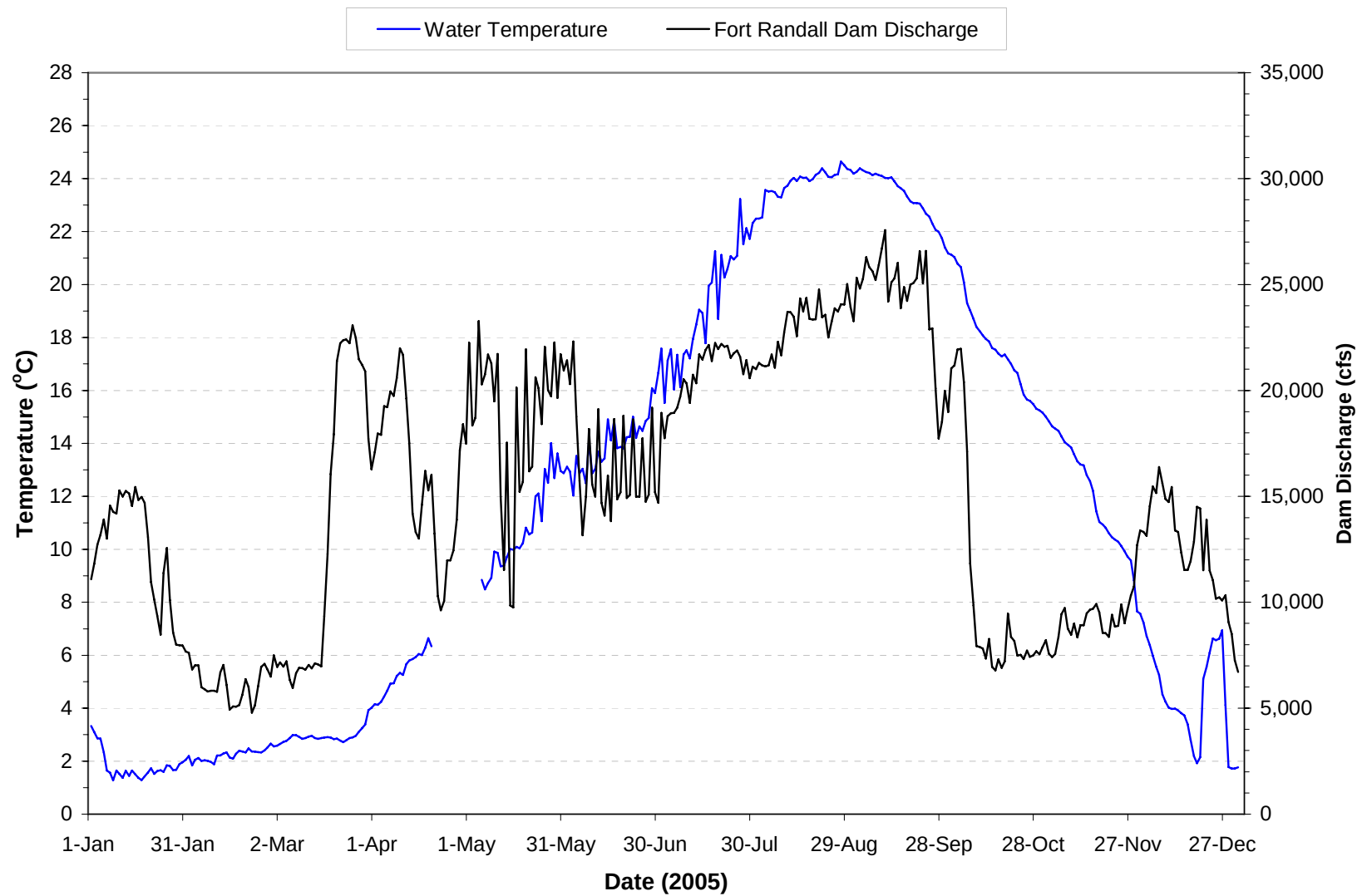
Plate 235. Mean daily water temperature and discharge of the Missouri River at Fort Randall Dam (i.e., site FTRPP1) for 2005. Mean daily temperatures and discharges based on hourly measurements recorded on discharge through Fort Randall Dam. (Note: Gaps in temperature plots are periods when monitoring equipment was not operational.)
