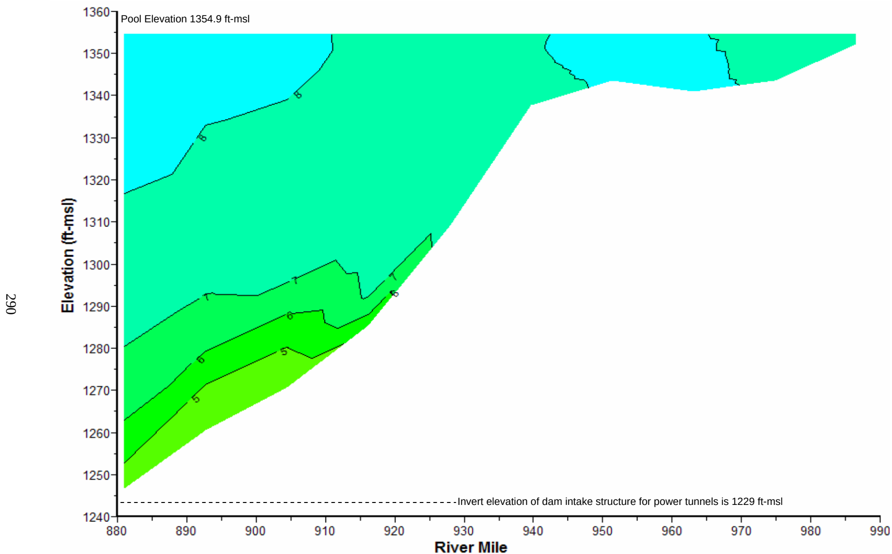
Plate 194. Longitudinal dissolved oxygen (mg/l) contour plot of Fort Randall Reservoir based on depth-profile dissolved oxygen concentrations measured at sites FTRLK0880A, FTRLK0892DW, FTRLK0911DW, FTRLK0924DW, FTRLK0940DW, FTRLK0955DW, FTRLK0968DW, and BBDPP1 on July 20, 2006.
