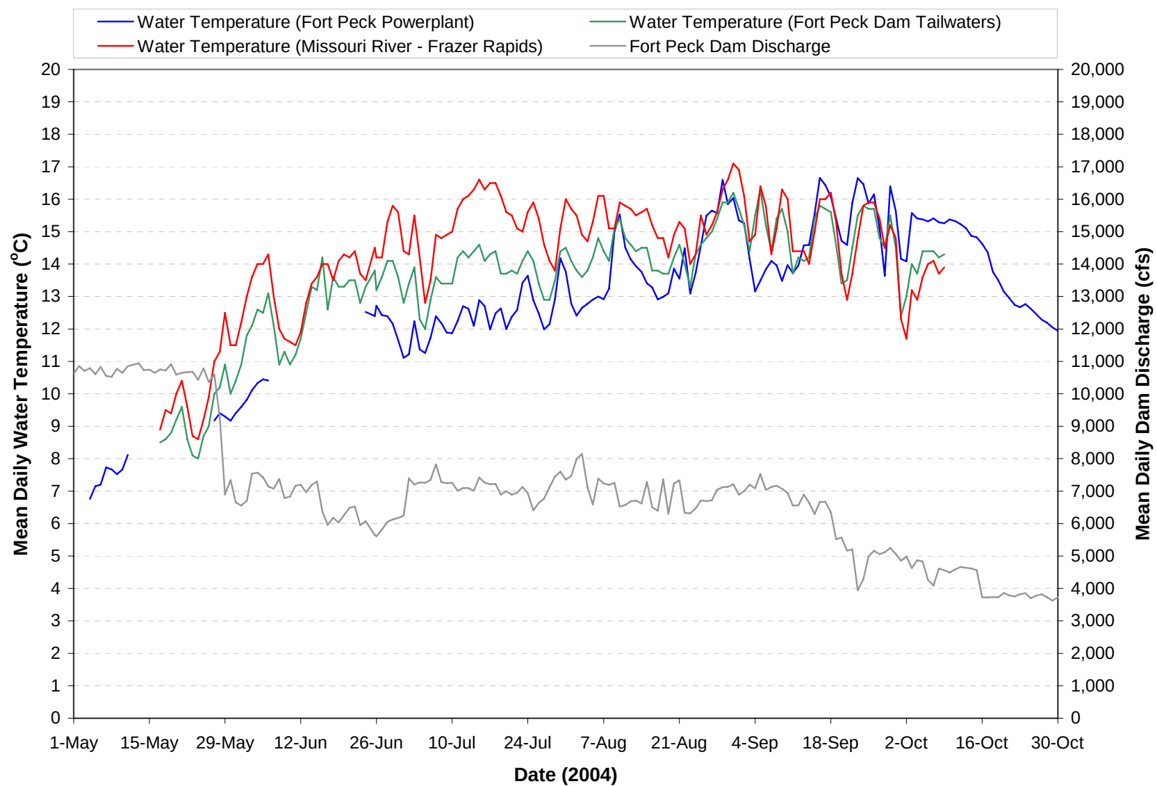
Plate 46. Mean daily water temperature monitored at the Fort Peck powerplant, Missouri River tailwaters, and Missouri River Frazer Rapids and the mean daily discharge of Fort Peck Dam from May through October during 2004.
