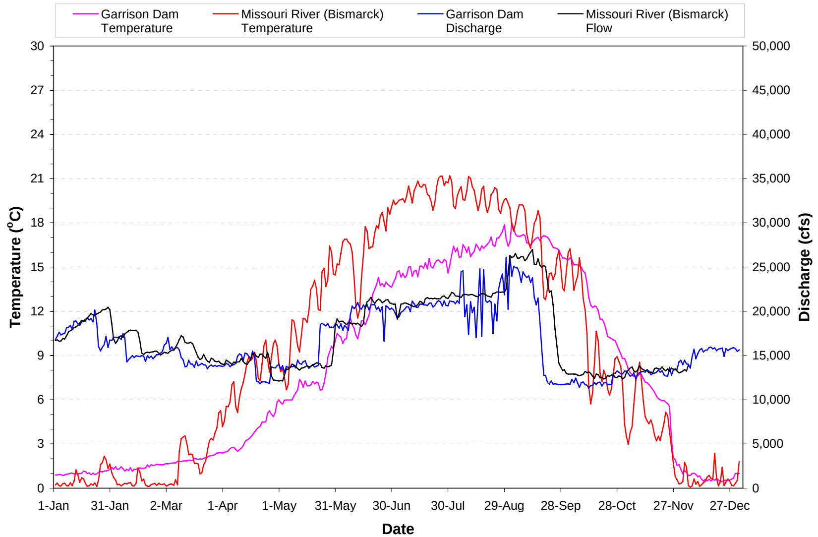
Plate 108. Mean daily water temperature and discharge for the Garrison Dam discharge and Missouri River at Bismarck, North Dakota for 2006. (Daily means based on hourly measurements.)
