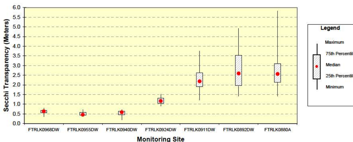
Figure 5.9. Box plot of Secchi transparencies measured in Fort Randall Reservoir during 2006. (Note: monitoring sites are oriented on the x-axis in an upstream to downstream direction.)
