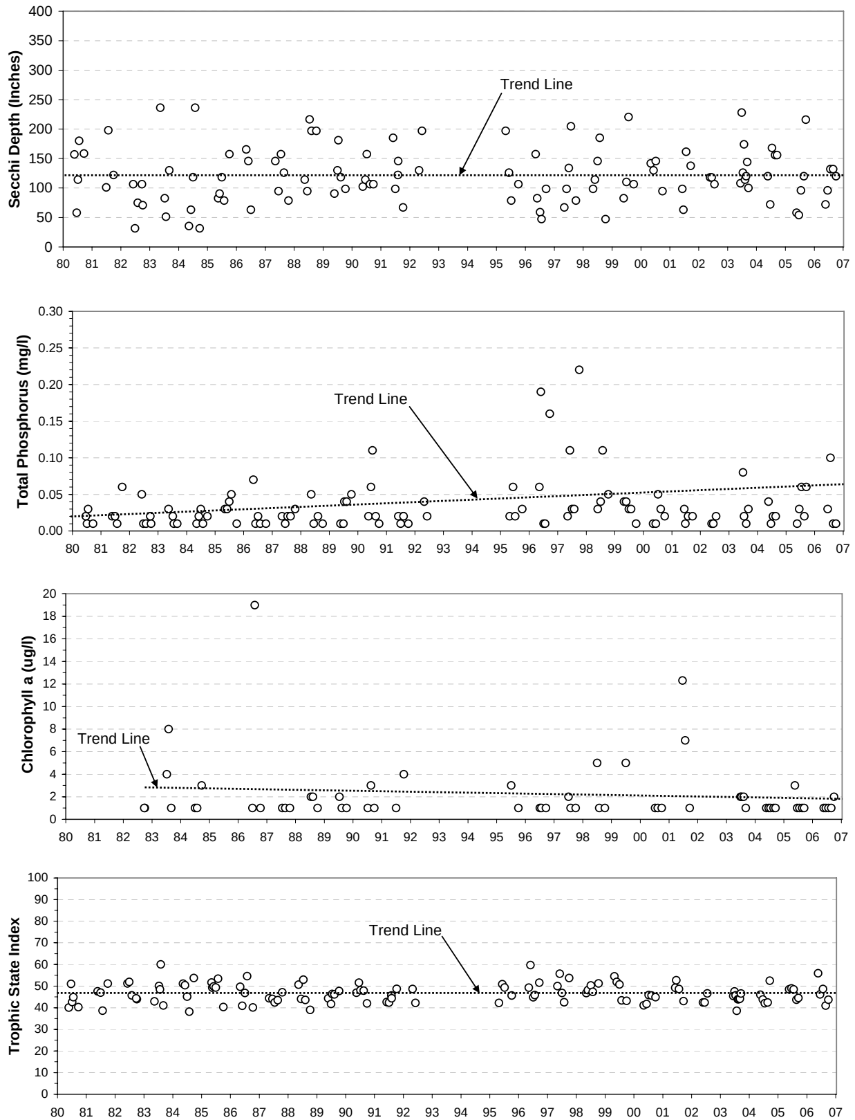
Plate 83. Historic trends for Secchi depth, total phosphorus, chlorophyll a , and Trophic State Index (TSI) monitored in Garrison Reservoir at the near-dam, ambient site (i.e., site GARLK1390A) over the 27-year period of 1980 to 2006.
