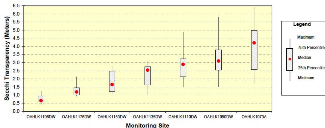
Figure 5.6. Box plot of Secchi transparencies measured in Oahe Reservoir during the period 2002 through 2006. (Note: monitoring sites are oriented on the x-axis in an upstream to downstream direction.)
