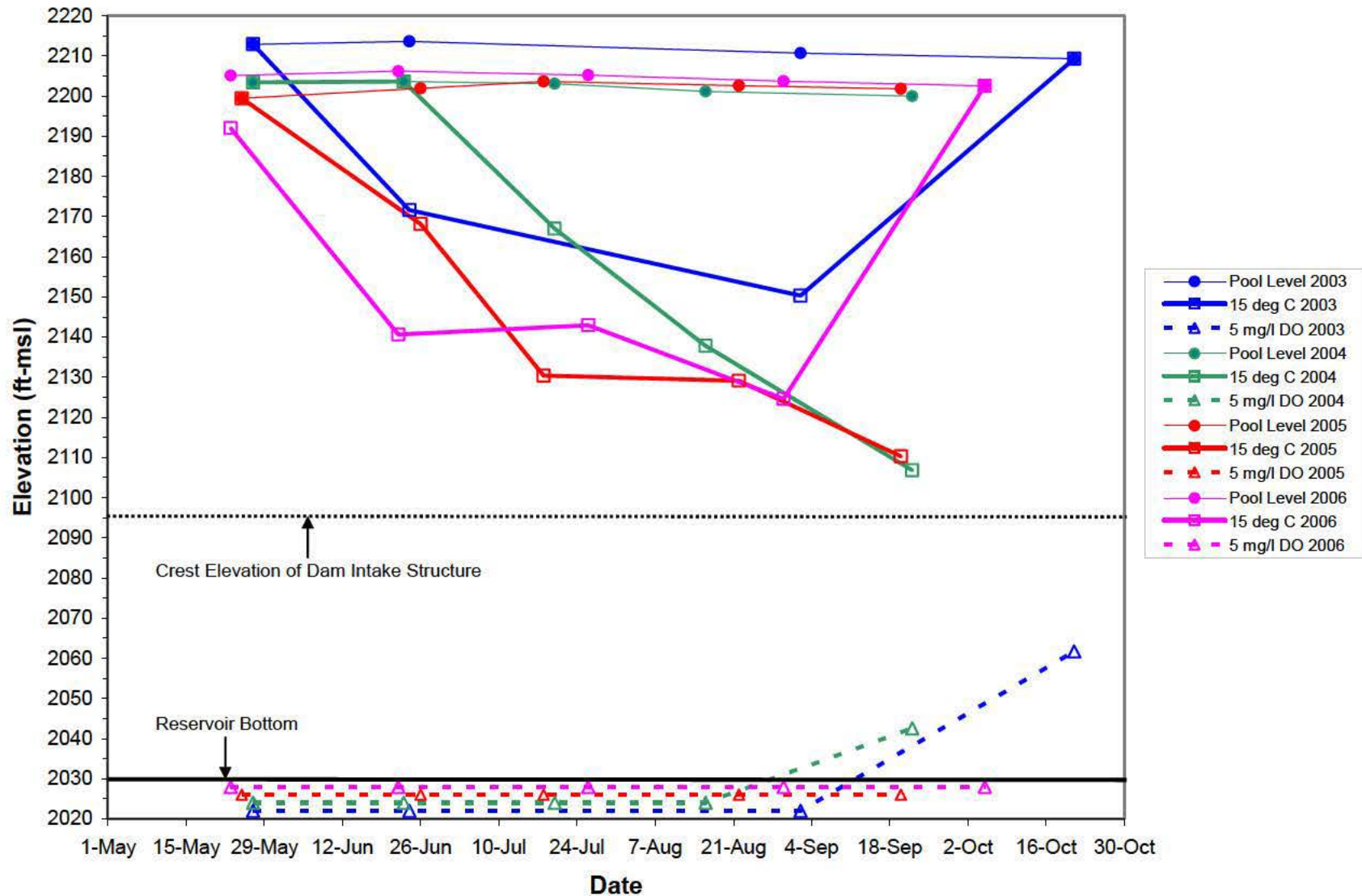
Plate 260. Elevation of the 15°C water temperature and 5 mg/l dissolved oxygen concentration isopleths for Fort Peck Reservoir based on water quality conditions monitored at a near-dam, deepwater location during 2003 through 2006. (Also shown are the reservoir pool elevation and the lower elevation of water withdrawal from the reservoir for power production.)
