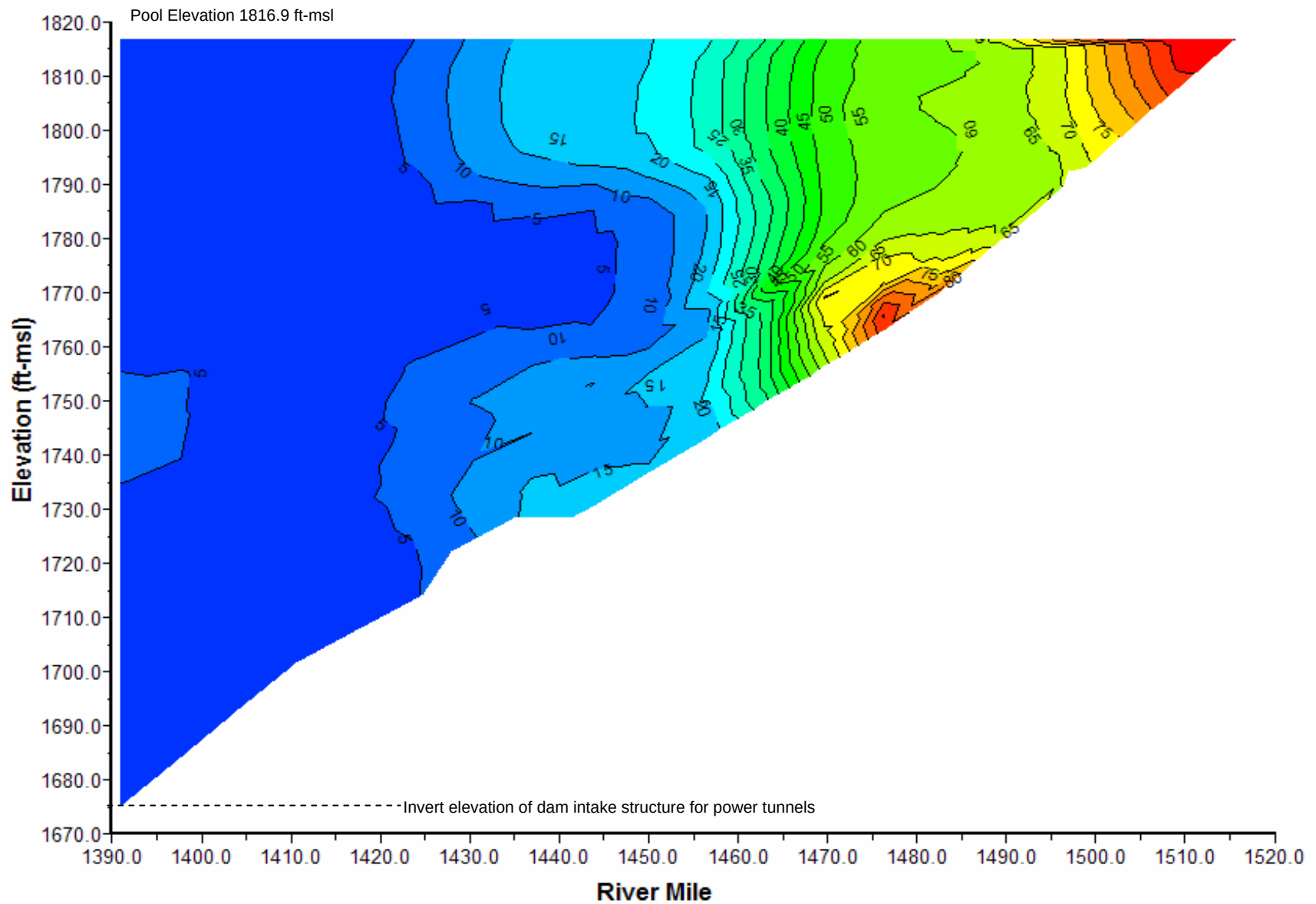
Plate 72. Longitudinal turbidity (NTU) contour plot of Garrison Reservoir based on depth-profile turbidity levels monitored at sites GARLK1390A, GARLK1412DW, GARLK1445DW, GARLK1481DW, and GARNFMORRR1 on June 20, 2006.
