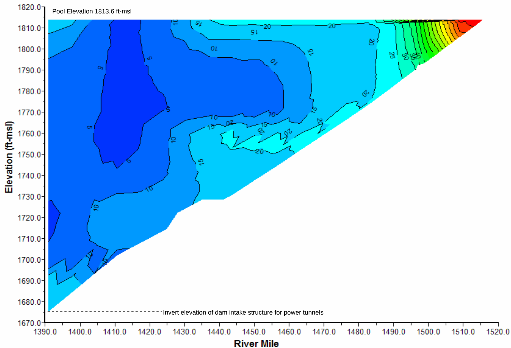
Plate 71. Longitudinal turbidity (NTU) contour plot of Garrison Reservoir based on depth-profile turbidity levels monitored at sites GARLK1390A, GARLK1412DW, GARLK1445DW, GARLK1481DW, and GARNFMORRR1 on May 25, 2006.
