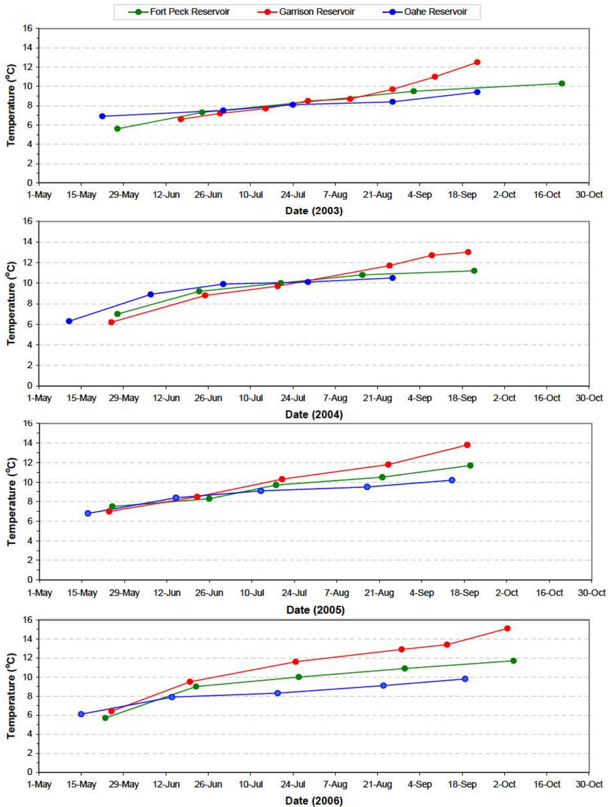
Plate 257. Near-bottom water temperatures measured at near-dam, deepwater locations in Fort Peck, Garrison, and Oahe Reservoirs during 2003 through 2006.
