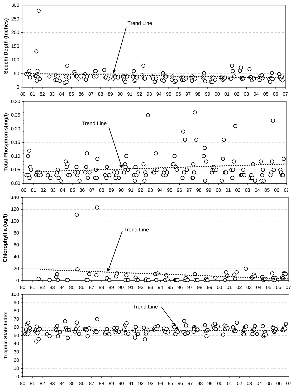
Plate 234. Historic trends for Secchi depth, total phosphorus, chlorophyll a , and Trophic State Index (TSI) monitored in Gavins Point Reservoir at the near-dam, ambient site (i.e., site GTPLK0811A) over the 27-year period of 1980 to 2006.
