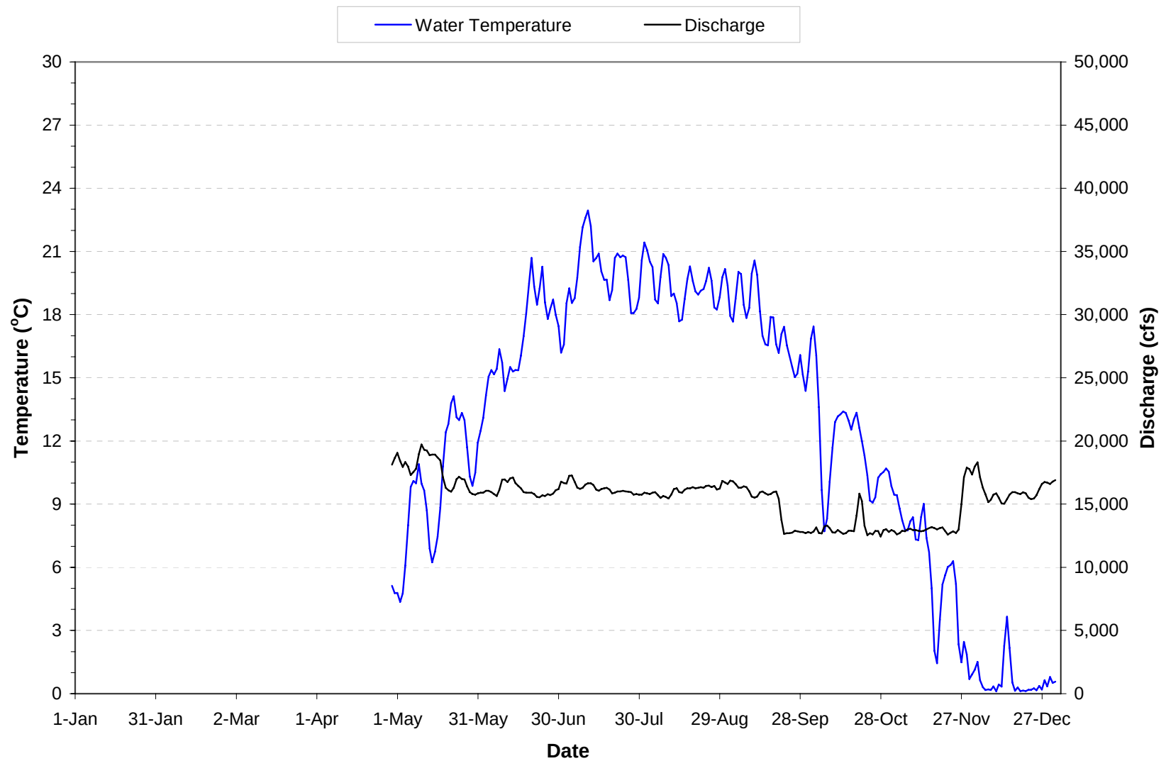
Plate 140. Mean daily water temperature and discharge of the Missouri River near Bismarck, North Dakota (i.e., site OAHNFMORR1) for 2005. Mean daily temperatures and discharges based on hourly measurements recorded on the Missouri River at Bismarck, North Dakota (USGS gaging station 06342500).
