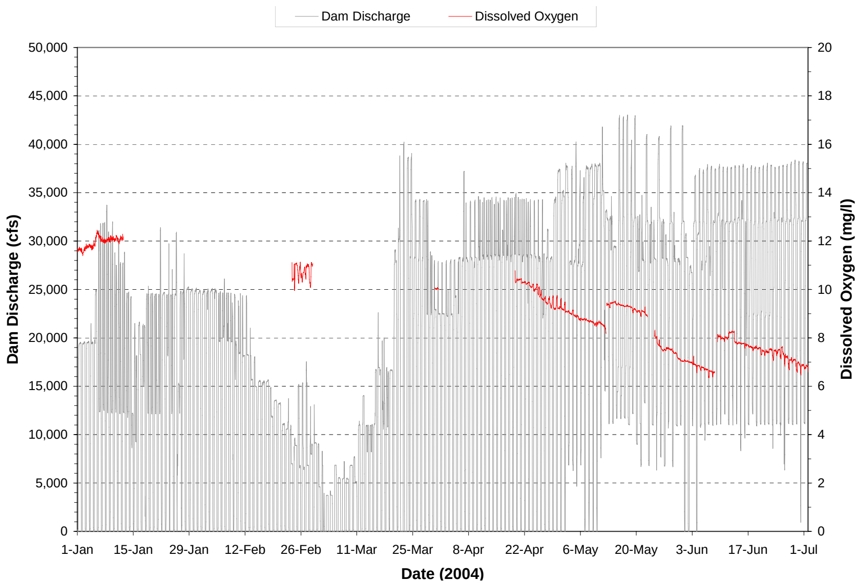
Plate 218. Hourly discharge and dissolved oxygen concentrations monitored at the Fort Randall powerplant on water discharged through the dam during the period January through June 2004. (Note: Gaps in dissolved oxygen plot represents periods when monitoring equipment was not operational.)
