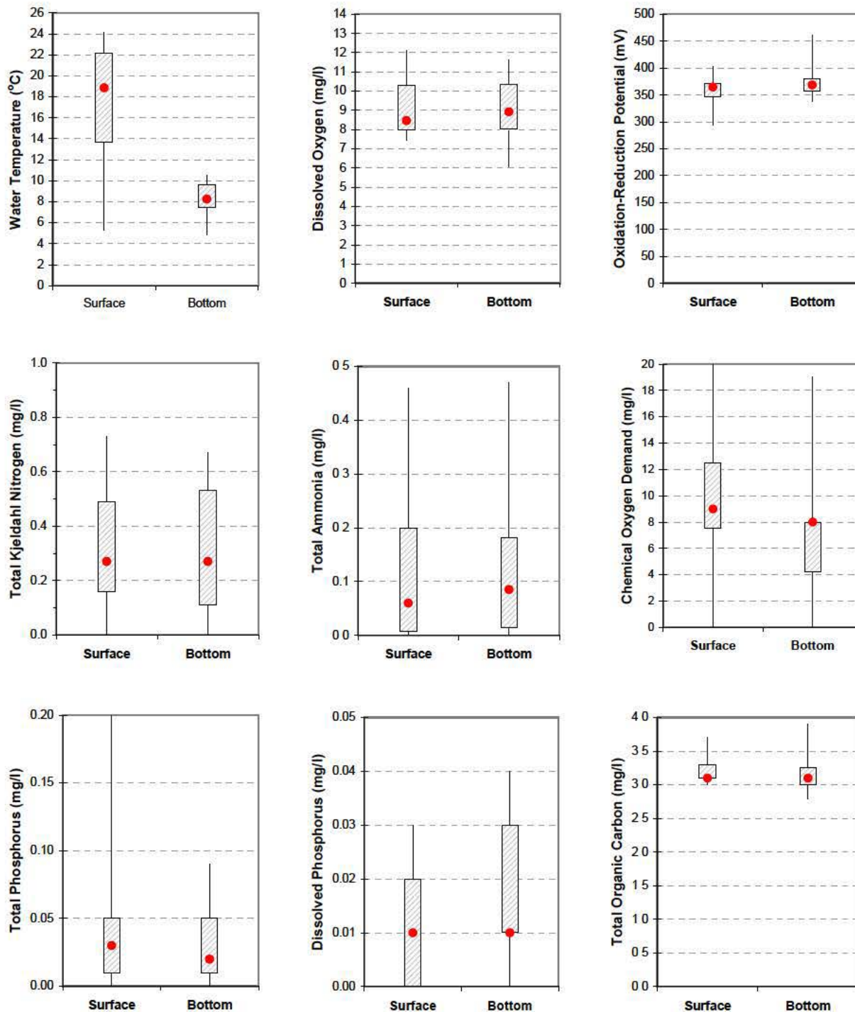
Plate 132. Box plots comparing surface and bottom water temperature, dissolved oxygen, oxidation-reduction potential, total Kjeldahl nitrogen, total ammonia nitrogen, chemical oxygen demand, total phosphorus, dissolved phosphorus, and total organic carbon measured in Oahe Reservoir at site OAHK1073A during the summer months of 2002 through 2006. (Box plots display minimum, 25 th percentile, 75 th percentile, and maximum. Median value is indicated by the red dot. Non-overlapping interquartile ranges of the adjacent box plots indicate a significant difference between surface and bottom measurements.)
