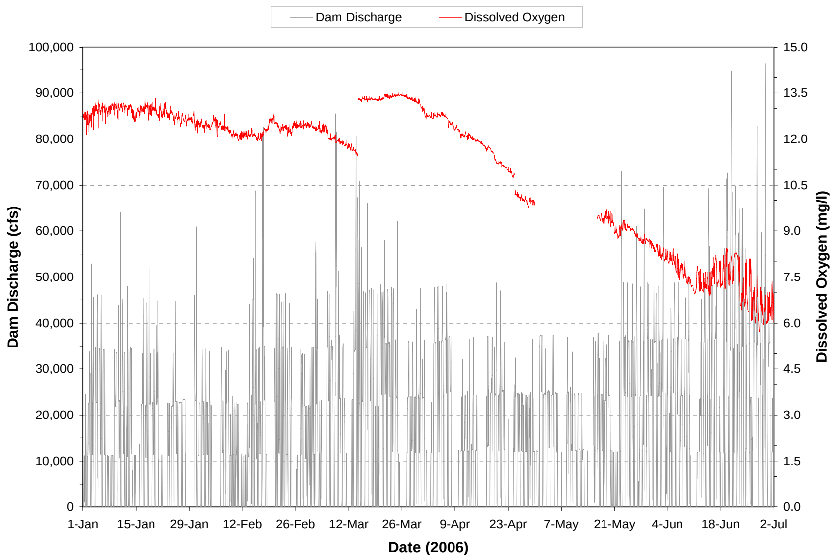
Plate 177. Hourly discharge and dissolved oxygen concentrations monitored at the Big Bend powerplant on water discharged through the dam during the period January through July 2006. (Note: Gaps in dissolved oxygen plot represents periods when monitoring equipment was not operational.)
