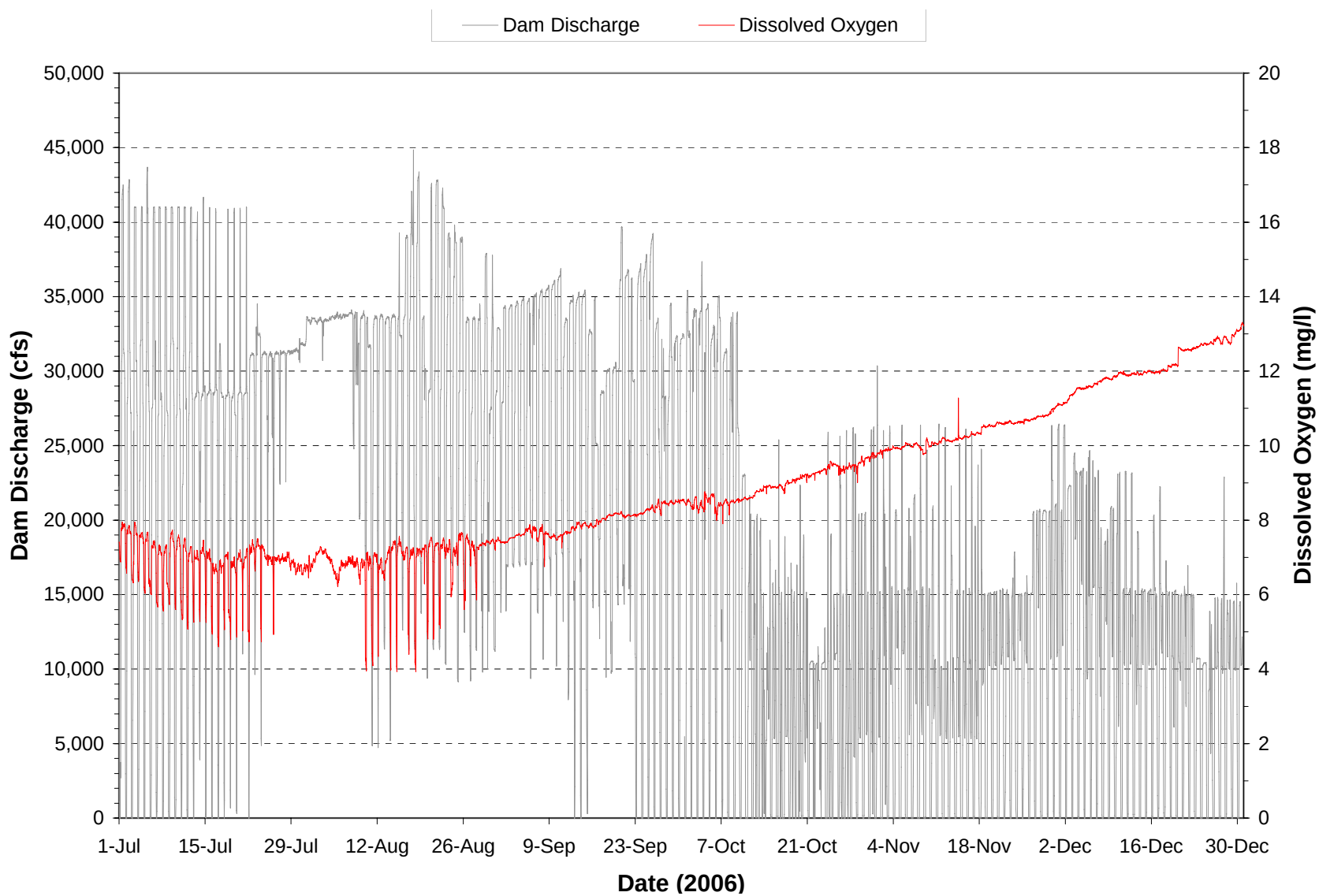
Plate 223. Hourly discharge and dissolved oxygen concentrations monitored at the Fort Randall powerplant on water discharged through the dam during the period July through December 2006.
