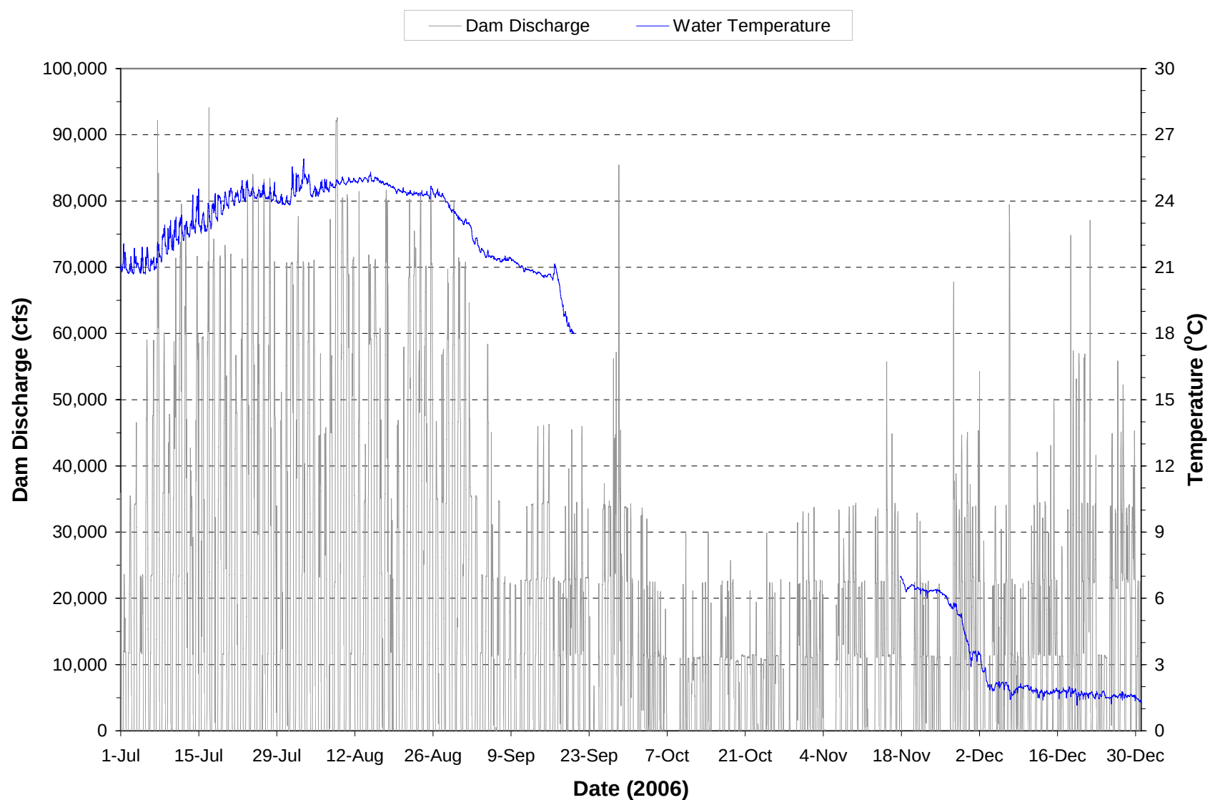
Plate 172. Hourly discharge and water temperature monitored at the Big Bend powerplant on water discharged through the dam during the period July through December 2006. (Note: Gaps in temperature plot represents periods when monitoring equipment was not operational.)
