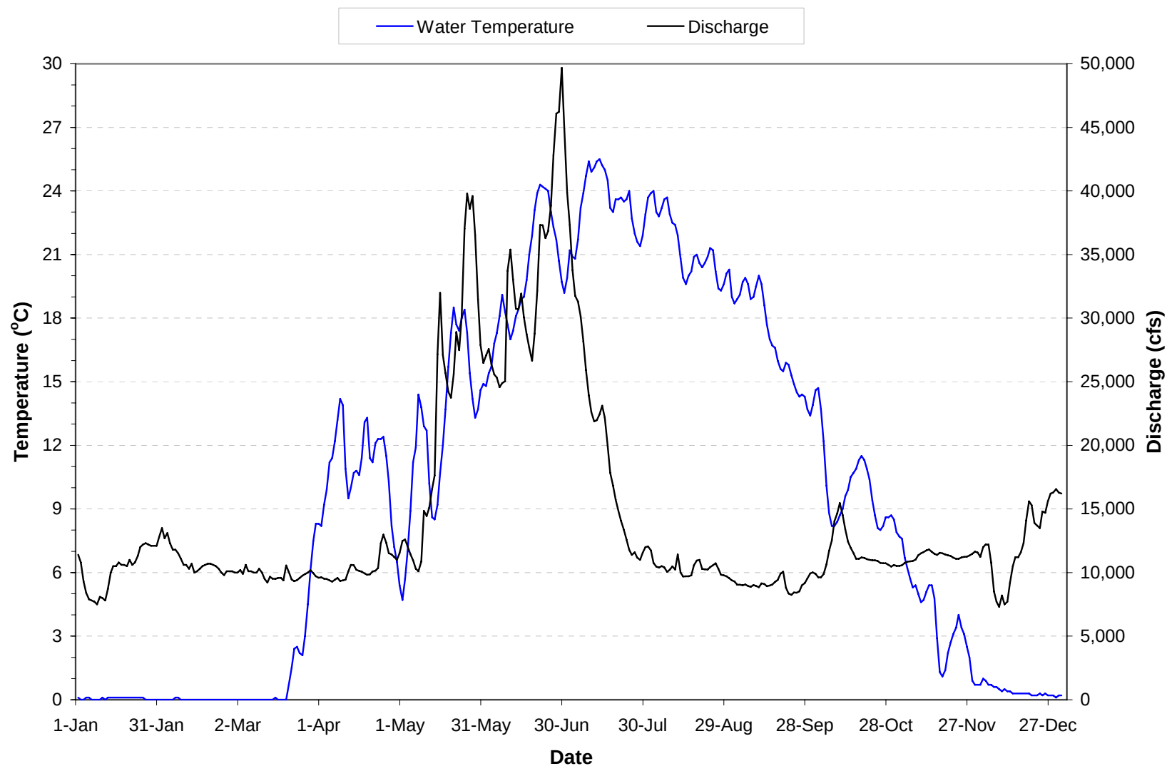
Plate 85. Mean daily water temperature and discharge of the Missouri River near Williston, North Dakota (i.e., site GARNFMORRR1) for 2005. Mean temperatures based on hourly measurements recorded on the Missouri River near Williston, North Dakota (USGS gaging station 06330000). Mean daily discharge estimated by adding mean daily discharge recorded for the Missouri River near Culbertson, Montana (USGS gaging station 06185500) and the mean daily discharge recorded for the Yellowstone River near Sidney, Montana (USGS gaging station 06329500).
