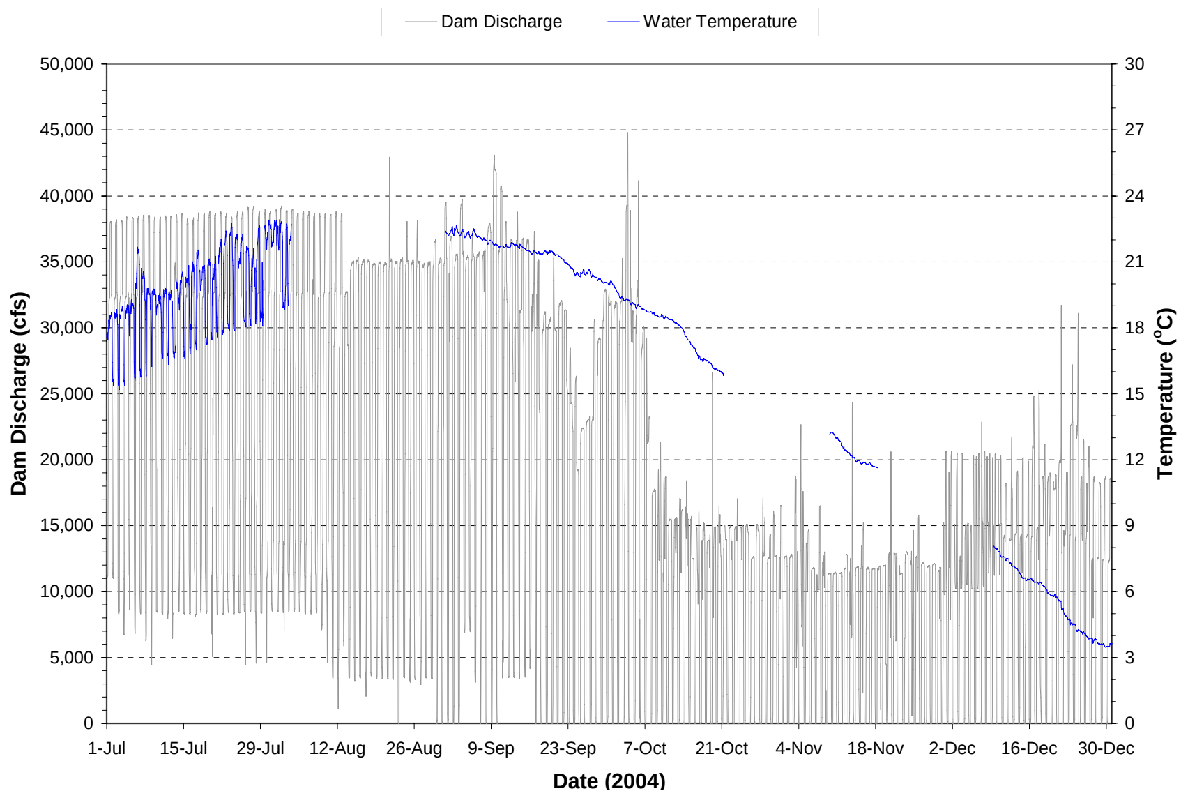
Plate 213. Hourly discharge and water temperature monitored at the Fort Randall powerplant on water discharged through the dam during the period July through December 2004. (Note: Gaps in temperature plot represents periods when monitoring equipment was not operational.)
