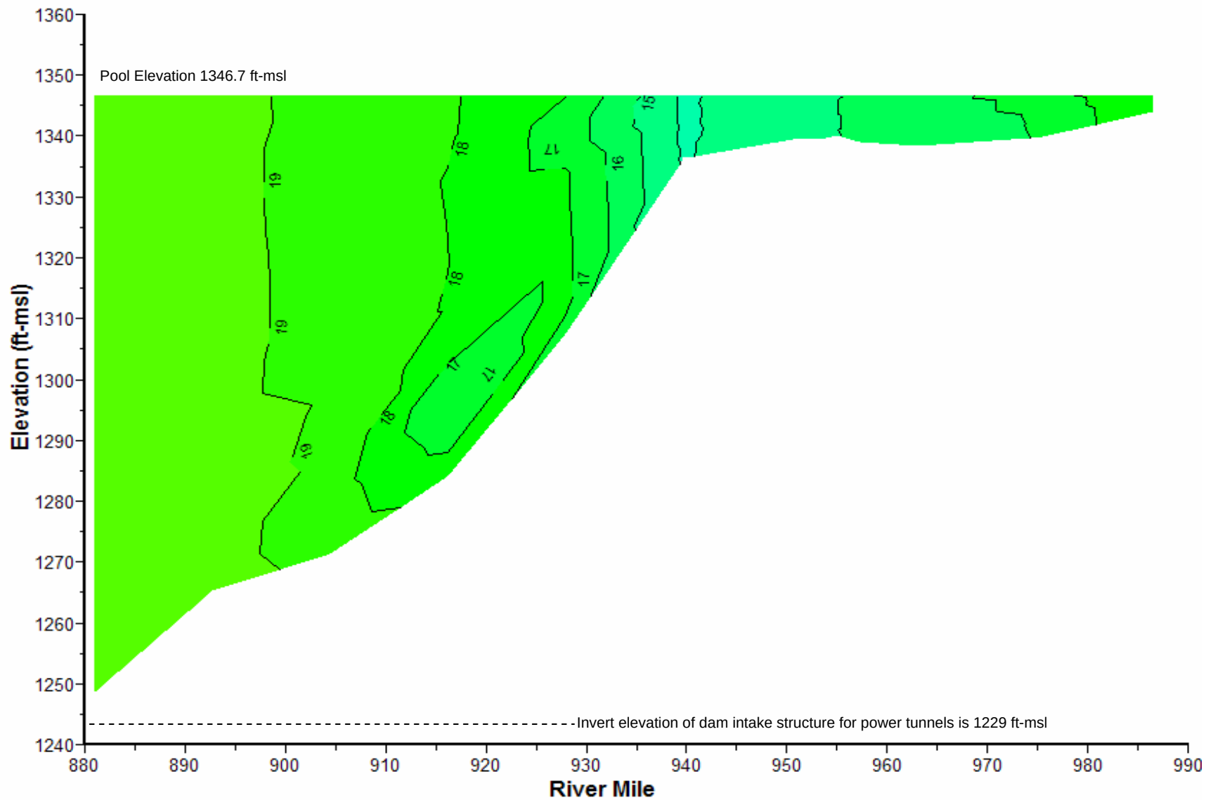
Plate 191. Longitudinal water temperature (°C) contour plot of Fort Randall Reservoir based on depth-profile water temperatures measured at sites FTRLK0880A, FTRLK0892DW, FTRLK0911DW, FTRLK0924DW, FTRLK0940DW, FTRLK0955DW, FTRLK0968DW, and BBDPP1 on September 21, 2006.
