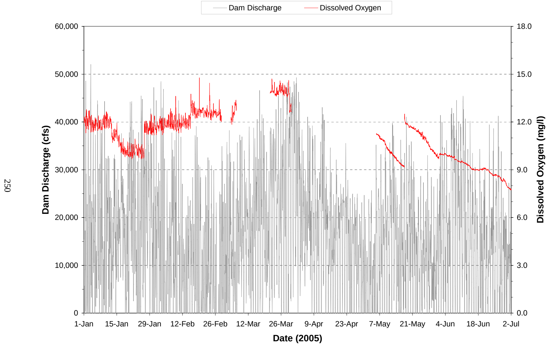
Plate 151. Hourly discharge and dissolved oxygen monitored at the Oahe powerplant on water discharged through the dam during the period January through June 2005. (Note: Gaps in dissolved oxygen plot represents periods when monitoring equipment was not operational.)
