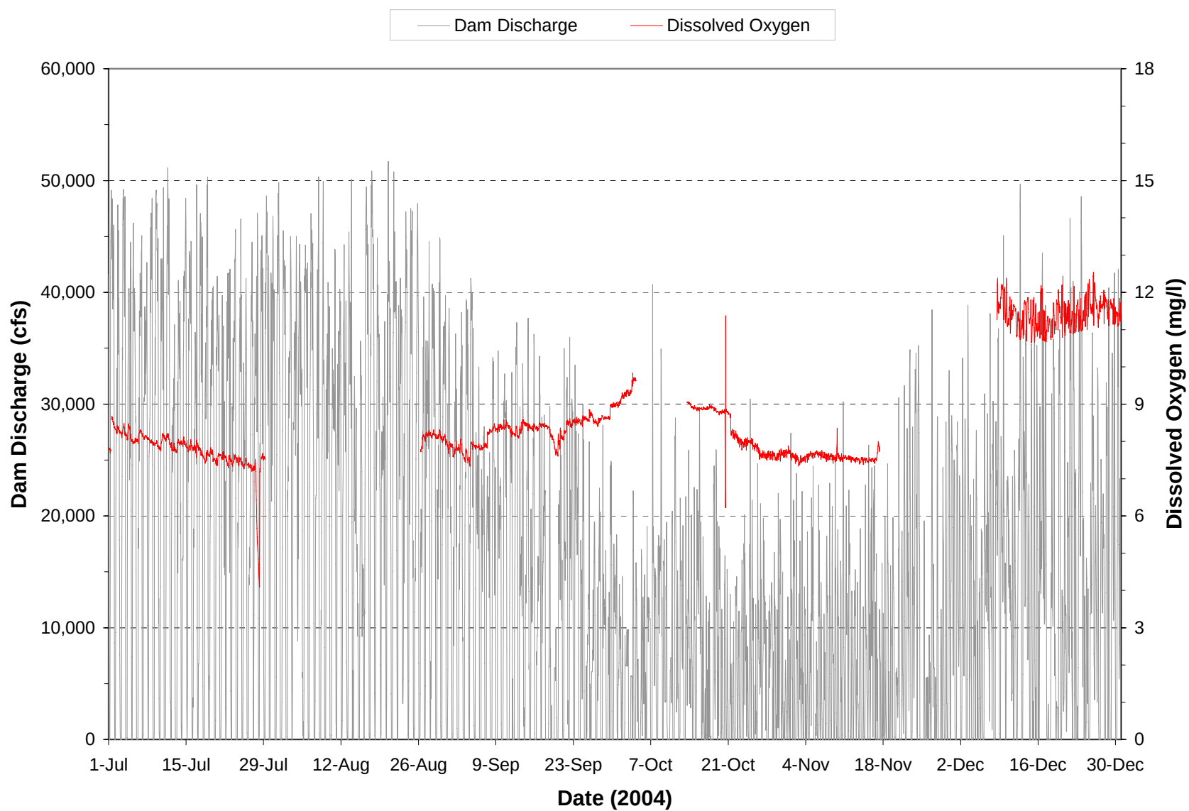
Plate 150. Hourly discharge and dissolved oxygen monitored at the Oahe powerplant on water discharged through the dam during the period July through December 2004. (Note: Gaps in dissolved oxygen plot represents periods when monitoring equipment was not operational.)
