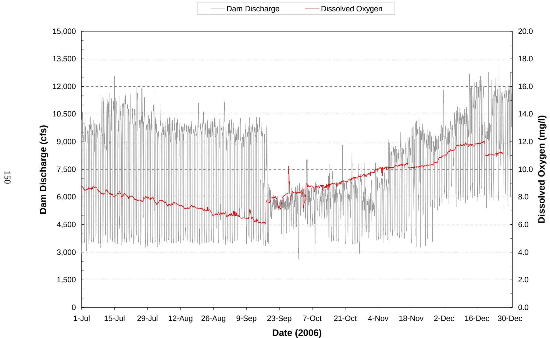
Plate 43. Hourly discharge and dissolved oxygen monitored at the Fort Peck powerplant on water discharged through the dam during the period July through December 2006. (Note: Gaps in dissolved oxygen plot represent periods when monitoring equipment was not operational.)
