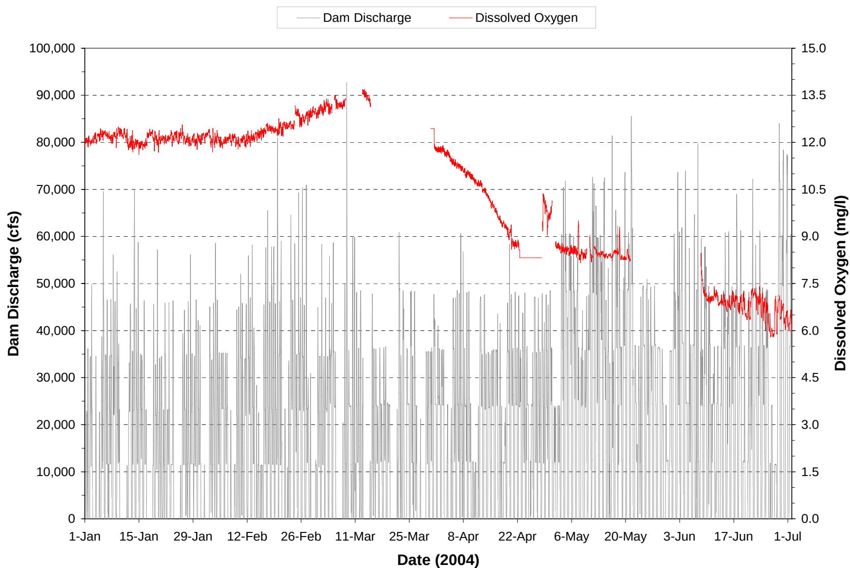
Plate 173. Hourly discharge and dissolved oxygen concentrations monitored at the Big Bend powerplant on water discharged through the dam during the period January through June 2004. (Note: Gaps in dissolved oxygen plot represents periods when monitoring equipment was not operational.)
