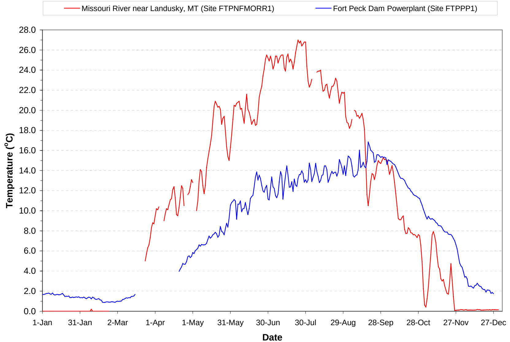
Plate 45. Mean daily water temperatures monitored at the Fort Peck Powerplant (i.e., site FTPPP1) and the Missouri River near Landusky, Montana (i.e., site FTPNFMORR1) during 2006. (Note: Gaps in temperature plots are periods when monitoring equipment was not operational.)
