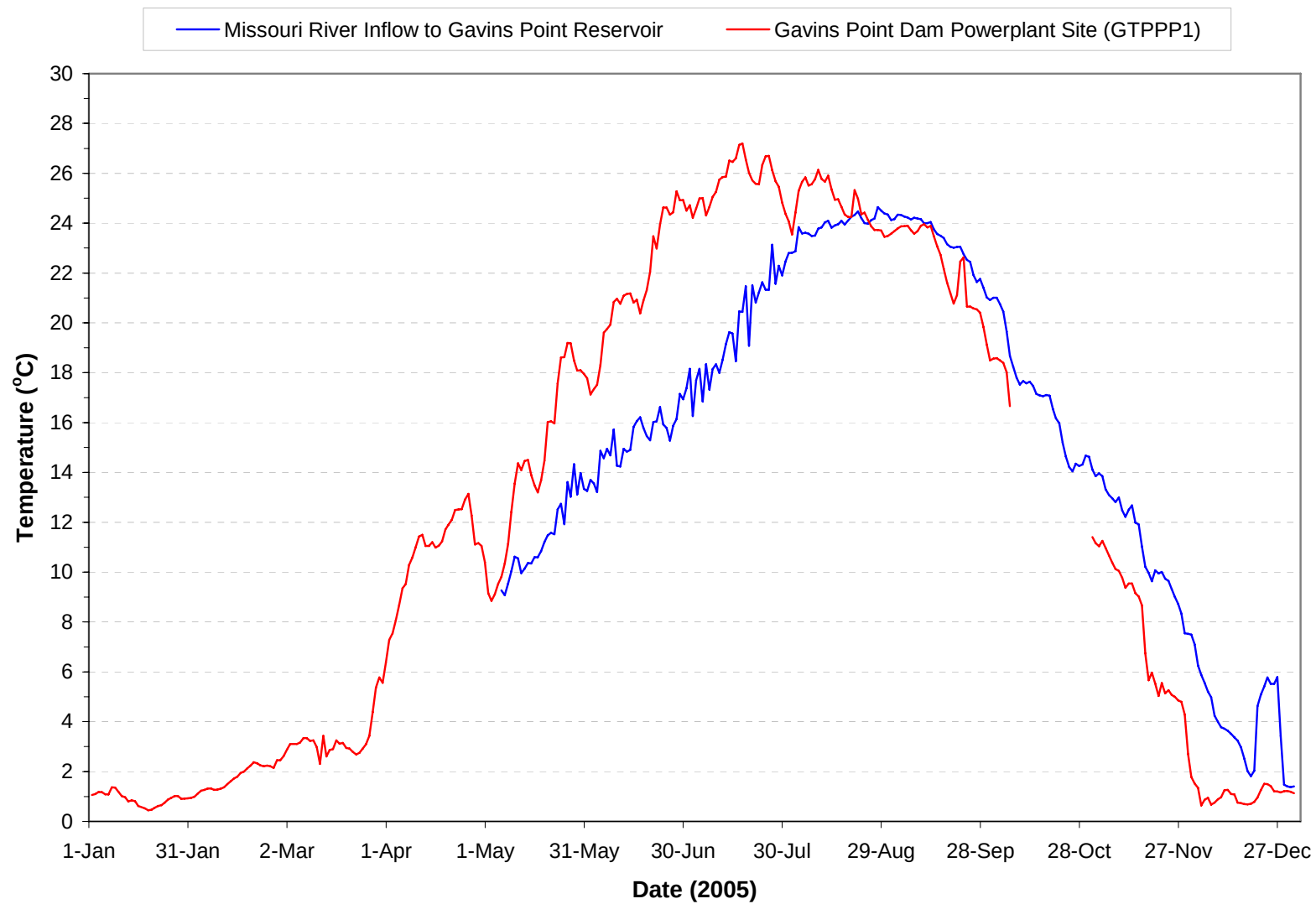
Plate 255. Mean daily water temperatures monitored at the Gavins Point Powerplant (i.e., site GT PPP1) and estimated for the Missouri River inflow to Gavins Point Reservoir during 2005. (Note: Gaps in temperature plots are periods when monitoring equipment was not operational.)
