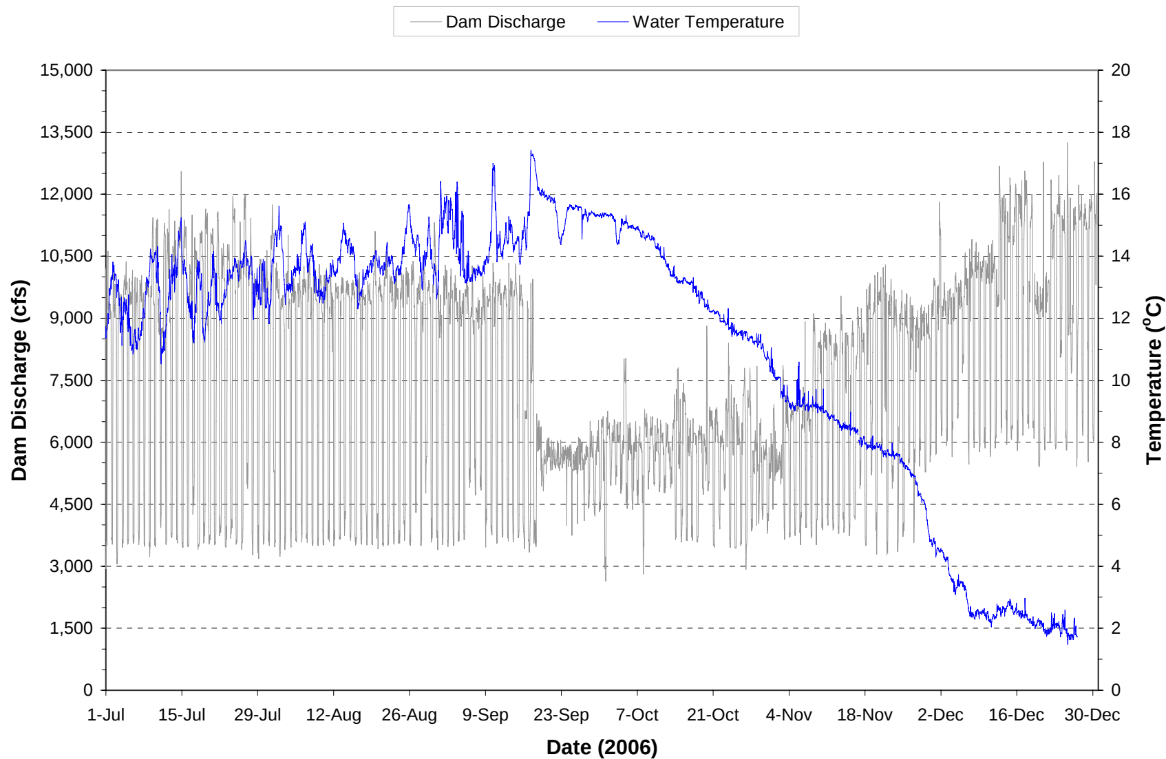
Plate 37. Hourly discharge and water temperature monitored at the Fort Peck powerplant on water discharged through the dam during the period July through December 2006. (Note: Gaps in temperature plot represents periods when monitoring equipment was not operational.)
