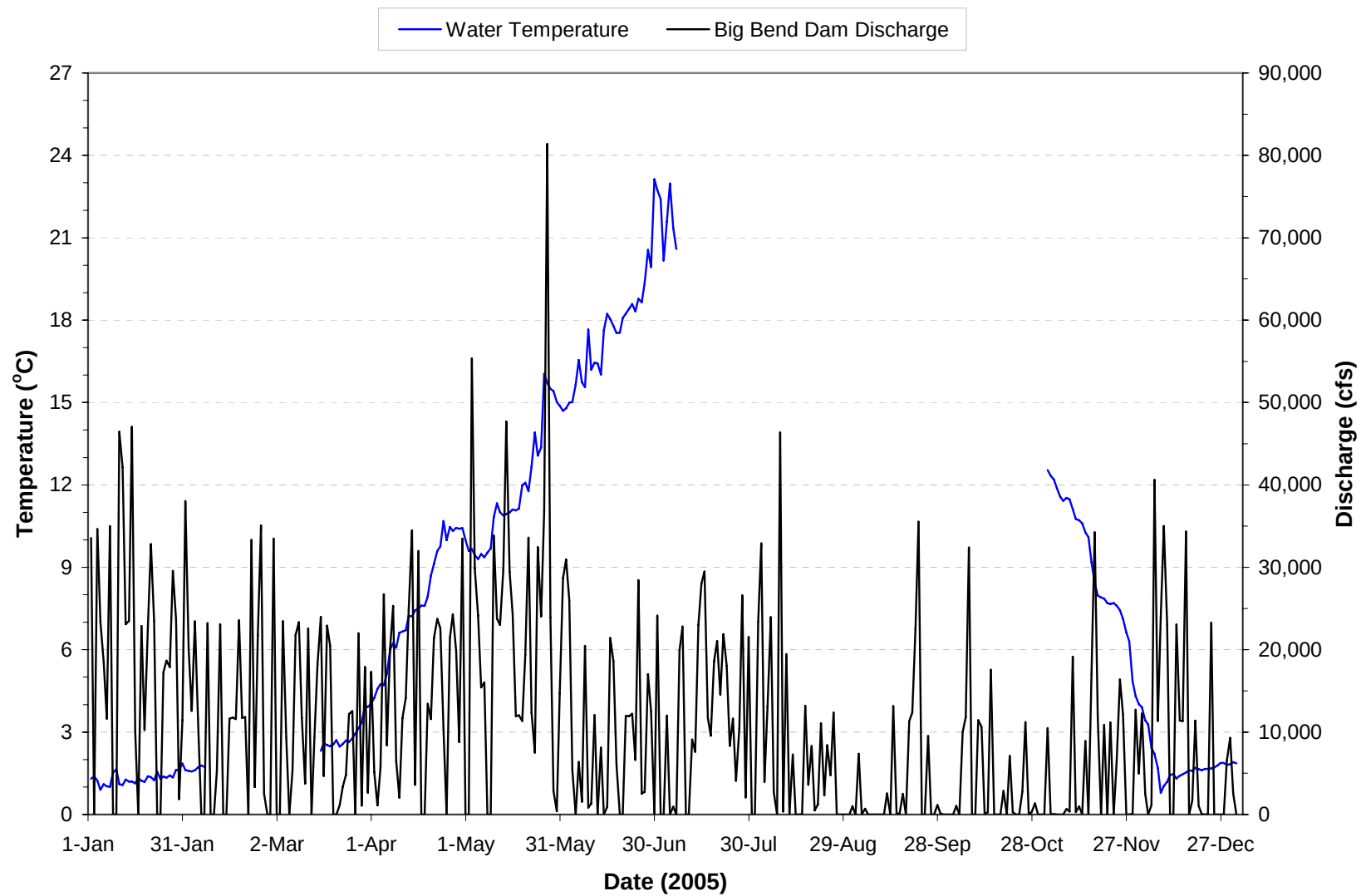
Plate 209. Mean daily water temperature and discharge of the Missouri River at Big Bend Dam (i.e., site BBDPP1) for 2005. Mean daily temperatures and discharges based on hourly measurements recorded on discharge through Big Bend Dam. (Note: Gaps in temperature plots are periods when monitoring equipment was not operational.)
