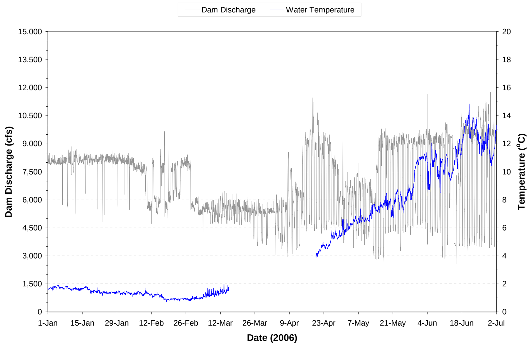
Plate 36. Hourly discharge and water temperature monitored at the Fort Peck powerplant on water discharged through the dam during the period January through June 2006. (Note: Gaps in temperature plot represents periods when monitoring equipment was not operational.)
