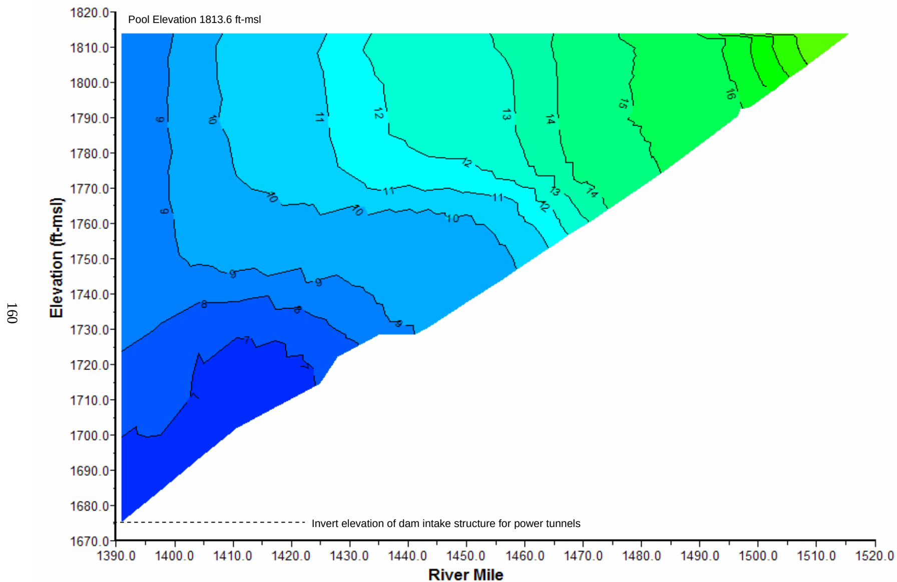
Plate 57. Longitudinal water temperature (°C) contour plot of Garrison Reservoir based on depth-profile water temperatures measured at sites GARLK1390A, GARLK1412DW, GARLK1445DW, GARLK1481DW, and GARNFMORRR1 on May 25, 2006.
