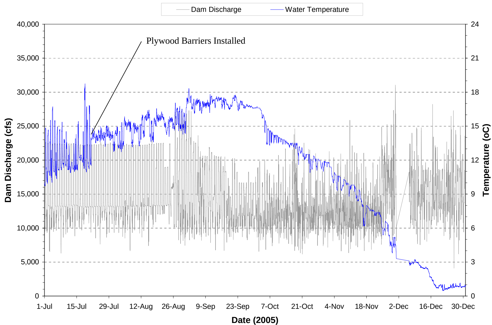
Plate 93. Hourly discharge and water temperature monitored at the Garrison powerplant on water discharged through the dam during the period July through December 2005.
