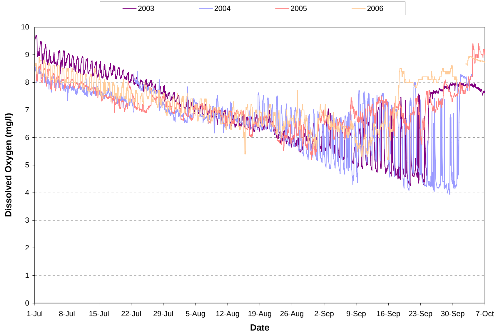
Plate 104. Dissolved oxygen concentrations of water discharged through Garrison Dam during the period July 1 through October 7 in 2003, 2004, 2005, and 2006.
