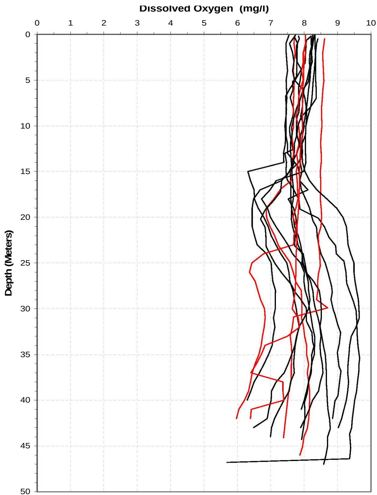
Plate 127. Dissolved oxygen depth profiles for Oahe Reservoir generated from data collected at the near-dam, deepwater ambient monitoring site (i.e., OAHLK1073A) during the months of July, August, and September over the 5-year period of 2002 to 2006. (Note: Red profile plots were measured in the month of September.)
