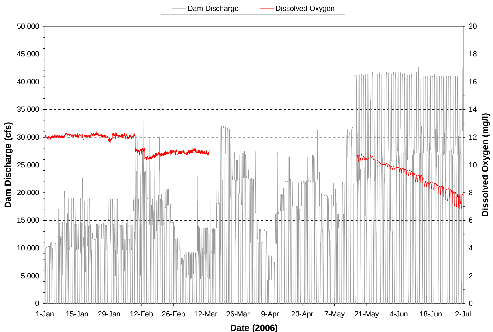
Plate 222. Hourly discharge and dissolved oxygen concentrations monitored at the Fort Randall powerplant on water discharged through the dam during the period January through June 2006. (Note: Gaps in dissolved oxygen plot represents periods when monitoring equipment was not operational.)
