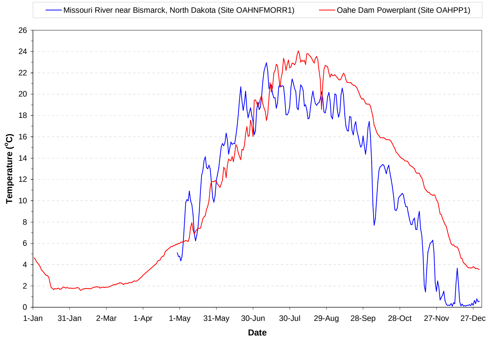
Plate 155. Mean daily water temperatures monitored at the Oahe Powerplant (i.e., site OAHPP1) and the Missouri River near Bismarck, North Dakota (i.e., site OAHNFMORR1) during 2005. (Note: Gaps in temperature plots are periods when monitoring equipment was not operational.)
