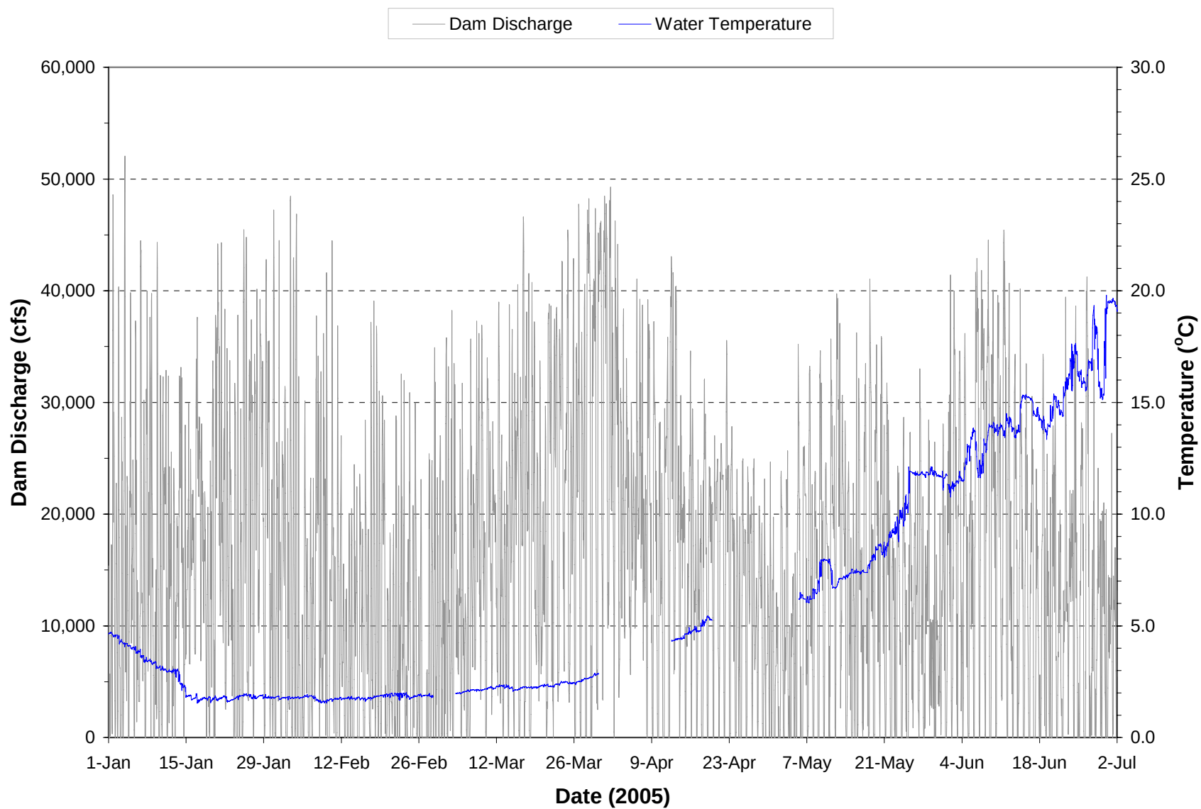
Plate 145. Hourly discharge and water temperature monitored at the Oahe powerplant on water discharged through the dam during the period January through June 2005. (Note: Gaps in temperature plot represents periods when monitoring equipment was not operational.)
