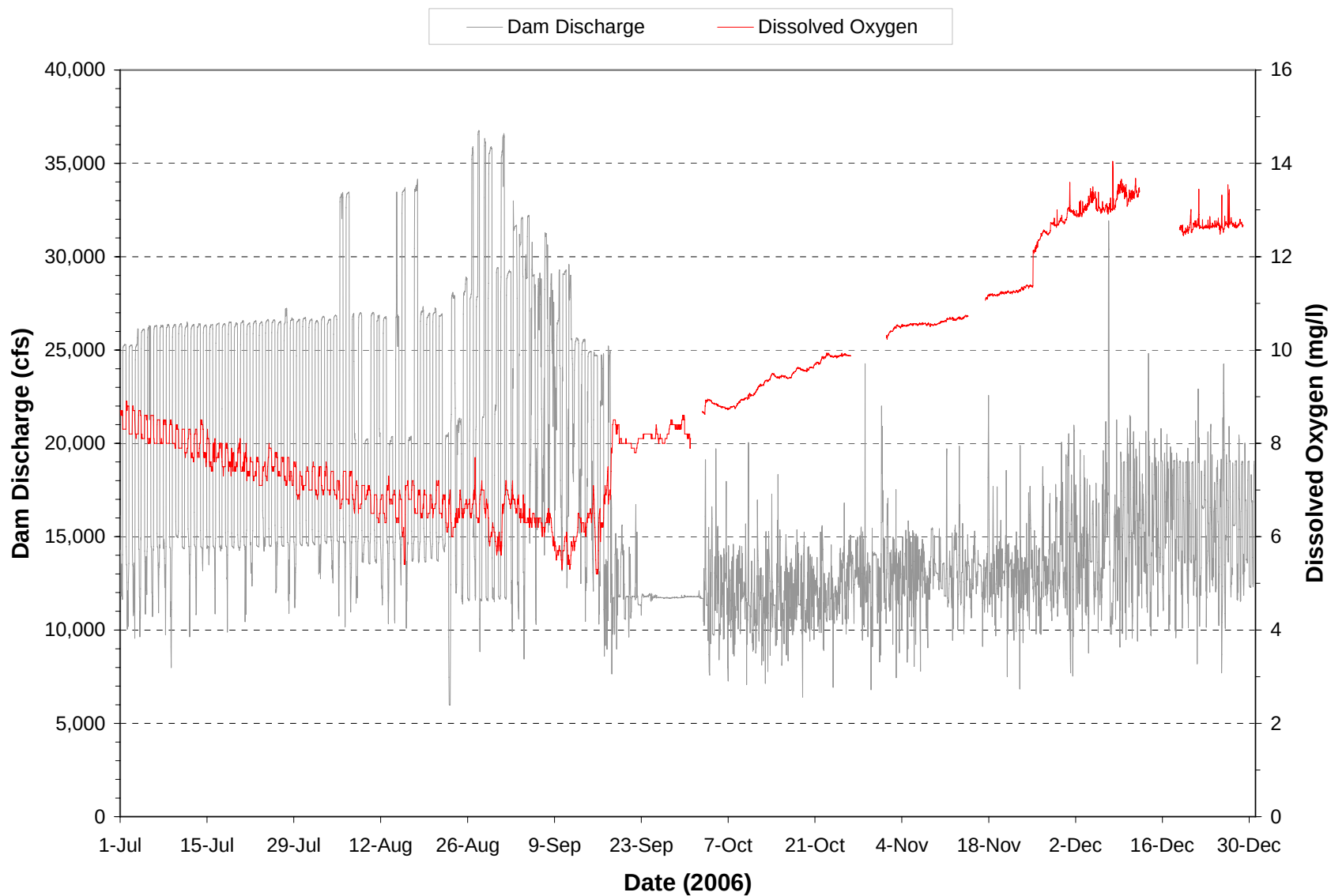
Plate 103. Hourly discharge and dissolved oxygen monitored at the Garrison powerplant on water discharged through the dam during the period July through December 2006. (Note: Gaps in dissolved oxygen plot represents periods when monitoring equipment was not operational.)
