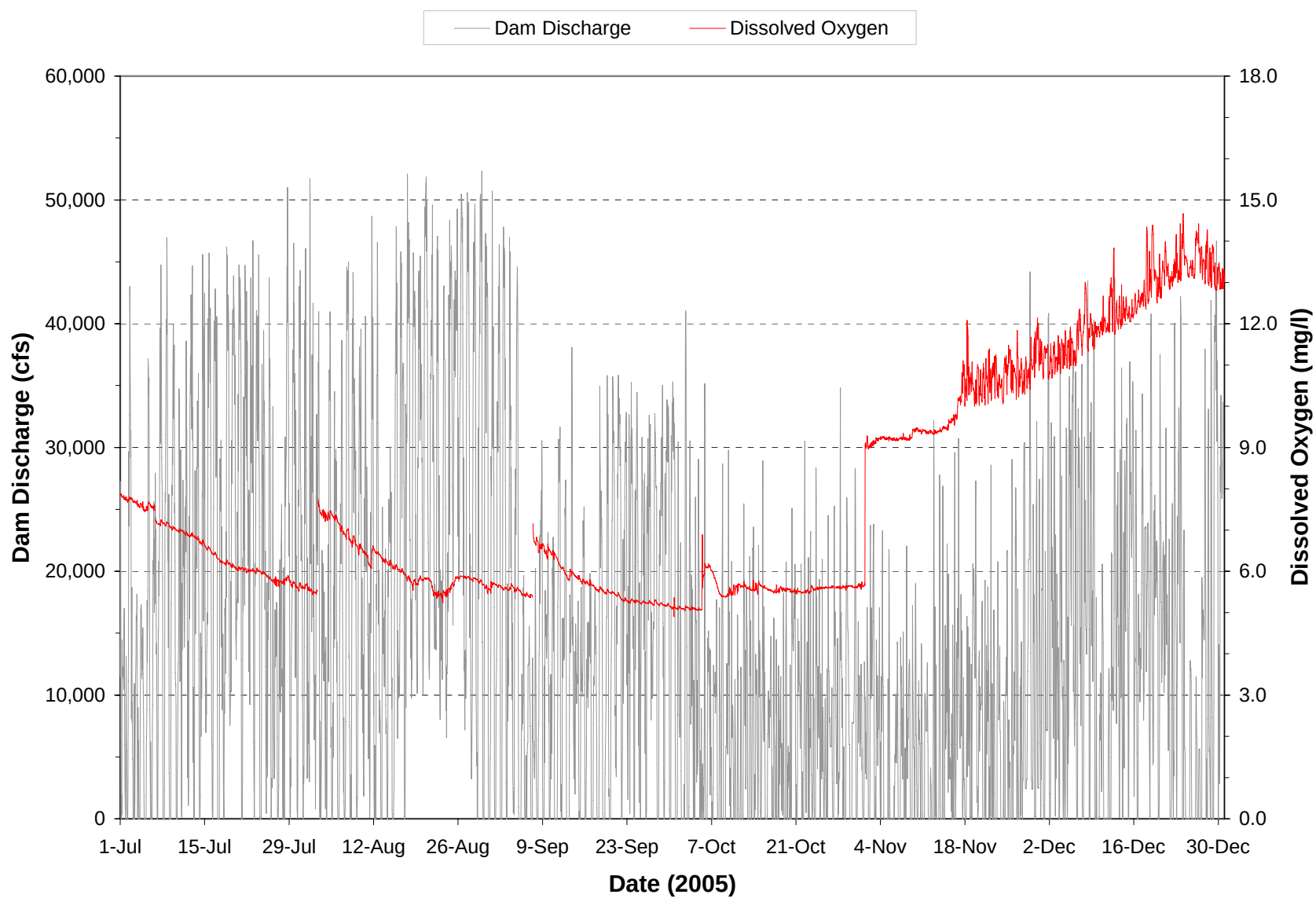
Plate 152. Hourly discharge and dissolved oxygen monitored at the Oahe powerplant on water discharged through the dam during the period July through December 2005. (Note: Gaps in dissolved oxygen plot represents periods when monitoring equipment was not operational.)
