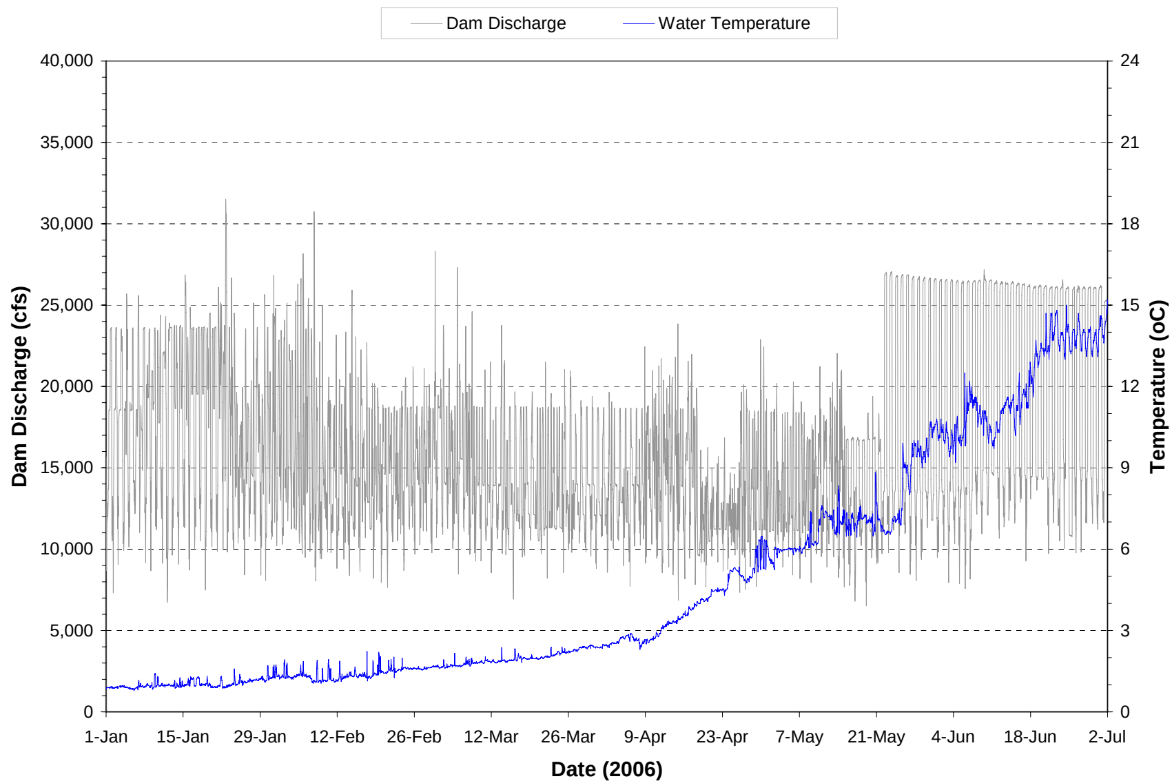
Plate 94. Hourly discharge and water temperature monitored at the Garrison powerplant on water discharged through the dam during the period January through June 2006.
