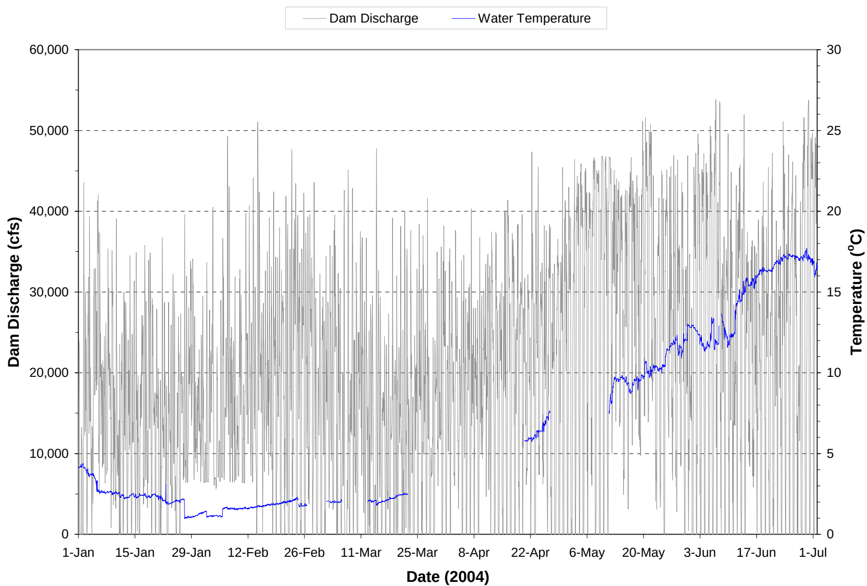
Plate 143. Hourly discharge and water temperature monitored at the Oahe powerplant on water discharged through the dam during the period January through June 2004. (Note: Gaps in temperature plot represents periods when monitoring equipment was not operational.)
