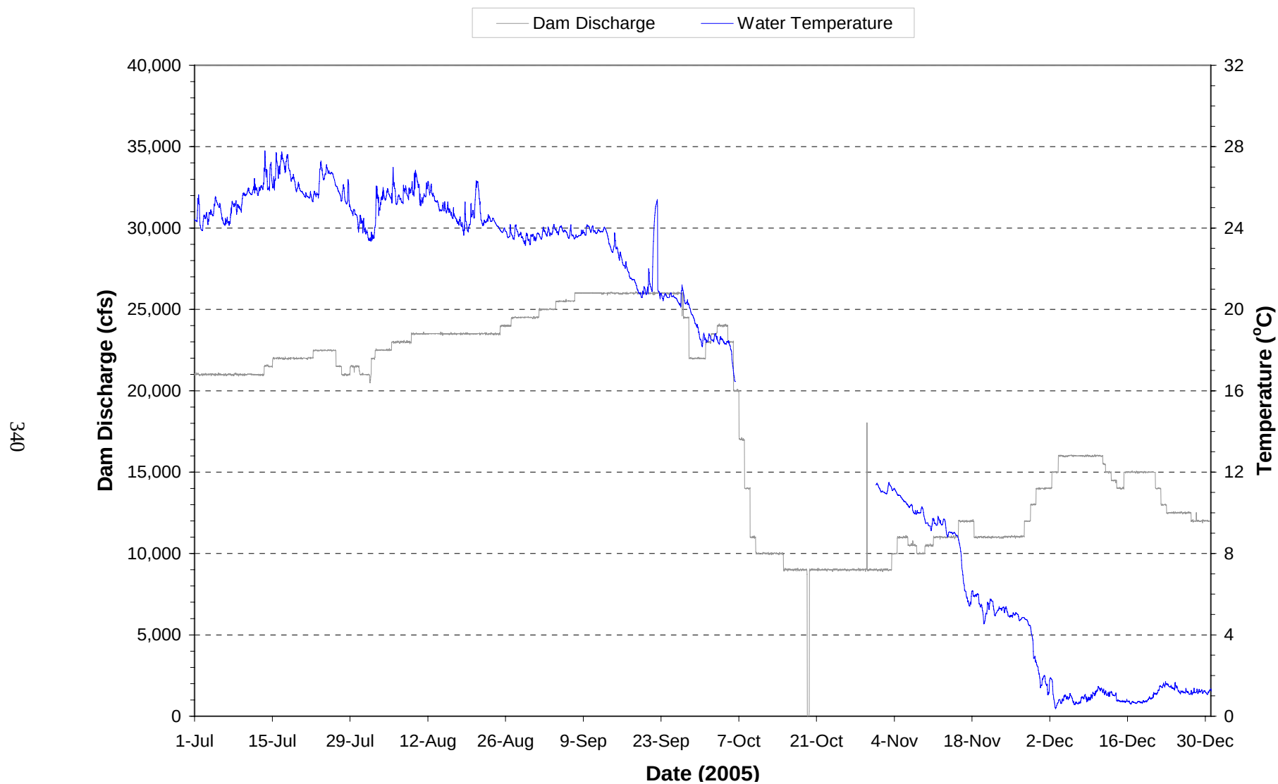
Plate 246. Hourly discharge and water temperature monitored at the Gavins Point powerplant on water discharged through the dam during the period July through December 2005. (Note: Gaps in temperature plot represents periods when monitoring equipment was not operational.)
