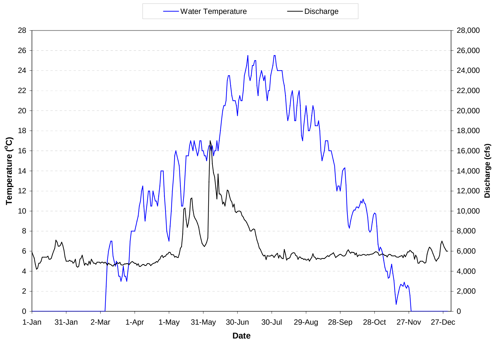
Plate 29. Mean daily water temperature and discharge of the Missouri River near Landusky, Montana (i.e., site FTPNFMORR1) for 2005. Means based on hourly measurements recorded at USGS gaging station 06115200.
