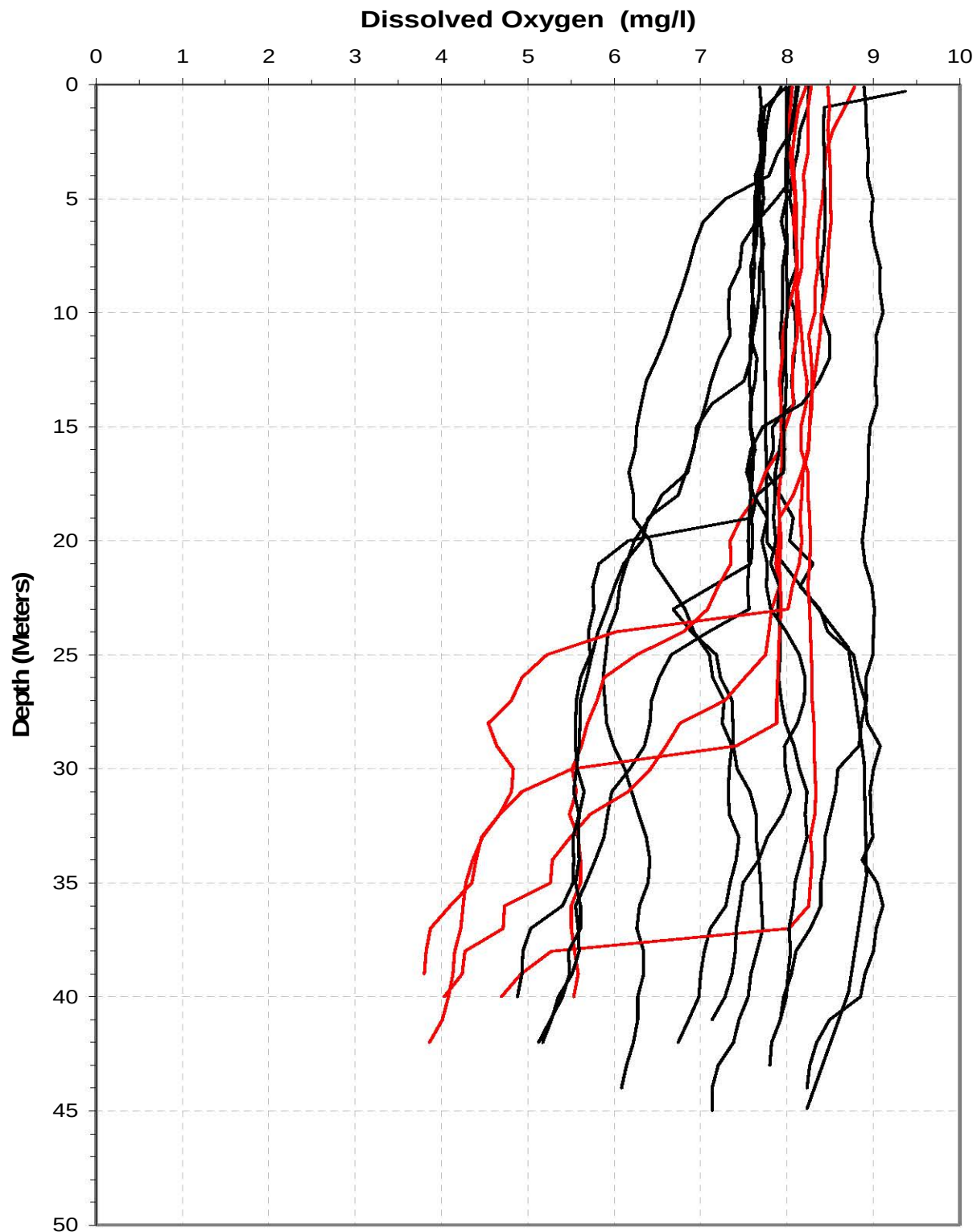
Plate 70. Dissolved oxygen depth profiles for Garrison Reservoir generated from data collected at the near-dam, deepwater ambient monitoring site (i.e., GARLK1390A) during the months of July, August, and September over the 5-year period of 2002 to 2006. (Note: Red profile plots were measured in the month of September.)
