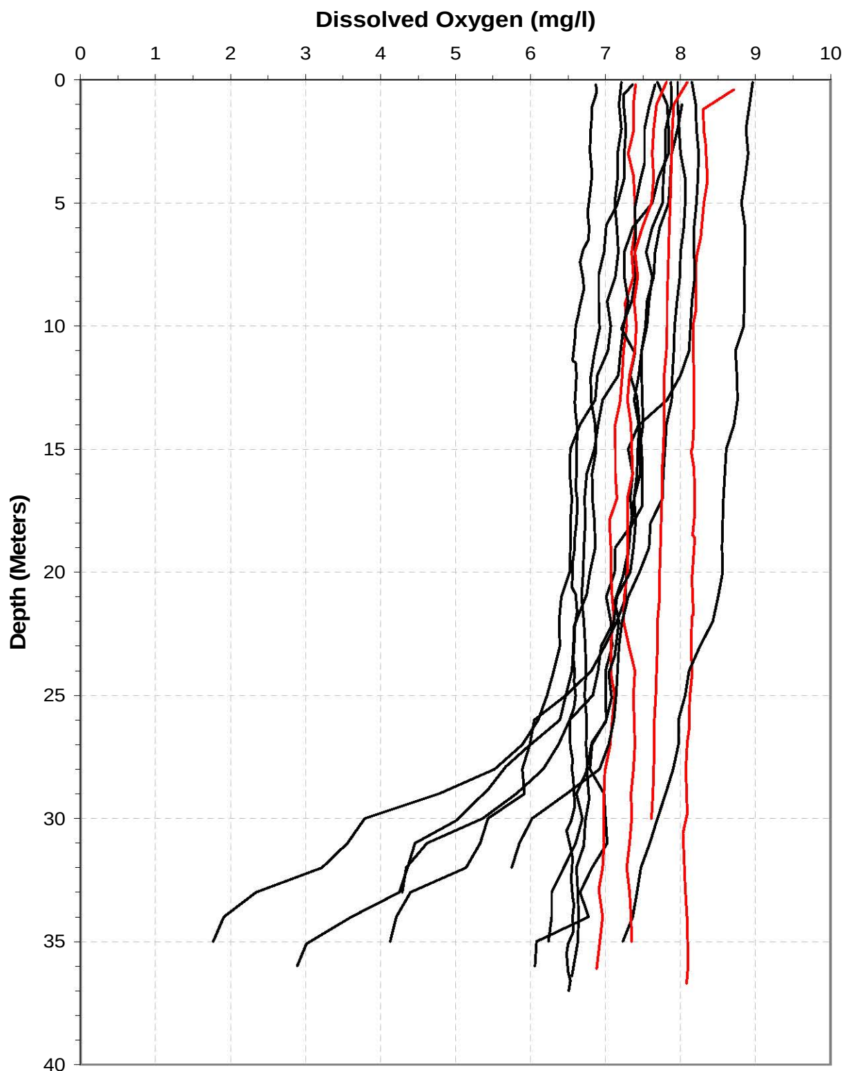
Plate 197. Dissolved oxygen depth profiles for Fort Randall Reservoir generated from data collected at the near-dam, deepwater ambient monitoring site (i.e., site FTRLK0880A) during the months of July, August, and September over the 5-year period of 2002 to 2006. (Note: Red profile plots were measured in the month of September.)
