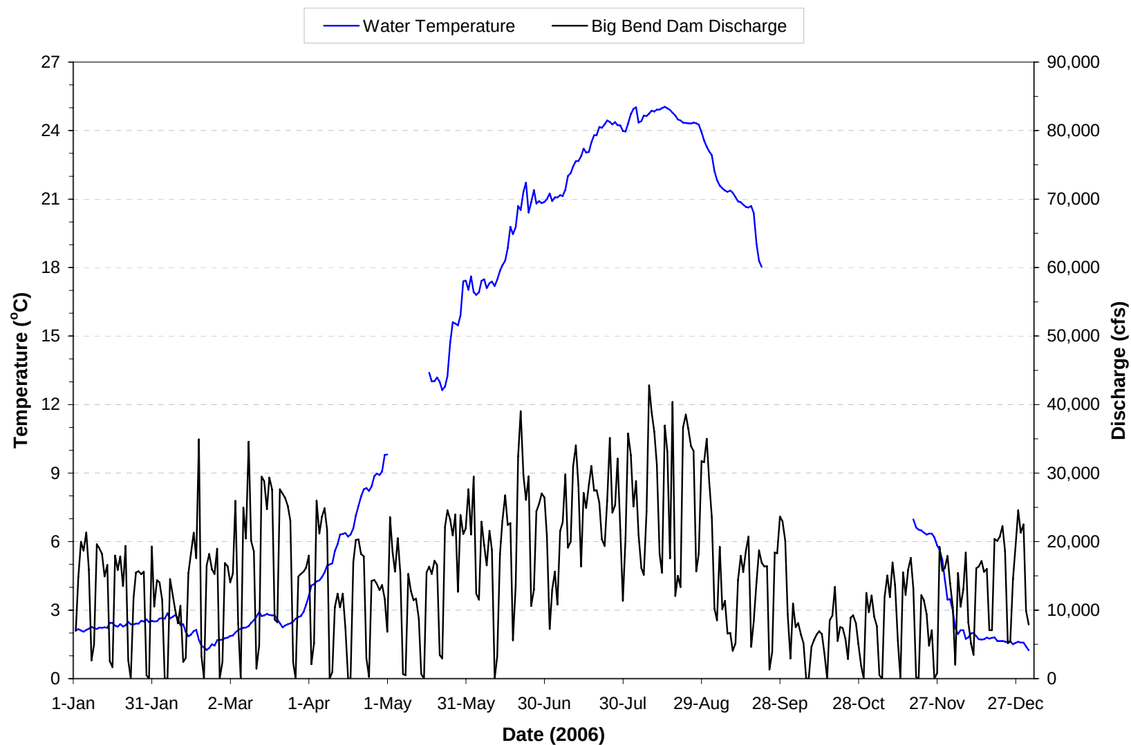
Plate 210. Mean daily water temperature and discharge of the Missouri River at Big Bend Dam (i.e., site BBDPP1) for 2006. Mean daily temperatures and discharges based on hourly measurements recorded on discharge through Big Bend Dam. (Note: Gaps in temperature plots are periods when monitoring equipment was not operational.)
