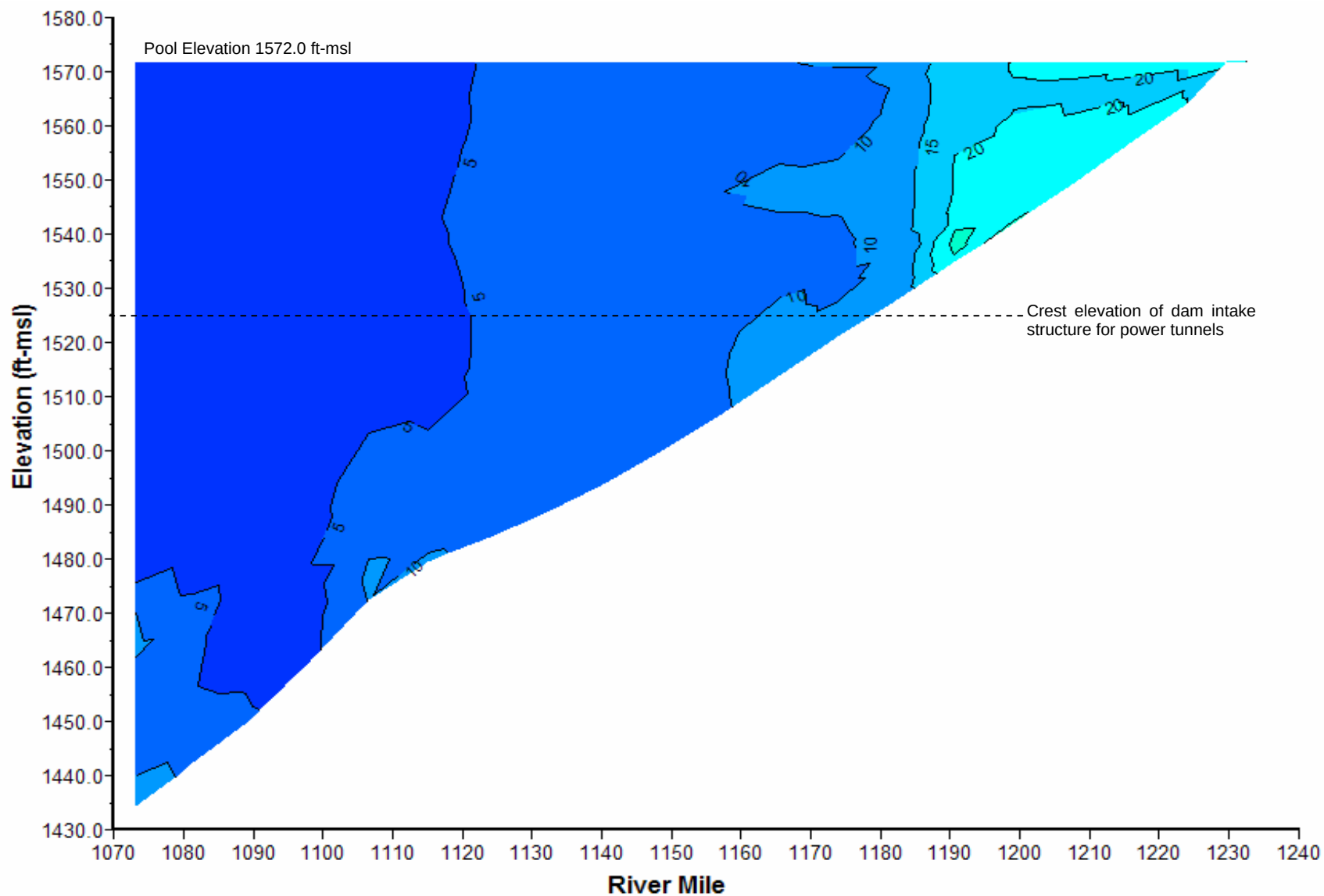
Plate 131. Longitudinal turbidity (NTU) contour plot of Oahe Reservoir based on depth-profile turbidity levels measured at sites OAHRLK1073A, OAHLK1090DW, OAHLK1110DW, OAHLK1135DW, OAHLK1153DW, OAHLK1176DW, OAHLK1196DW and OAHNFMORR1 on September 19, 2006.
