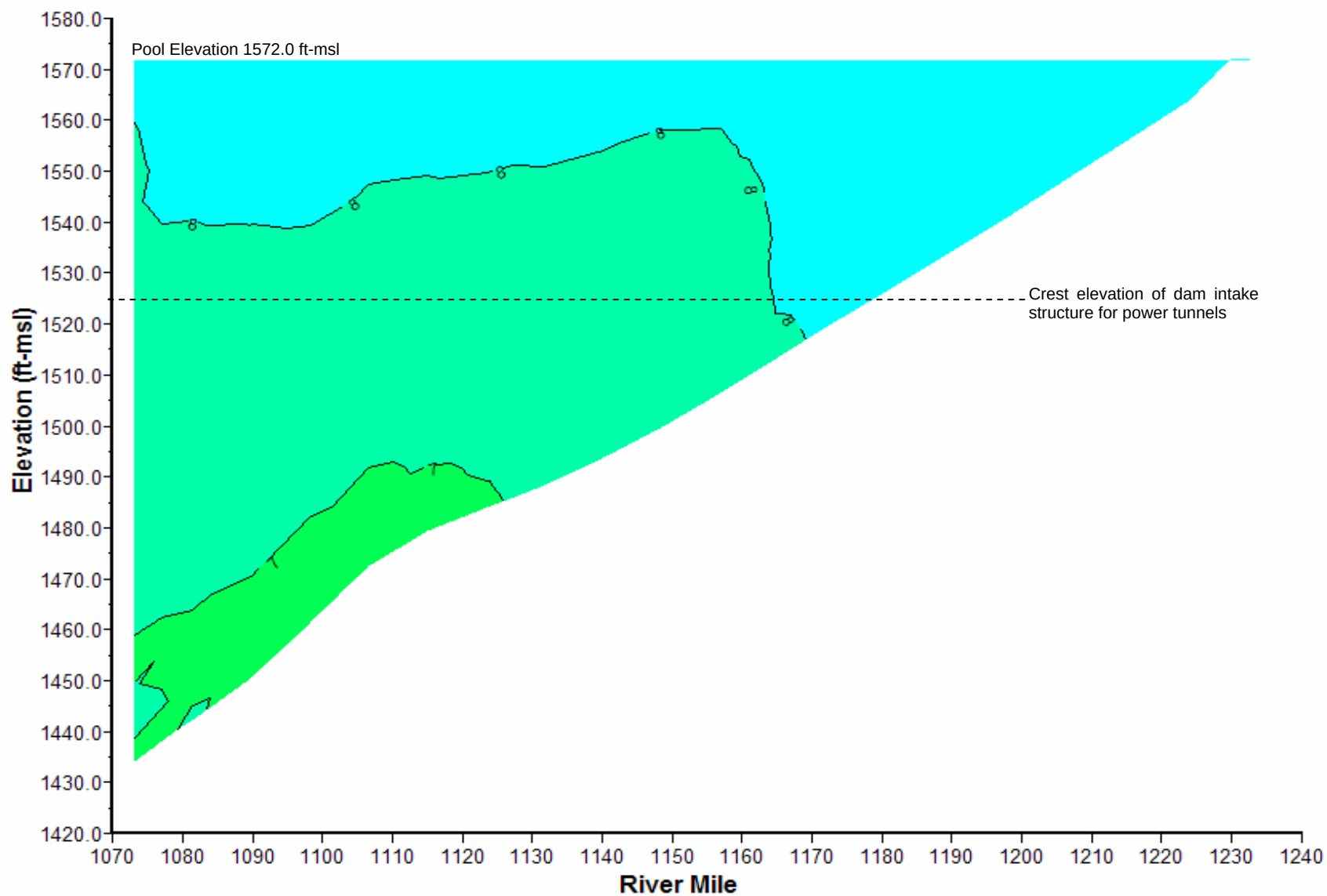
Plate 126. Longitudinal dissolved oxygen (mg/l) contour plot of Oahe Reservoir based on depth-profile dissolved oxygen concentrations measured at sites OAHRLK1073A, OAHLK1090DW, OAHLK1110DW, OAHLK1135DW, OAHLK1153DW, OAHLK1176DW, OAHLK1196DW and OAHNFMORR1 on September 19, 2006.
