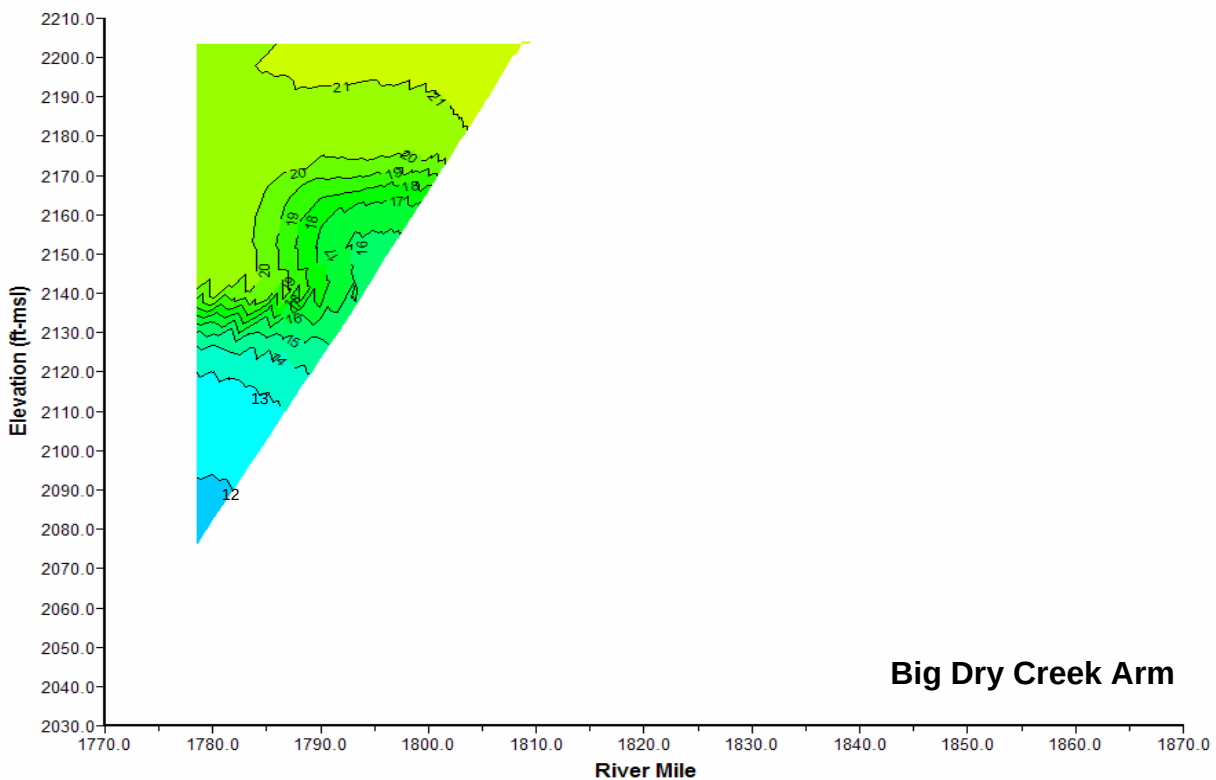
Plate 9. Longitudinal water temperature ( ^{\circ}\text{C} ) contour plot of Fort Peck Reservoir based on depth-profile water temperatures measured at sites FTPLK1772A, FTPLK1778DW, FTPLK1789DW, FTPLKBDCA01, FTPLKBDCA02, and FTPNFMORR1 on August 30, 2006.
