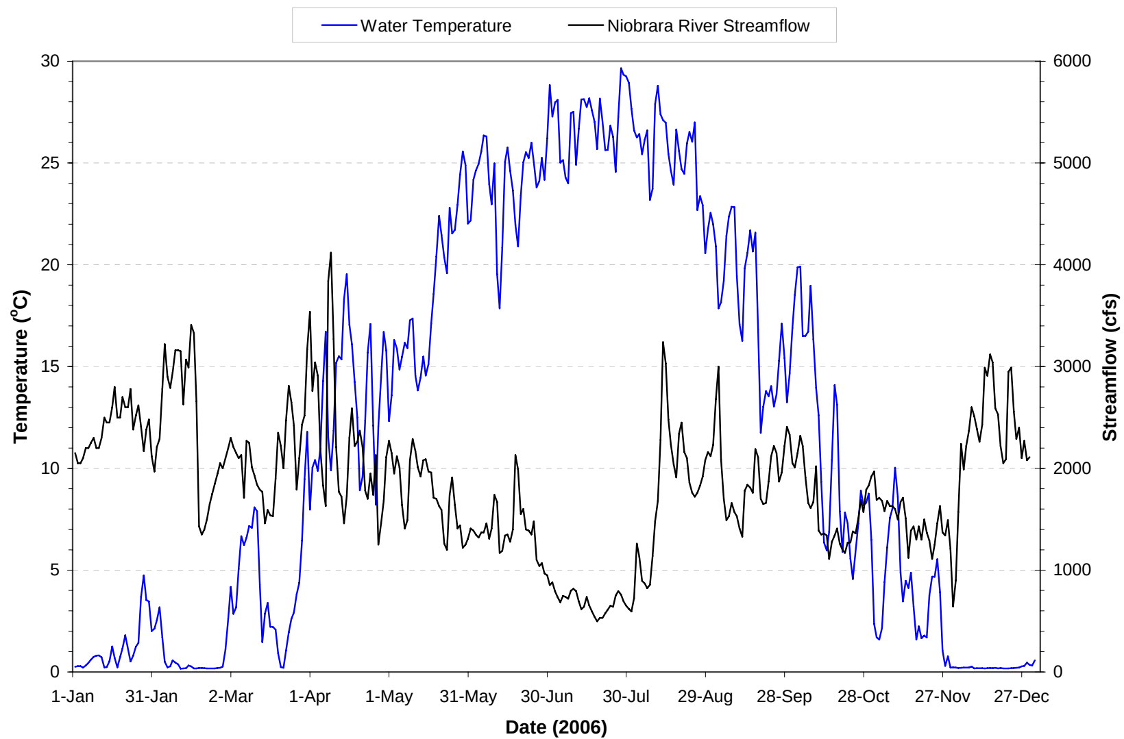
Plate 239. Mean daily water temperature and streamflow of the Niobrara River near Verdel, Nebraska (i.e., site USGS 06465500) for 2006. Mean daily temperatures and streamflows based on hourly measurements recorded at the USGS gaging station.
