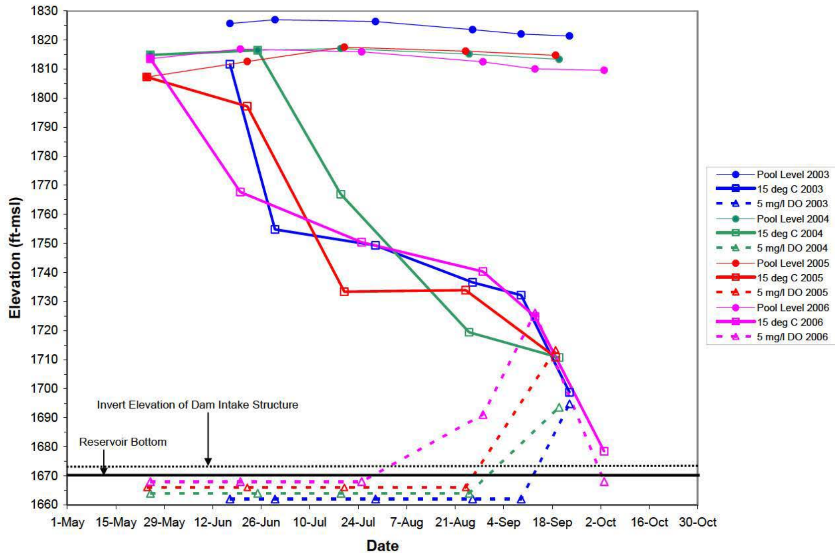
Plate 261. Elevation of the 15°C water temperature and 5 mg/l dissolved oxygen concentration isopleths for Garrison Reservoir based on water quality conditions monitored at a near-dam, deepwater location during 2003 through 2006. (Also shown are the reservoir pool elevation and the lower elevation of water withdrawal from the reservoir for power production.)
