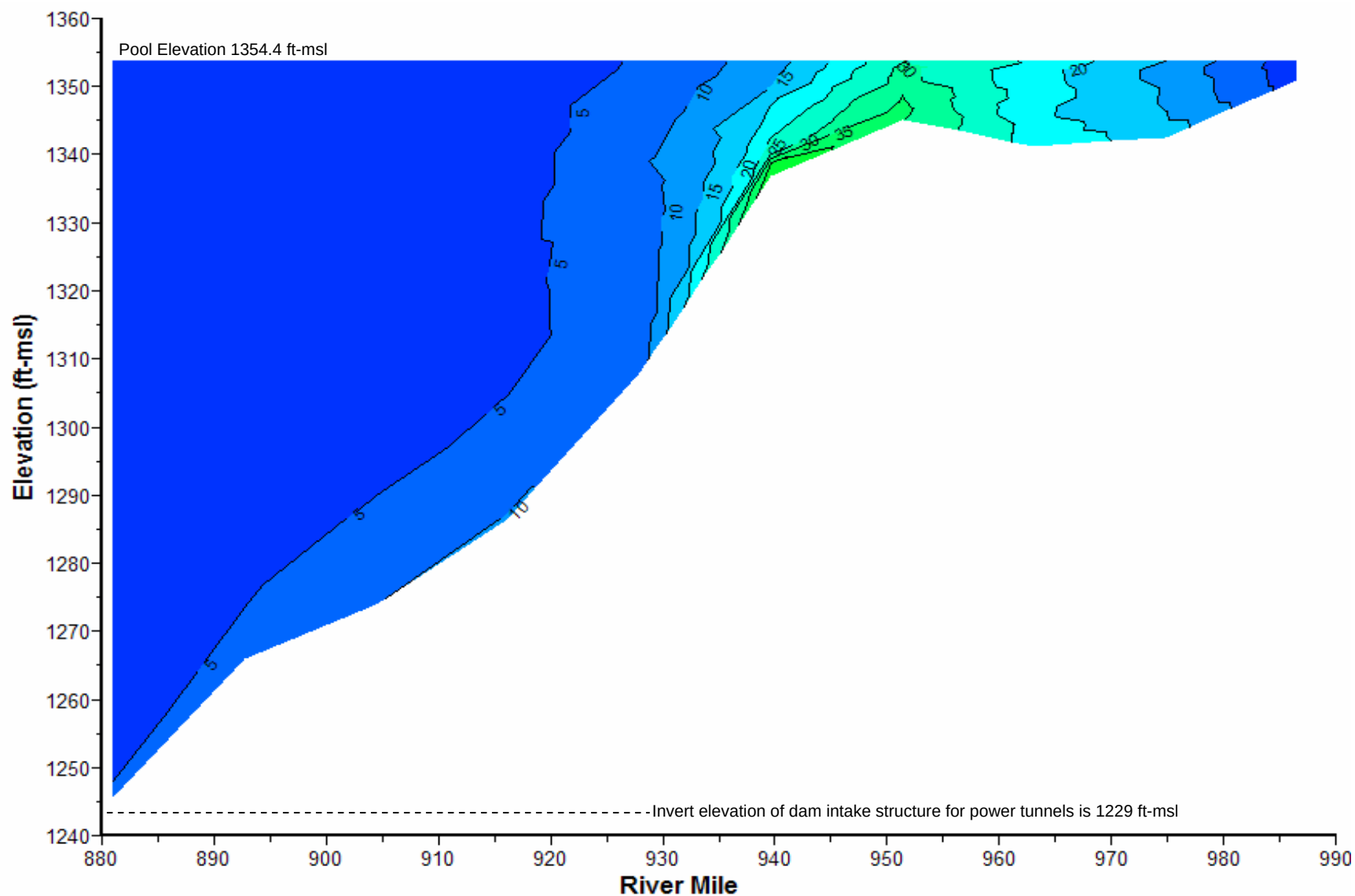
Plate 198. Longitudinal turbidity (NTU) contour plot of Fort Randall Reservoir based on depth-profile dissolved oxygen concentrations measured at sites FTRLK0880A, FTRLK0892DW, FTRLK0911DW, FTRLK0924DW, FTRLK0940DW, FTRLK0955DW, FTRLK0968DW, and BBDPP1 on June 15, 2006.
