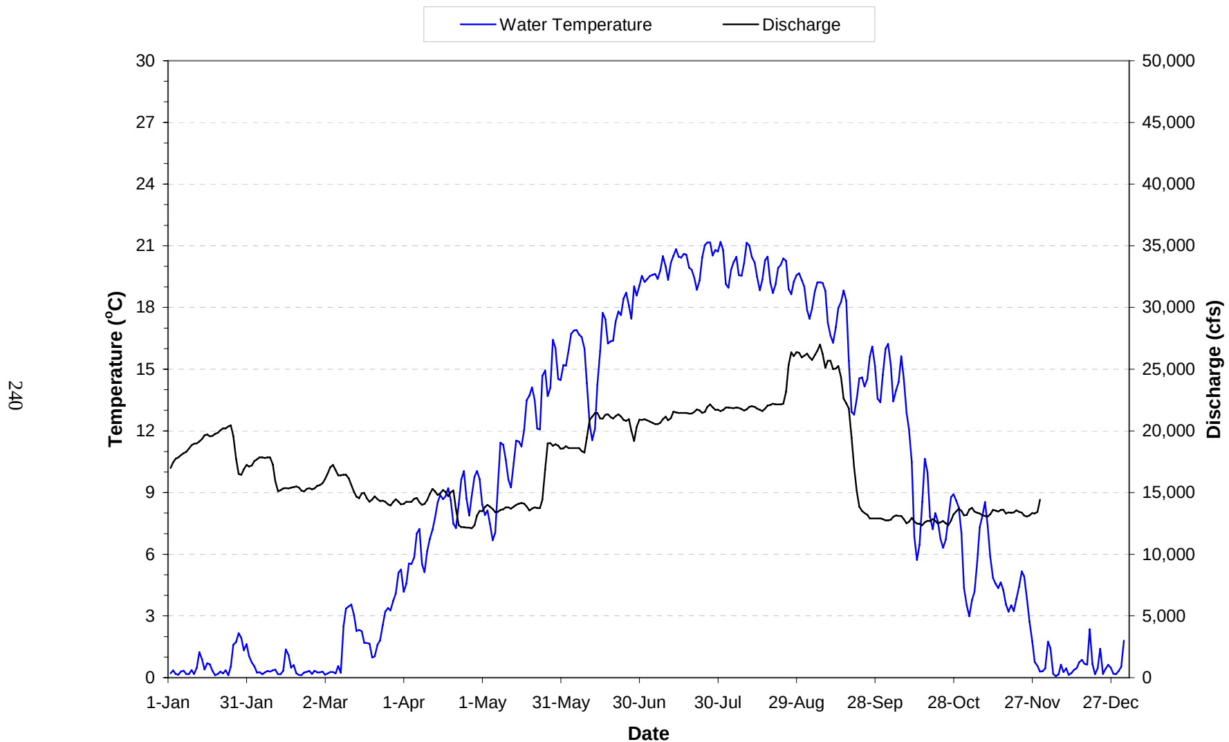
Plate 141. Mean daily water temperature and discharge of the Missouri River near Bismarck, North Dakota (i.e., site OAHNFMORR1) for 2006. Mean daily temperatures and discharges based on hourly measurements recorded on the Missouri River at Bismarck, North Dakota (USGS gaging station 06342500).
