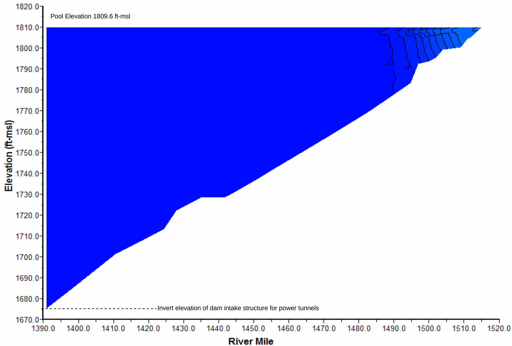
Plate 76. Longitudinal turbidity contour plot of Garrison Reservoir based on depth-profile turbidity levels monitored at sites GARLK1390A, GARLK1412DW, GARLK1445DW, GARLK1481DW, and GARNFMORRR1 on October 3, 2006.
