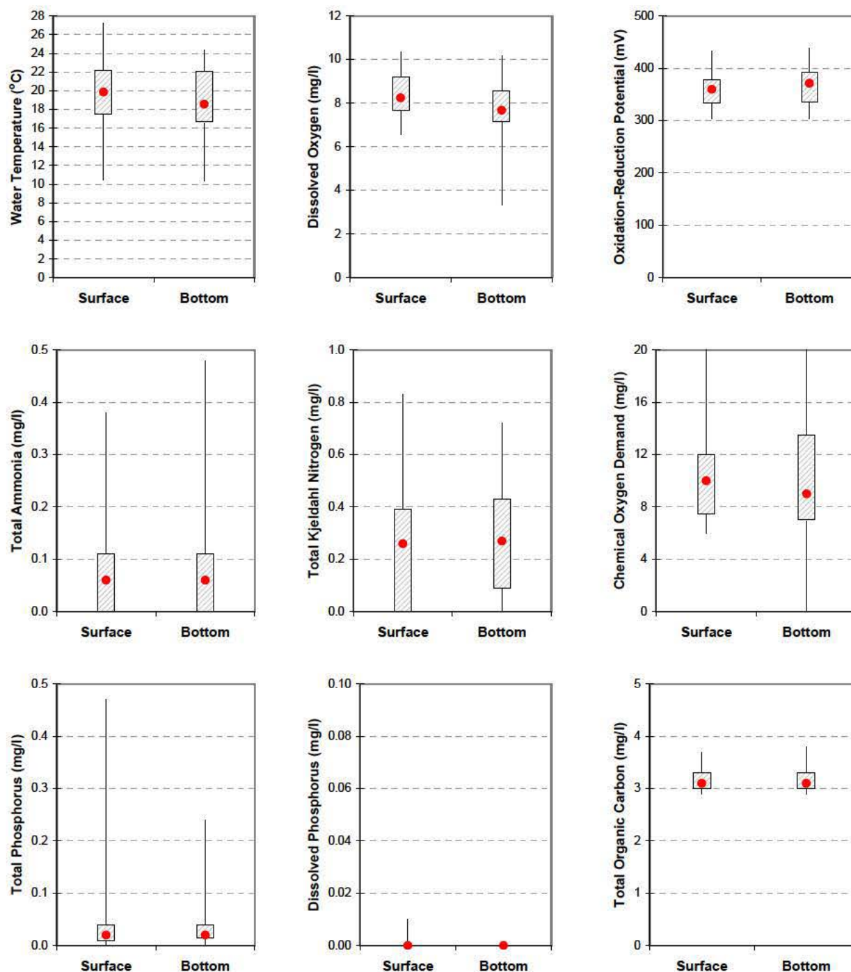
Plate 160. Box plots comparing surface and bottom water temperature, dissolved oxygen, oxidation-reduction potential, total Kjeldahl nitrogen, total ammonia nitrogen, chemical oxygen demand, total phosphorus, dissolved phosphorus, and total organic carbon measured in Big Bend Reservoir at site BBDLK0987A during the summer months of 2002 through 2006. (Box plots display minimum, 25 th percentile, 75 th percentile, and maximum. Median value is indicated by the red dot. Non-overlapping interquartile ranges of the adjacent box plots indicate a significant difference between surface and bottom measurements.)
