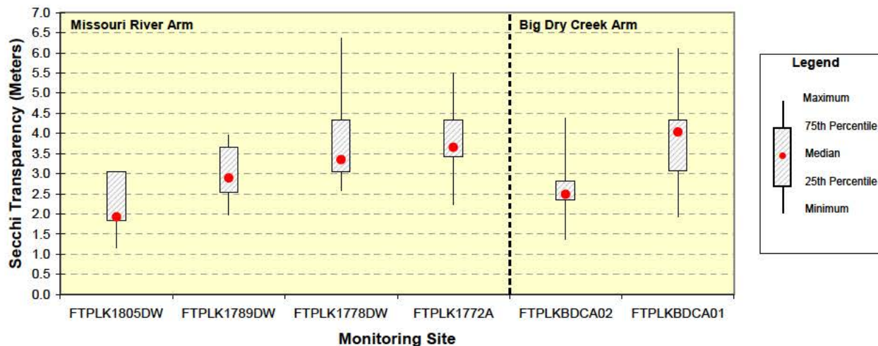
Figure 5.2. Box plot of Secchi transparencies measured in Fort Peck Reservoir during the period 2004 through 2006. (Note: monitoring sites are oriented on the x-axis in an upstream to downstream direction for both arms of the reservoir.)
