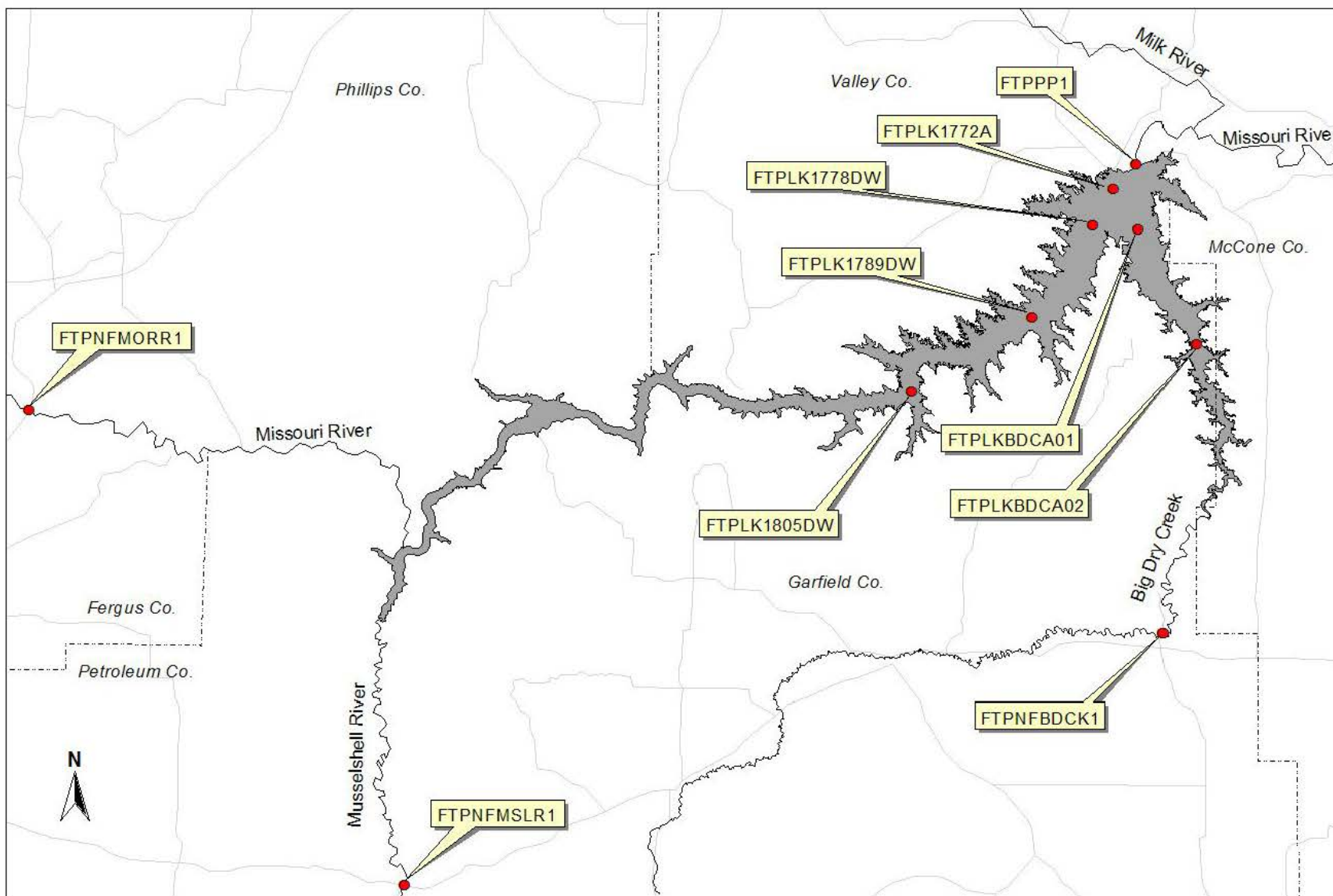
Figure 5.1. Location of sites where water quality monitoring was conducted by the District at the Fort Peck Project during the period 2002 through 2006.
