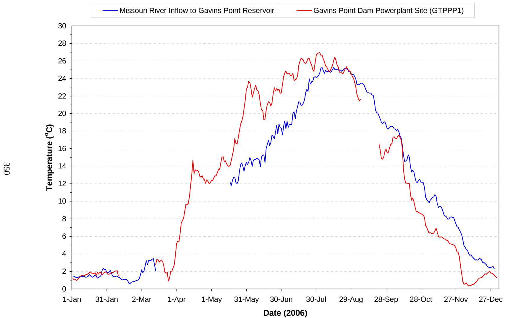
Plate 256. Mean daily water temperatures monitored at the Gavins Point Powerplant (i.e., site GT PPP1) and estimated for the Missouri River inflow to Gavins Point Reservoir during 2006. (Note: Gaps in temperature plots are periods when monitoring equipment was not operational.)
