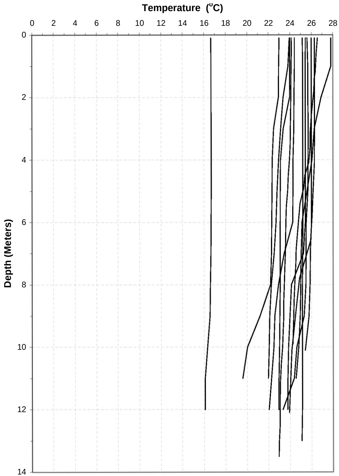
Plate 229. Temperature depth profiles for Gavins Point Reservoir generated from data collected at the near-dam, deepwater ambient monitoring site (i.e., site GPTLK0811A) during the months of July, August, and September over the 5-year period of 2002 to 2006.
