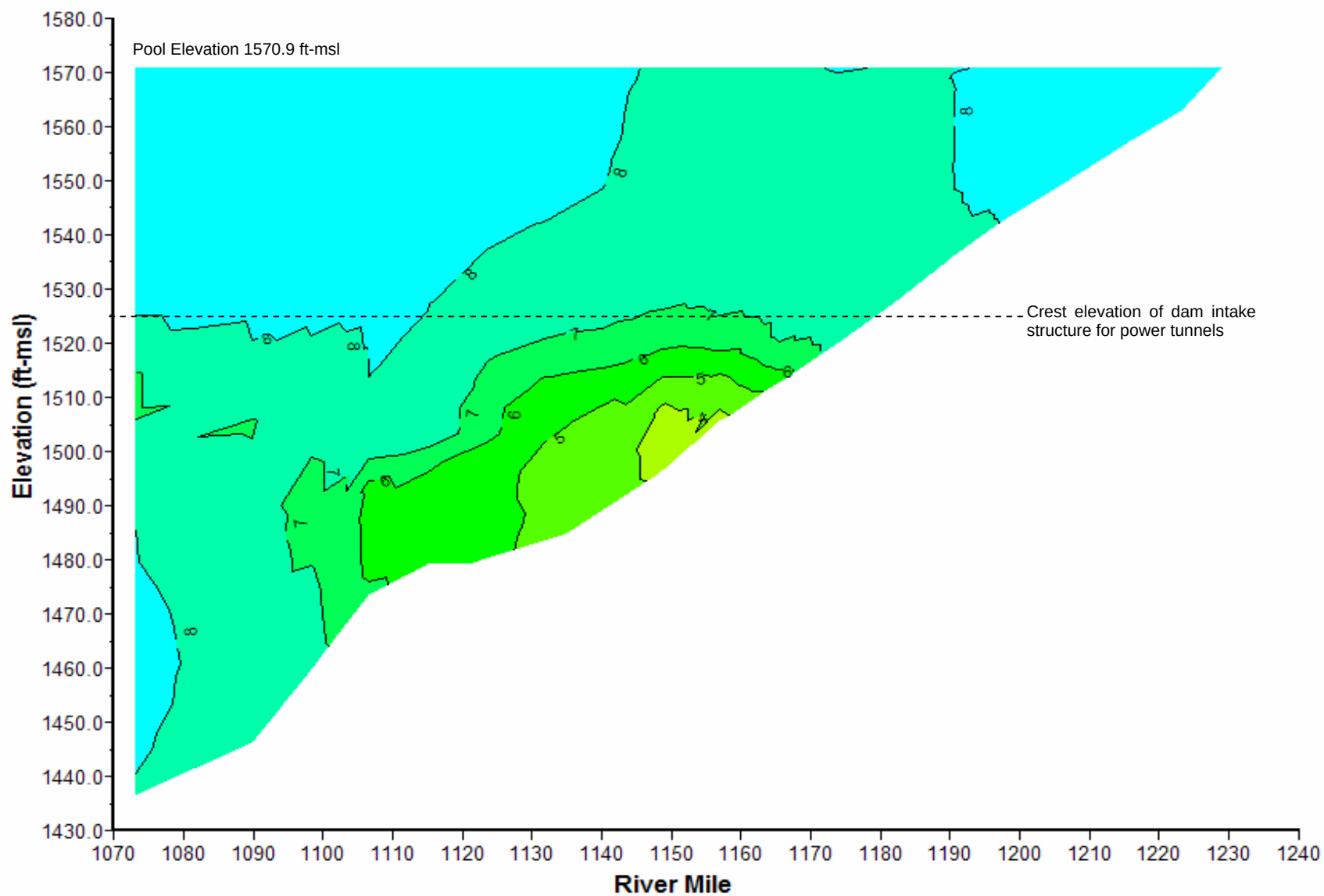
Plate 125. Longitudinal dissolved oxygen (mg/l) contour plot of Oahe Reservoir based on depth-profile dissolved oxygen concentrations measured at sites OAHRLK1073A, OAHLK1090DW, OAHLK1110DW, OAHLK1135DW, OAHLK1153DW, OAHLK1176DW, OAHLK1196DW and OAHNFMORR1 on August 23, 2006.
