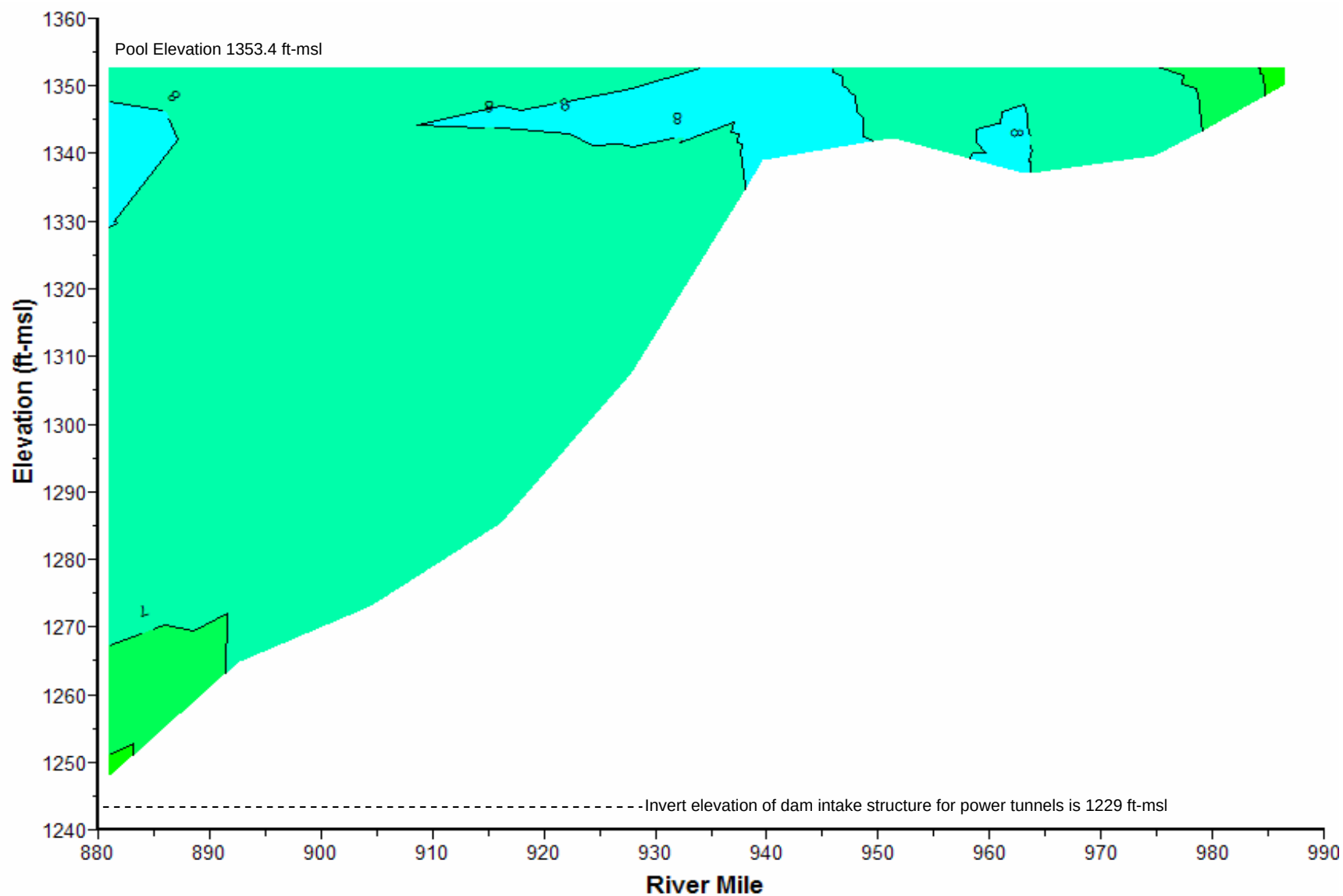
Plate 195. Longitudinal dissolved oxygen (mg/l) contour plot of Fort Randall Reservoir based on depth-profile dissolved oxygen concentrations measured at sites FTRLK0880A, FTRLK0892DW, FTRLK0911DW, FTRLK0924DW, FTRLK0940DW, FTRLK0955DW, FTRLK0968DW, and BBDPP1 on August 24, 2006.
