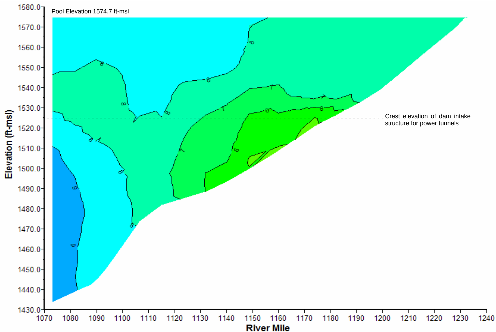
Plate 124. Longitudinal dissolved oxygen (mg/l) contour plot of Oahe Reservoir based on depth-profile dissolved oxygen concentrations measured at sites OAHRLK1073A, OAHLK1090DW, OAHLK1110DW, OAHLK1135DW, OAHLK1153DW, OAHLK1176DW, OAHLK1196DW and OAHNFMORR1 on July 19, 2006.
