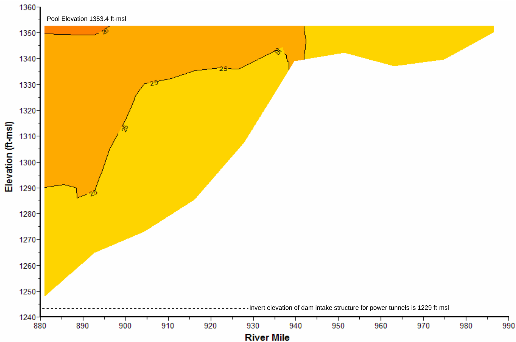
Plate 190. Longitudinal water temperature (°C) contour plot of Fort Randall Reservoir based on depth-profile water temperatures measured at sites FTRLK0880A, FTRLK0892DW, FTRLK0911DW, FTRLK0924DW, FTRLK0940DW, FTRLK0955DW, FTRLK0968DW, and BBDPP1 on August 24, 2006.
