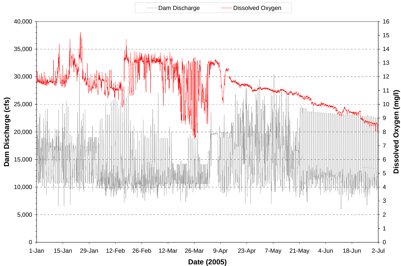
Plate 100. Hourly discharge and dissolved oxygen monitored at the Garrison powerplant on water discharged through the dam during the period January through June 2005.
