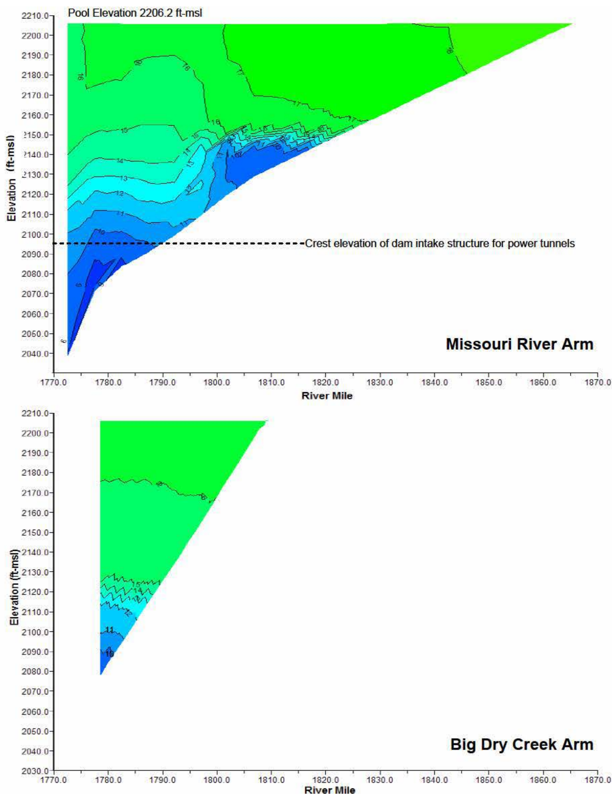
Plate 7. Longitudinal water temperature (°C) contour plot of Fort Peck Reservoir based on depth-profile water temperatures measured at sites FTPLK1772A, FTPLK1778DW, FTPLK1789DW, FTPLK1805DW, FTPLKBDCA01, FTPLKBDCA02, and FTPNFMORR1 on June 22, 2006.
