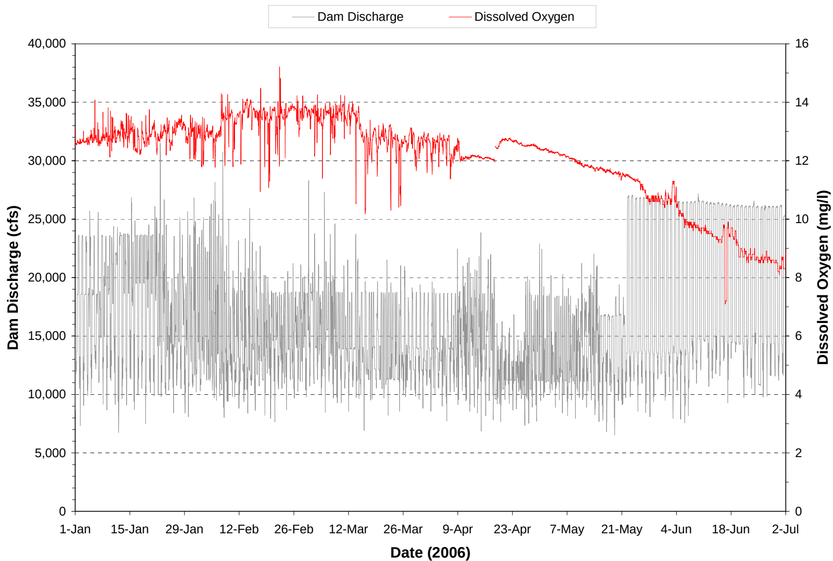
Plate 102. Hourly discharge and dissolved oxygen monitored at the Garrison powerplant on water discharged through the dam during the period January through June 2006.
