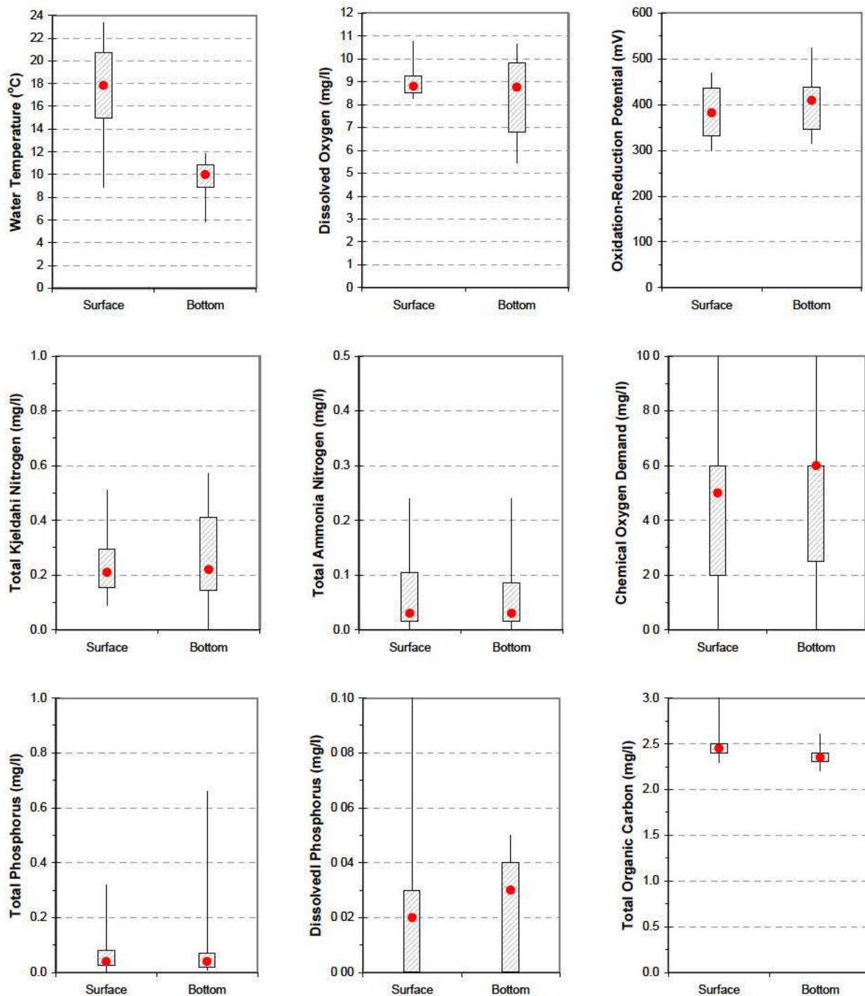
Plate 21. Box plots comparing surface and bottom water temperature, dissolved oxygen, oxidation-reduction potential, total Kjeldahl nitrogen, total ammonia nitrogen, chemical oxygen demand, total phosphorus, dissolved phosphorus, and total organic carbon measured in Fort Peck Reservoir at site FTPLK1772A during the summer months of 2004 through 2006. (Box plots display minimum, 25 th percentile, 75 th percentile, and maximum. Median value is indicated by the red dot. Non-overlapping interquartile ranges of the adjacent box plots indicate a significant difference between surface and bottom measurements.)
