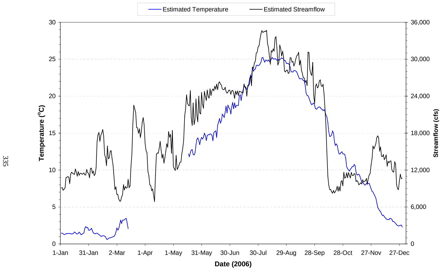
Plate 241. Mean daily water temperature and streamflow estimated for the Missouri River inflow to Gavins Point Reservoir for 2006. The mean daily discharge was estimated by adding the mean daily discharges determined for the Fort Randall Dam outflow and Niobrara River near Verdel, Nebraska at USGS gaging station 06465500. The mean daily temperature was estimated by flow weighting the mean daily water temperatures determined at the two sites. (Note: Gaps in temperature plots are periods when monitoring equipment was not operational.)
