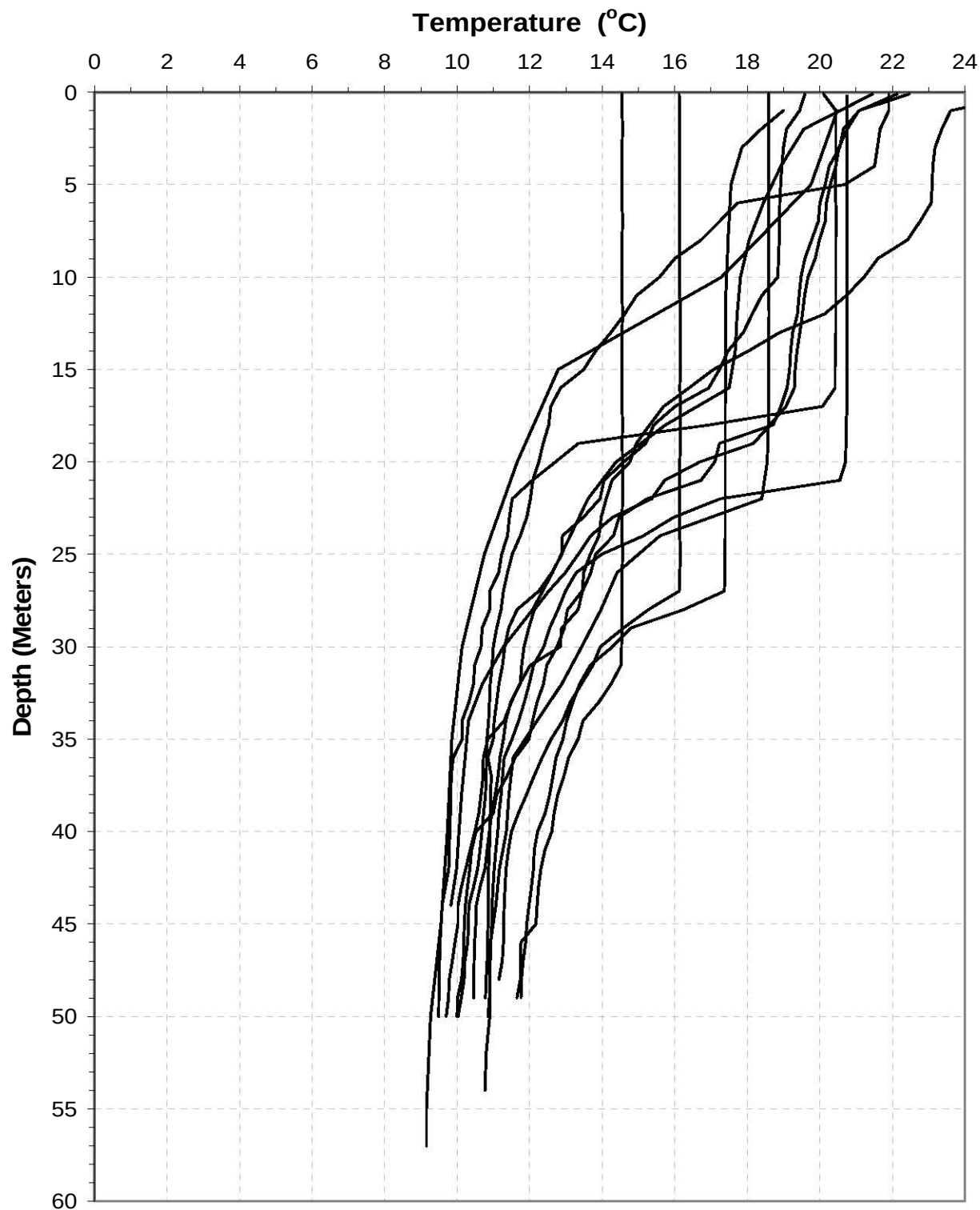
Plate 11. Temperature depth profiles for Fort Peck Reservoir compiled from data collected at the near-dam, deepwater ambient monitoring site (i.e., FTPLK1772A) during the months of July, August, and September over the 5-year period of 2002 to 2006.
