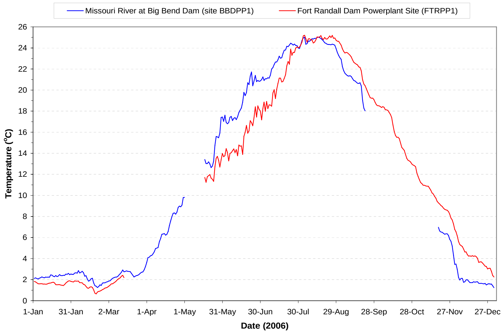
Plate 225. Mean daily water temperatures monitored at the Fort Randall Powerplant (i.e., site FTRPP1) and the Missouri River at Big Bend Dam (i.e., site BBDPP1) during 2006. (Note: Gaps in temperature plots are periods when monitoring equipment was not operational.)
