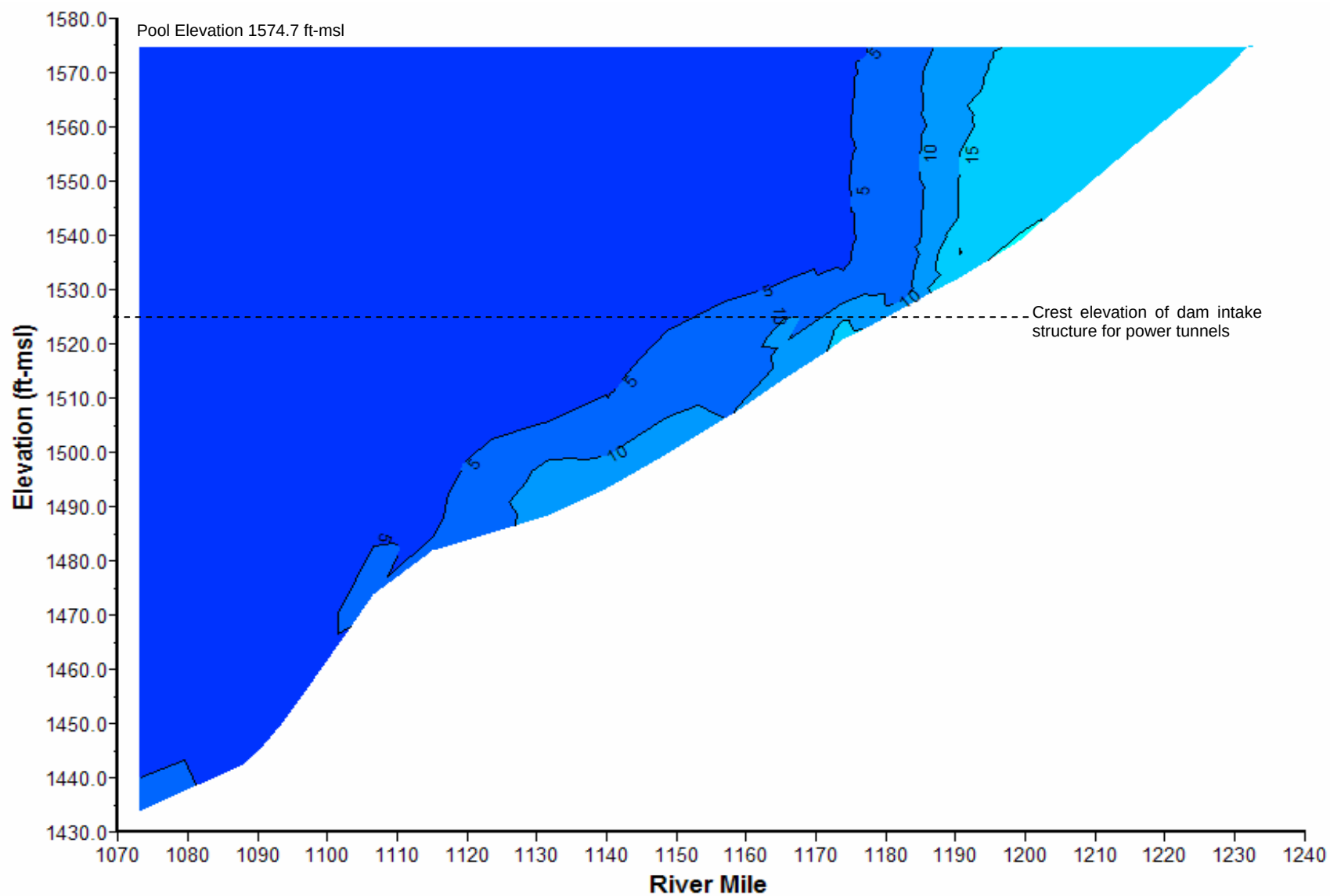
Plate 129. Longitudinal turbidity (NTU) contour plot of Oahe Reservoir based on depth-profile turbidity levels measured at sites OAHRLK1073A, OAHLK1090DW, OAHLK1110DW, OAHLK1135DW, OAHLK1153DW, OAHLK1176DW, OAHLK1196DW and OAHNFMORR1 on July 19, 2006.
