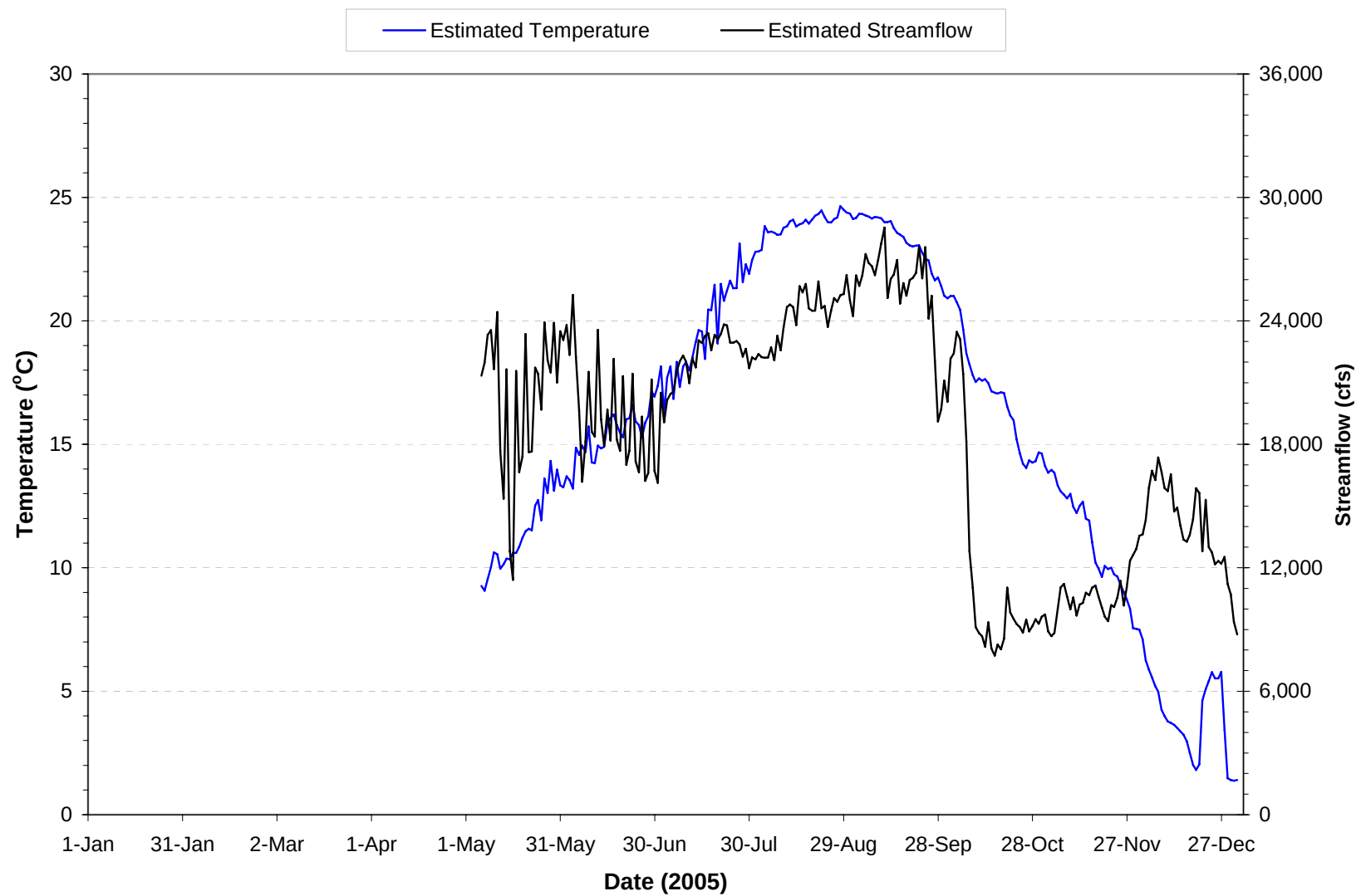
Plate 240. Mean daily water temperature and streamflow estimated for the Missouri River inflow to Gavins Point Reservoir for 2005. The mean daily discharge was estimated by adding the mean daily discharges determined for the Fort Randall Dam outflow and Niobrara River near Verdel, Nebraska at USGS gaging station 06465500. The mean daily temperature was estimated by flow weighting the mean daily water temperatures determined at the two sites.
