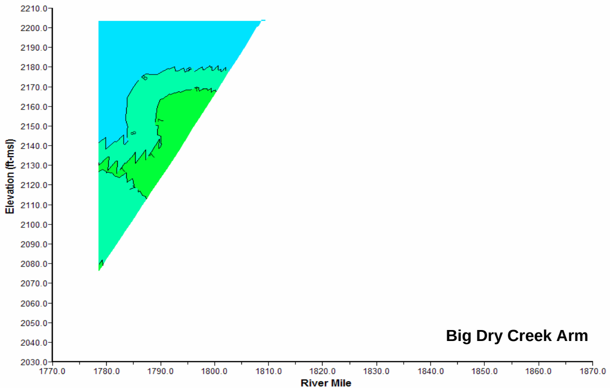
Plate 14. Longitudinal dissolved oxygen (mg/l) contour plot of Fort Peck Reservoir based on depth-profile dissolved oxygen concentrations monitored at sites FTPLK1772A, FTPLK1778DW, FTPLK1789DW, FTPLKBDCA01, FTPLKBDCA02, and FTPNFMORR1 on August 30, 2006.
