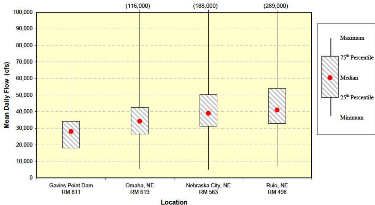
Figure 6.1. Distribution of mean daily flows recorded at gaging sites on the Missouri River at Gavins Point Dam, Omaha, NE, Nebraska City, NE, and Rulo, NE during the 40-year period of 1967 through 2006.
