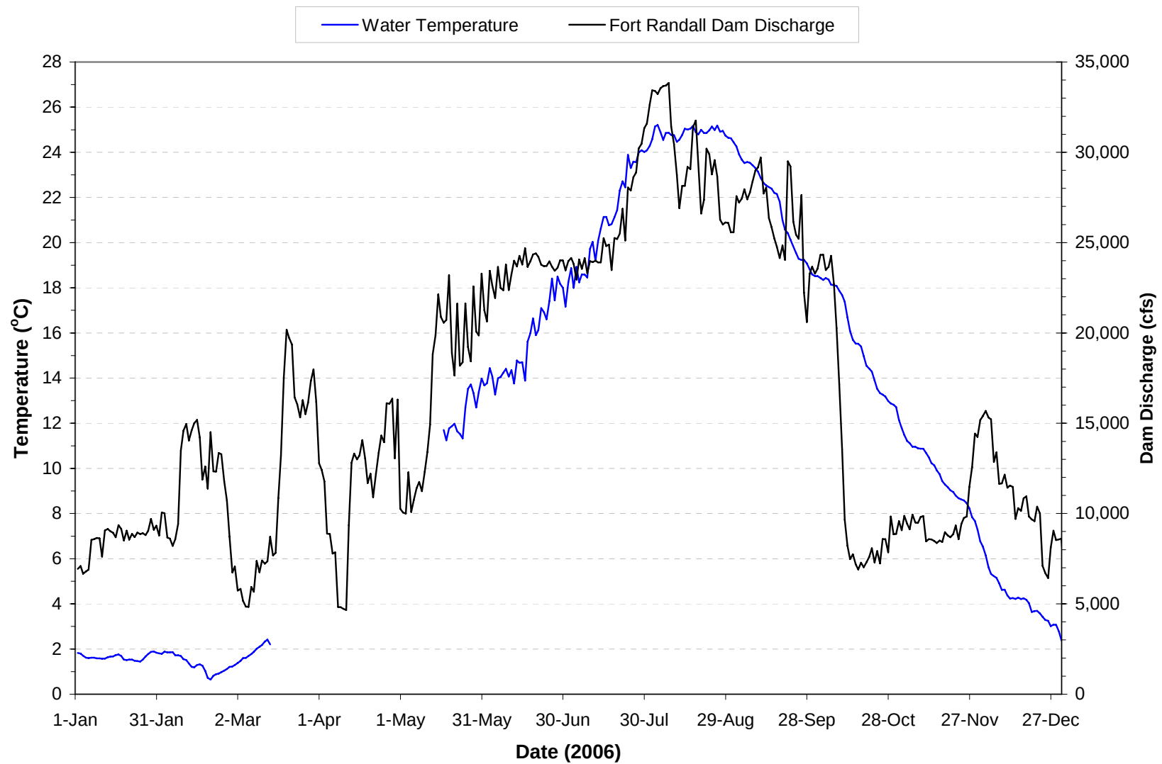
Plate 236. Mean daily water temperature and discharge of the Missouri River at Fort Randall Dam (i.e., site FTRPP1) for 2006. Mean daily temperatures and discharges based on hourly measurements recorded on discharge through Fort Randall Dam. (Note: Gaps in temperature plots are periods when monitoring equipment was not operational.)
