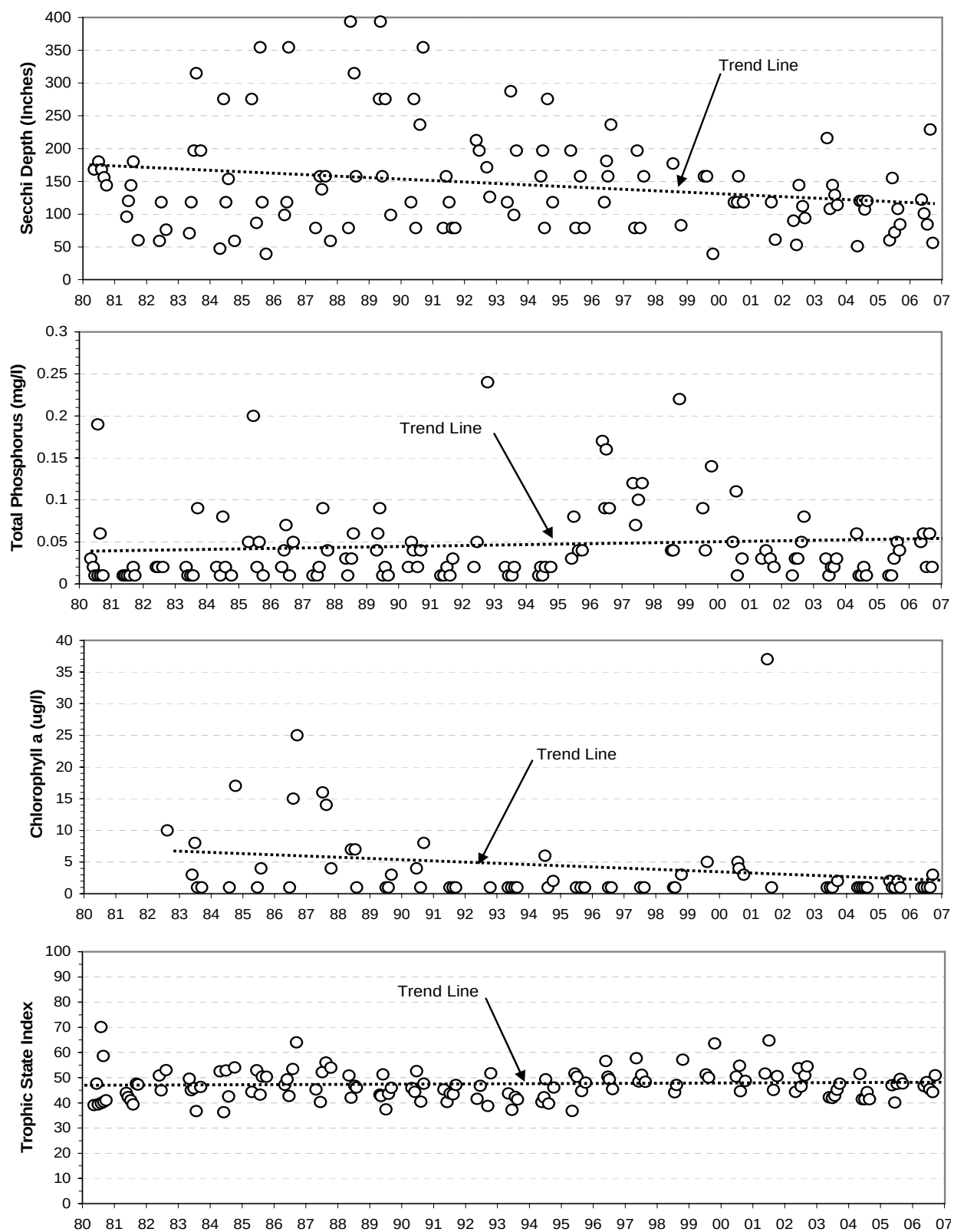
Plate 208. Historic trends for Secchi depth, total phosphorus, chlorophyll a , and Trophic State Index (TSI) monitored in Fort Randall Reservoir at the near-dam, ambient site (i.e., site FTRLK0880A) over the 27-year period of 1980 to 2006.
