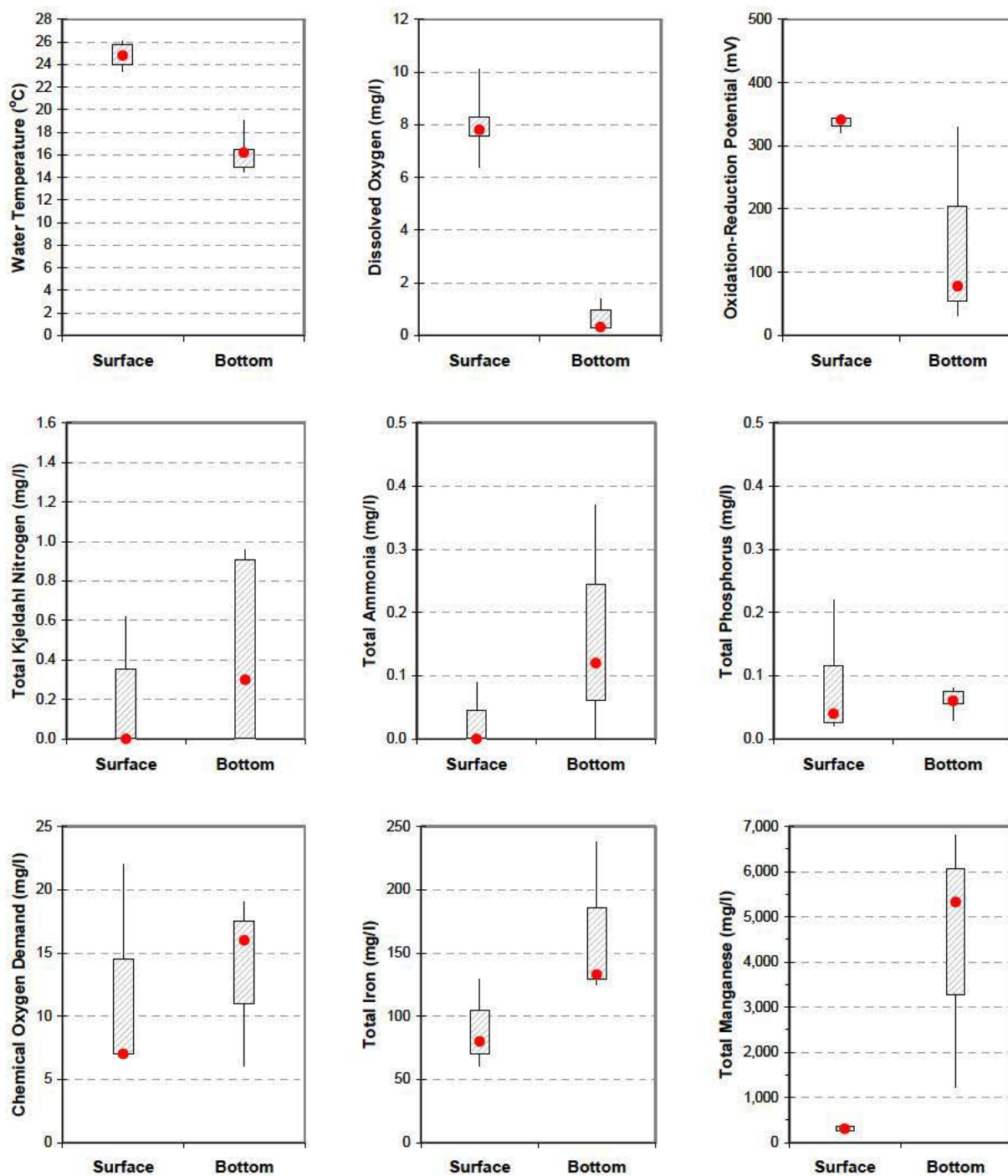
Plate 278. Box plots comparing surface and bottom water temperature, dissolved oxygen, oxidation-reduction potential, total Kjeldahl nitrogen, total ammonia nitrogen, total phosphorus, chemical oxygen demand, total iron, and total manganese measured in Lake Yankton at site YAKLKND1 during the summer months of 2002 and 2006. (Box plots display minimum, 25 th percentile, 75 th percentile, and maximum. Median value is indicated by the red dot. Non-overlapping interquartile ranges of the adjacent box plots indicate a significant difference between surface and bottom measurements.)
