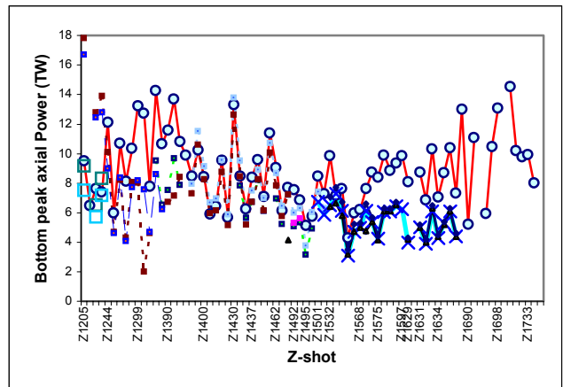
Figure 5. XRD unfold and bolometric powers for 75 Z-machine shots.
