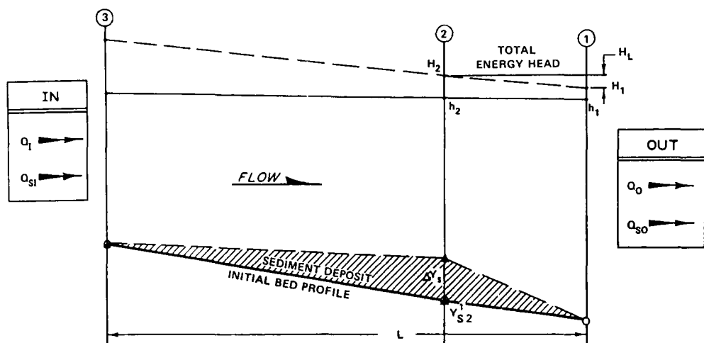
Definition Sketch for HEC-6 Modeling Computations
