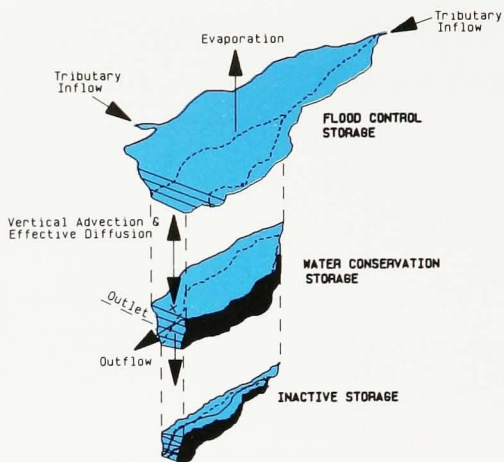
Stratified Reservoir Representation
