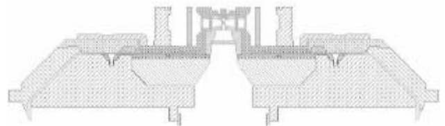
Figure 2. A disk and cone current feed with solid dielectric insulation delivers the current to the cylindrical load. Massive blocks prevent the conductors from separating during the discharge.
