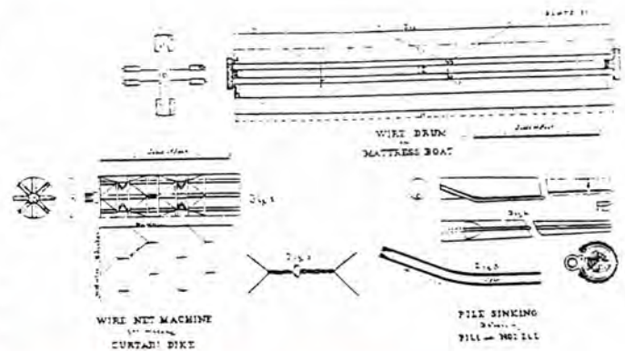
ILLUSTRATION 34. Wire net machine
