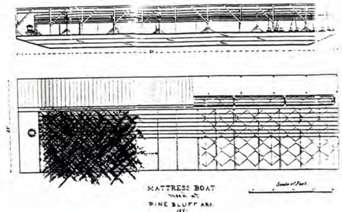
ILLUSTRATION 35. Mattress boat
