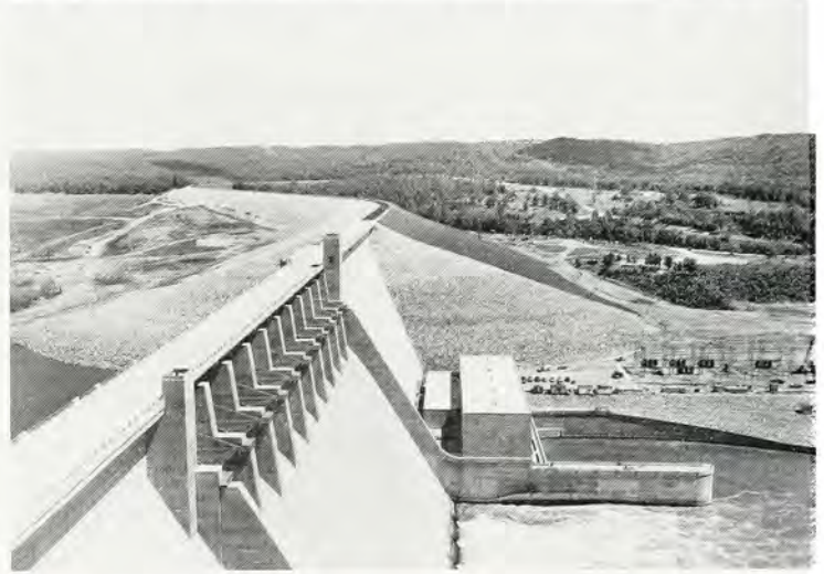
ILLUSTRATION 94. Table Rock Dam complete. Work continues on Power House and Switch Yard.
