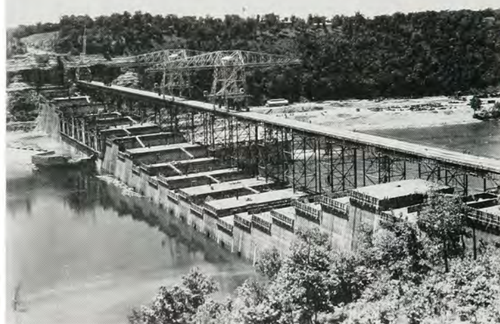
ILLUSTRATION 86. Bull Shoals Dam under construction.
