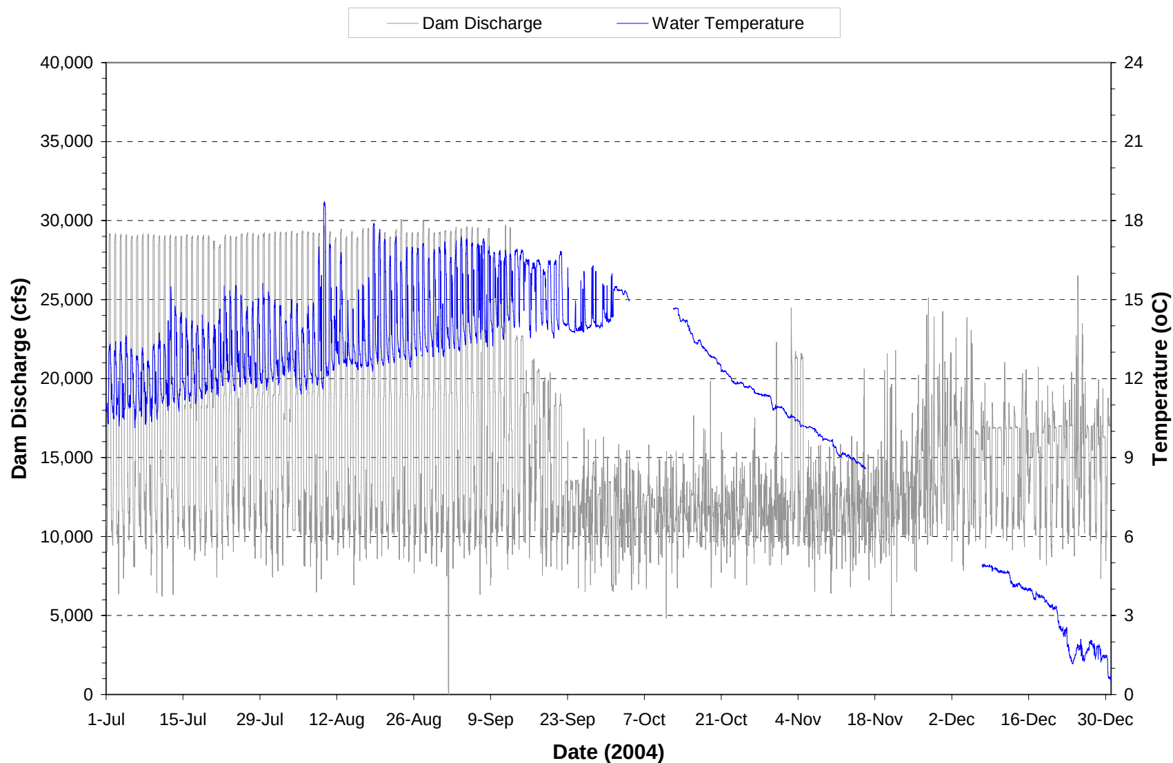
Plate 93. Hourly discharge and water temperature monitored at the Garrison powerplant on water discharged through the dam during the period July through December 2004. (Note: Gaps in temperature plot represents periods when monitoring equipment was not operational.)
