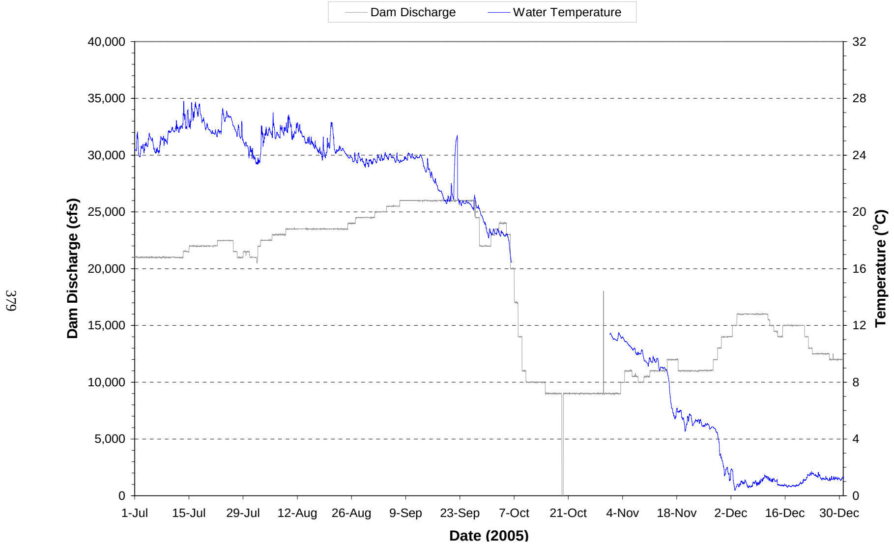
Plate 280. Hourly discharge and water temperature monitored at the Gavins Point powerplant on water discharged through the dam during the period July through December 2005. (Note: Gaps in temperature plot represents periods when monitoring equipment was not operational.)
