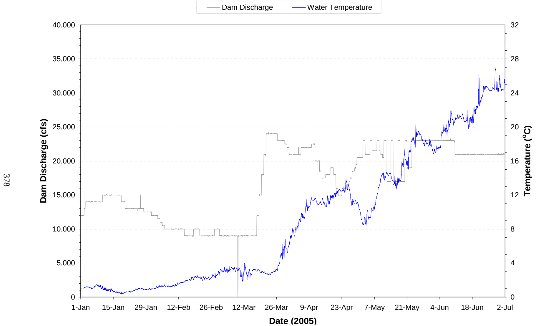
Plate 279. Hourly discharge and water temperature monitored at the Gavins Point powerplant on water discharged through the dam during the period January through June 2005. (Note: Gaps in temperature plot represents periods when monitoring equipment was not operational.)
