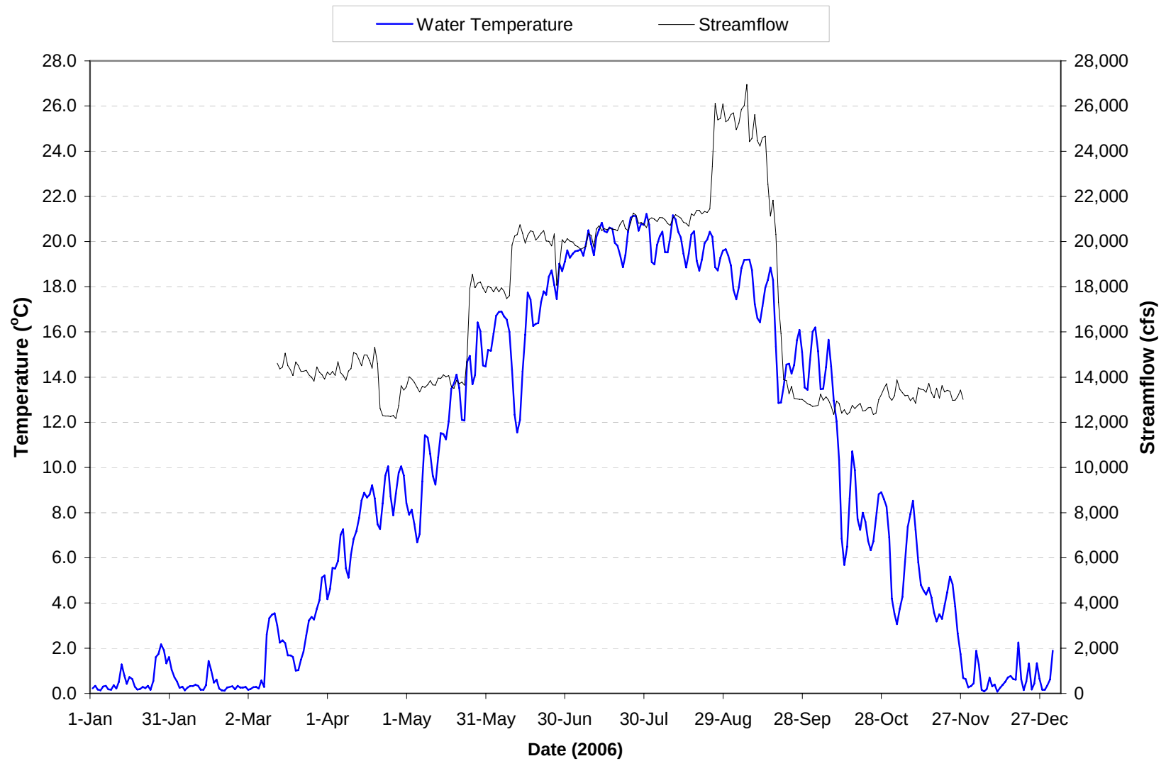
Plate 154. Mean daily water temperature and discharge of the Missouri River near Bismarck, North Dakota (i.e., site OAHNFMORR1) for 2006. Mean daily temperatures and discharges based on hourly measurements recorded on the Missouri River at Bismarck, North Dakota (USGS gaging station 06342500).
