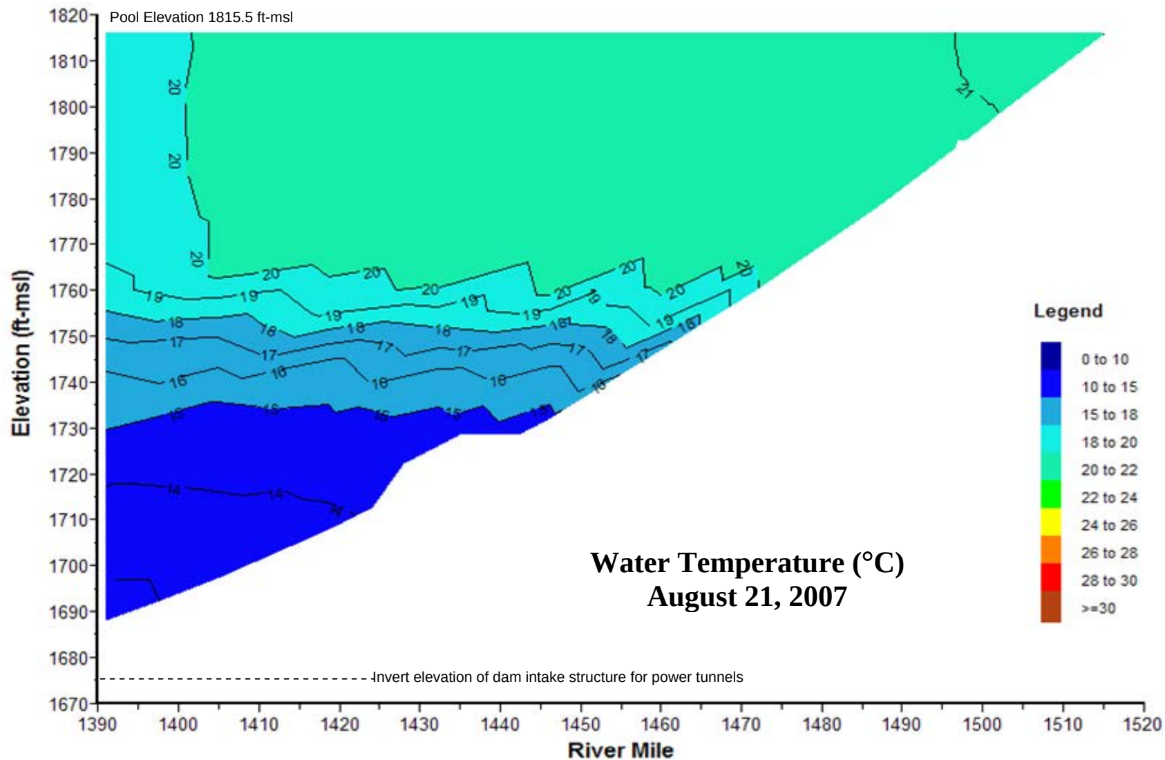
Plate 63. Longitudinal water temperature (°C) contour plot of Garrison Reservoir based on depth-profile water temperatures measured at sites GARLK1390A, GARLK1412DW, GARLK1445DW, GARLK1481DW, and GARNFMORRR1 on August 21, 2007.
