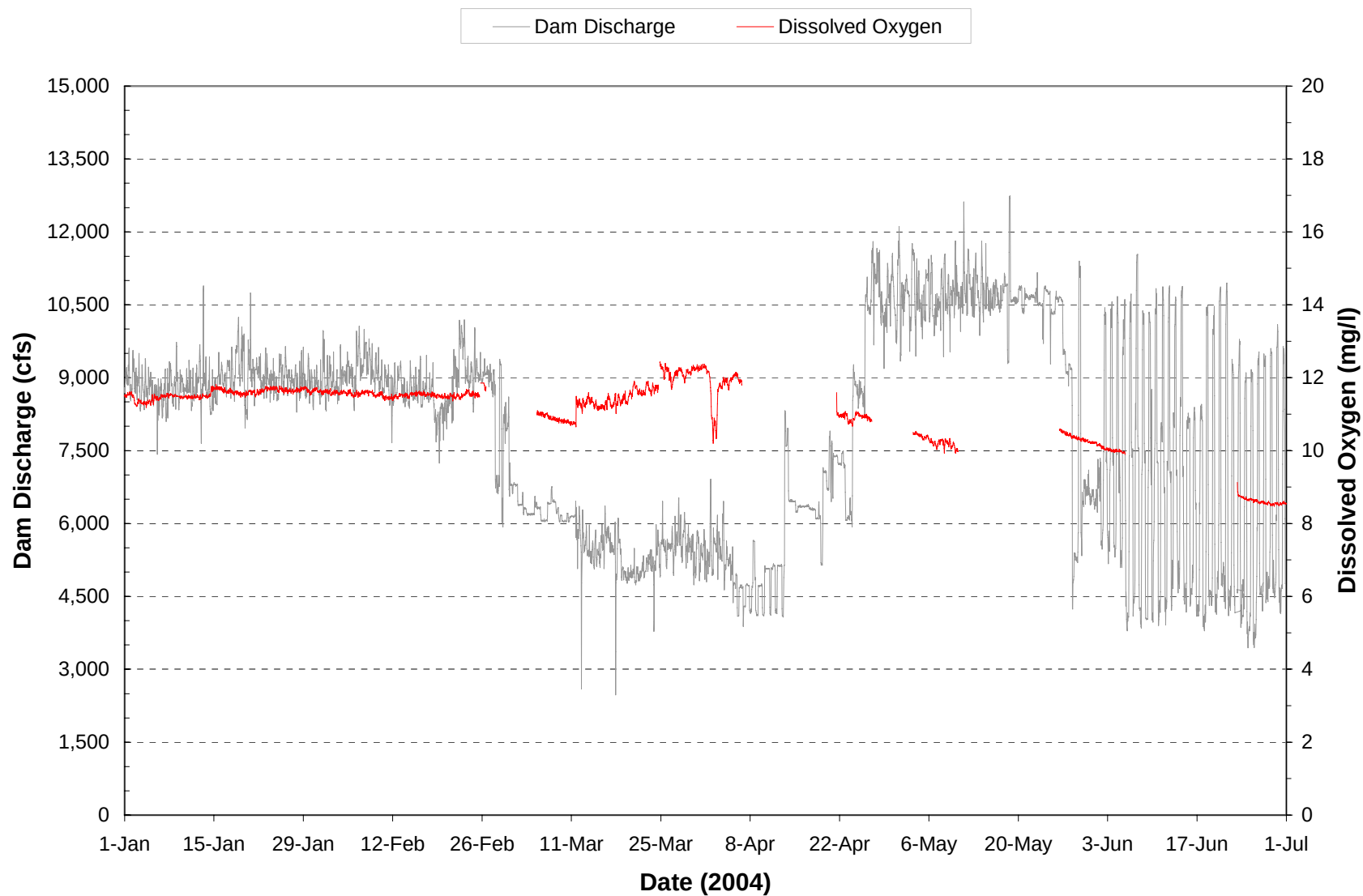
Plate 38. Hourly discharge and dissolved oxygen monitored at the Fort Peck powerplant on water discharged through the dam during the period January through June 2004. (Note: Gaps in dissolved oxygen plot represent periods when monitoring equipment was not operational.)
