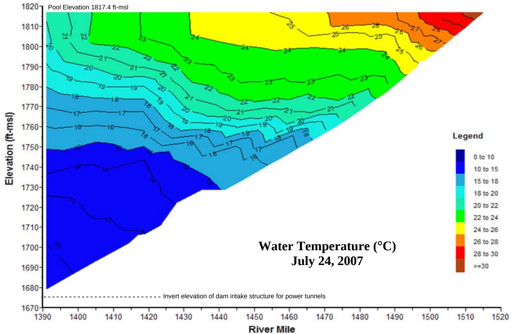
Plate 62. Longitudinal water temperature (°C) contour plot of Garrison Reservoir based on depth-profile water temperatures measured at sites GARLK1390A, GARLK1412DW, GARLK1445DW, GARLK1481DW, and GARNFMORRR1 on July 24, 2007.
