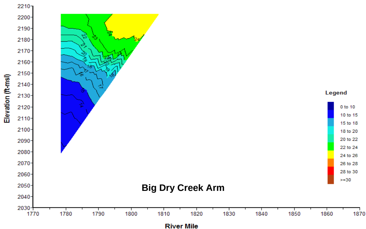
Plate 8. Longitudinal water temperature (°C) contour plot of Fort Peck Reservoir based on depth-profile water temperatures measured at sites FTPLK1772A, FTPLK1805DW, FTPLKBDCA02, and FTPNFMORR1 on July 25, 2007.
