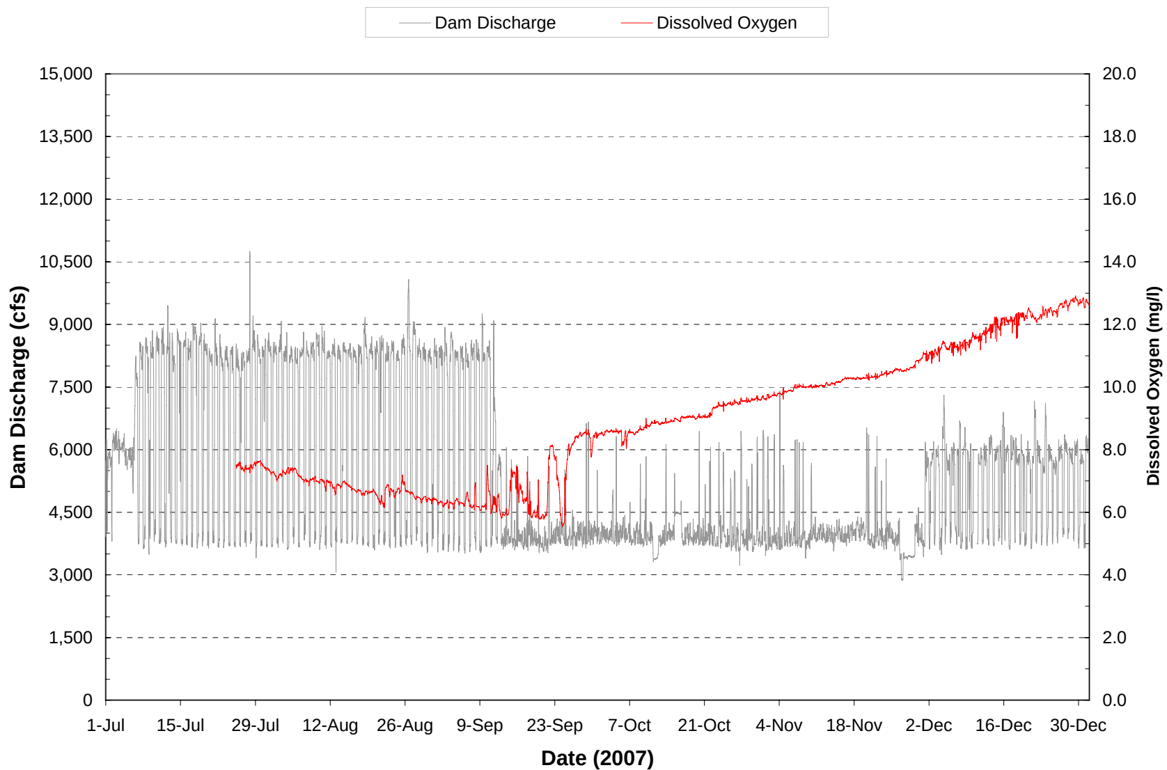
Plate 45. Hourly discharge and dissolved oxygen monitored at the Fort Peck powerplant on water discharged through the dam during the period July through December 2007. (Note: Gaps in dissolved oxygen plot represent periods when monitoring equipment was not operational.)
