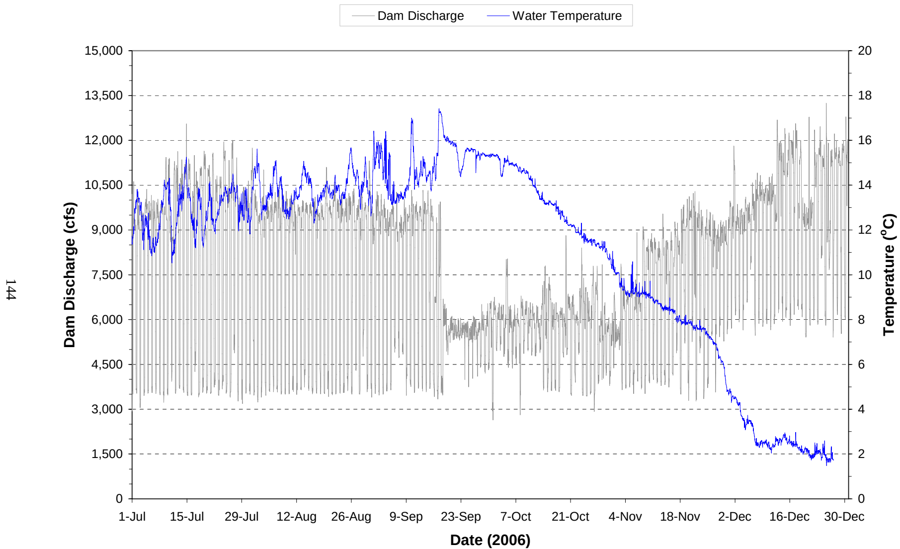
Plate 35. Hourly discharge and water temperature monitored at the Fort Peck powerplant on water discharged through the dam during the period July through December 2006. (Note: Gaps in temperature plot represents periods when monitoring equipment was not operational.)
