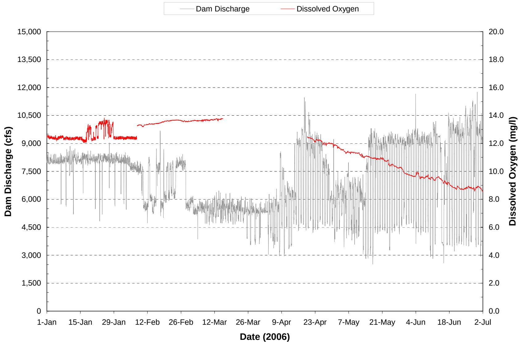
Plate 42. Hourly discharge and dissolved oxygen monitored at the Fort Peck powerplant on water discharged through the dam during the period January through June 2006. (Note: Gaps in dissolved oxygen plot represent periods when monitoring equipment was not operational.)
