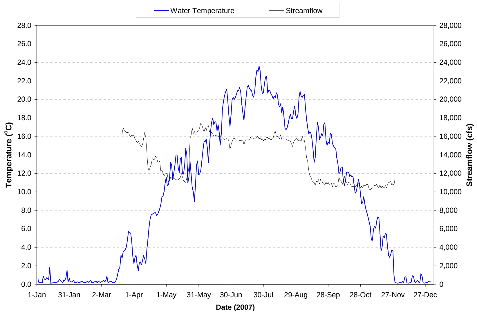
Plate 155. Mean daily water temperature and discharge of the Missouri River near Bismarck, North Dakota (i.e., site OAHNFMORR1) for 2007. Mean daily temperatures and discharges based on hourly measurements recorded on the Missouri River at Bismarck, North Dakota (USGS gaging station 06342500).
