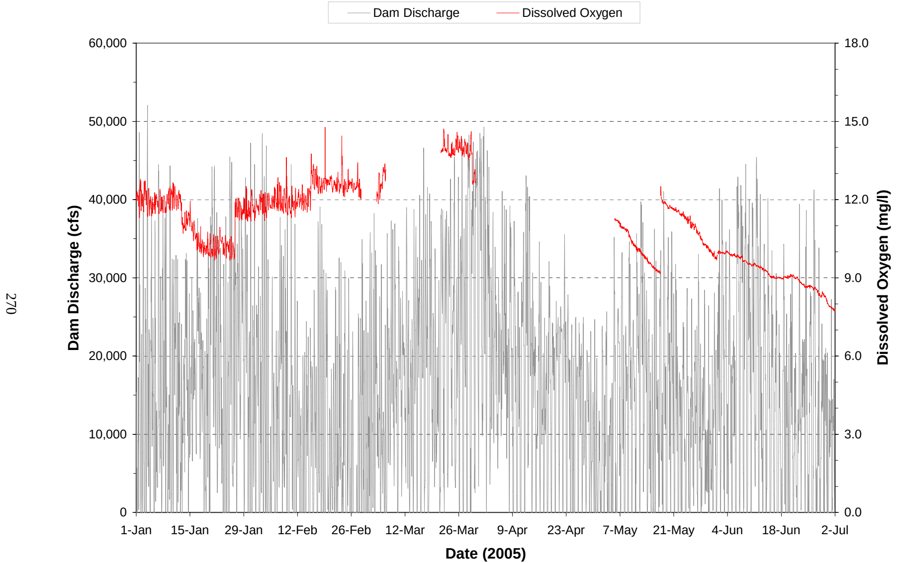
Plate 167. Hourly discharge and dissolved oxygen monitored at the Oahe powerplant on water discharged through the dam during the period January through June 2005. (Note: Gaps in dissolved oxygen plot represents periods when monitoring equipment was not operational.)
