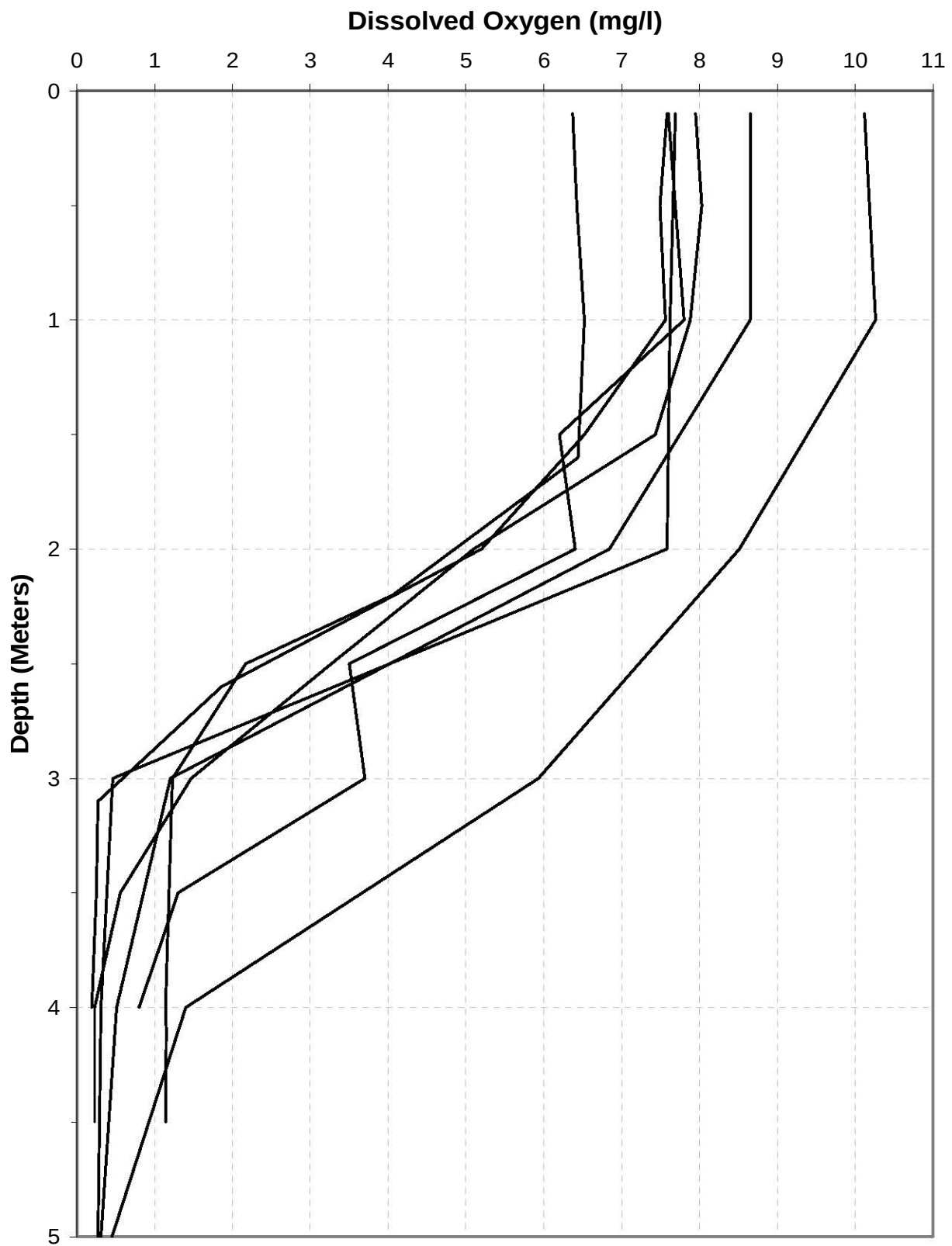
Plate 316. Dissolved oxygen depth profiles for Lake Yankton generated from data collected at the deepwater ambient monitoring site during the summer months of 2002 and 2006.
