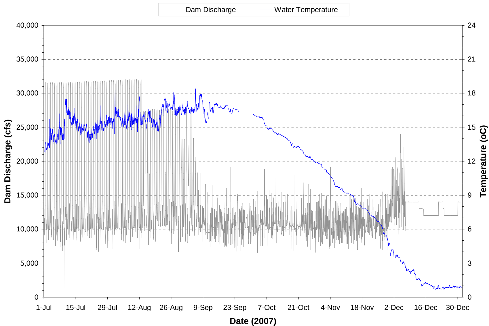
Plate 99. Hourly discharge and water temperature monitored at the Garrison powerplant on water discharged through the dam during the period July through December 2007. (Note: Gaps in temperature plot represents periods when monitoring equipment was not operational.)
