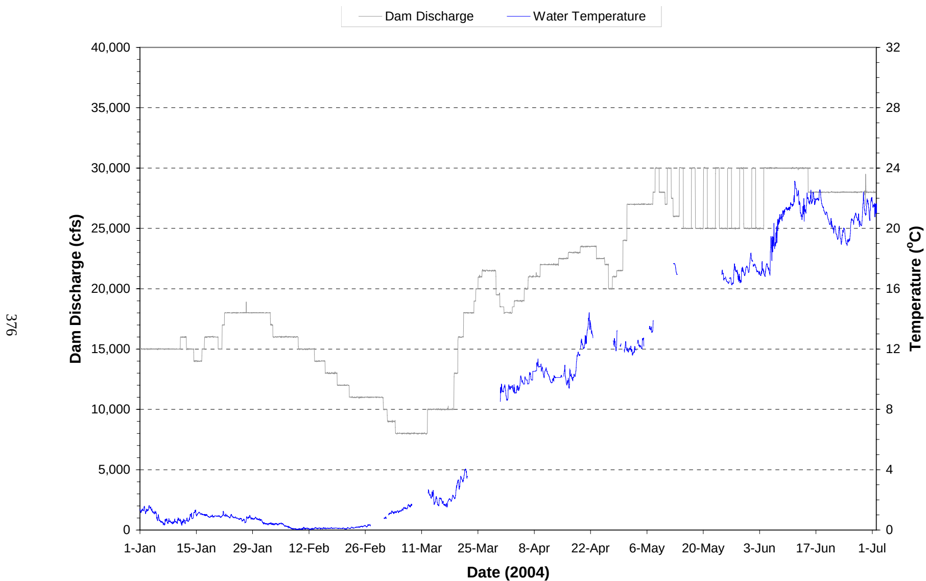
Plate 277. Hourly discharge and water temperature monitored at the Gavins Point powerplant on water discharged through the dam during the period January through June 2004. (Note: Gaps in temperature plot represents periods when monitoring equipment was not operational.)
