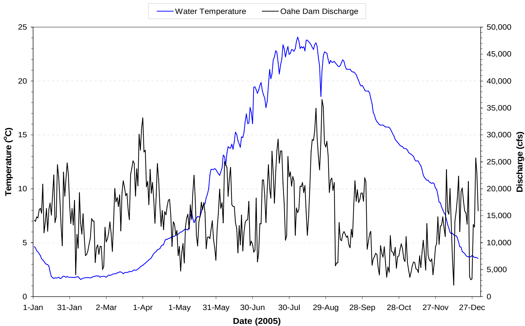
Plate 183. Mean daily water temperature and discharge of the Missouri River at Oahe Dam (i.e., site OAHPP1) for 2005. Mean daily temperatures and discharges based on hourly measurements recorded on discharge through Oahe Dam.
