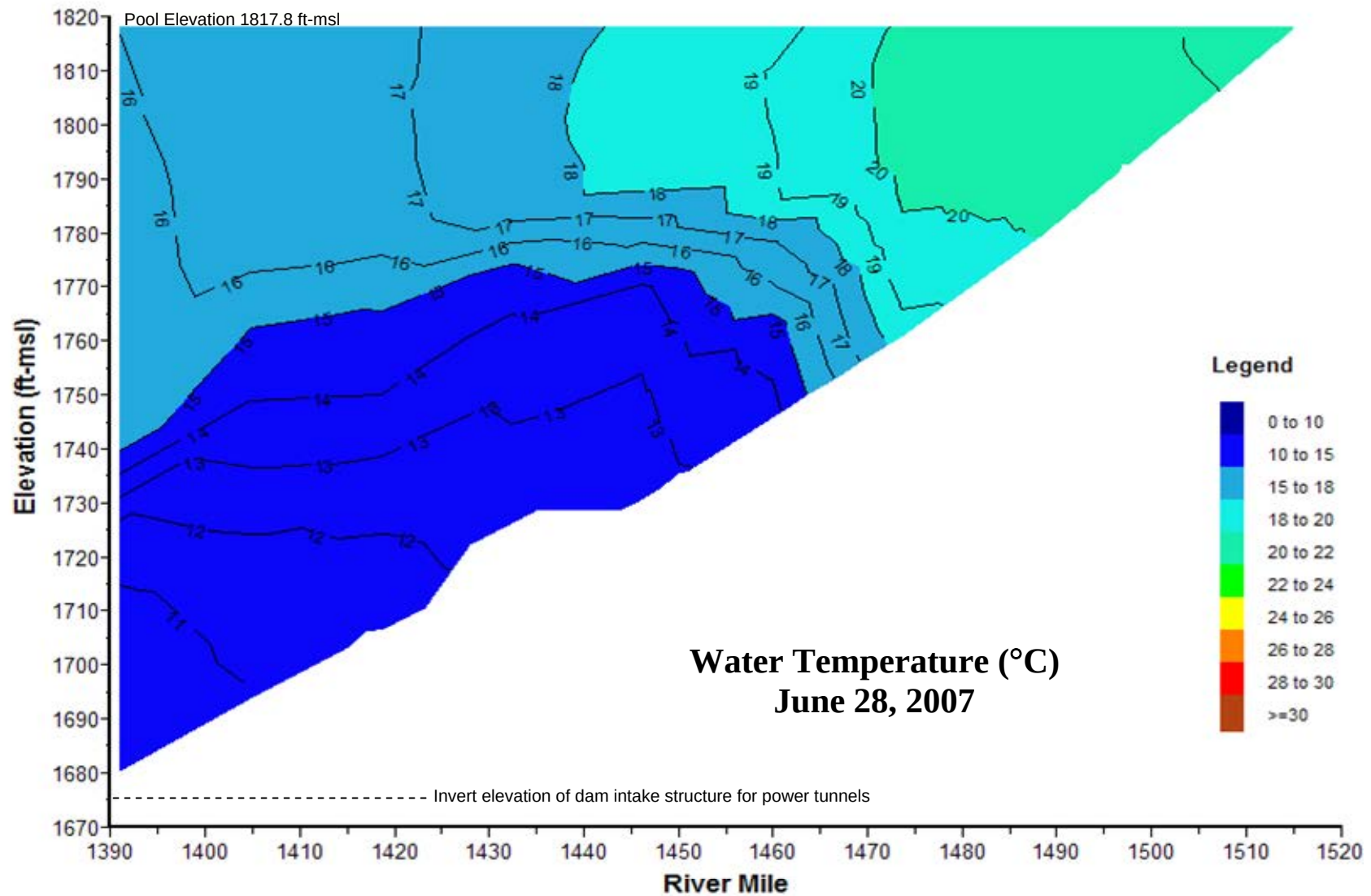
Plate 61. Longitudinal water temperature (°C) contour plot of Garrison Reservoir based on depth-profile water temperatures measured at sites GARLK1390A, GARLK1412DW, GARLK1445DW, GARLK1481DW, and GARNFMORRR1 on June 28, 2007.
