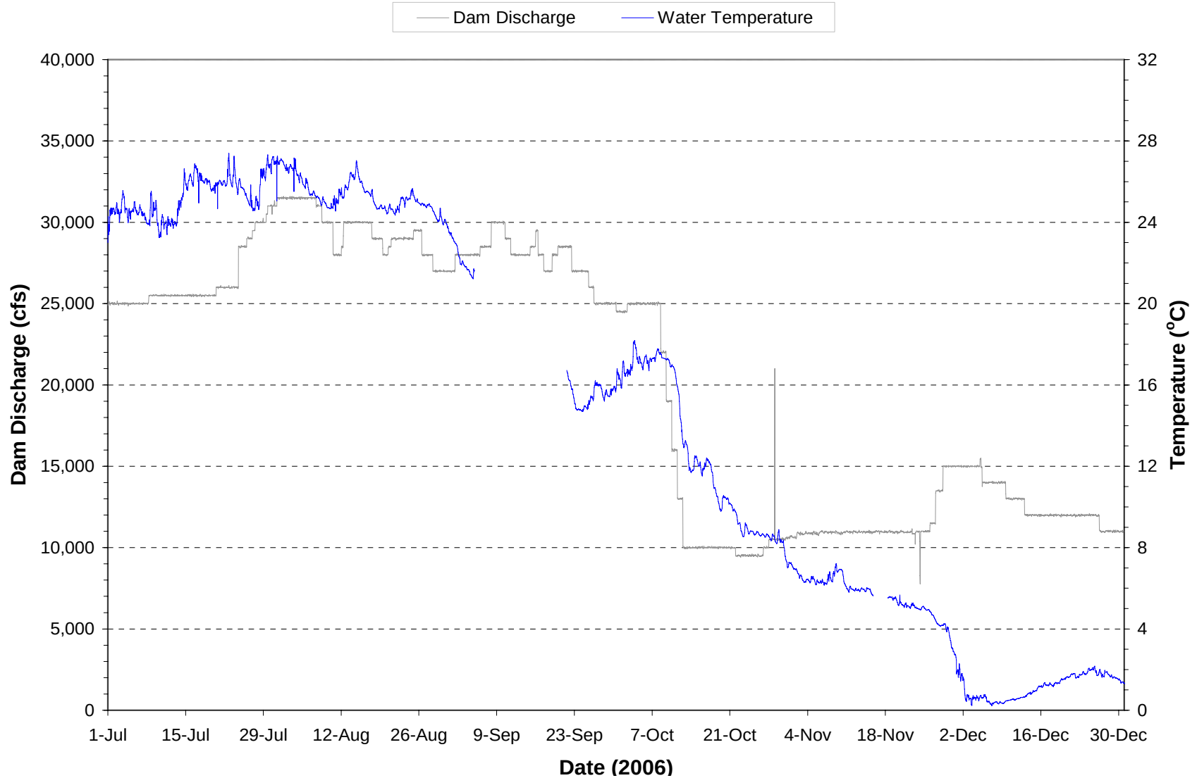
Plate 282. Hourly discharge and water temperature monitored at the Gavins Point powerplant on water discharged through the dam during the period July through December 2006. (Note: Gaps in temperature plot represents periods when monitoring equipment was not operational.)
