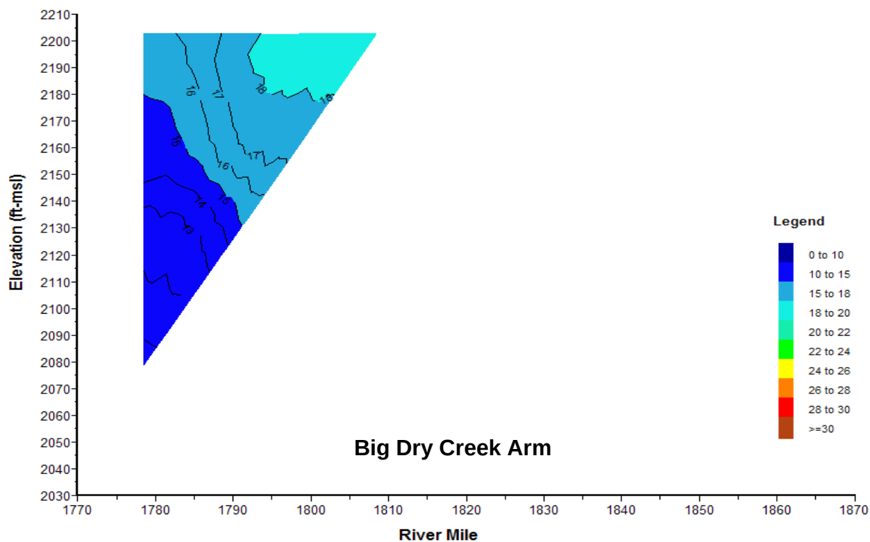
Plate 7. Longitudinal water temperature ( ^{\circ}\text{C} ) contour plot of Fort Peck Reservoir based on depth-profile water temperatures measured at sites FTPLK1772A, FTPLK1805DW, FTPLKBDCA02, and FTPNFMORR1 on June 26, 2007.
