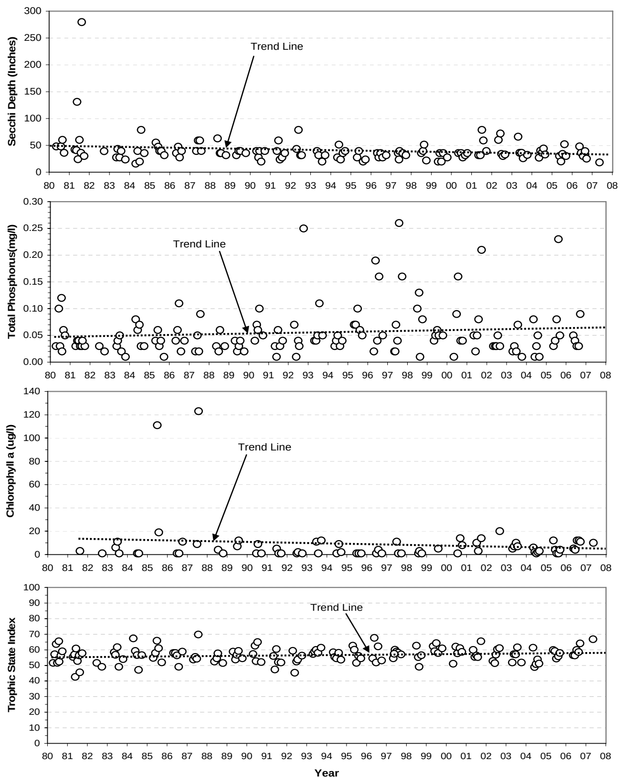
Plate 265. Historic trends for Secchi depth, total phosphorus, chlorophyll a , and Trophic State Index (TSI) monitored in Gavins Point Reservoir at the near-dam, ambient site (i.e., site GTPLK0811A) over the 28-year period of 1980 to 2007.
