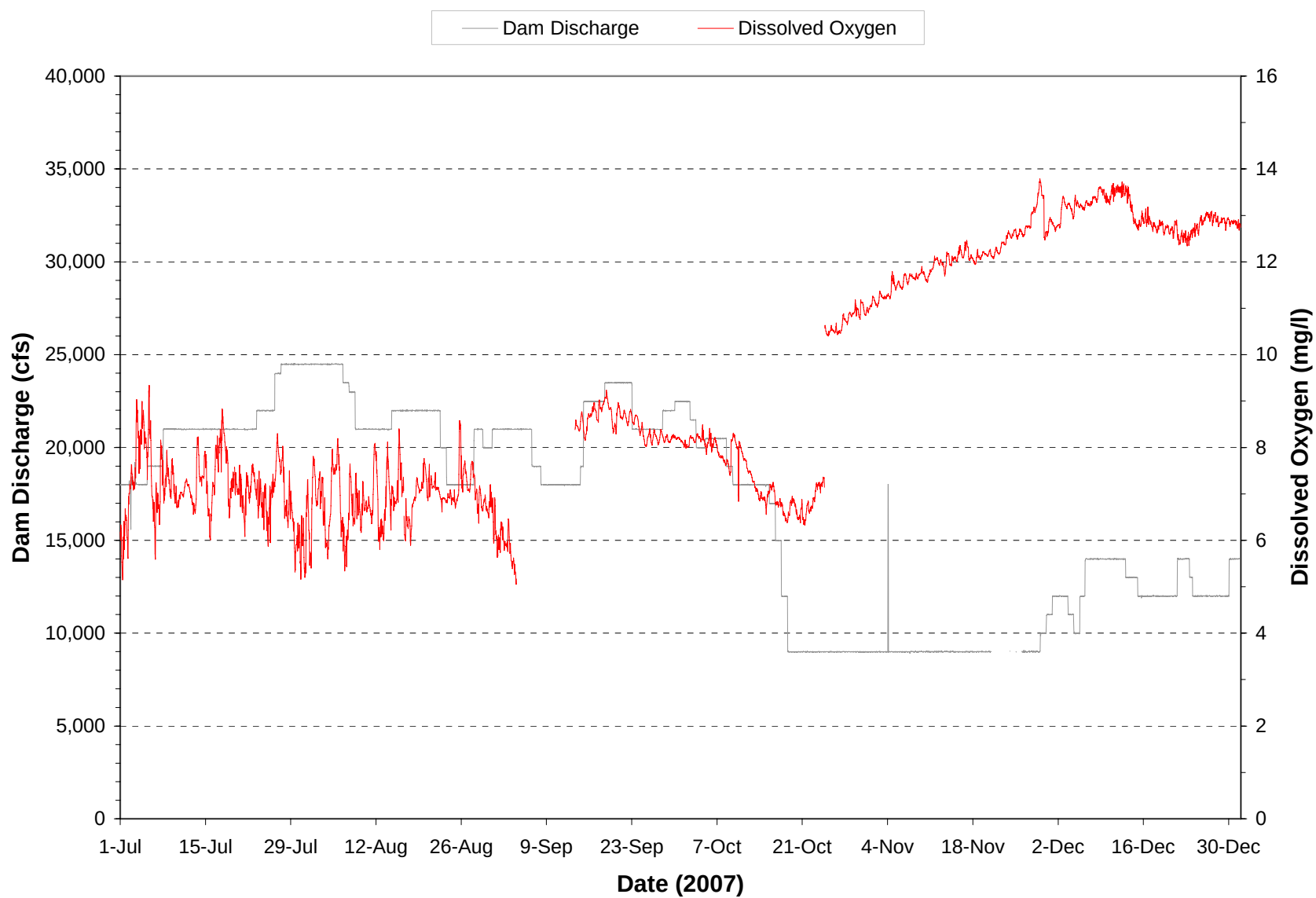
Plate 292. Hourly discharge and dissolved oxygen monitored at the Gavins Point powerplant on water discharged through the dam during the period July through December 2007. (Note: Gaps in dissolved oxygen plot represents periods when monitoring equipment was not operational.)
