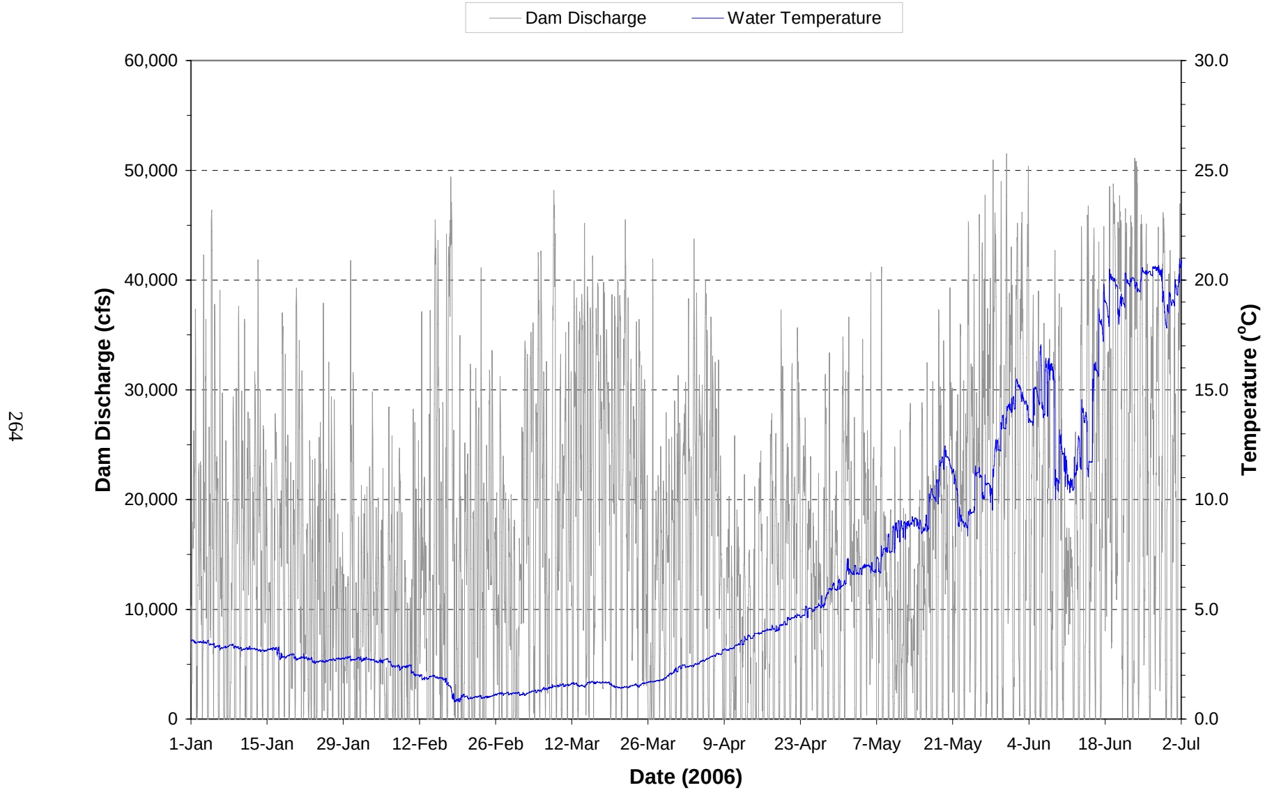
Plate 161. Hourly discharge and water temperature monitored at the Oahe powerplant on water discharged through the dam during the period January through June 2006.
