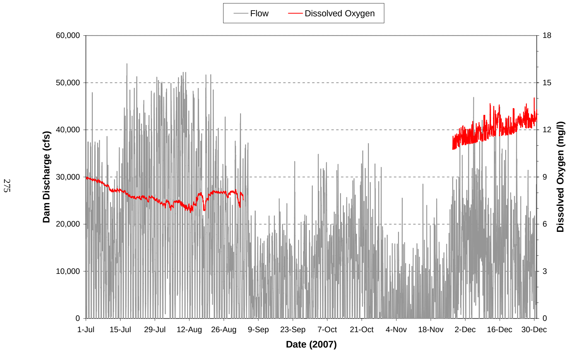
Plate 172. Hourly discharge and dissolved oxygen monitored at the Oahe Powerplant on water discharged through the dam during the period July through December 2007. (Note: Gaps in dissolved oxygen plot represents periods when monitoring equipment was not operational.)
