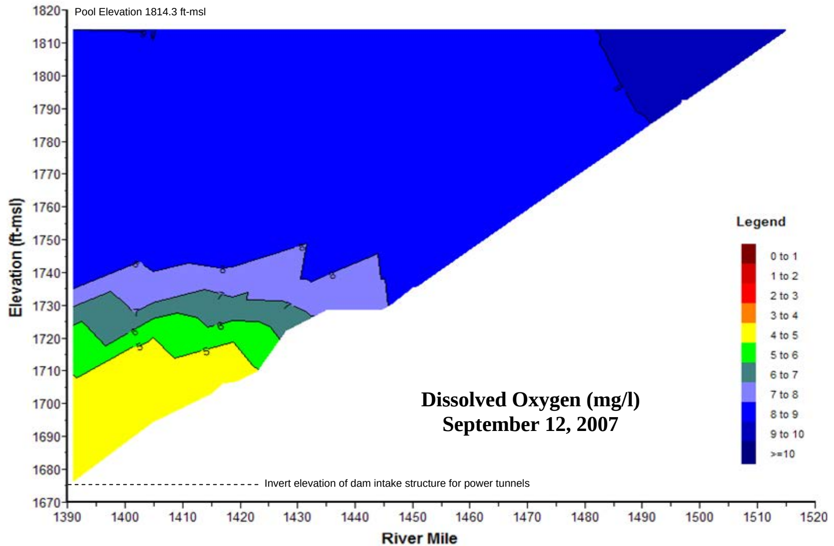
Plate 71. Longitudinal dissolved oxygen (mg/l) contour plot of Garrison Reservoir based on depth-profile dissolved oxygen concentrations measured at sites GARLK1390A, GARLK1412DW, GARLK1445DW, GARLK1481DW, and GARNFMORRR1 on September 12, 2007.
