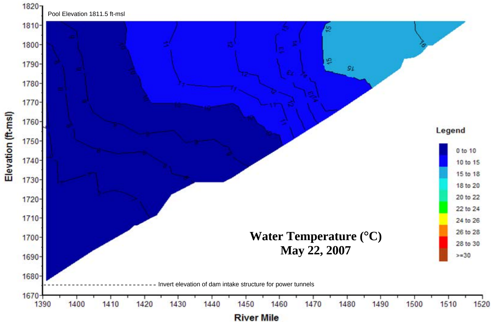
Plate 60. Longitudinal water temperature (°C) contour plot of Garrison Reservoir based on depth-profile water temperatures measured at sites GARLK1390A, GARLK1412DW, GARLK1445DW, GARLK1481DW, and GARNFMORRR1 on May 22, 2007.
