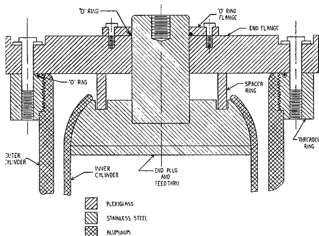
Figure 2. PFL End Details
