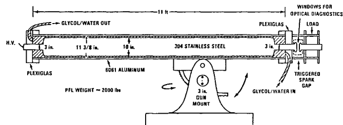
Figure 1. Pulse Forming Line
