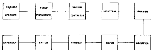
Figure 3. Block Diagram of Charging System
