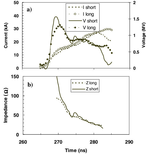
Figure 6. a) Voltage and current waveforms and b) impedance waveforms for long (shot 218) and short (shot 313) cathodes.
