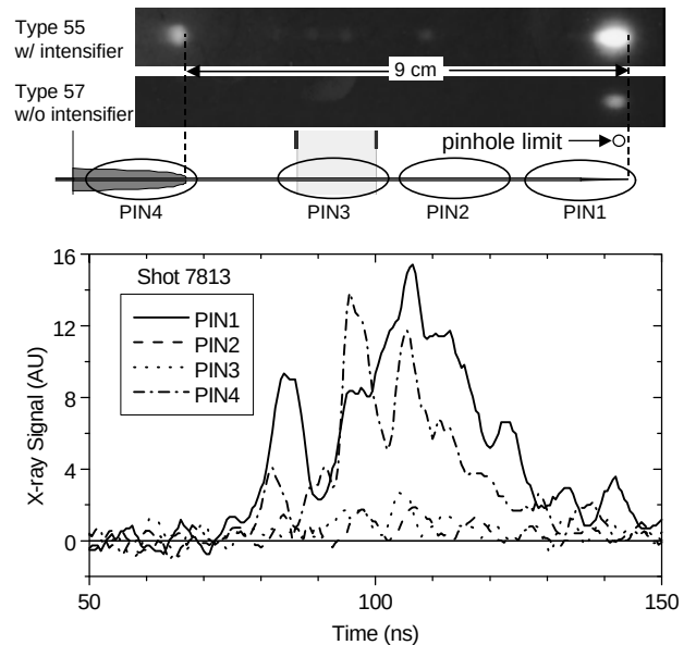
Figure 5. Side-on x-ray pinhole camera images, electrode configuration, and PIN diode signals for shot 7813.
