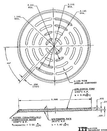
FIGURE 6 MOLYBDENUM/COPPER LAMINATE GRID
