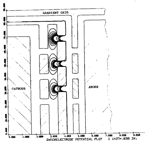
FIGURE 7 EQUIPOTENTIAL FIELD LINE PLOT
