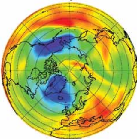
Ozone Mixing Ratio 3 mb
