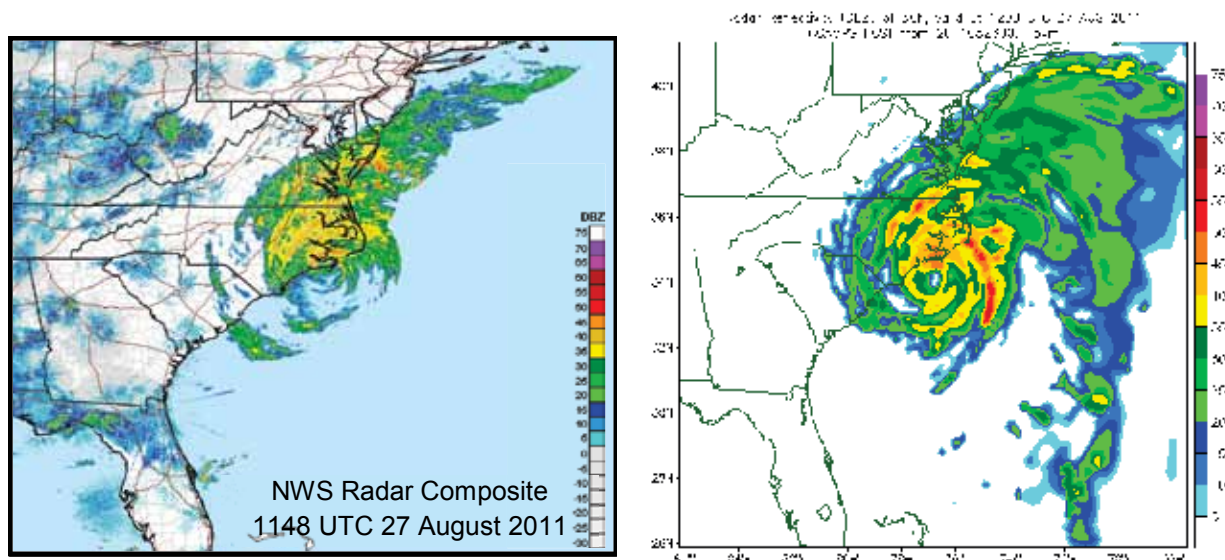
FIGURE 2 The NWS composite radar reflectivity valid at 1148 UTC 27 August 2011 (left panel) (source NOAA) and the COAMPS-TC 36 h forecast radar reflectivity performed in real time and valid at 1200 UTC 27 August (right panel) for Hurricane Irene. The COAMPS-TC reflectivity is shown for the second grid mesh, which has a horizontal resolution of 15 km.
