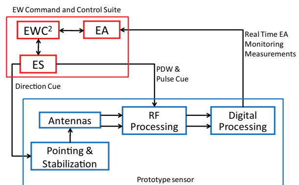
FIGURE 5 Illustration of how the prototype sensor will fit within the EW command and control suite. The sensor will receive direction cueing and pulse descriptor words (PDW) from the ES sensors.
