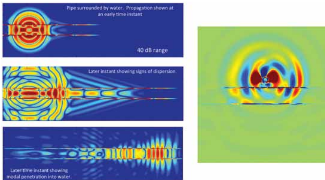
Snapshots of acoustic wave propagation showing the dispersion of a simple pulse into guided waves supported by the oil-steel-water pipe system (left panel). Acoustic scattering of the water-penetrating guided acoustic wave mode by a spherical elastic object exterior to the pipe (right panel).
