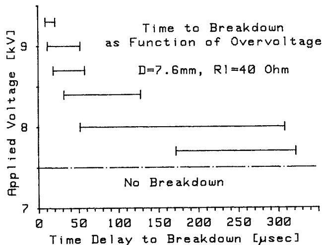
Fig. 4 - Time delays to breakdown (measured for 40 discharges each) as function of overvoltage on discharge. E-beam current 1.75 A, 1 \mu sec pulsewidth, 760 Torr methane.
