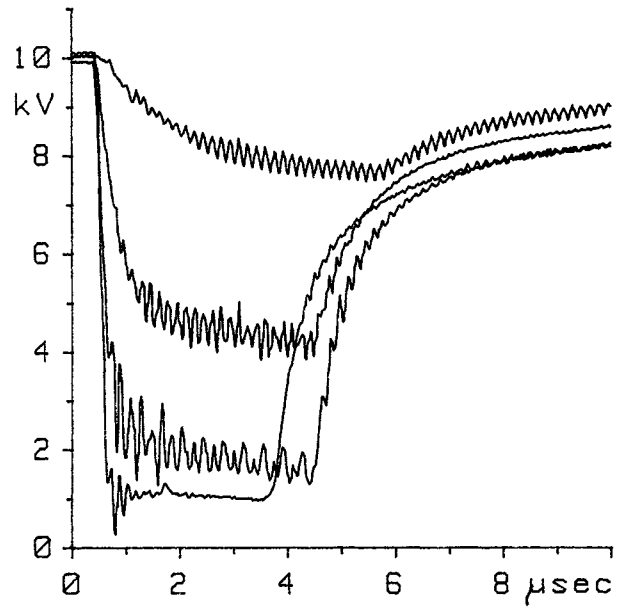
Fig. 6 - Discharge voltage for E-beam currents (from top) of .05, 0.4, 1 and 1.6 A, 40 ohm load, 760 Torr methane.
