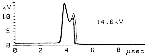
Fig. 5 - Time delays to breakdown, inductive load (225 \mu H) for two overvoltages. Time scale is enlarged to show inductive peak pulse only (compare with Fig. 1). Maximum peak pulse voltage with no breakdown for these conditions: 12.2 kV.
