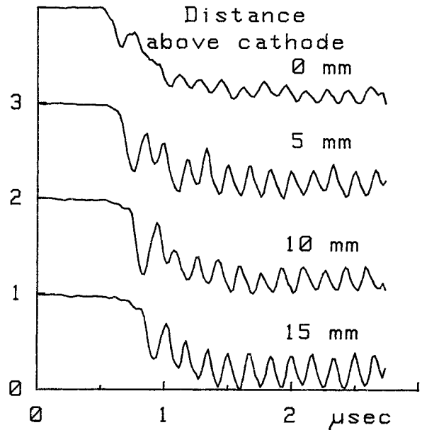
Fig. 7 - Spatially resolved optical radiation from discharge at 4 different positions above cathode.
